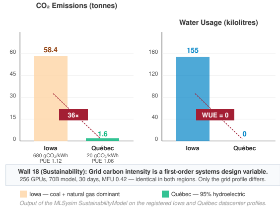
Figure 8: Geography as a Systems Variable: Iowa vs. Québec. An identical 256-GPU cluster training a 70B model for 30 days produces 36 \times more CO 2 in Iowa (coal/gas grid circa 2020, 680 \text{ gCO}_2/\text{kWh} , PUE 1.12) than in Québec (95% hydroelectric, 20 \text{ gCO}_2/\text{kWh} , PUE 1.06): 58.4 vs. 1.6 tonnes. Water usage diverges even more sharply because Québec’s registered WUE is zero. Hardware, model, parallelism strategy, and MFU are identical; only the regional grid profile differs between the two sites.
