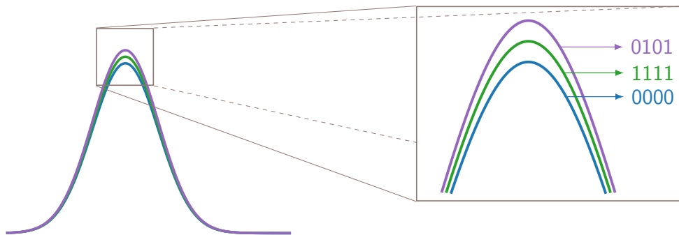
Figure 13.17: Power traces: Cryptographic computations reveal subtle, data-dependent variations in power consumption that reflect internal states during specific operations.
