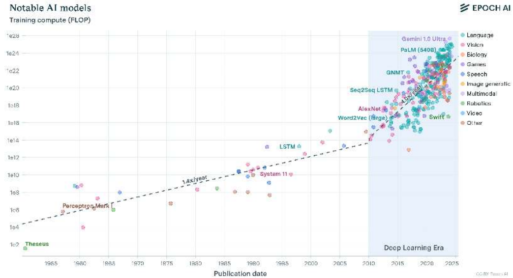
Figure 1.6: Model training compute trends: Training compute has grown exponentially, accelerating dramatically in the deep learning era. The fitted trends shift from roughly 1.4\times per year before 2010 to roughly 4\times per year inside the deep learning era, both far steeper than Moore’s Law ( \sim 2 years). The fastest stretch was steeper still: within the 2012–2019 frontier subset, compute doubled approximately every 3.4 months. This trajectory explains why efficiency has become a strategic imperative rather than an optional optimization.
