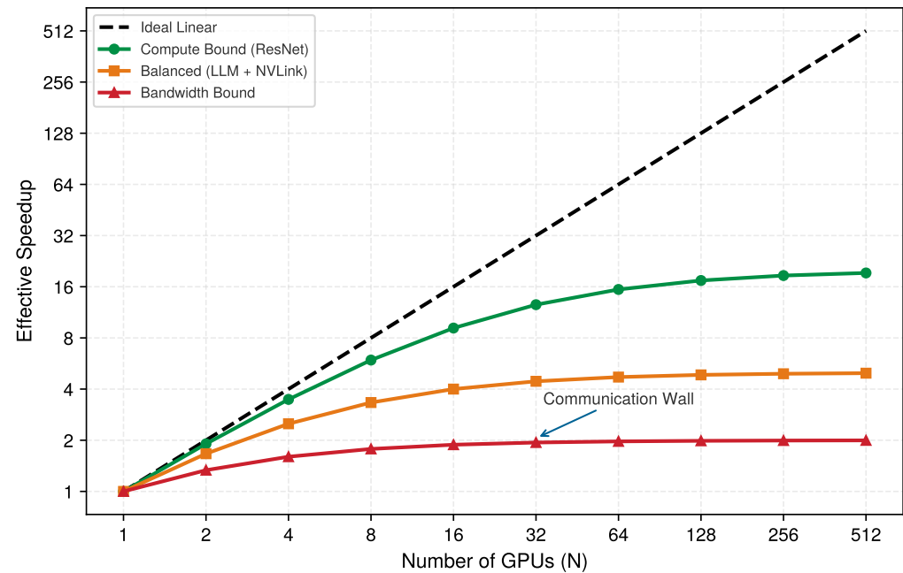
Figure 5.8: The scaling tax: Effective speedup vs. number of GPUs. While ideal scaling (dashed black) is linear, real-world systems pay a ‘tax’ for communication. Compute-bound models like ResNet (green) scale well because they have high arithmetic intensity. Bandwidth-bound models like GPT-3 (red) hit a communication wall where adding more GPUs yields diminishing returns (efficiency < 50 percent).
