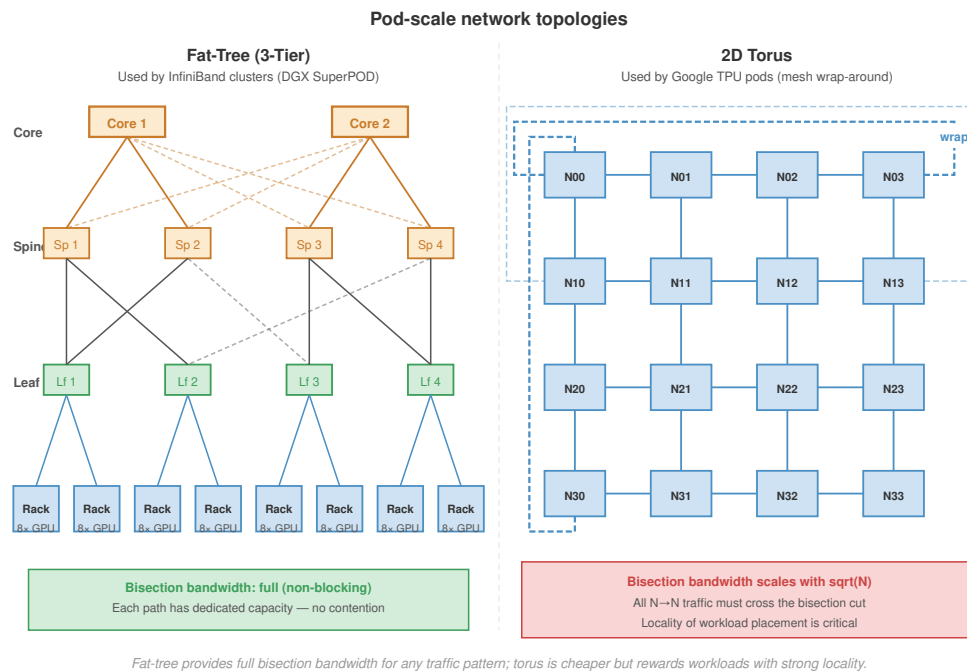
Figure 2.14: Pod-scale network topologies: Two dominant pod topologies compared. (Left) Fat-tree (3-tier) with leaf, spine, and core tiers: full bisection bandwidth, used by InfiniBand clusters such as DGX SuperPOD. (Right) 2D torus with wrap-around links: bisection bandwidth scales as \mathcal{O}(\sqrt{N}) , cheaper at scale but rewards workloads with strong locality; used by Google TPU pods. The choice shapes which parallelism strategies run efficiently.
