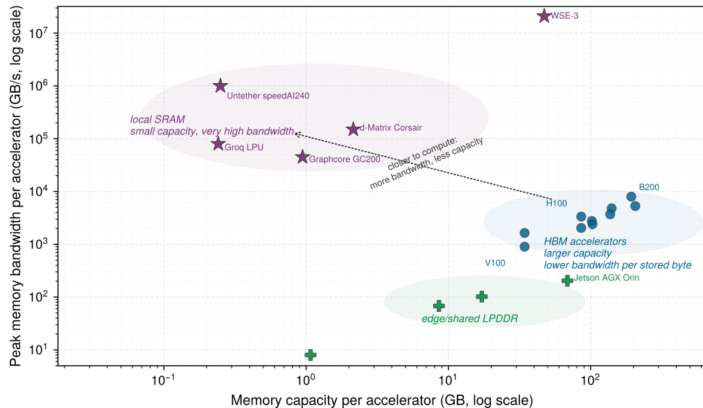
Figure 2.6: Accelerator memory tiers: Peak memory bandwidth and capacity separate local-SRAM designs, HBM accelerators, and edge/shared-LPDDR devices. The dotted arrow marks the design trade-off: moving data closer to compute raises bandwidth but reduces capacity.
