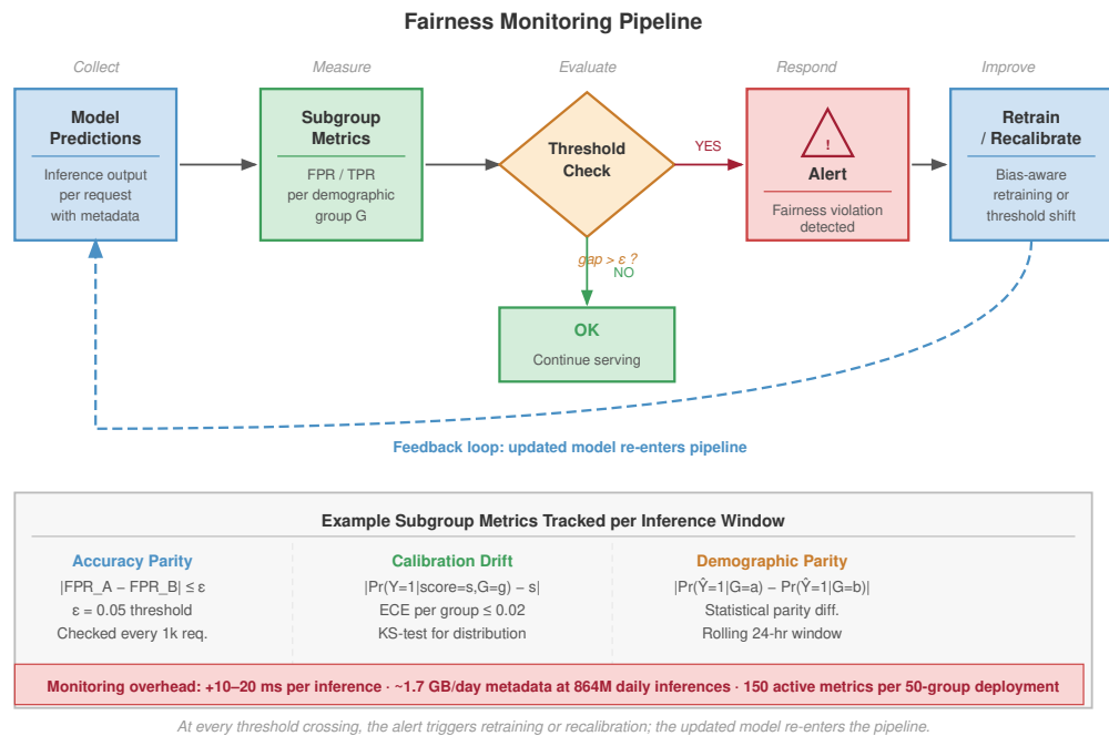
Figure 16.10: Fairness Monitoring Pipeline: End-to-end observability for deployed models. Model predictions feed subgroup metric computation across demographic segments; a threshold check identifies performance or fairness regressions; and alerts trigger automated retraining or manual review. This continuous feedback loop ensures that responsible AI properties are maintained postdeployment.
