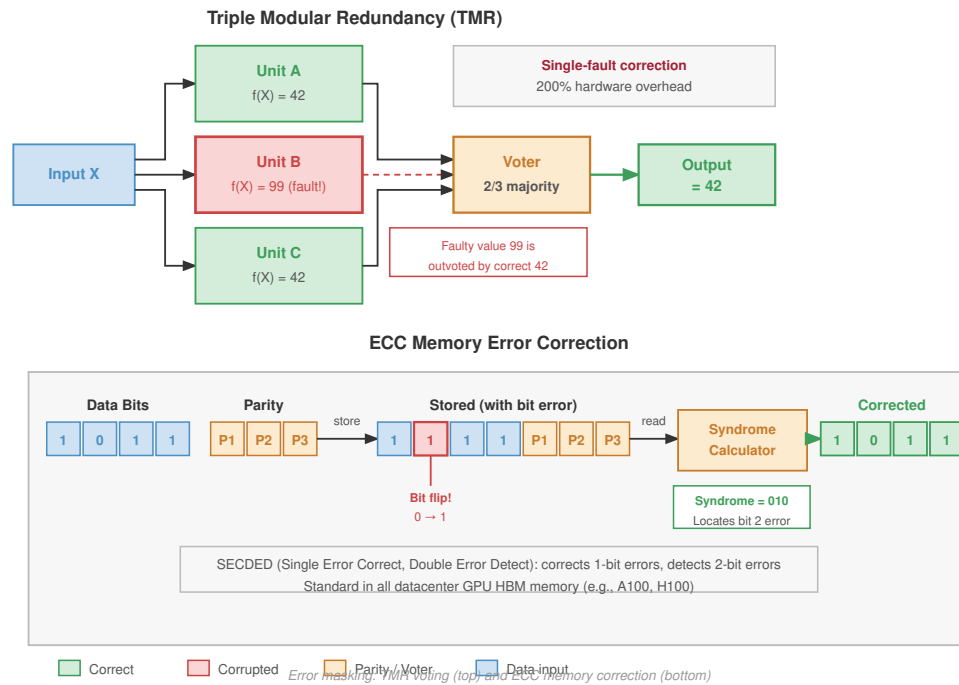
Figure 7.22: Error masking via voting: In triple modular redundancy, the same computation runs on three independent units. A voter circuit takes a majority vote of the results. Even if one unit suffers a fault (for example, bit flip), the system ‘masks’ the error by selecting the matching outputs from the other two units, allowing continuous operation without interruption.
