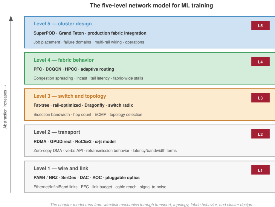
Figure 3.1: The five-level network model for ML training: Five layered levels span from the physical wire to cluster-scale design. Level 1, Wire and Link: PAM4/NRZ signaling, SerDes, direct attach copper (DAC), active optical cable (AOC), pluggable optics, Ethernet and InfiniBand link layers. Level 2, Transport: RDMA, GPUDirect, RoCEv2, zero-copy DMA, and the \alpha - \beta communication model. Level 3, Switch and Topology: fat-tree, rail-optimized, Dragonfly, adaptive routing. Level 4, Fabric Behavior: priority flow control (PFC), DCQCN, HPCC congestion control, adaptive routing, incast handling. Level 5, Cluster Design: NVIDIA SuperPOD, Meta Grand Teton, and other production fabric integrations.
