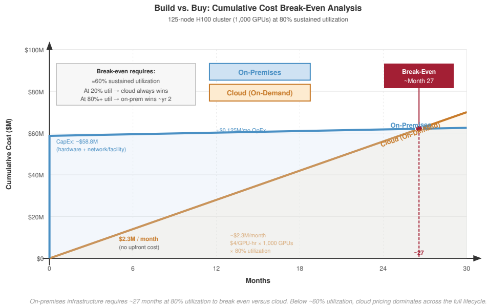
Figure 12.3: Build vs. buy TCO: The curves compare cumulative cost over a 30-month horizon for a high-utilization H100 reference cluster. On-premises deployment begins with a CapEx step plus monthly OpEx, whereas cloud rental cost rises linearly.
