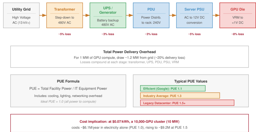
Figure 2.11: The power delivery path: The journey of energy from the high-voltage grid to the low-voltage transistor involves multiple conversion stages, each with its own efficiency loss. The cumulative delivery loss, combined with overhead for cooling (measured by PUE), dictates how much power a facility must draw from the grid. The critical engineering challenge is the rack power distribution unit (PDU) to voltage regulator module (VRM) transition, where 10–40 kW of power must be delivered within a single cabinet.
