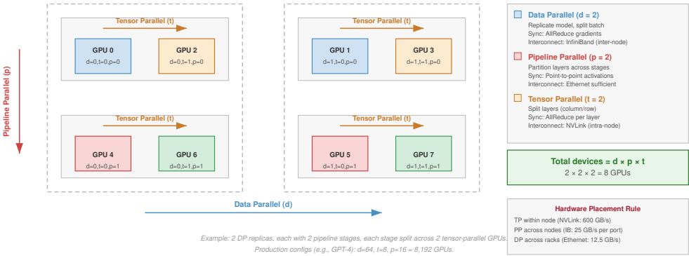
Figure 5.19: 3D parallelism strategy space: An 8-GPU configuration fills a (d, p, t) coordinate grid that combines data parallelism (replicas), pipeline parallelism (layer stages), and tensor parallelism (within-layer splits). One training step coordinates d \times p \times t GPUs, with communication occurring within layers, at microbatch stage boundaries, and once per optimizer step, respectively.
