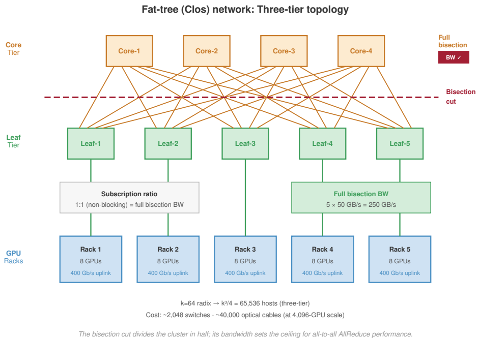
Figure 3.9: Nonblocking fat-tree topology: A three-tier Clos network built from radix- k switches. By ensuring that the number of uplinks at each level matches the number of downlinks, the topology provides full BW_{\text{bisection}} between any two pods. The multiple parallel paths between leaf and spine enable hardware-based adaptive routing to spray packets and avoid congestion.
