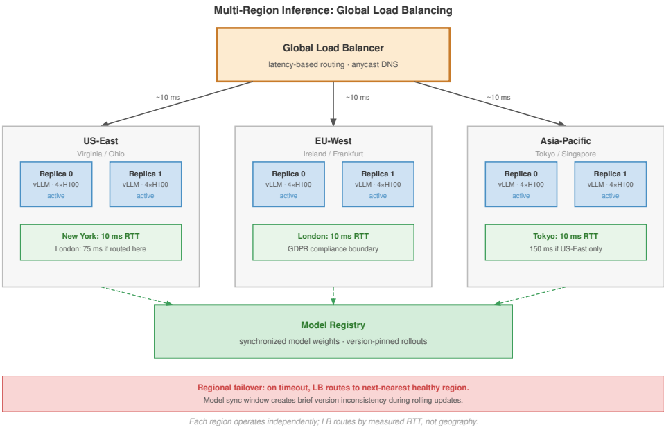
Figure 10.23: Global load balancing across inference regions: A global load balancer routes requests to three independent regional deployments (US-East, EU-West, Asia-Pacific) based on latency. Each region operates independently; a shared model registry synchronizes weights. During regional failure, the LB reroutes to the next nearest healthy region.
