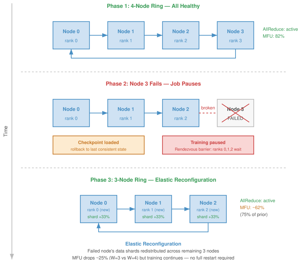
Figure 7.27: Elastic training recovery: Unlike static training which aborts on failure, elastic training adapts. When a worker fails, the job pauses, redistributes the dataset and model shards across the remaining N - 1 workers, and resumes training from the last consistent state. This capability transforms hard failures into temporary throughput degradations.
