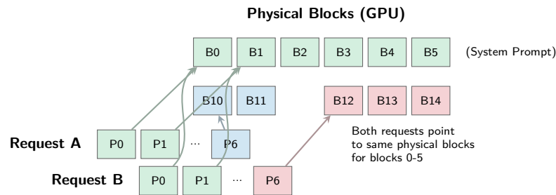
Figure 10.11: Prefix caching via block sharing: PagedAttention enables efficient prefix caching by allowing multiple sequences’ block tables to point to the same physical blocks for shared content. In this example, the System Prompt is stored in blocks 0-5. Request A and Request B map their first 6 logical pages to these same physical blocks, storing only their unique suffixes in new blocks. This dramatically reduces memory usage and prefill computation for workloads with shared context.
