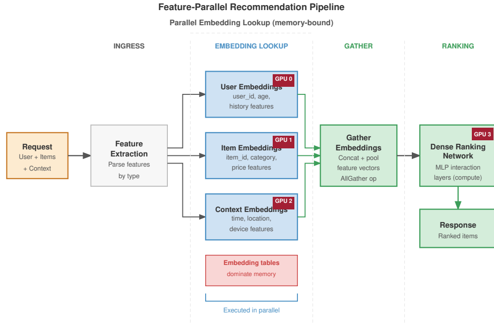
Figure 10.7: Feature-parallel batching pipeline: Requests are batched by feature type (Users, Items, Context) and dispatched to specialized embedding servers in parallel. The retrieved embeddings are then concatenated and processed by the dense ranking head. This architecture enables scaling to trillions of parameters by decoupling embedding storage from dense compute.
