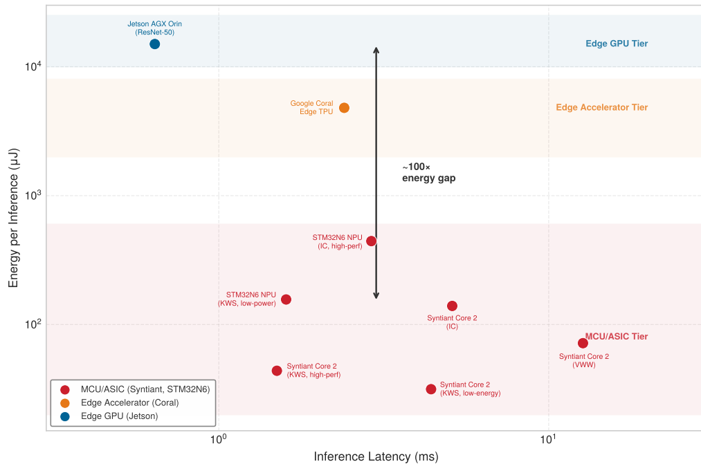
Figure 11.7: The edge inference landscape: Published inference latency and energy measurements from MLPerf Tiny and official benchmarks reveal three distinct hardware tiers separated by approximately 100× in energy consumption. Dedicated neural processors (Syntiant, STM32N6) achieve keyword spotting in under 5 ms at 30–160 microjoules, while edge GPUs (Jetson Orin) deliver sub-millisecond latency at 15 mJ.
