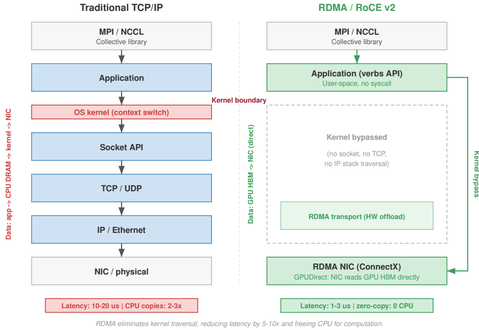
Figure 3.7: Traditional TCP/IP vs. RDMA/RoCE v2 stacks: The traditional TCP/IP path (left) traverses the application, OS kernel (context switch), Socket API, TCP/UDP, IP/Ethernet, and NIC, with latency of 10–20 \mu s and two to three CPU-mediated copies. The RDMA/RoCE v2 path (right) exposes a user-space Verbs API that bypasses the kernel, offloading transport to the RDMA NIC (GPUDirect reads GPU HBM directly), with latency of 1–3 \mu s and zero-copy CPU overhead.
