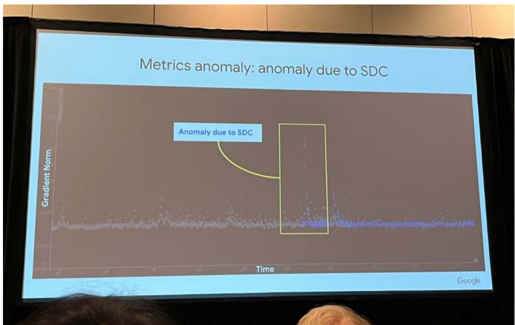
Figure 7.8: Gradient norm deviation: Transient hardware faults, such as silent data corruption (SDC), can disrupt optimization by causing abrupt changes in gradient norms. Google's production examples show SDC anomalies surfacing as visible gradient-norm spikes. Source: (Dean 2024).
