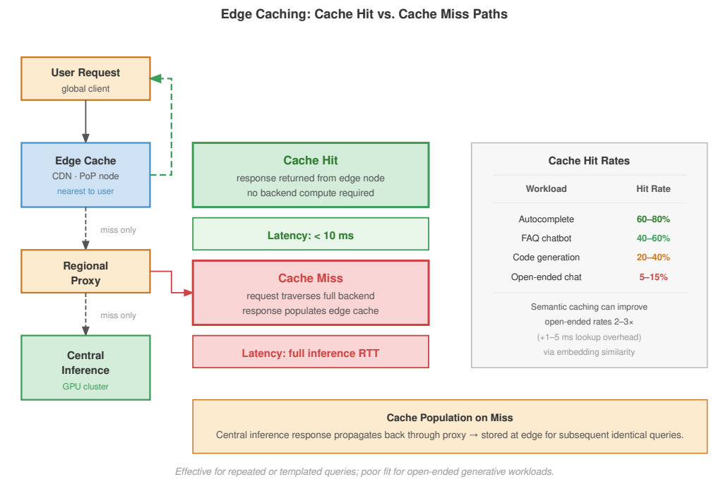
Figure 10.24: Cache hit and cache miss paths at the edge: A cache hit returns immediately from the CDN edge node (<10 ms). A cache miss flows through to central inference and populates the cache on return. Hit rate determines the effective cost saving; open-ended generative workloads have low repeatability and benefit little from this pattern.
