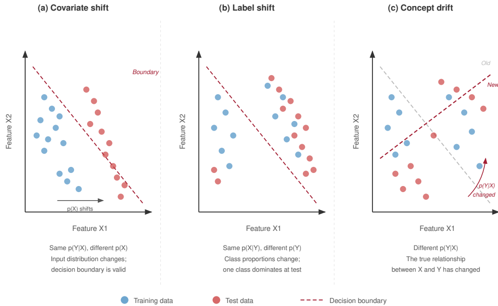
Figure 14.9: Types of distribution shift: Covariate shift changes p(x) while holding p(y | x) fixed; label shift changes p(y) while holding p(x | y) fixed; and concept drift changes p(y | x) . Distinguishing these cases determines whether reweighting, recalibration, or model adaptation is appropriate.
