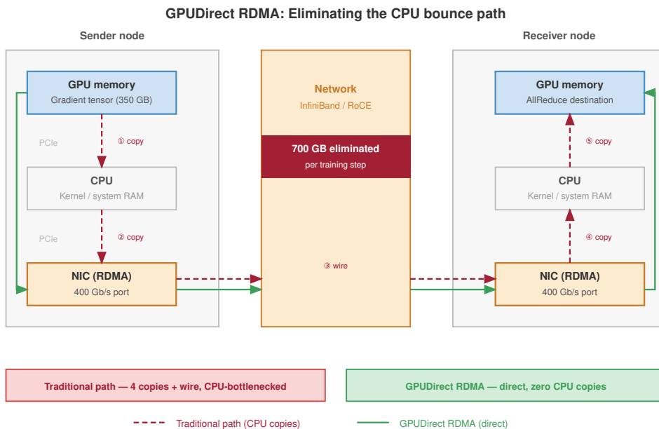
Figure 3.6: GPUDirect RDMA data path: The red traditional path stages an accelerator payload in registered host memory before the NIC reads it. The green GPUDirect path lets the NIC access GPU memory over PCIe, eliminating the host-memory bounce.
