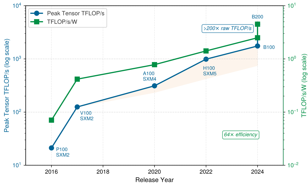
Figure 2.5: The accelerator efficiency wall: Peak Tensor Core throughput (blue, left axis) and power efficiency (green, right axis) for six generations of NVIDIA data center GPUs, both on logarithmic scales. The series follows the advertised low-precision Tensor Core mode for each generation, so precision changes are part of the hardware trend rather than an apples-to-apples FP16 comparison. Raw throughput has grown over 200× from the P100 to the B200, but efficiency (TFLOP/s per watt) has grown far less. The shaded region highlights the widening gap that the power grid, cooling systems, and data center infrastructure must absorb.
