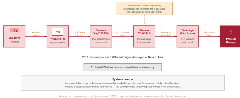
Figure 13.2: Stuxnet: The attack chain targeted PLCs through Windows and Siemens software vulnerabilities, allowing digital malware to damage physical infrastructure. ML systems face an analogous trust-boundary problem when training data, dependencies, or model weights are compromised.
