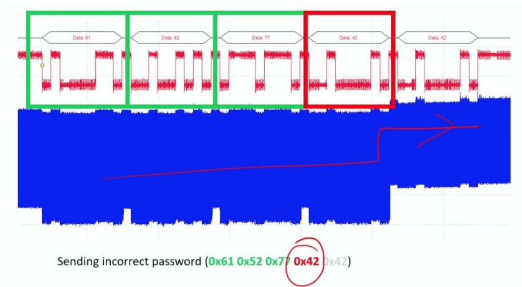
Figure 13.14: Side-channel attack vulnerability: Power consumption patterns reveal cryptographic key information during authentication; consistent power usage indicates correct password bytes, while abrupt changes signal incorrect input and halted processing. Even without knowing the password, an attacker can infer it by analyzing the device's power usage during authentication attempts. Source: Colin O'Flynn.
