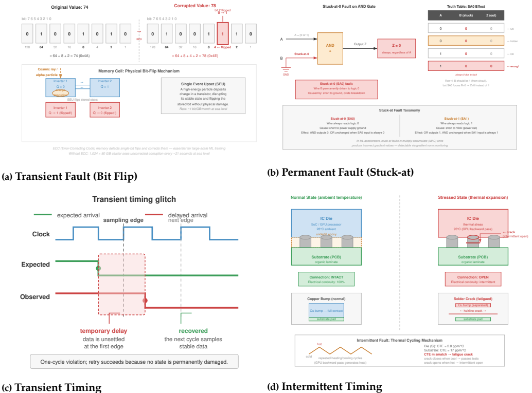
Figure 7.13: Temporal taxonomy of hardware faults: Four panels show how the three temporal categories manifest in practice. Transient panels (bit flip and timing glitch) show temporary disruptions that do not cause permanent damage. The intermittent panel shows sporadic errors driven by unstable conditions or aging. The permanent panel (stuck-at-0/1) shows irreversible physical damage that requires replacement.
