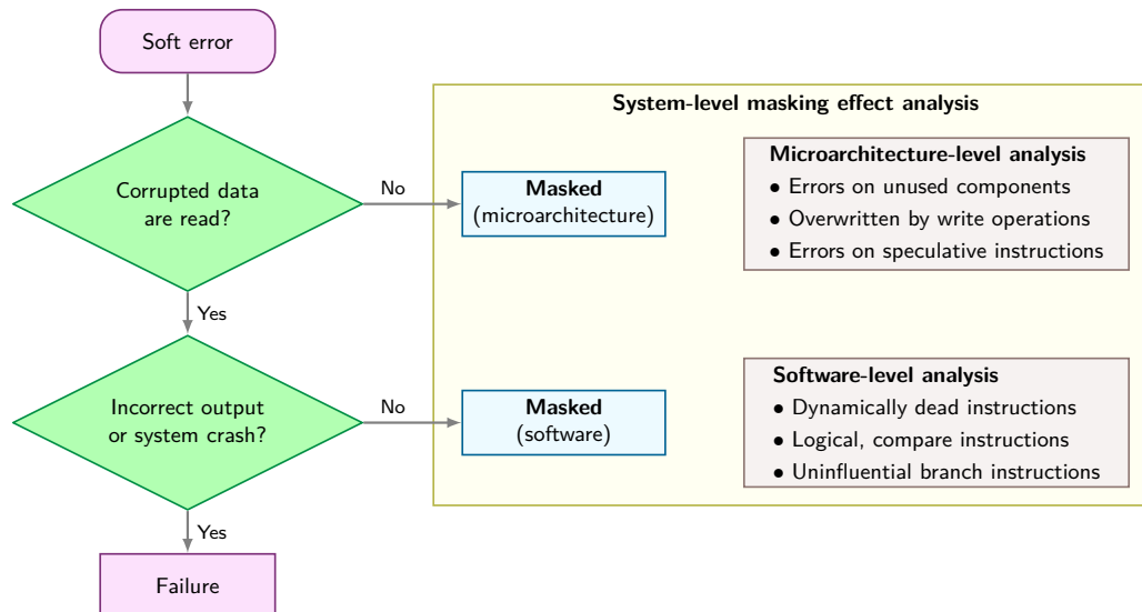
Figure 7.23: Error masking: Microarchitectural redundancy can absorb single-bit faults before they propagate to observable system errors, highlighting a discrepancy between hardware-level and software-level fault models. This figure details how fault masking occurs within microarchitectural components, demonstrating that software-based error detection tools may underestimate the true resilience of a system to transient errors.
