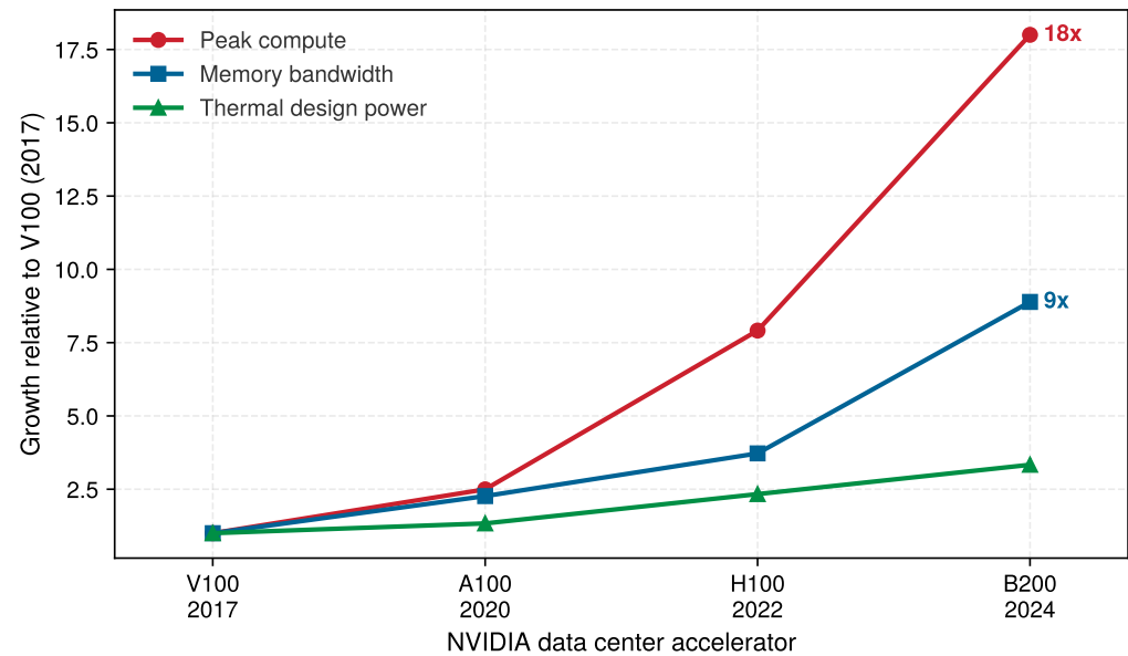
Figure 2.4: Compute, bandwidth, and power scale at three different rates: Peak compute, memory bandwidth, and thermal design power for NVIDIA data center accelerators, normalized to the V100. Compute rises 18×, bandwidth 8.9×, and TDP 3.3×, so each generation buys arithmetic faster than it buys the bytes or the watts to feed it. Specifications come from the MLSysIM hardware registry.
