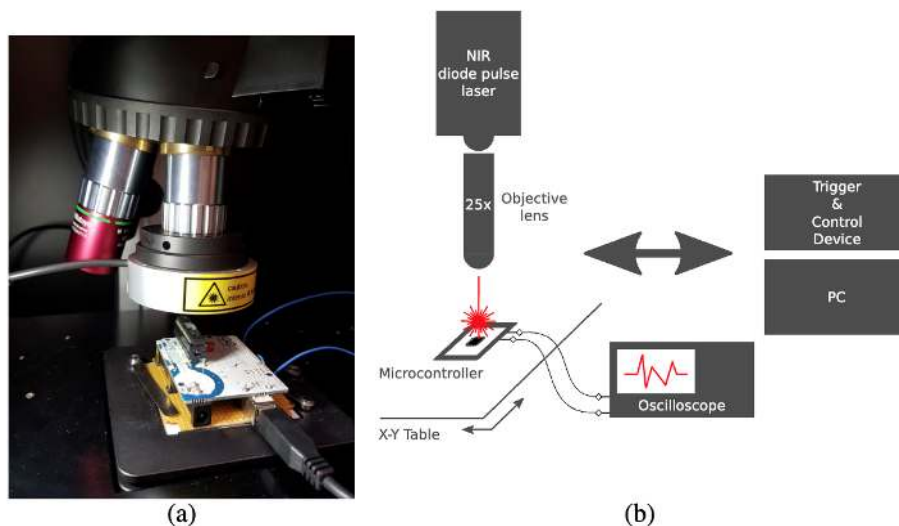
Figure 13.11: Laser fault injection: Focused laser pulses induce bit flips within microcontroller memory, enabling attackers to manipulate model execution and compromise system integrity. Researchers use this technique to simulate hardware errors, revealing vulnerabilities in embedded machine learning systems and informing the development of fault-tolerant designs.
