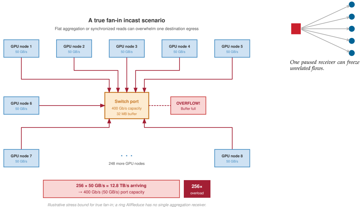
Figure 3.12: A true incast burst: This deliberately worst-case fan-in scenario sends 256 sources at 50 GB/s toward one 400 Gb/s (50 GB/s) egress with a 32 MB buffer. The 12.8 TB/s offered load oversubscribes the destination egress by 256×. Flat aggregation or synchronized reads can create this pattern; bandwidth-optimal ring AllReduce does not, because each rank exchanges point-to-point chunks.
