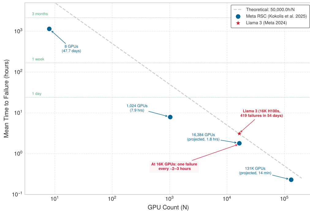
Figure 7.5: Published failure rates from production clusters: Measured MTTF values and fitted projections from Meta’s RSC clusters (Kokolis et al. 2025) plotted with Llama 3 training measurements (Dubey et al. 2024) against the theoretical 1/N curve. At 16,384 GPUs, the Kokolis projection and Llama 3 empirical measurement both fall in the 2-to-3-hour failure range, confirming that fault tolerance is a mathematical necessity, not an edge case. Data sources: Kokolis et al., arXiv:2410.21680; Meta, arXiv:2407.21783.
