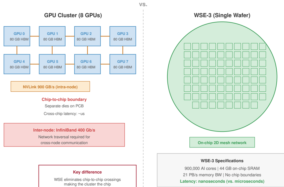
Figure 2.2: Wafer-scale engine (WSE) architecture: Unlike a cluster assembled from discrete packages and boards, a WSE uses most of a 300 mm wafer as one routed compute fabric. Defect-aware software routes around unusable regions, while the on-wafer mesh and distributed SRAM replace off-package transfers for mapped operations.
