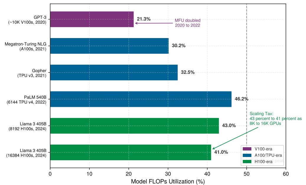
Figure 5.17: The MFU progression: Model FLOPs Utilization across published training systems, ordered chronologically. MFU doubled from 21 percent (GPT-3, 2020) to 46 percent (PaLM, 2022) through advances in hybrid parallelism and communication overlap, then plateaued near 40–45 percent for large-scale runs. The Llama 3 data points illustrate the scaling tax: MFU drops from 43 percent at 8,192 GPUs to 41 percent at 16,384 GPUs as communication overhead grows with cluster size. Data sources: Chowdhery et al. (2022), Dubey et al. (2024).
