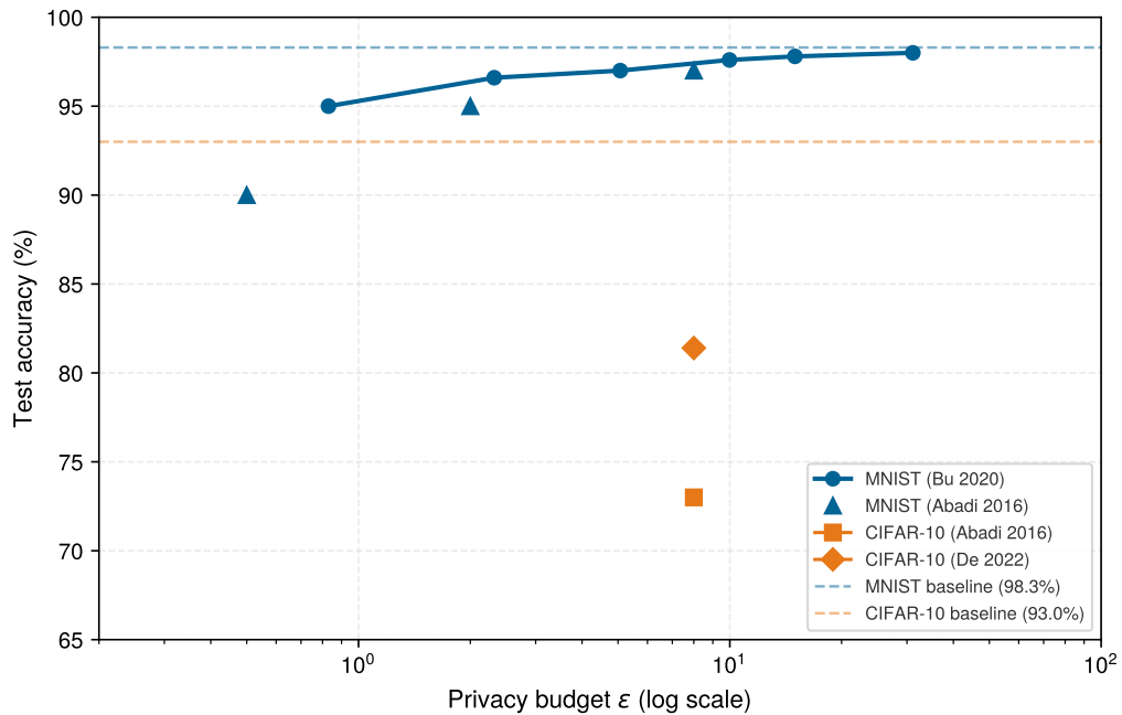
Figure 13.26: Published privacy-utility results: Accuracy at selected privacy budgets from (Abadi et al. 2016; Bu et al. 2020; De et al. 2022). MNIST stays comparatively accurate under single-digit epsilon budgets in these experiments, while CIFAR-10 trained from scratch without extra data remains harder, with De et al. reporting 81.4 percent at \epsilon = 8 . Comparisons require the full mechanism, accountant, adjacency relation, training regime, and data rather than epsilon alone.
