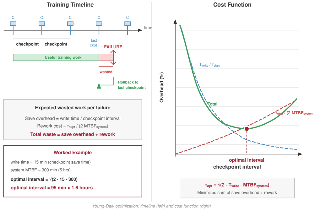
Figure 7.4: The Young-Daly optimal checkpoint: Total wasted work is the sum of checkpointing overhead (which decreases with interval \tau_{\text{ckpt}} ) and rework cost (which increases with \tau_{\text{ckpt}} ). The minimum point defines the optimal interval
