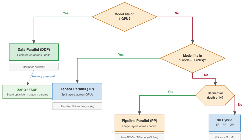
Figure 5.3: Parallelism strategy decision tree: Starting from the model’s memory requirements, the tree follows the constraints that determine which parallelism strategies are physically feasible. The critical branches compare model memory with single-GPU and single-node capacity; leaf nodes identify the resulting strategy and dominant hardware constraint.
