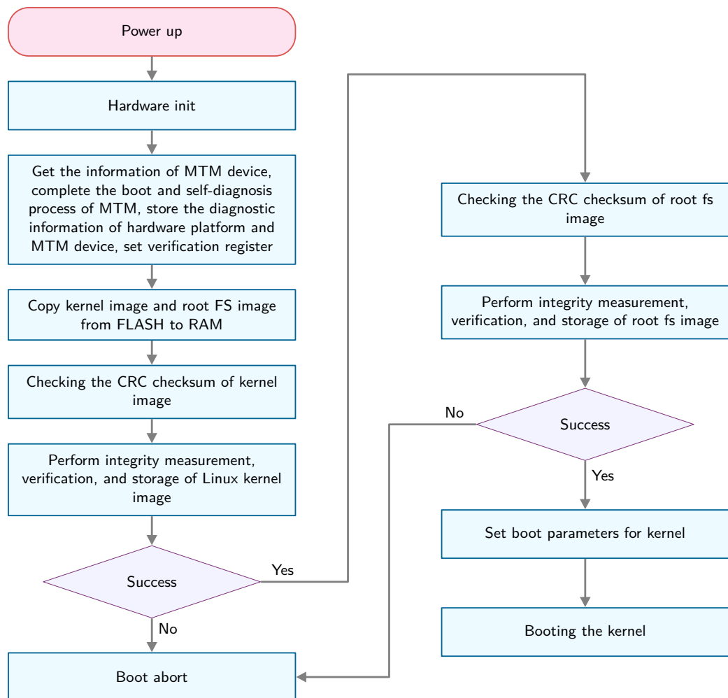
Figure 13.23: Secure boot sequence: Embedded systems employ a layered boot process to verify firmware and software integrity, establishing a root of trust before executing machine learning workloads and protecting against preruntime attacks. This architecture ensures only authenticated code runs, safeguarding model data and preventing unauthorized model substitution or modification during deployment.
