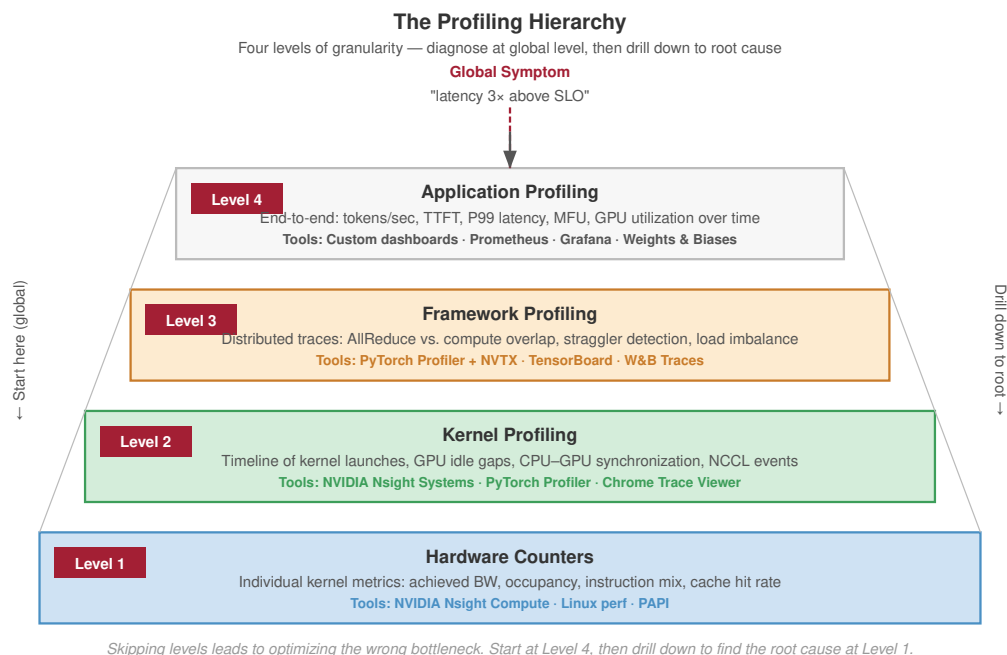
Figure 9.8: The profiling hierarchy: Diagnosis begins with application-level symptoms, then narrows through framework and kernel evidence to hardware counters. Each lower level trades breadth for the detail needed to isolate a root cause.
