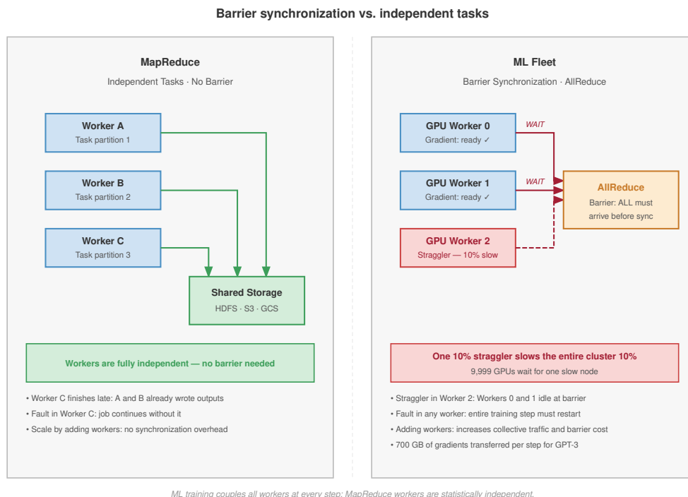
Figure 1.5: Barrier synchronization vs. independent tasks: MapReduce workers (left) operate independently, writing results to shared storage without coordination. A straggler delays only its own output. ML Fleet workers (right) must synchronize gradients at an AllReduce barrier every training step, meaning a single 10% straggler slows the entire cluster by 10%.
