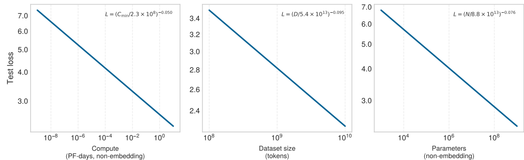
Figure 15.5: Model Scaling Laws: In the ranges studied by Kaplan et al. (2020), increasing model size, dataset size, and compute consistently reduced test loss. The figure reproduces source-paper notation, where N denotes parameter count and C_{\min} denotes compute; elsewhere this book uses P for parameter count and O for operation count. These scaling laws explain why larger models, more data, and increased compute became attractive design choices within that regime.
