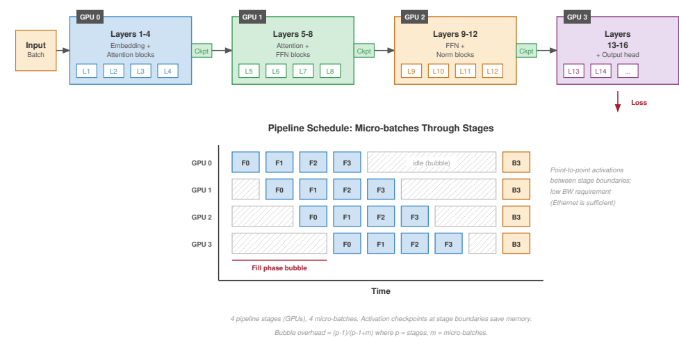
Figure 5.13: Layer-wise model parallelism: The upper path assigns four consecutive transformer blocks to each of four GPUs, with activation checkpoints at device boundaries. The lower schedule shows forward work in blue, backward work in orange, and hatched pipeline bubbles. Partitioning reduces the weight footprint per GPU to one-quarter of the model, but sequential dependencies leave downstream devices waiting during pipeline fill.
