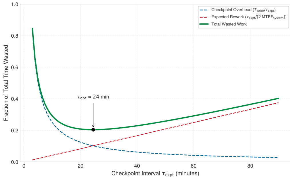
Figure 7.24: The checkpoint trade-off: Checkpoint save overhead decreases with longer intervals, but wasted computation from failures increases. The Young-Daly optimal interval minimizes total overhead. For an illustrative 175B-model cluster (~2.5-minute checkpoint writes, 2-hour MTBF), the optimal interval is approximately 24 minutes; the calculation that follows derives the exact interval for this chapter’s 10,000-GPU cluster.
