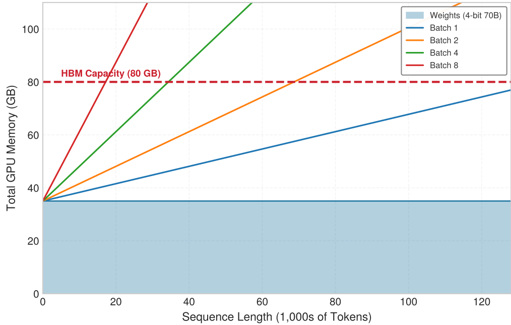
Figure 10.9: The KV cache wall: Total GPU memory usage for a 4-bit quantized 70B model (35 GB weights) on an 80 GB H100. While the model fits easily at small context lengths, the KV cache (sloped lines) eventually consumes all remaining HBM. At 128K context, a batch size of 2 is physically impossible on a single GPU (35 GB + 84 GB > 80 GB), forcing the system to either reduce batch size (killing throughput) or shard the model.
