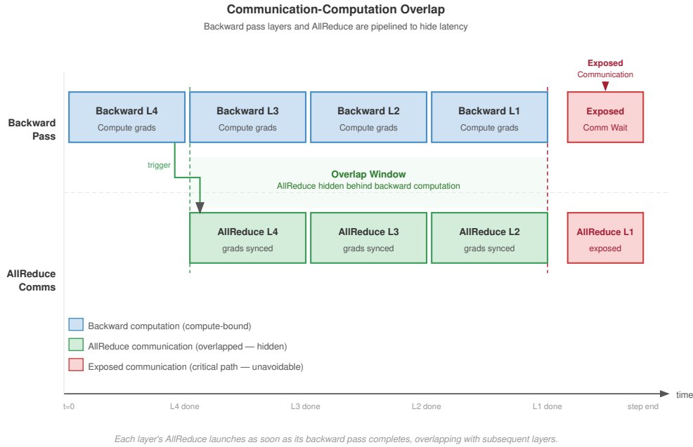
Figure 6.4: Communication-computation overlap: By pipelining collective operations with the backward pass, systems can hide network latency behind arithmetic execution. Overlap is successful only when the nonoverlappable overhead ( o ) is minimized, allowing the bulk transfer term to proceed while the GPU computes the next layer's gradients.
