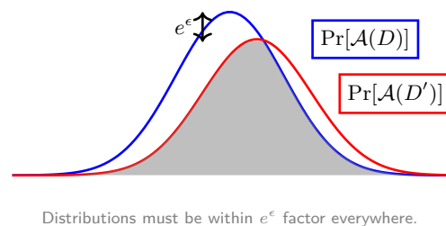
Figure 13.25: Differential privacy indistinguishability: Differential privacy bounds how much the output distribution can change between adjacent datasets D and D' . The privacy parameters limit, rather than eliminate, the information an observer can gain about any one individual's inclusion.
