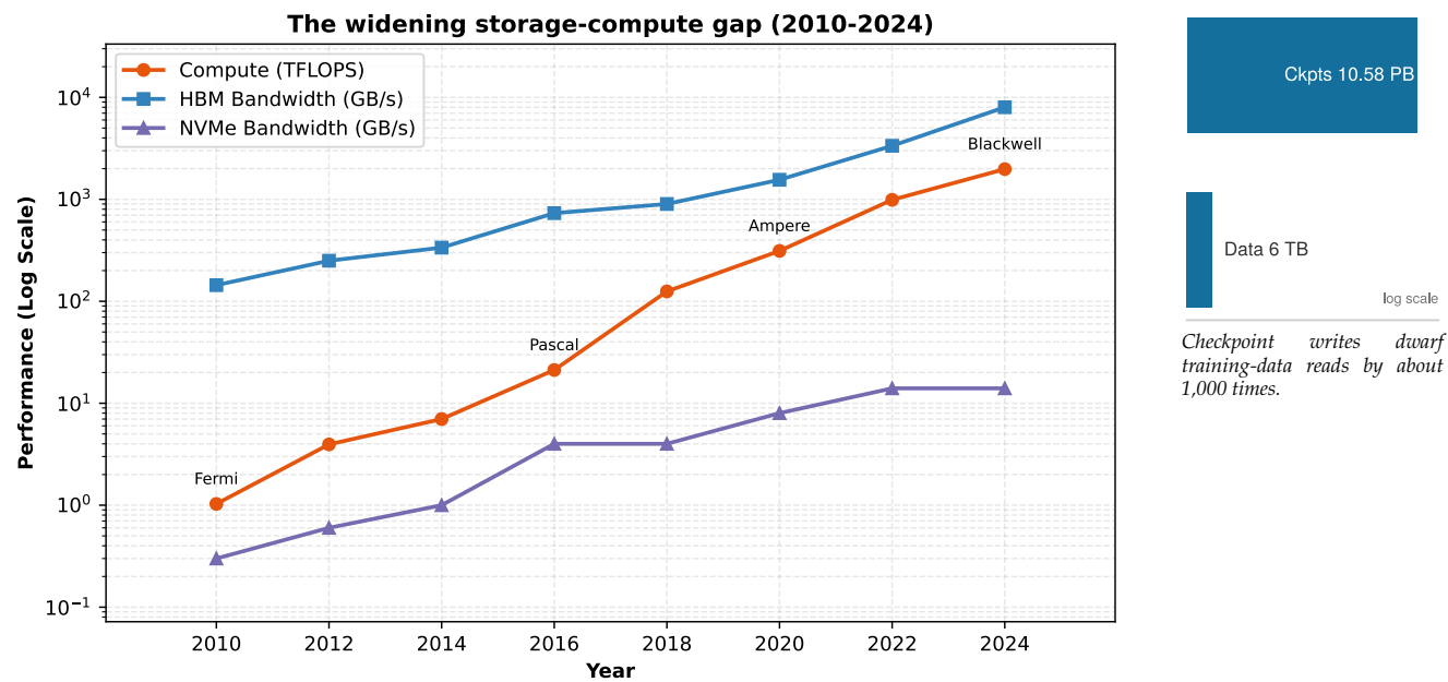
Figure 4.1: The storage-compute gap: Accelerator compute, HBM bandwidth, and NVMe bandwidth from 2010 to 2024 on a common log scale. Compute rises fastest and local storage slowest, so the fuel line into the accelerator becomes the binding constraint long before arithmetic does.
