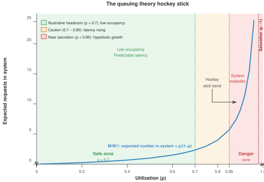
Figure F.1: The queuing hockey stick: For an M/M/1 queue, \rho_{\text{serv}}/(1 - \rho_{\text{serv}}) is the expected number of requests in the system, including the request in service. Its hyperbolic rise near saturation explains why production systems retain utilization headroom; the shaded operating bands are illustrative rather than universal thresholds.
