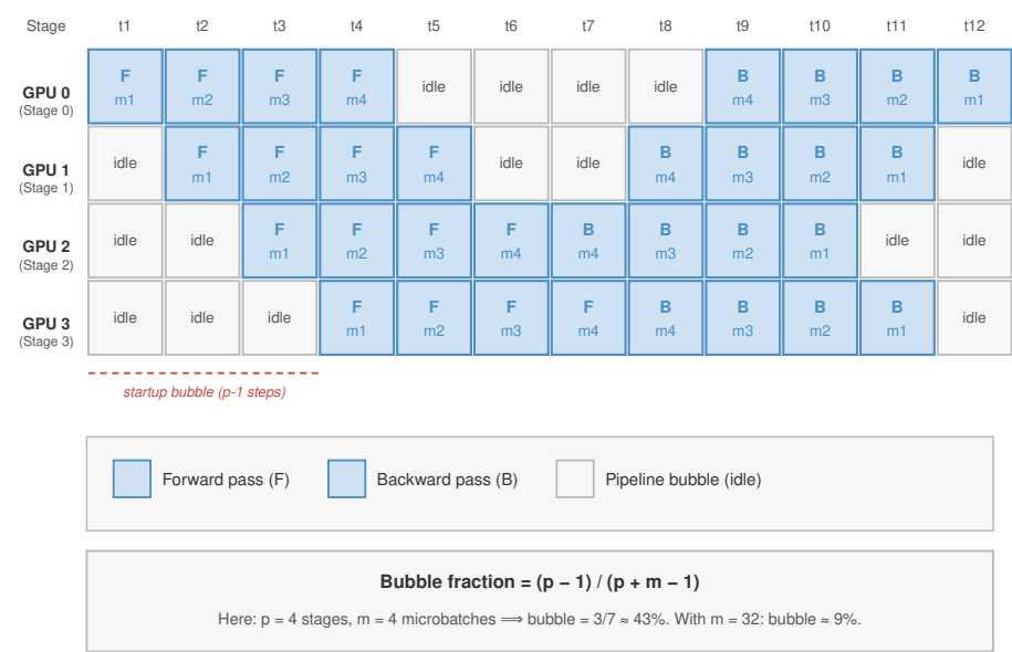
Figure 5.14: Pipeline parallelism schedule: A 4-stage pipeline processes 4 microbatches through forward passes ( F_{i,j} ) and backward passes ( B_{i,j} ) over time. Rows represent pipeline stages, and columns represent time steps. Staggering the work lets one stage process a microbatch while another handles an earlier or later microbatch, reducing idle time without eliminating the fill, drain, and dependency bubbles visible in the schedule.
