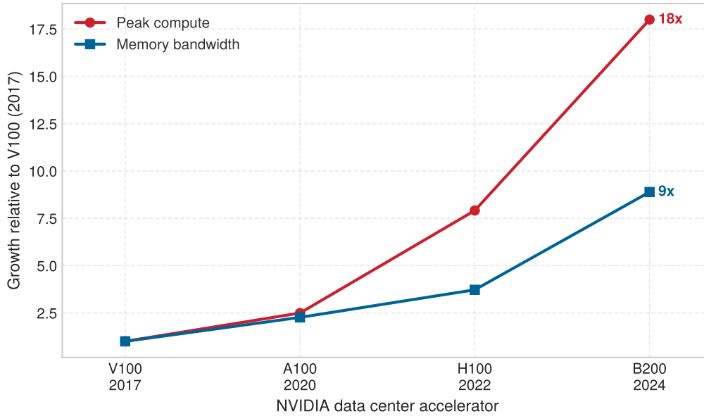
Figure 10.5: Decode inherits the bandwidth deficit: Peak compute and memory bandwidth for four accelerator generations, normalized to the V100. Compute rises 18× against bandwidth’s 8.9×, and because decode reads the full weight set once per token it advances at the lower of the two rates. Specifications come from the MLSysIM hardware registry.
