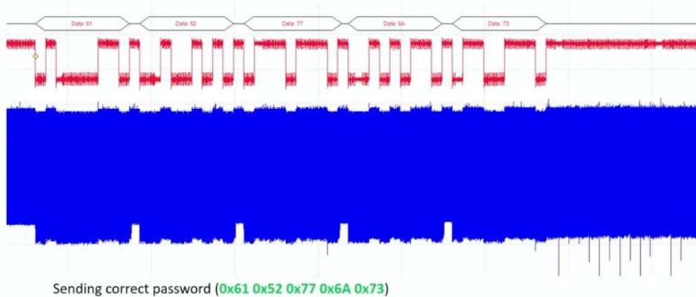
Figure 13.13: Power profile: The device's power consumption remains stable during authentication when the correct password is entered, setting a baseline for comparison in subsequent figures. Source: Colin O'Flynn.
