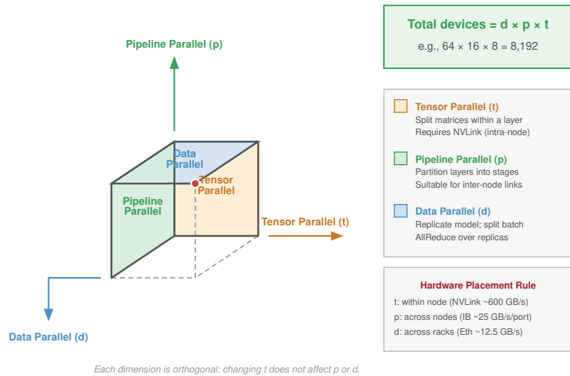
Figure 5.2: The 3D parallelism cube: The cube visualizes three distinct partitioning axes: data parallelism (replicating the model), pipeline parallelism (splitting depth), and tensor parallelism (splitting layers). Large-model training occupies a feasible point (d, p, t) only when divisibility, memory, batch, topology, and failure-domain constraints are satisfied together.
