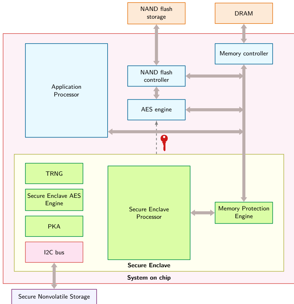
Figure 13.22: Secure enclave architecture: Hardware-isolated enclaves enhance system security by encapsulating sensitive data and cryptographic operations within a dedicated processor and memory. This design minimizes the attack surface and protects important keys even if the main application processor is compromised, providing a trusted execution environment for security-important tasks. Source: Apple.
