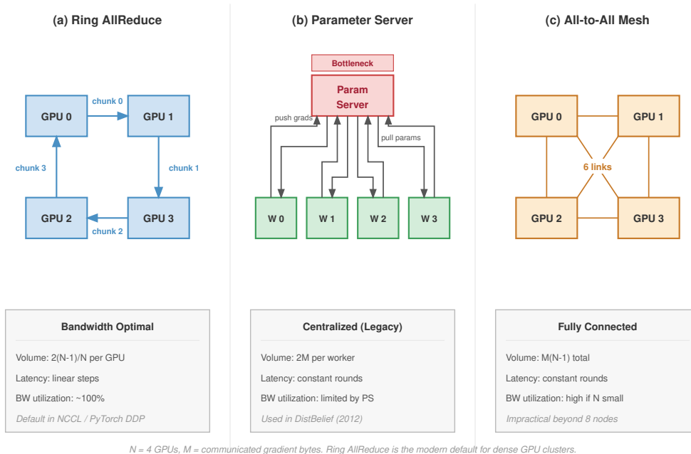
Figure 5.5: Gradient synchronization topologies: The panels compare three communication patterns. (a) Ring AllReduce distributes bandwidth evenly across links but has linear latency scaling. (b) A parameter server centralizes traffic and creates a server bottleneck. (c) An All-to-All mesh completes an exchange in one communication round, but its link count grows quadratically, making the topology impractical beyond small groups.
