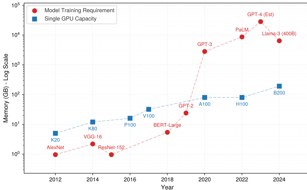
Figure 5.1: The memory wall: Accelerator memory capacity plotted against the memory a state-of-the-art model needs to train. Capacity climbs steadily while demand climbs faster, and the widening gap is why weights, gradients, and optimizer state must be split across devices rather than merely compressed.
