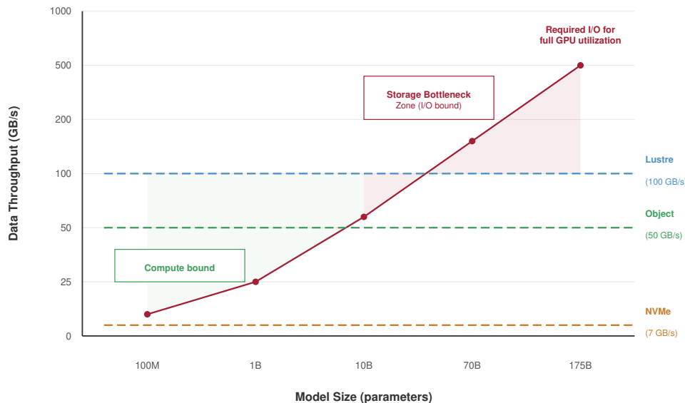
Figure 4.3: The storage bottleneck zone: Required I/O throughput for full GPU utilization rises with model size from 100 million to 175 billion parameters. The red curve shows storage demand; horizontal dashed lines mark common storage-tier ceilings (NVMe at 7 GB/s, object storage at 50 GB/s, and Lustre at 100 GB/s). Between the compute-bound and storage-bottleneck regions lies the transition where storage, not compute, limits training throughput.
