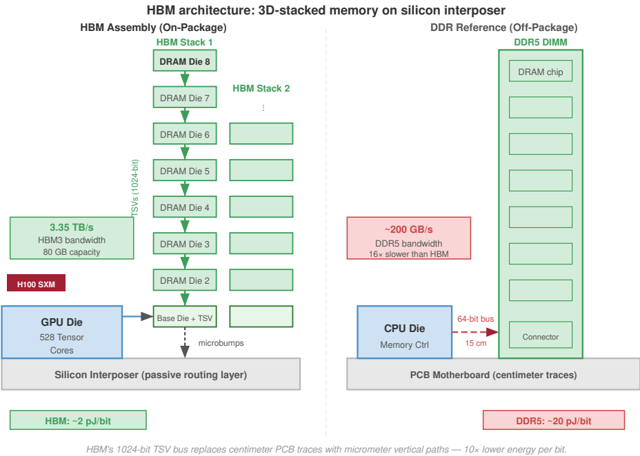
Figure 2.8: HBM 3D-stacked architecture: High-bandwidth memory achieves its performance by vertically stacking DRAM dies and connecting them via through-silicon vias. The entire stack sits on a silicon interposer alongside the GPU die, enabling a 1024-bit-wide bus and reducing signal travel distance from centimeters to micrometers. This physical proximity is the key to breaking the memory wall.
