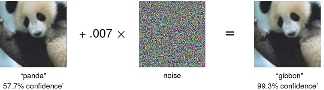
Figure 14.14: GoogLeNet Imperceptible Misclassification: Subtle, intentionally crafted noise added to an image causes a trained deep neural network (GoogLeNet) to misclassify a panda as a gibbon, despite the perturbed image remaining visually indistinguishable to humans. This classic demonstration underscores neural network fragility and motivates adversarial training. Source: (Goodfellow et al. 2015).
