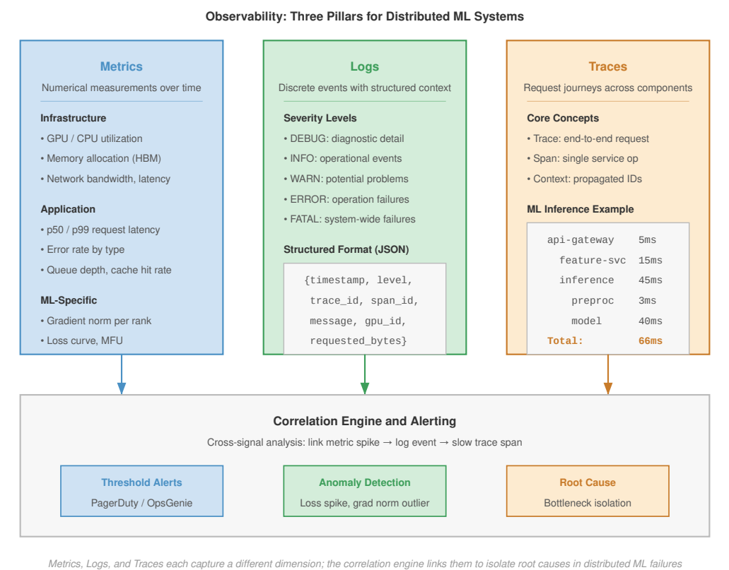
Figure 7.30: The three pillars of observability: Diagnosis of fleet failures requires correlating three signal types. Metrics reveal when and where a problem occurs (for example, GPU utilization drops). Logs provide the what through event context (for example, an out-of-memory exception). Traces provide the why by linking events across the distributed lifecycle (for example, identifying the request that triggered the memory spike).
