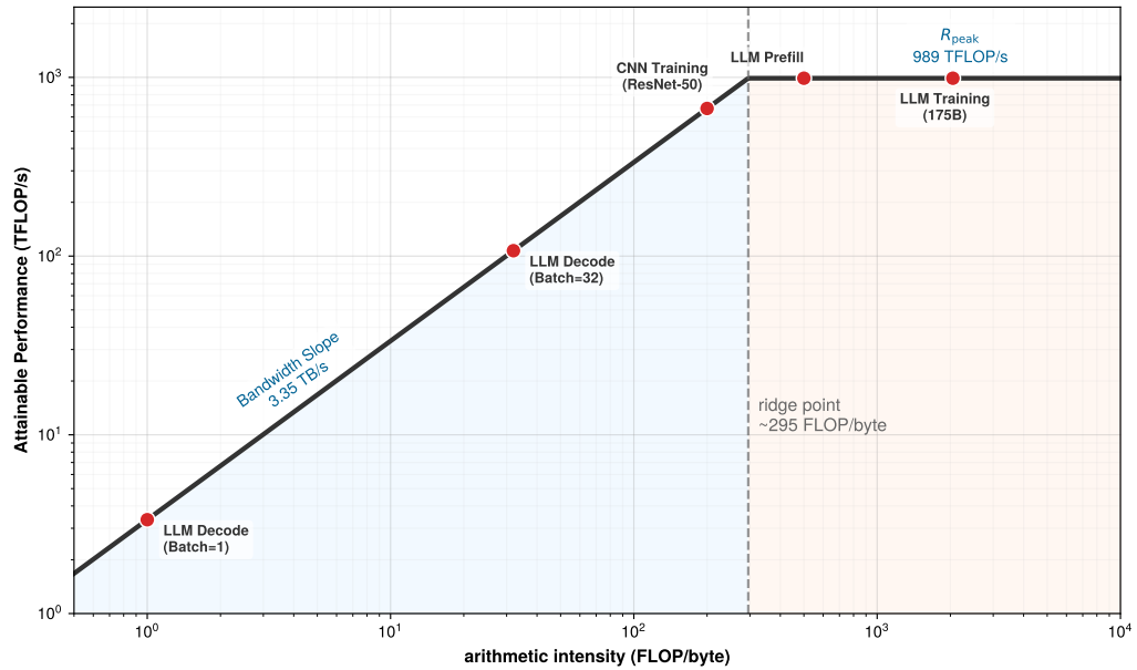
Figure 2.10: The H100 roofline landscape: The FP16 roofline for an NVIDIA H100 marks the memory-bandwidth and peak-compute ceilings, with representative ML workloads spanning memory-bound and compute-bound regions.
