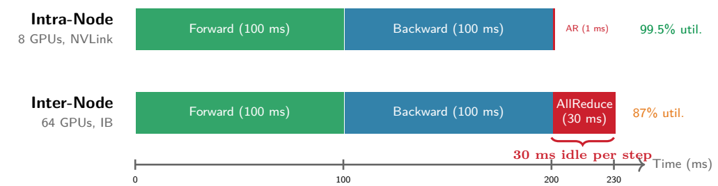
Figure 3.4: The bandwidth cliff in a training step: Illustrative normalized timelines for the same compute phases: an 8-GPU intra-node job (top) using NVLink at 900 GB/s, and a 64-GPU inter-node job (bottom) using InfiniBand at 50 GB/s. The AllReduce phase (red) grows from a thin sliver to a dominant fraction of the step. Without communication-computation overlap, GPUs sit idle during the entire AllReduce, and the utilization gap between the two scenarios is 12.5 percentage points (99.5 percent vs. 87 percent).
