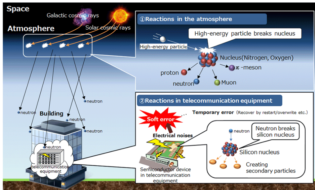
Figure 7.15: Transient fault mechanism: Cosmic rays and electromagnetic interference induce bit flips within hardware by altering electrical charges in memory cells and transistors. Source: NTT.
