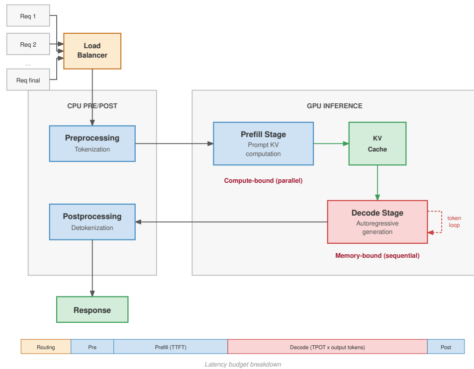
Figure 10.8: End-to-end inference pipeline: A detailed view of the request lifecycle: client requests arrive at a load balancer, then undergo preprocessing (tokenization) on the CPU. The data moves to the GPU for the compute-bound prefill stage and the memory-bound decode stage, which uses the KV cache. Finally, the response is postprocessed on the CPU (detokenization) and sent back. This visualization highlights the critical “Serving Tax” components (serialization, routing, coordination) that consume latency budget outside of the actual GPU compute time.
