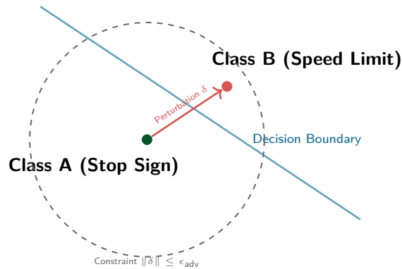
Figure 13.8: Adversarial decision boundary: High-dimensional neural networks often have nonlinear decision boundaries. An adversary seeks to find a minimal perturbation \delta that pushes a clean data point x across the boundary into another class region, while ensuring the perturbation is small enough ( \epsilon_{adv} ) to remain imperceptible or physically plausible.
