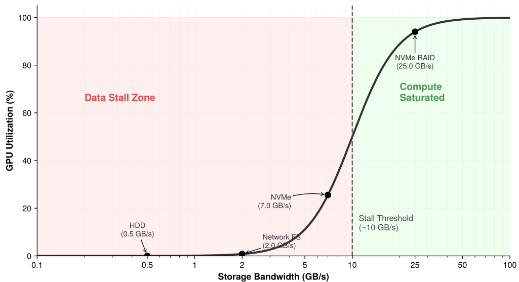
Figure 4.5: The data-stall frontier: GPU utilization follows a steep S-curve as storage bandwidth increases. Around the illustrative 10 GB/s threshold for an 8-GPU node, utilization crosses from waiting-dominated to compute-dominated. The positions of common storage technologies explain why tiered architectures are essential.
