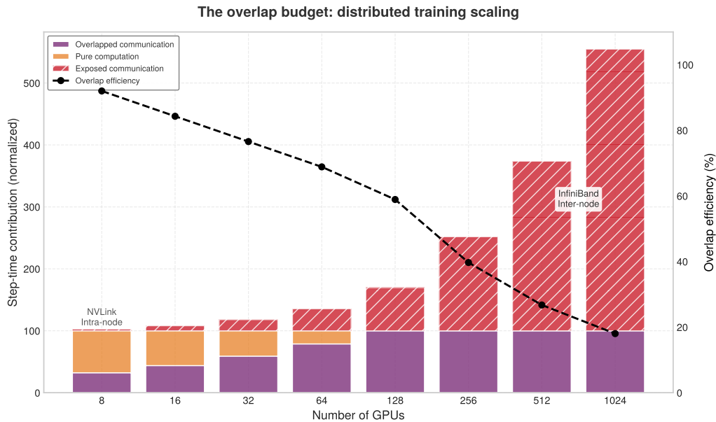
Figure 9.7: The overlap budget: This illustrative normalized scenario holds the computation budget at 100 units as GPU count increases from 8 to 1,024. Communication overhead grows with scale, leaving more communication exposed above the fixed compute budget. The black line reports the fraction of communication hidden behind computation, which falls from roughly 90 percent to roughly 18 percent.
