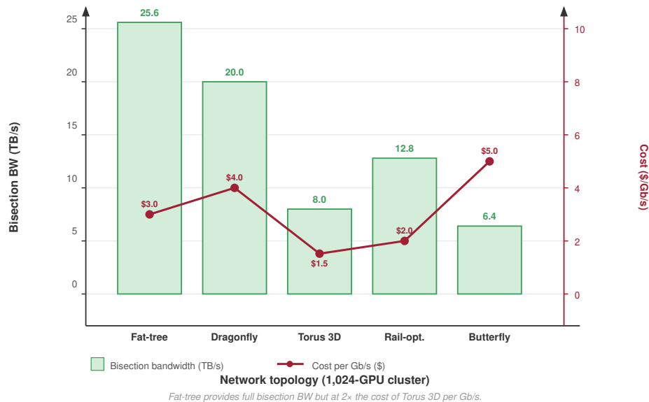
Figure 3.11: An illustrative bandwidth-cost scenario for ML network topologies: Assumed BW_{\text{bisection}} (TB/s, left axis) and cost per Gb/s (right axis) for five topology configurations on a 1,024-GPU cluster: Fat-tree (25.6 TB/s, $3.0/Gb/s), Dragonfly (20.0, $4.0), Torus 3D (8.0, $1.5), Rail-opt (12.8, $2.0), and Butterfly (6.4, $5.0). These scenario values illustrate the comparison method rather than universal properties of each topology family.
