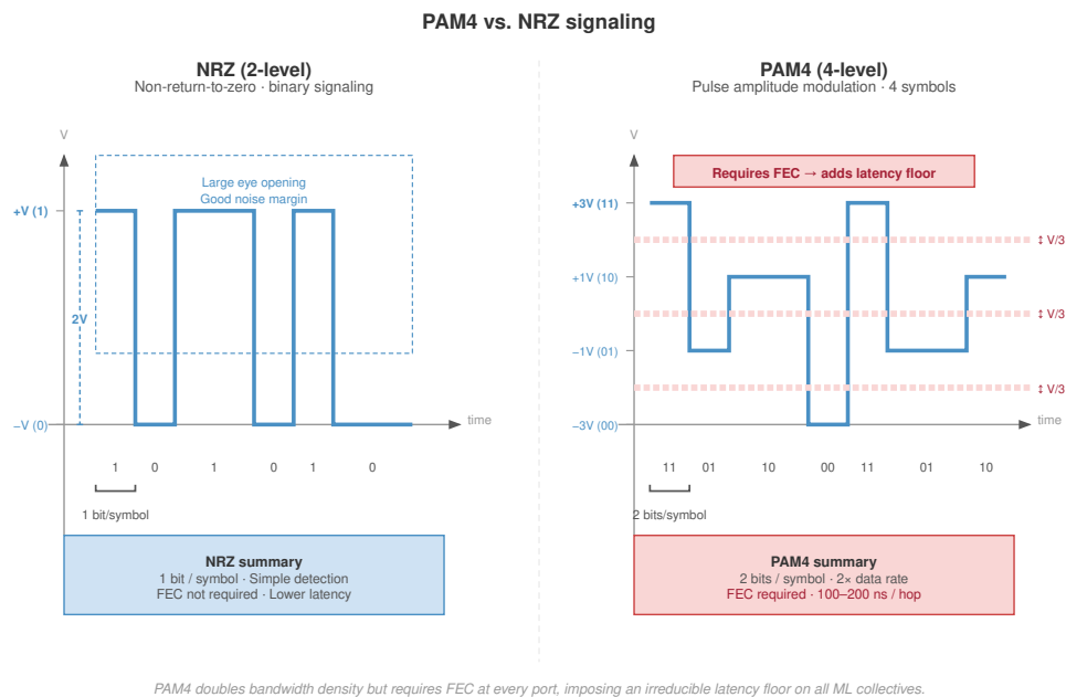
Figure 3.5: From NRZ to PAM4 signaling: To increase bandwidth without doubling clock frequency, high-speed interconnects moved from NRZ (2 voltage levels, 1 bit per symbol) to PAM4 (4 voltage levels, 2 bits per symbol). The trade-off is reduced noise margin: the ‘eye’ of the signal is smaller, necessitating forward error correction (FEC) and increasing the irreducible \alpha latency of the fabric.
