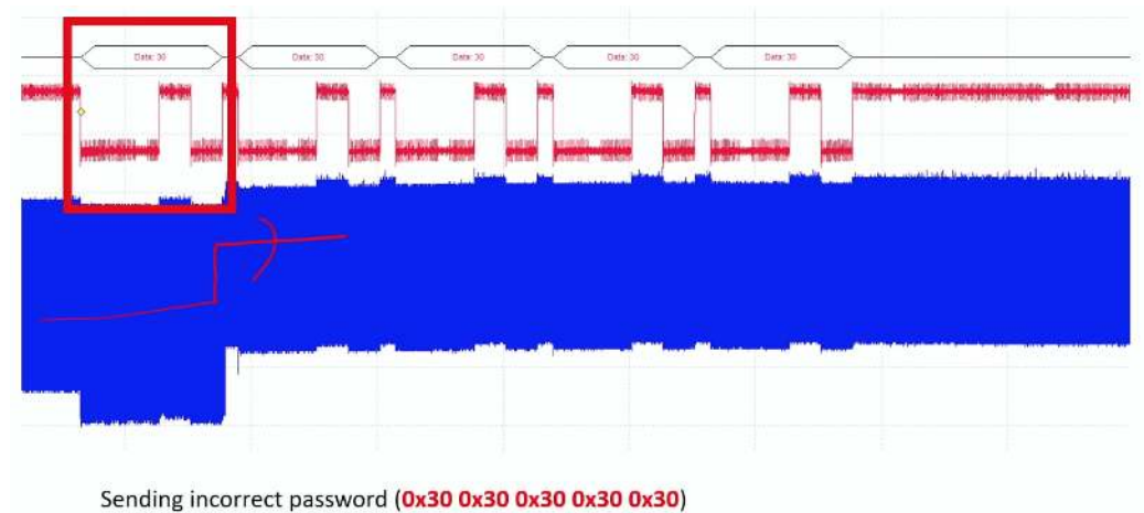
Figure 13.15: Power consumption jump: The blue line's sharp increase after processing the first byte indicates immediate authentication failure, highlighting how incorrect passwords are quickly detected through power usage. Source: Colin O'Flynn.
