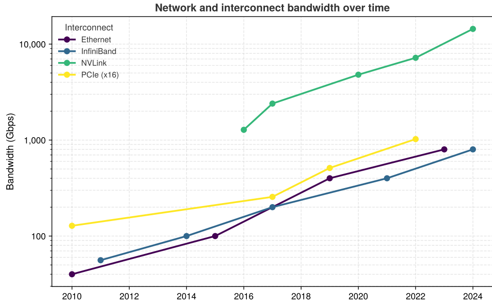
Figure 3.2: Historical network bandwidth scaling: Intra-node NVLink, inter-node InfiniBand and Ethernet, and the PCIe host bus, plotted on a common log scale from 2010 to 2024. NVLink pulls roughly an order of magnitude clear of the others, so the same collective costs far more when it crosses a machine boundary than when it stays inside one.
