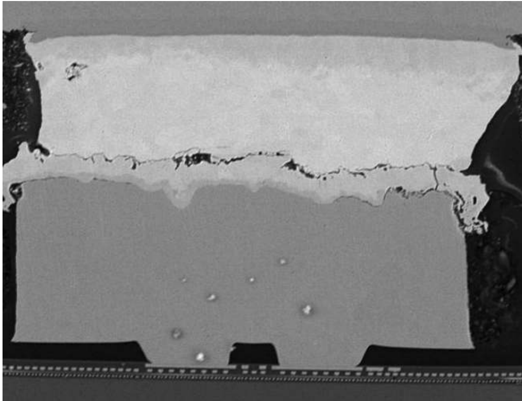
Figure 7.18: Intermittent fault mechanism: Physical degradation via micro-cracks between copper bumps and package solder joints creates variable electrical resistance. Source: constantinescu.
