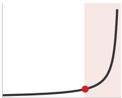
Past about 70 percent utilization, queue wait time explodes.
