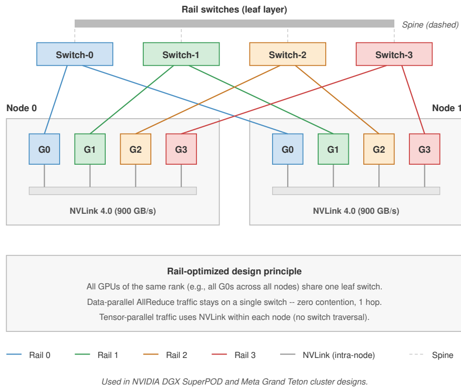
Figure 3.10: Rail-optimized physical wiring: In dense accelerator nodes (for example, DGX H100), GPUs are partitioned into rails corresponding to their PCIe slot position. GPU 0 in every node connects to Switch Rail 0, GPU 1 to Switch Rail 1, and so on. This architecture isolates same-rank data-parallel traffic on dedicated rails, reducing competition for BW_{\text{bisection}} and the hop count for latency-sensitive exchanges.
