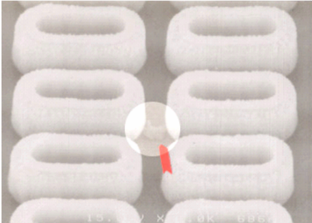
Figure 7.19: DRAM residue fault: Contamination and microscopic particle accumulation between DRAM cell contacts causing intermittent electrical connection failures. Source: Constantinescu.
