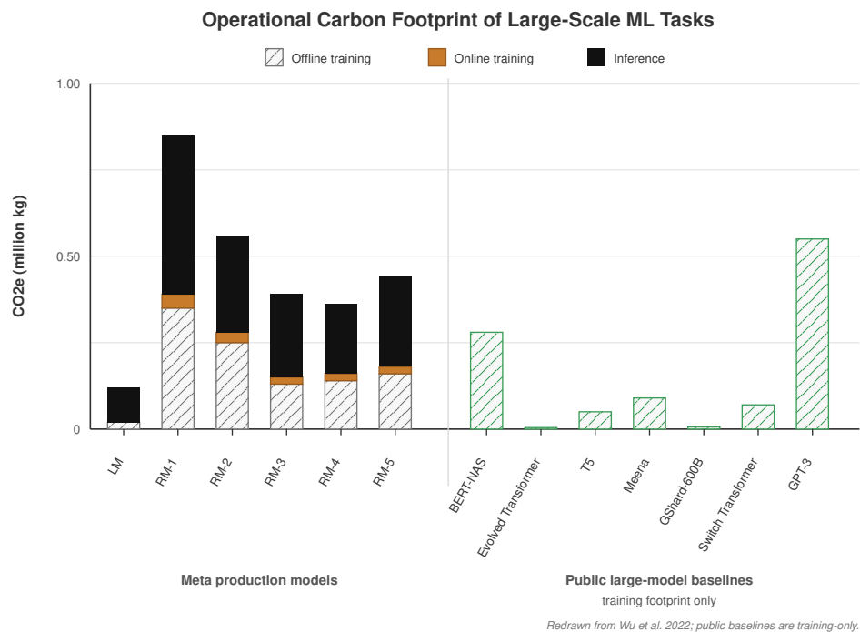
Figure 15.15: Operational Carbon Footprint of Large-Scale ML Tasks: Stacked bars show lifetime CO 2 e for Meta’s recommendation models (RM-1 through RM-5), a language model (LM), and several open-source large models (BERT-NAS, Evolved Transformer, T5, Meena, GShard-600B, Switch Transformer, GPT-3). Recommendation models are dominated by inference (solid black), while the public open-source baselines report training-only footprints (hatched), underscoring that inference serving at scale can rival or exceed training emissions for deployed systems. Source: (Wu et al. 2022).
