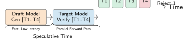
Figure 9.6: Speculative decoding process: Instead of generating tokens sequentially with the large target model, a small draft model proposes a sequence of K tokens. The target model verifies all K tokens in a single parallel forward pass. Drafted tokens that pass the acceptance test are emitted together; the first rejected token triggers a corrected sample and discards the remaining draft.
