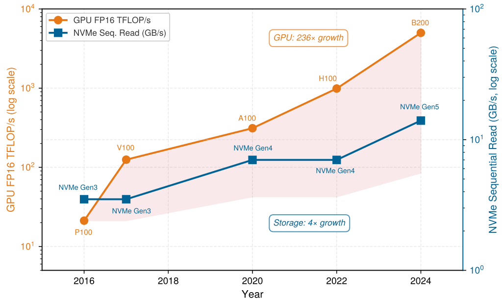
Figure 4.2: The storage-compute chasm: GPU peak FP16 throughput (orange, left axis) and NVMe sequential read bandwidth (blue, right axis) from 2016 to 2024 appear on logarithmic scales. GPU throughput has grown 236× while storage bandwidth has grown only 4× over the same period. The shaded region highlights the widening gap that data-pipeline engineering must bridge through prefetching, caching, and format optimization.
