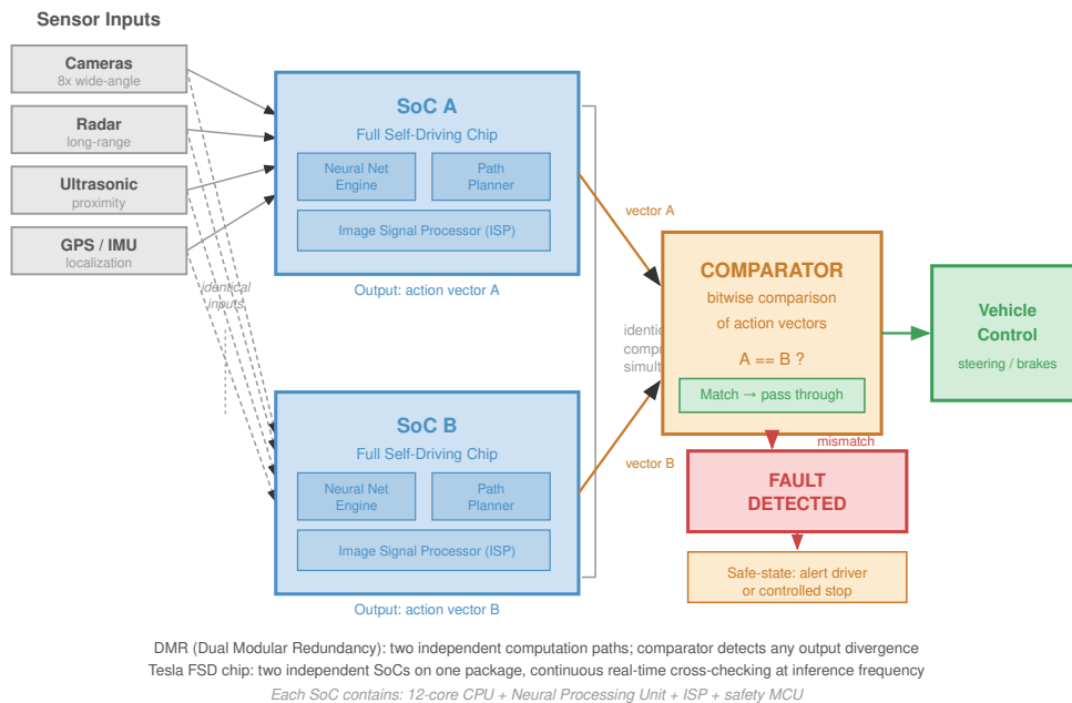
Figure 7.21: Dual modular redundancy (DMR): Tesla's full self-driving computer employs a DMR architecture, replicating critical computations across two independent system-on-chips (SoCs). A hardware comparator unit validates that both chips produce matching outputs before allowing a control command to reach the vehicle's actuators, ensuring that a single-chip hardware failure or bit flip cannot trigger dangerous driving behavior.
