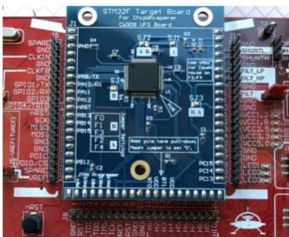
Figure 13.18: STM32F target board: The measurement setup exposes power consumption during AES operations on the microcontroller. Those traces provide the observations from which a side-channel model can infer data-dependent internal behavior.
