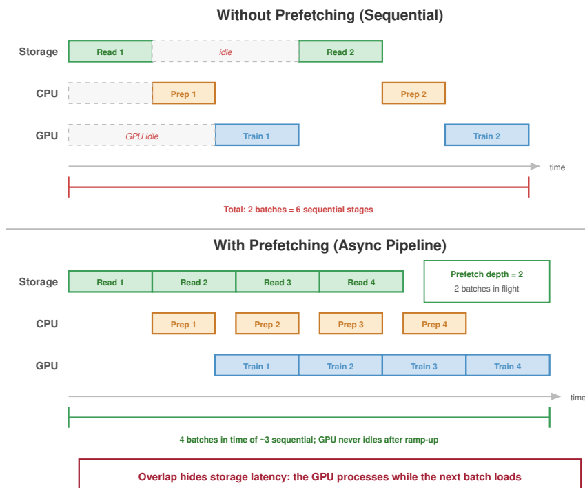
Figure 4.6: Pipelined data loading: The CPU prepares batch i + 1 while the GPU processes batch i . Pipelining hides storage latency, but only if the prefetch buffer is deep enough to absorb variance.
