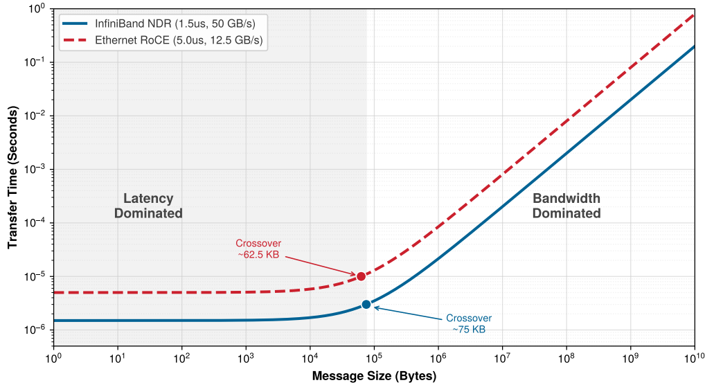
Figure 3.8: The \alpha - \beta crossover: Modeled transfer time as a function of message size for an NDR InfiniBand path and a 100 Gb/s RoCE baseline using the scenario parameters in the text. Small messages are latency dominated (flat region), while large messages are bandwidth dominated (linear region). Measured crossover points vary with the end-to-end path.
