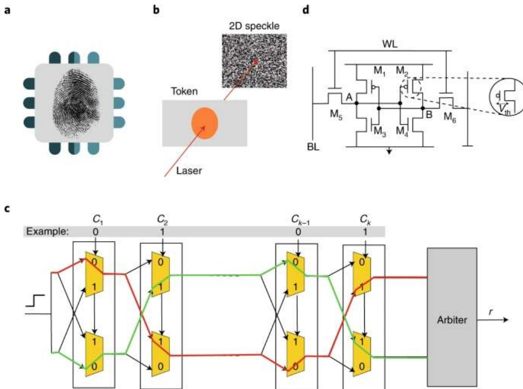
Figure 13.24: Physical unclonable functions: PUFs generate unique hardware fingerprints from inherent manufacturing variations. The figure shows several types: a chip-level fingerprint concept, optical PUFs that use laser speckle patterns, electronic arbiter PUFs that rely on timing differences in response to a challenge, and SRAM PUFs that exploit manufacturing variations in memory cells.
