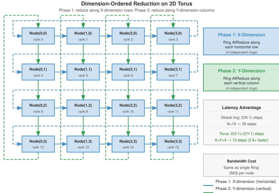
Figure 6.10: Dimension-ordered reduction on a torus topology: In a 2D torus mesh (a simplified representation of 3D TPU pods), AllReduce proceeds in sequential steps along the X and Y dimensions. Reducing along one dimension at a time follows direct-neighbor links and can reduce contention relative to a topology-unaware schedule.
