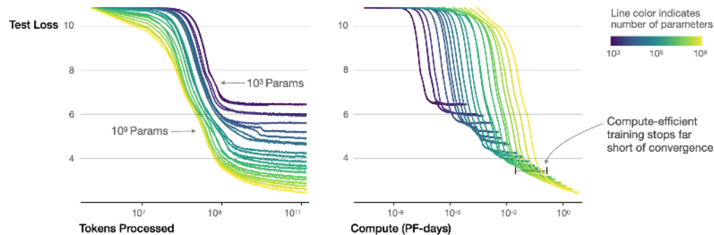
Figure 1.8: Scaling laws and compute optimality: Larger models consistently achieve better performance with increased training data and compute, but diminishing returns necessitate careful resource allocation during training. Optimal model size and training duration depend on the available compute budget, as evidenced by the convergence of loss curves at different parameter scales and training token counts.
