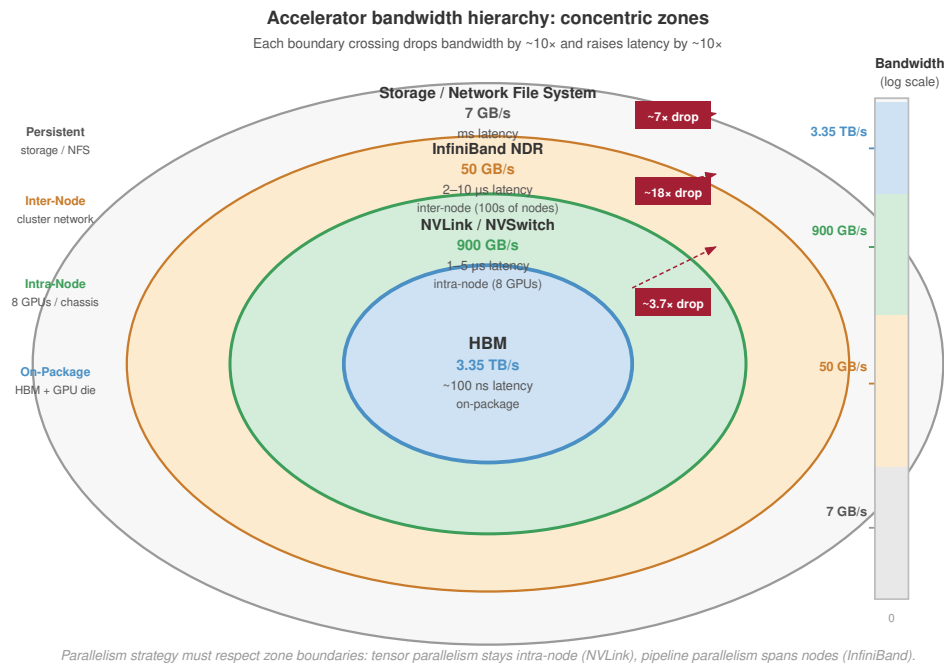
Figure 2.13: The infrastructure bandwidth hierarchy: Concentric zones visualize the bandwidth tiers an ML workload crosses. HBM (3.35 TB/s) sits at the innermost zone; each outward boundary crossing drops bandwidth ~10× and raises latency ~10×: NVLink/NVSwitch (900 GB/s), InfiniBand NDR (50 GB/s), and storage/network file system (7 GB/s) at the outermost zone. Exploiting this hierarchy through tiered algorithms is the primary task of distributed systems engineering.
