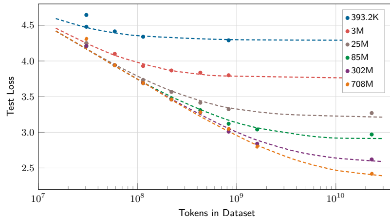
Figure 1.9: Loss vs. dataset size across model scales: Test loss curves show how models of different sizes (393K to 708M parameters) benefit from increased training data. Larger models achieve lower loss, but all curves exhibit diminishing returns at high token counts.
