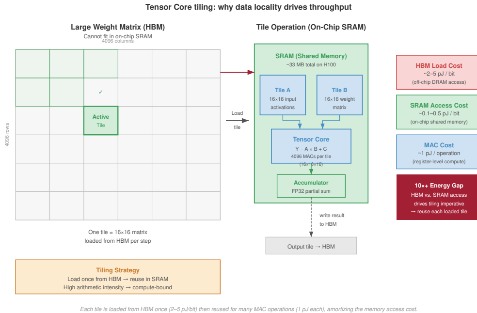
Figure 2.7: Tensor Core tiling strategy: To overcome the HBM bandwidth bottleneck, GPUs decompose large matrix operations into small tiles that fit within the streaming multiprocessor's (SM) fast SRAM. Data is loaded once into SRAM and reused across multiple Tensor Core operations, effectively multiplying the arithmetic value of every byte fetched from HBM.
