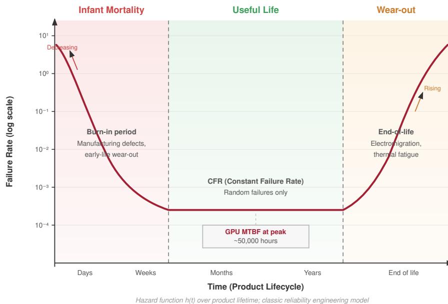
Figure 7.12: The bathtub curve: Hardware failure rates \lambda(t) vary over time. (1) Infant mortality: high failure rate initially due to manufacturing defects. (2) Useful life: constant, low failure rate where random failures dominate. (3) Wear-out: increasing failure rate as components age. Burn-in testing aims to filter out infant mortality failures before deployment.
