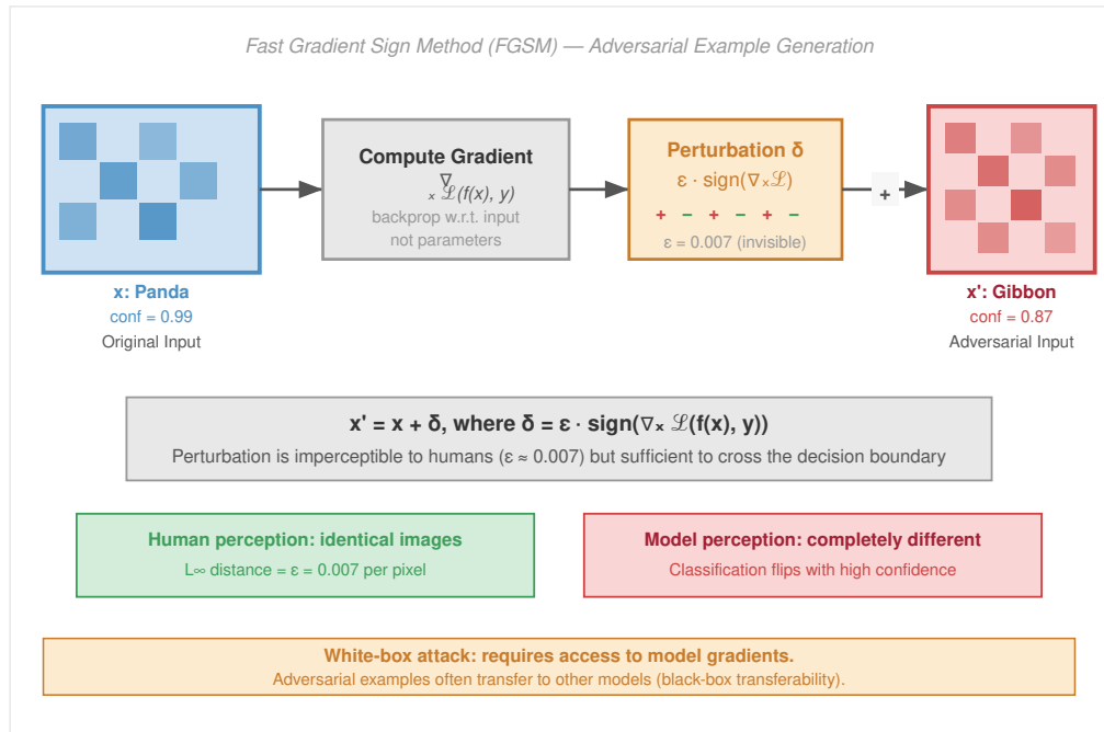
Figure 14.13: Gradient-Based Attack Mechanism: Fast Gradient Sign Method (FGSM) and related gradient-based attacks generate subtle input noise with magnitude controlled by \epsilon that maximizes the loss function \mathcal{L}(\theta, x, y) and forces misclassification. The perturbation moves the input x across the learned decision boundary. Source: adapted from a gradient-based-attacks tutorial at defence.AI.
