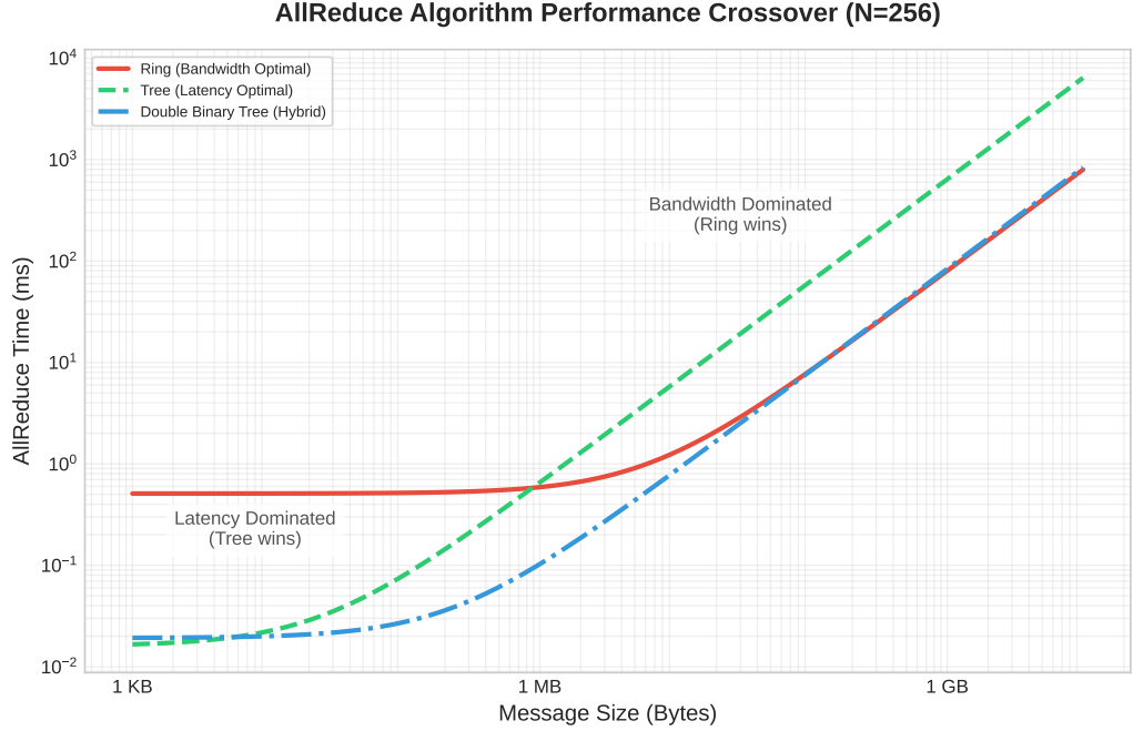
Figure 6.7: Algorithm crossover in collective communication: Performance analysis of Ring, Tree, and Double Binary Tree AllReduce algorithms across message sizes (1 KB to 10 GB) for a 256-GPU cluster with 200 Gbps interconnect.
