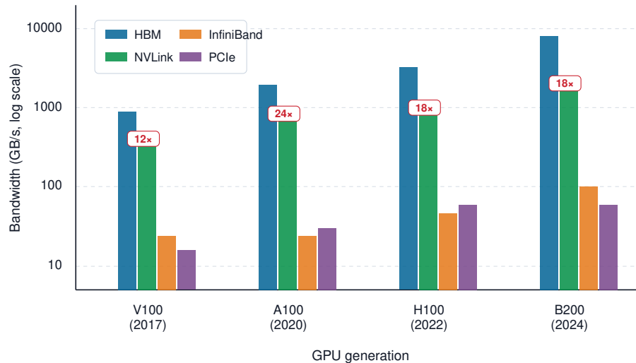
Figure 3.3: The bandwidth hierarchy: Bandwidth at four levels of the communication hierarchy across four GPU generations, on a logarithmic scale. While HBM and NVLink bandwidth have grown roughly 9\times and 6\times respectively from V100 to B200, InfiniBand has grown only 4\times . The annotations show the ratio of NVLink bidirectional-total bandwidth to one InfiniBand port, quantifying the cliff that distributed training must cross at every synchronization point; on a like-with-like per-direction basis the H100-to-NDR cliff is about half that, roughly 9\times (see text).
