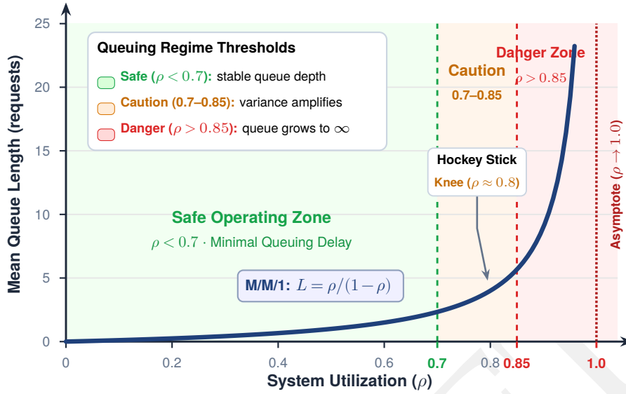
Figure F.1: The queuing hockey stick: For an M/M/1 queue, \rho_{\text{serv}} / (1 - \rho_{\text{serv}}) is the expected number of requests in the system, including the request in service. Its hyperbolic rise near saturation explains why production systems retain utilization headroom; the shaded operating bands are illustrative rather than universal thresholds.
