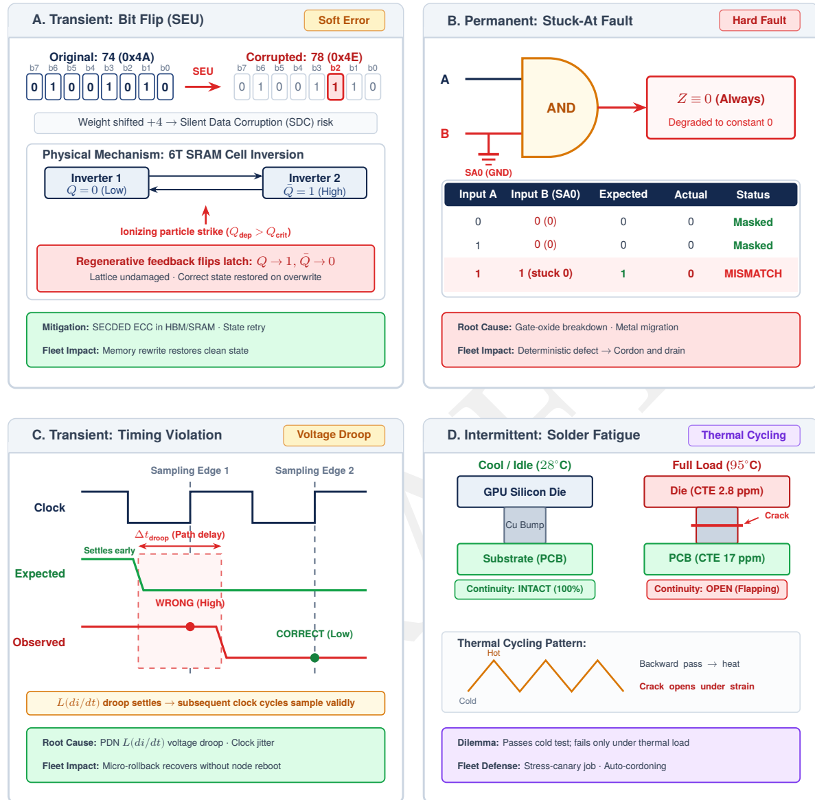
Figure 7.13: Temporal taxonomy of hardware faults: Four panels show how the three temporal categories manifest in practice. Transient panels (bit flip and timing glitch) show temporary disruptions that do not cause permanent damage. The intermittent panel shows sporadic errors driven by unstable conditions or aging. The permanent panel (stuck-at-0/1) shows irreversible physical damage that requires replacement.
