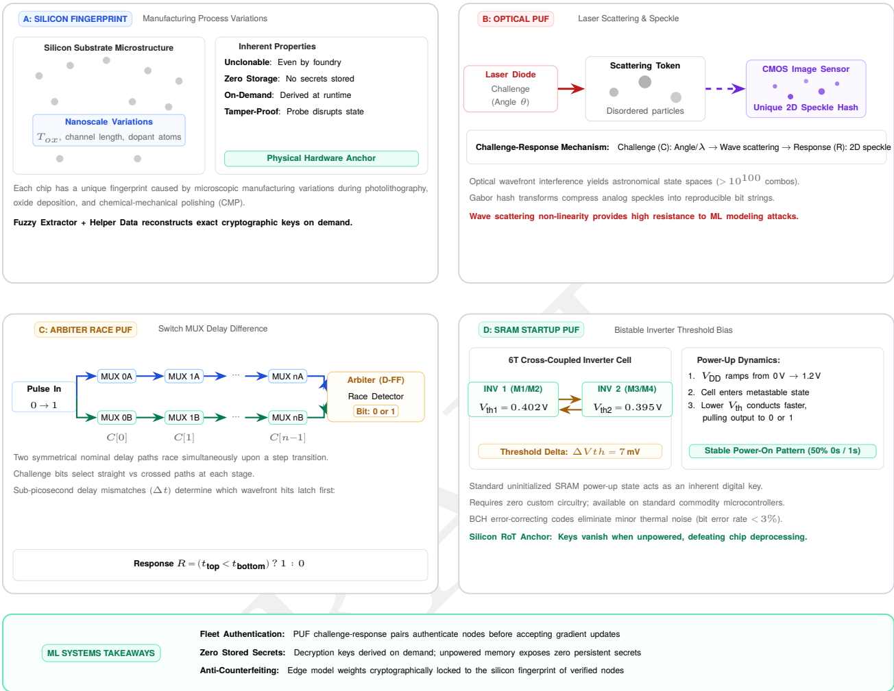
Figure 13.24: Physical unclonable functions: PUFs generate unique hardware fingerprints from inherent manufacturing variations. The figure shows several types: a chip-level fingerprint concept, optical PUFs that use laser speckle patterns, electronic arbiter PUFs that rely on timing differences in response to a challenge, and SRAM PUFs that exploit manufacturing variations in memory cells.
