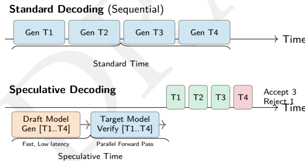
Figure 9.11: Speculative decoding process: Instead of generating tokens sequentially with the large target model, a small draft model proposes a sequence of K tokens. The target model verifies all K tokens in a single parallel forward pass. Drafted tokens that pass the acceptance test are emitted together; the first rejected token triggers a corrected sample and discards the remaining draft.
