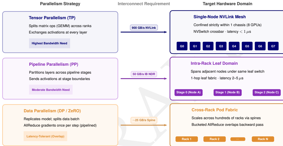
Figure 8.8: Hierarchical placement for 3D parallelism: Optimal placement maps distributed training dimensions to matching physical interconnect layers. Tensor parallelism (TP) maps strictly inside nodes across NVLink (900 GB/s); pipeline parallelism (PP) maps across adjacent nodes within a rack (50 GB/s); and data parallelism (DP) spans across racks via rail-aligned spine fabrics.
