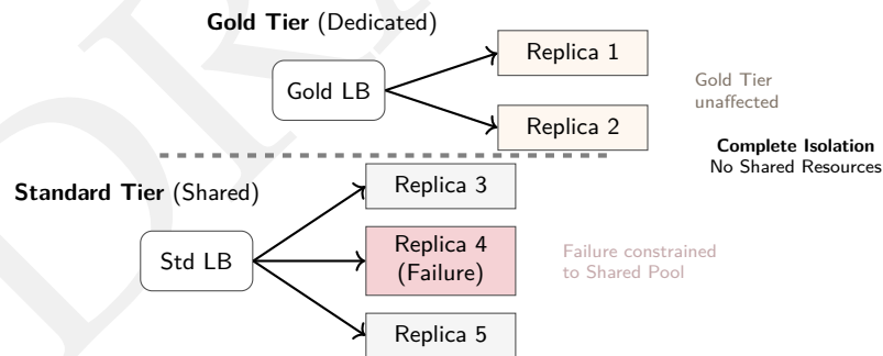
Figure 10.21: Bulkhead isolation patterns: To prevent cascading failures in multi-tenant systems, bulkheads isolate resources. Deployment-level bulkheads (shown) assign dedicated physical replicas to high-priority tenants, ensuring complete isolation. Request-level bulkheads enforce strict concurrency limits within shared processes. Like ship compartments, these boundaries ensure that a failure or resource exhaustion in one segment cannot sink the entire platform.
