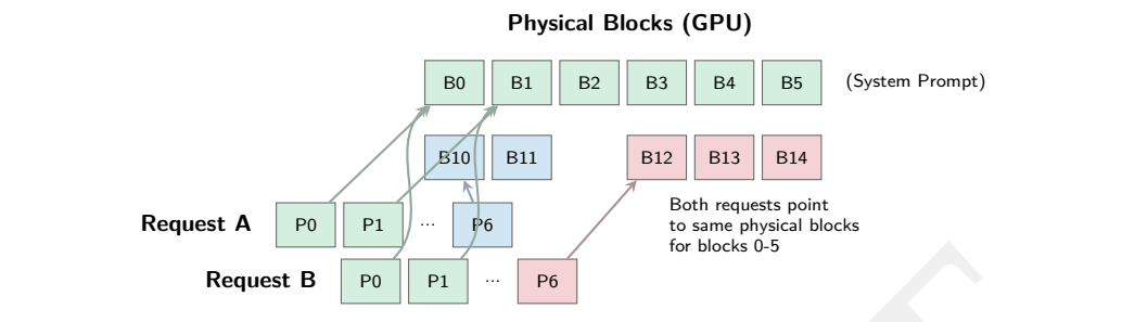
Figure 10.12: Prefix caching via block sharing: PagedAttention enables efficient prefix caching by allowing multiple sequences’ block tables to point to the same physical blocks for shared content. In this example, the System Prompt is stored in blocks 0-5. Request A and Request B map their first 6 logical pages to these same physical blocks, storing only their unique suffixes in new blocks. This dramatically reduces memory usage and prefill computation for workloads with shared context.
