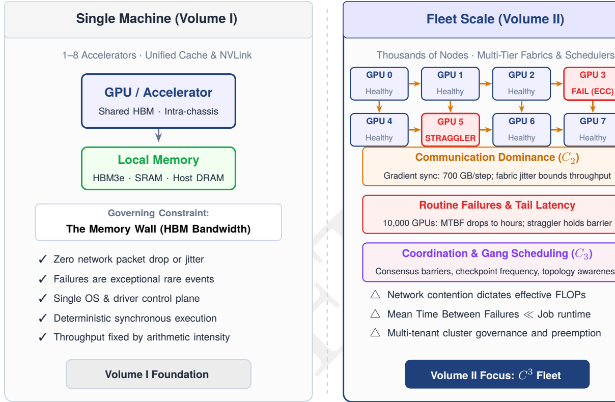
Figure 1.3: The scale discontinuity: Single-machine workloads (left) often bind on local memory bandwidth and require no inter-node coordination. Fleet-scale workloads (right) can bind on communication, encounter routine component failures during long runs, and require governance across a larger operational boundary.
