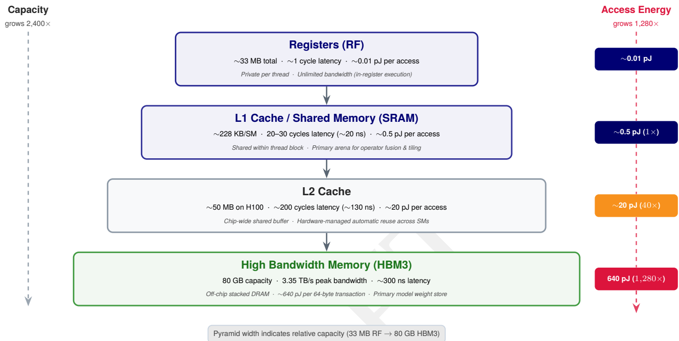
Figure 9.2: GPU memory hierarchy and data movement: Visual hierarchy from fast on-chip registers and SRAM down through L2 cache to off-chip HBM3. Latency scales from 1 clock cycle (~0.01 pJ) to hundreds of nanoseconds (~640 pJ per transaction), illustrating the extreme cost disparity between SRAM-resident computation and off-chip memory traffic.
