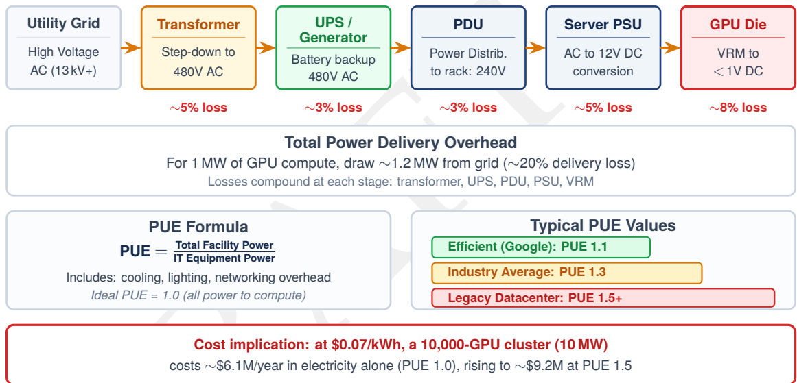
Figure 2.11: The power delivery path: The journey of energy from the high-voltage grid to the low-voltage transistor involves multiple conversion stages, each with its own efficiency loss. The cumulative delivery loss, combined with overhead for cooling (measured by PUE), dictates how much power a facility must draw from the grid. The critical engineering challenge is the rack power distribution unit (PDU) to voltage regulator module (VRM) transition, where 10–40 kW of power must be delivered within a single cabinet.
