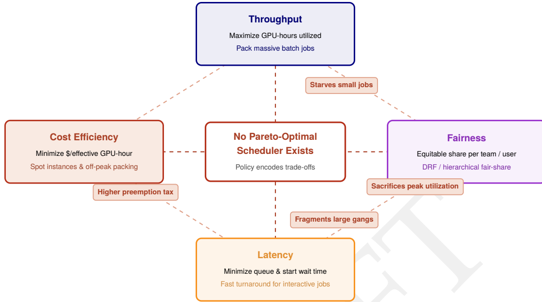
Figure 8.1: Scheduling trade-offs across competing fleet objectives: A four-way trade-off diamond (Throughput, Latency, Fairness, Cost Efficiency) illustrates the tensions governing cluster scheduling. Throughput favors long, unbroken runs; Latency favors aggressive preemption for interactive jobs; Fairness fragments resources to equalize shares; and Cost Efficiency leverages discounted, interruptible capacity.
