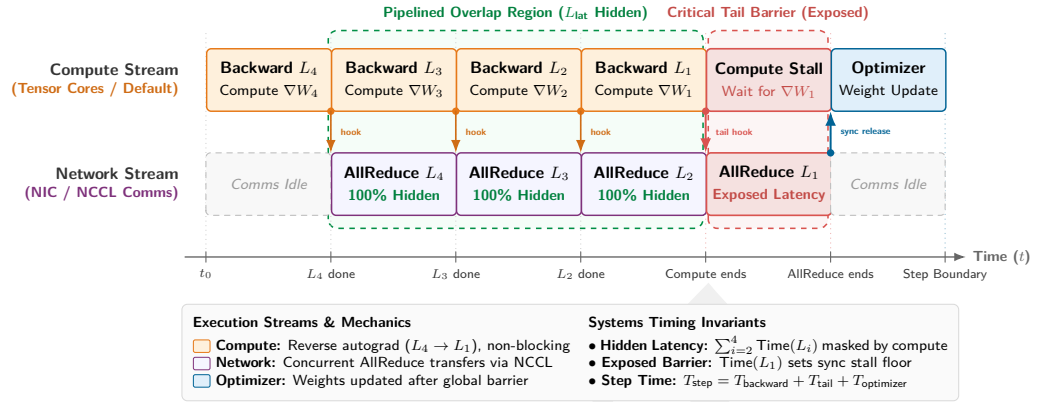
Figure 6.4: Communication-computation overlap: By pipelining collective operations with the backward pass, systems can hide network latency behind arithmetic execution. Overlap is successful only when the nonoverlappable overhead ( o ) is minimized, allowing the bulk transfer term to proceed while the GPU computes the next layer’s gradients.
