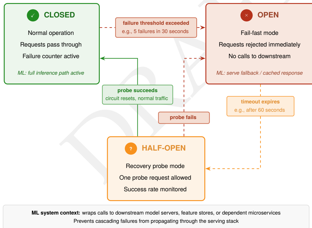
Figure 7.30: Circuit breaker states: The circuit breaker protects the system from cascading failure. Closed: normal operation. Open: error threshold exceeded; all requests fail fast to prevent resource exhaustion. Half-open: after a timeout, a limited number of requests are allowed through to probe the dependency's health. Success resets to closed; failure returns to open.
