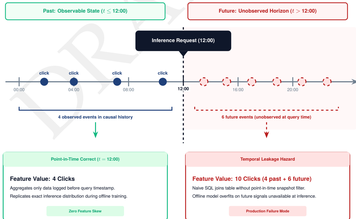
Figure 12.12: Point-in-time correctness: A point-in-time join prevents leakage by pairing each training event with feature values as they existed at the event timestamp , not with their current values. The resulting example contains only information that would have been available at inference time.
