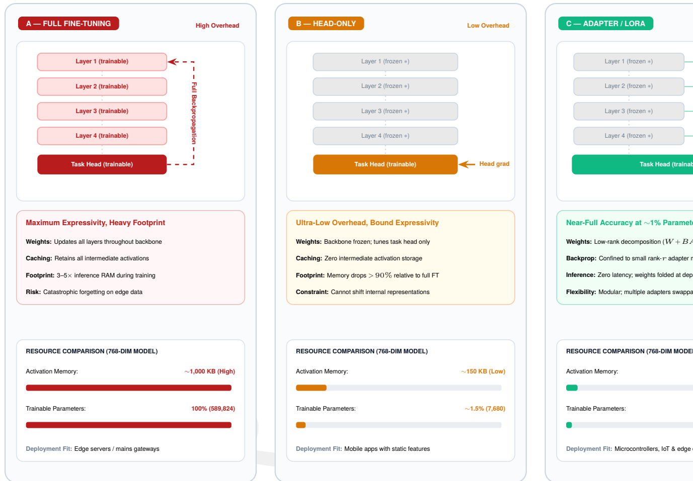
Figure 11.16: Federated personalization architectures: The panels compare strategies for adapting global models to local data. Full fine-tuning updates every parameter; head-only adaptation freezes the feature extractor; and adapter-based learning, such as LoRA, inserts small trainable modules into a frozen backbone. Each step trades additional local compute and state for greater adaptation capacity.
