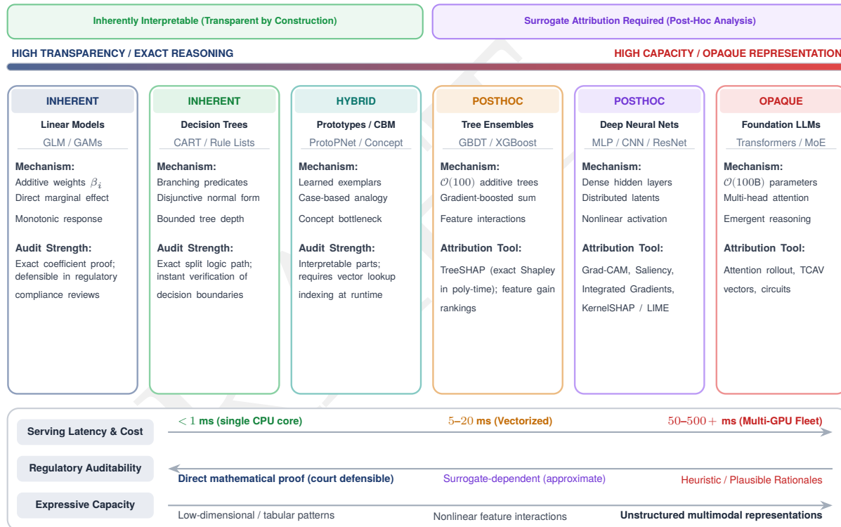
Figure 16.9: Model Interpretability Spectrum: Inherently interpretable models, such as linear regression and decision trees, offer transparent reasoning, while complex models like neural networks require posthoc explanation techniques to understand their predictions. This distinction guides model selection based on application needs, prioritizing transparency in regulated domains or when stakeholder trust is important.
