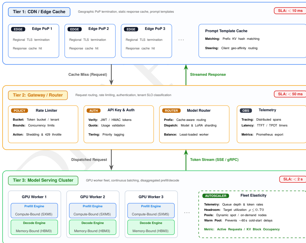
Figure 10.3: Serving deployment stack: A three-tier serving stack with cumulative latency budget from top to bottom. Tier 1 (CDN/Edge Cache) handles geographic distribution and cached static responses (SLA <10 ms). Tier 2 (Gateway/Router) handles request routing, rate limiting, and authentication (SLA <50 ms). Tier 3 (Model Serving Cluster) runs GPU workers with autoscaling and continuous batching (SLA <2 s).
