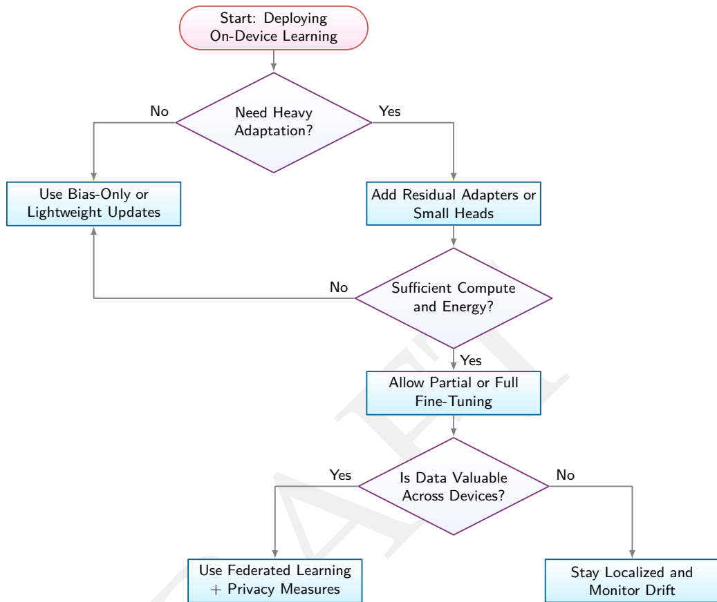
Figure 11.21: Tiered adaptation strategy: The flowchart integrates adaptation policy across device tiers and fleet-wide data-sharing requirements. Lightweight devices use bias-only updates, capable devices add residual adapters, and devices with sufficient compute allow full fine-tuning; data value across devices determines whether learning remains localized or becomes federated.
