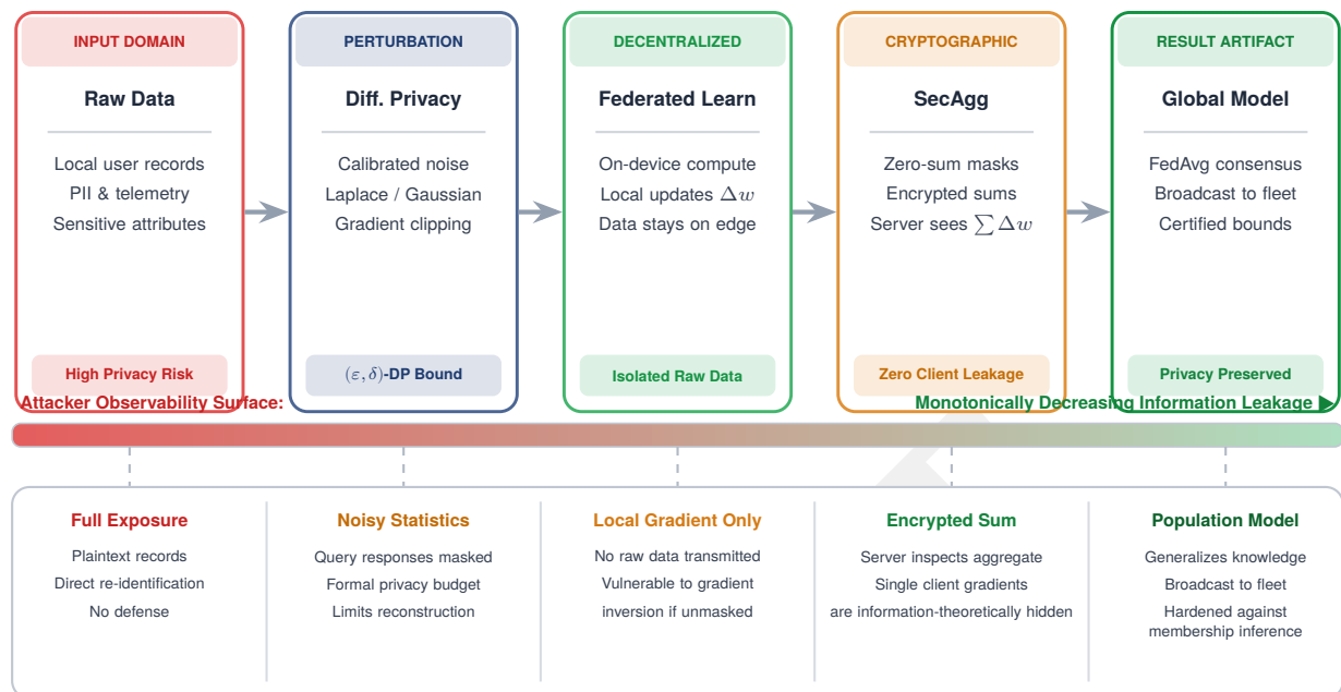
Figure 16.3: Privacy-Preserving Machine Learning Pipeline: A multi-stage architecture for training a global model while minimizing data exposure. The pipeline applies sequential safeguards—differential privacy, federated learning, and secure aggregation—that progressively reduce attacker visibility into raw personal data.
