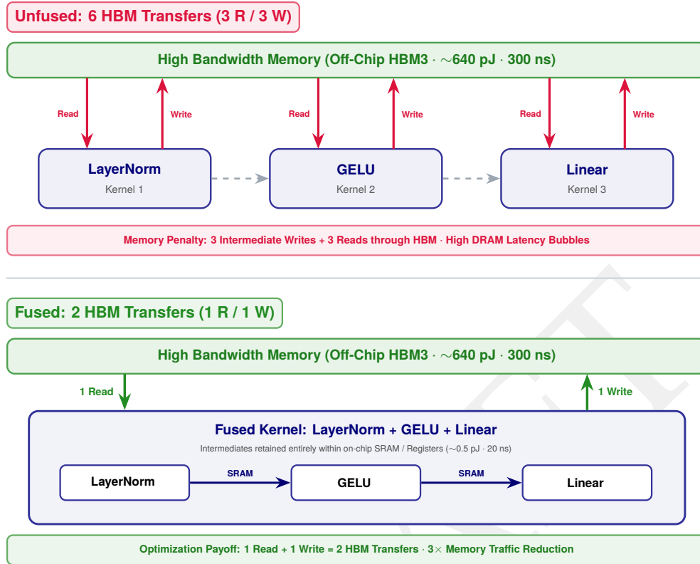
Figure 9.6: Operator fusion before and after. Top: three separate kernels each read from and write to HBM, materializing intermediates Z_1 and Z_2 , with six HBM round-trips along the unfused path. Bottom: a single fused kernel reads inputs once, holds intermediates retained entirely within on-chip SRAM / Registers ( \sim 0.5 pJ · 20 ns), and writes only the final output, leaving just two HBM round-trips. The fused path delivers roughly a 3× reduction in HBM traffic per layer.
