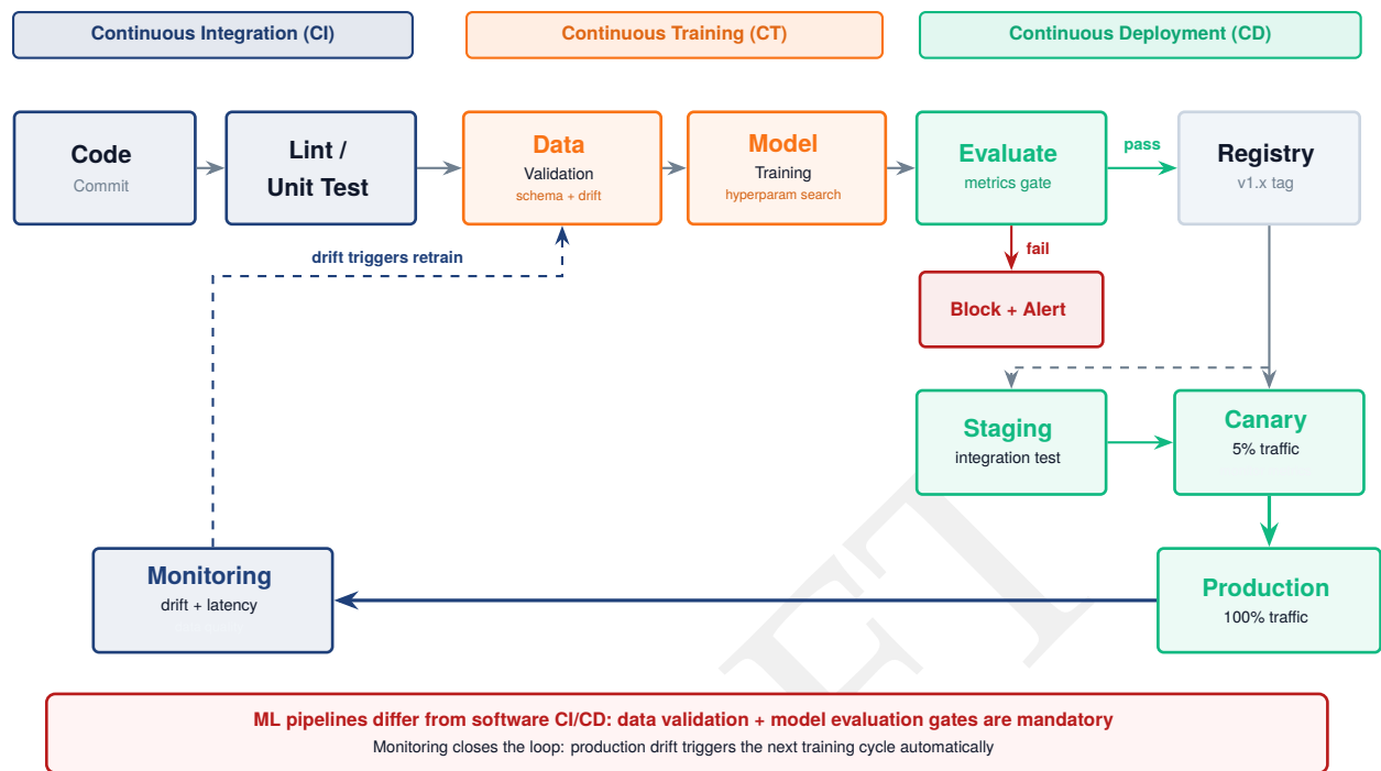
Figure 12.6: ML CI/CD pipeline: The automated workflow transforms code and data into a deployed service. Stages include Data Validation (schema/drift checks), Training, Evaluation (metric gates), Artifact Registration, and Staged Deployment (canary rollout). Feedback loops automatically trigger retrains or alerts if gates fail.
