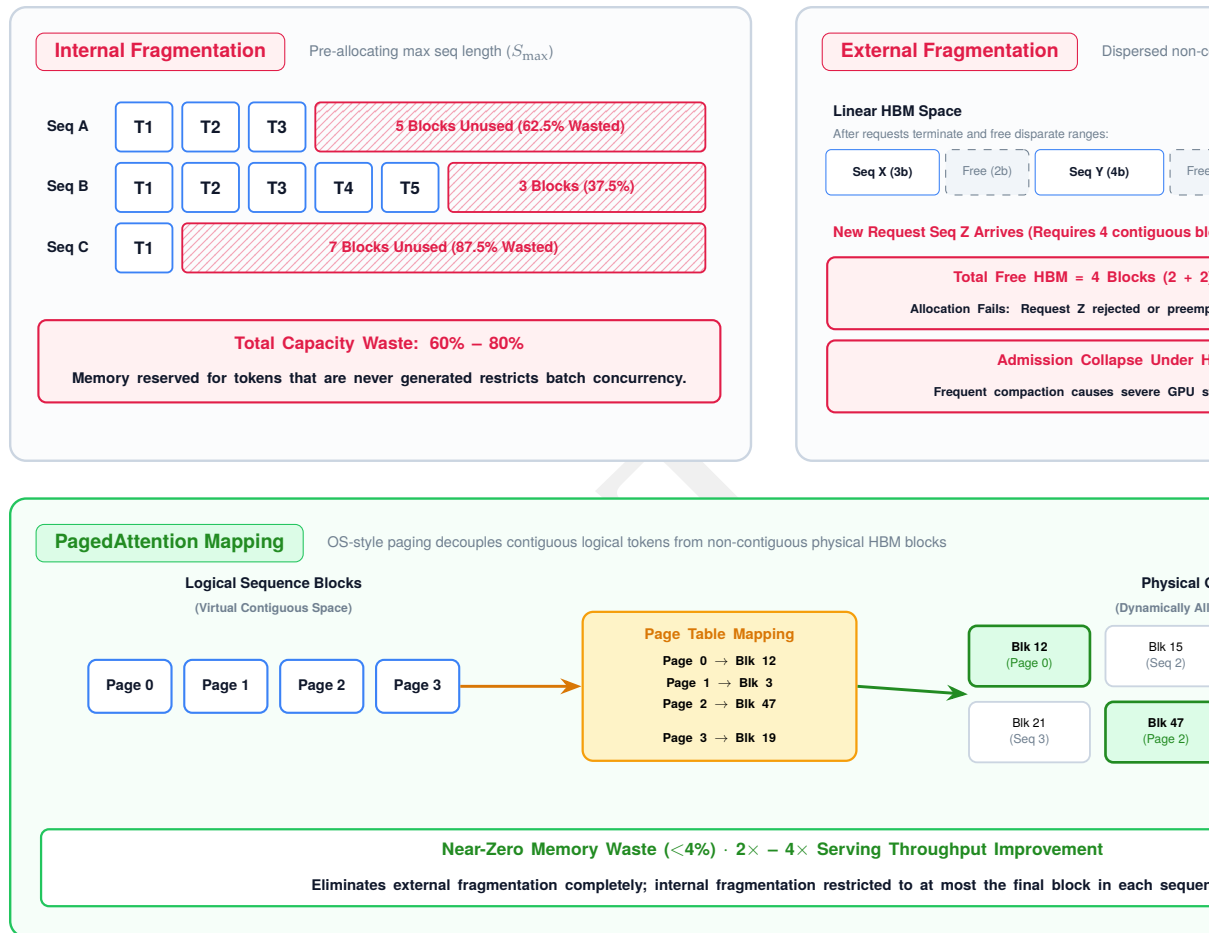
Figure 10.11: KV cache fragmentation and the PagedAttention solution: Top left: internal fragmentation wastes memory by preallocating for the maximum sequence length. Top right: external fragmentation leaves unusable memory gaps. Bottom: PagedAttention solves this by mapping contiguous logical pages of a sequence to noncontiguous physical memory blocks via a block table, allowing the system to fill fragmentation gaps with small blocks from any sequence.
