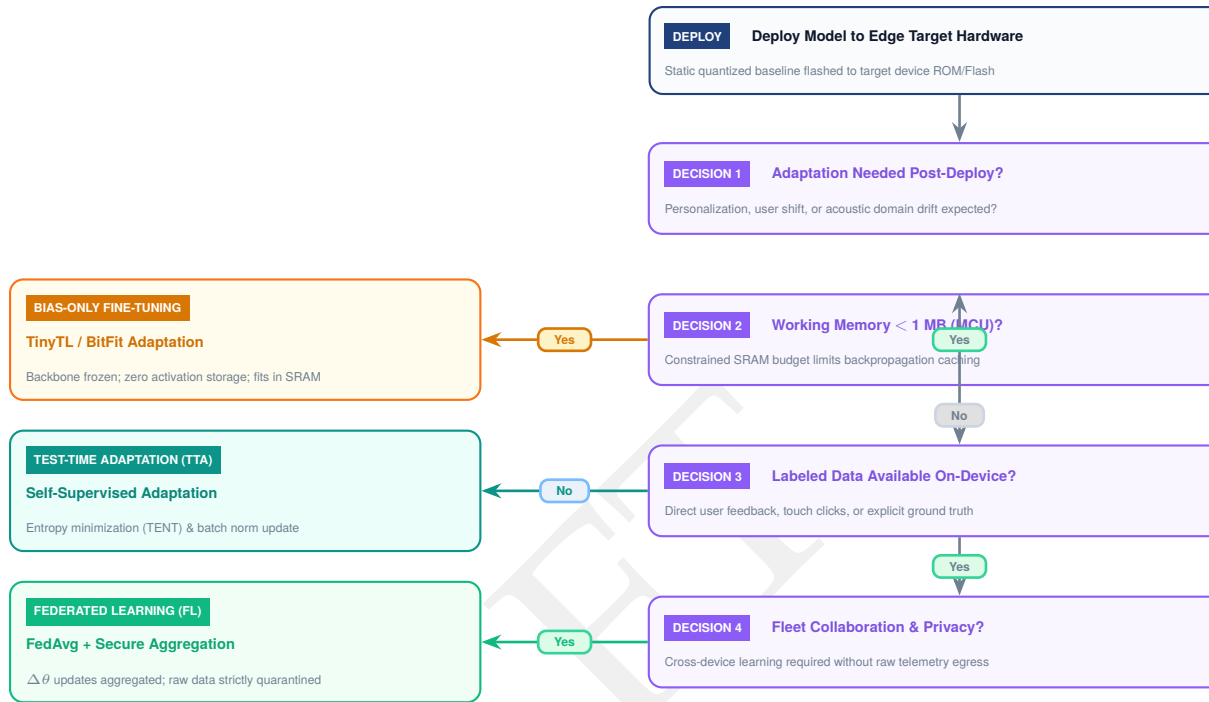
Figure 11.18: On-device learning design flow: This decision framework selects a technique for one device and policy. It maps adaptation complexity, compute availability, and data-sharing constraints to bias-only updates, adapters, full fine-tuning, localized learning, or federated coordination.
