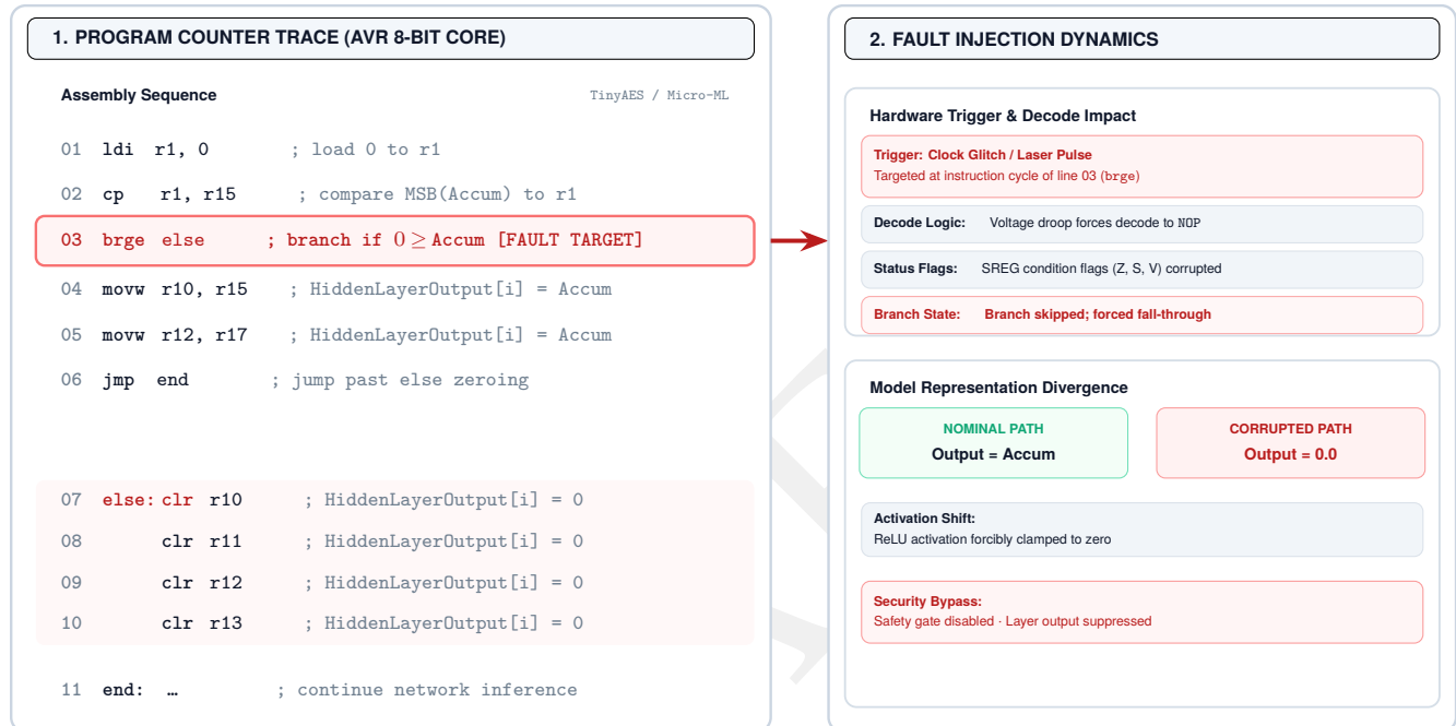
Figure 13.12: Fault injection attack: Manipulating assembly code bypasses safety checks, forcing a neuron’s output to zero regardless of input and demonstrating a hardware vulnerability in machine learning systems.
