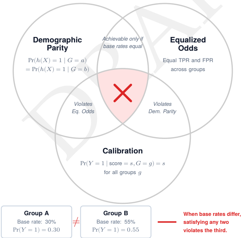
Figure 16.1: Fairness Impossibility Trade-Offs: Visualizing why common fairness criteria can conflict. Calibrated risk scores generally cannot also satisfy equalized error-rate conditions when base rates differ and prediction is imperfect; demographic parity adds a separate selection-rate constraint that may conflict with either goal. This forces engineers to make explicit normative choices based on the application context.
