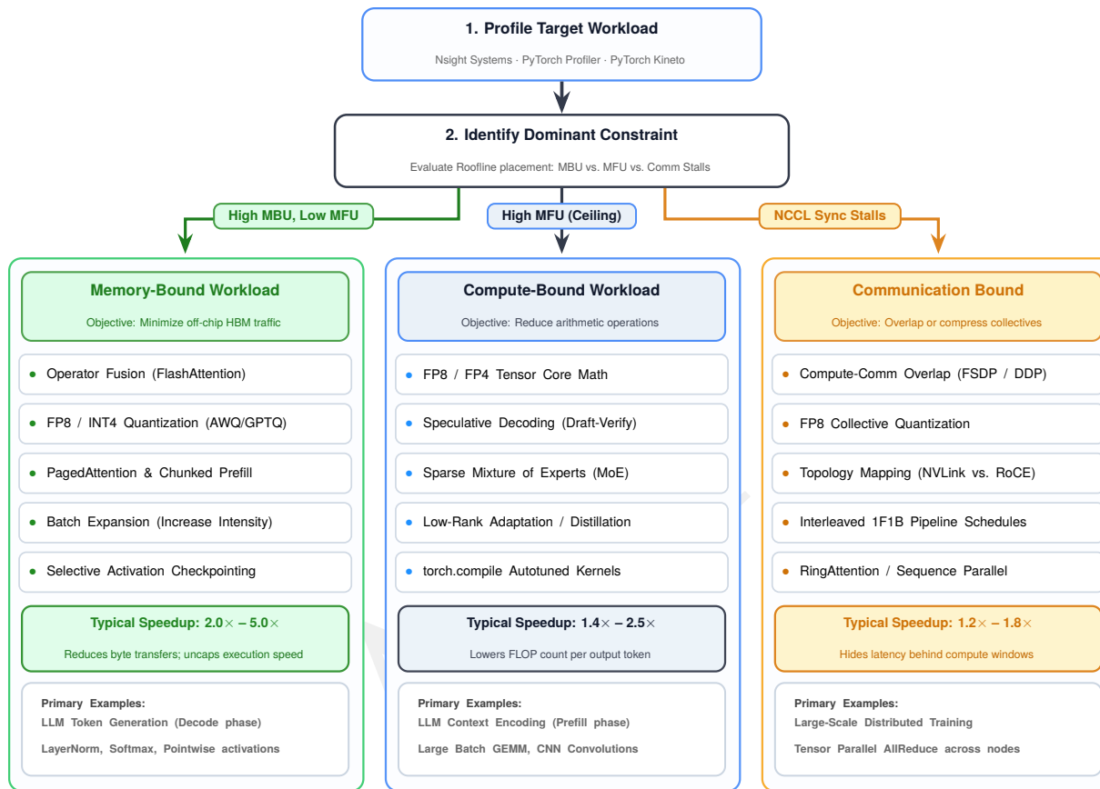
Figure 9.14: Optimization playbook decision tree: Systematic troubleshooting flow beginning with workload profiling and roofline classification, routing into memory-bound, compute-bound, or communication-bound playbooks with expected throughput speedups and iterative re-profiling.
