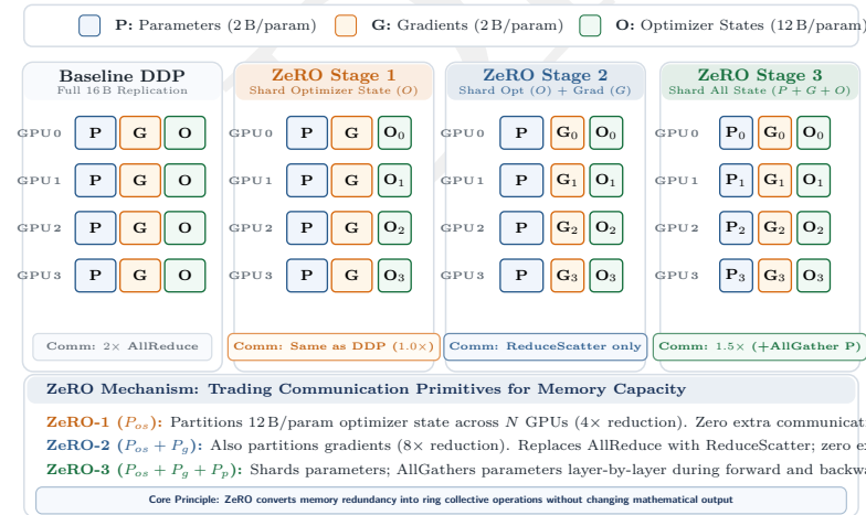
Figure 5.8: ZeRO state partitioning across GPU ranks: Memory layout per GPU for 4 workers under standard DDP versus ZeRO stages 1, 2, and 3. ZeRO-1 shards optimizer states ( O/4 ), ZeRO-2 adds gradient sharding ( G/4 ), and ZeRO-3 partitions all model state ( P/4, G/4, O/4 ).
