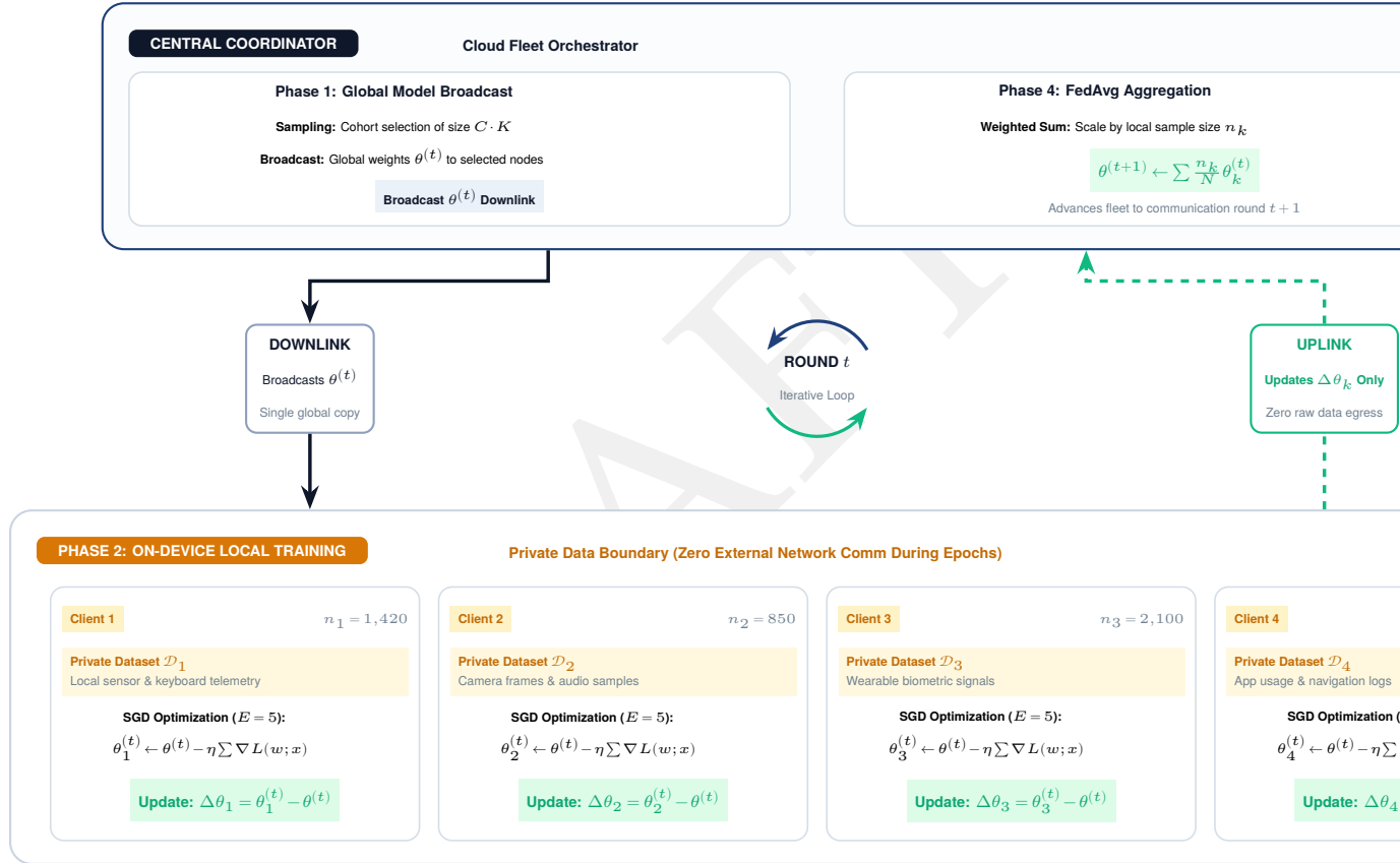
Figure 11.12: Federated averaging protocol: The four-phase cycle begins when the server broadcasts a global model to participating clients. Clients train locally on private data, upload model updates, and the server aggregates those updates into the next global model.
