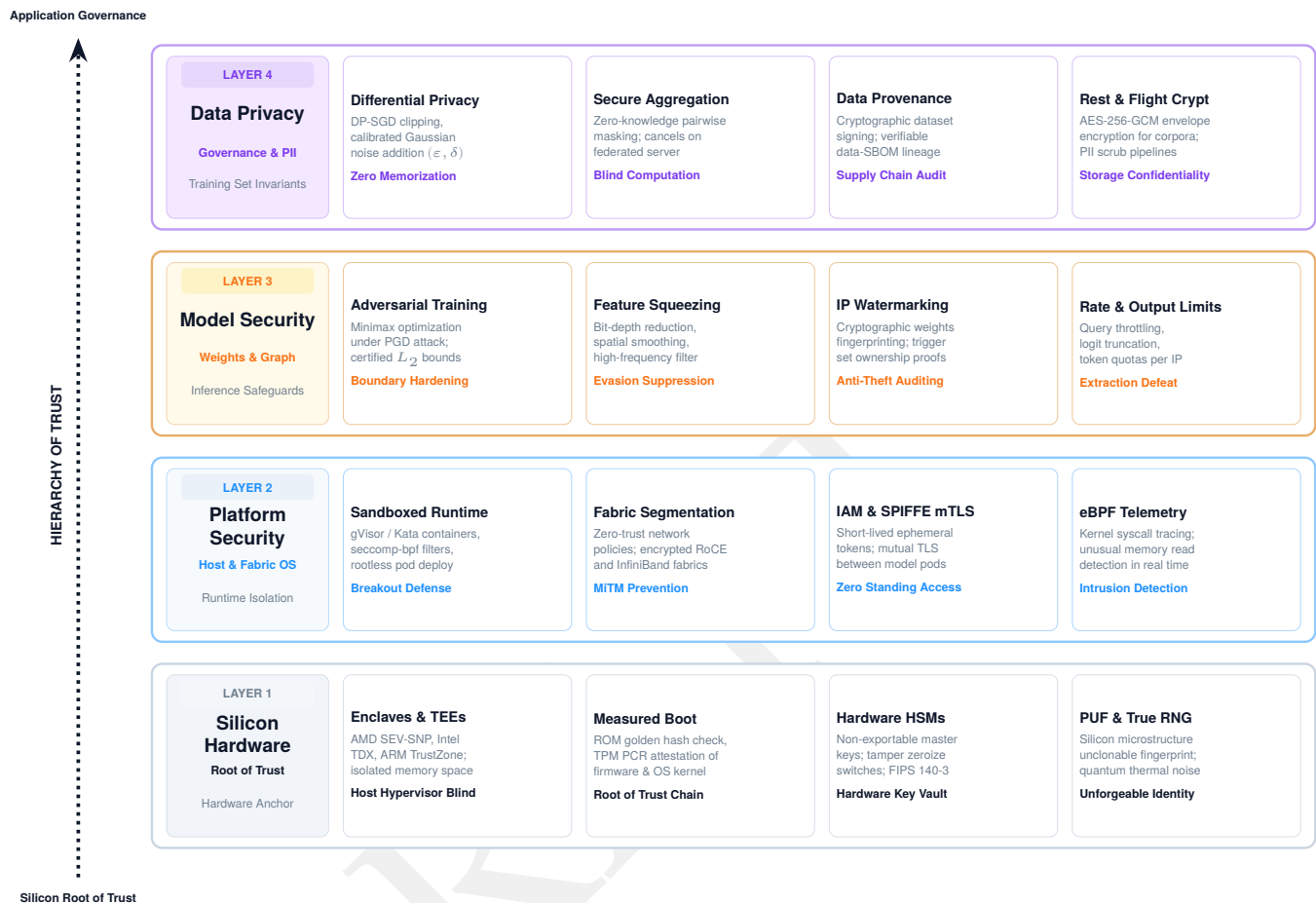
Figure 13.19: Layered defense stack: Machine learning systems require multi-faceted security strategies that progress from foundational hardware protections to data-centric privacy techniques, building trust across all layers. This architecture integrates safeguards at the hardware, system, model, and data levels to mitigate threats and ensure robust deployment in production environments.
