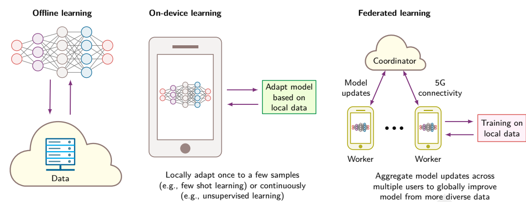
Figure 11.11: Federated learning balances data privacy with collective model improvement by coordinating local training across distributed devices, unlike offline learning’s centralized approach or on-device learning’s isolated adaptation. Each paradigm handles data location and model update strategies differently, revealing the trade-offs between personalization, data security, and global knowledge sharing.
