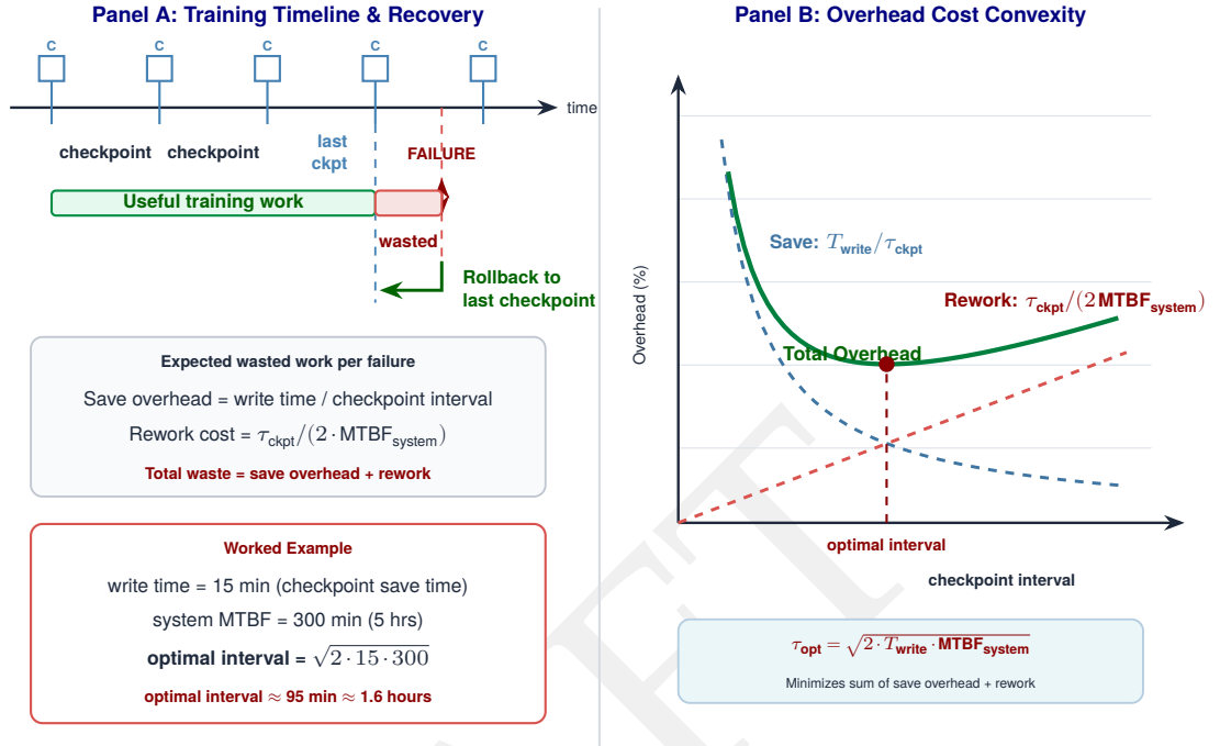
Figure 7.4: The Young-Daly optimal checkpoint: Total wasted work is the sum of checkpointing overhead (which decreases with interval \tau_{\text{ckpt}} ) and rework cost (which increases with \tau_{\text{ckpt}} ). The minimum point defines the optimal interval
