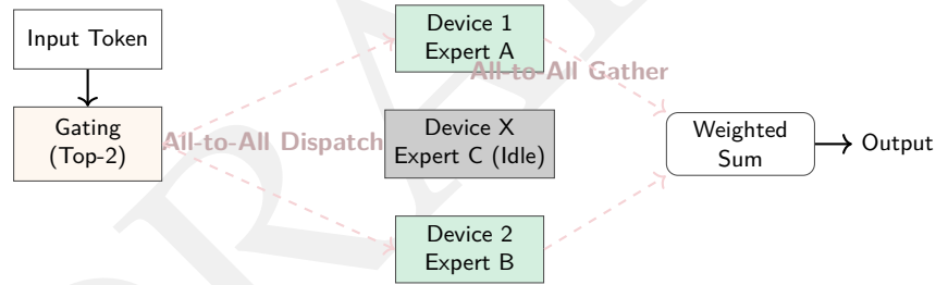
Figure 10.15: Mixture-of-experts (MoE) routing: Expert parallelism distributes “experts” across different devices. For each token, a gating mechanism selects the top- k experts. An AllToAll communication step dispatches tokens to the devices hosting their selected experts (1). Experts process the tokens in parallel (2). A second AllToAll step gathers the results back to the original device (3). This pattern enables massive model capacity but introduces all-to-all communication overhead.
