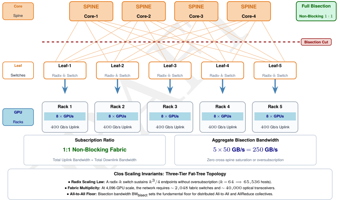
Figure 3.9: Nonblocking fat-tree topology: A three-tier Clos network built from radix- k switches. By ensuring that the number of uplinks at each level matches the number of downlinks, the topology provides full BW_{\text{bisection}} between any two pods. The multiple parallel paths between leaf and spine enable hardware-based adaptive routing to spray packets and avoid congestion.
