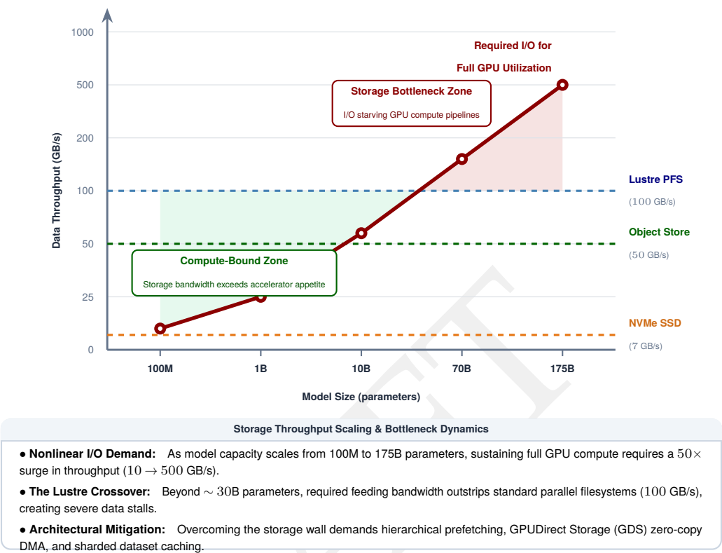
Figure 4.3: The storage bottleneck zone: Required I/O throughput for full GPU utilization rises with model size from 100 million to 175 billion parameters. The red curve shows storage demand; horizontal dashed lines mark common storage-tier ceilings (NVMe at 7 GB/s, object storage at 50 GB/s, and Lustre at 100 GB/s). Between the compute-bound and storage-bottleneck regions lies the transition where storage, not compute, limits training throughput.
