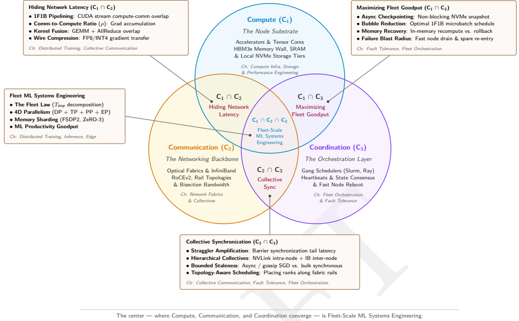
Figure 1.13: The C^3 Intersection Landscape: Compute ( C_1 ), Communication ( C_2 ), and Coordination ( C_3 ) partition distributed execution time across the node substrate, networking backbone, and orchestration layer. Pairwise intersections govern how effectively systems hide network latency, maximize fleet goodput, and synchronize collective operations. Their center is Fleet-Scale ML Systems Engineering.
