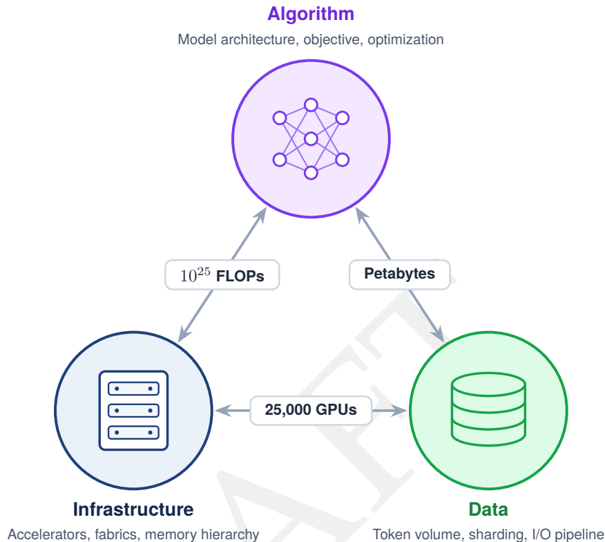
Figure 1.15: The AI triad at scale: The three interdependent components of every ML system. At production scale, each component's requirements intensify: data pipelines must handle petabytes with consistent quality; algorithms can demand 10^{25} FLOPs for large-model training; and infrastructure must coordinate thousands of accelerators while maintaining fault tolerance. Changes to any vertex cascade through the others, creating the multi-dimensional optimization challenge that defines ML systems engineering.
