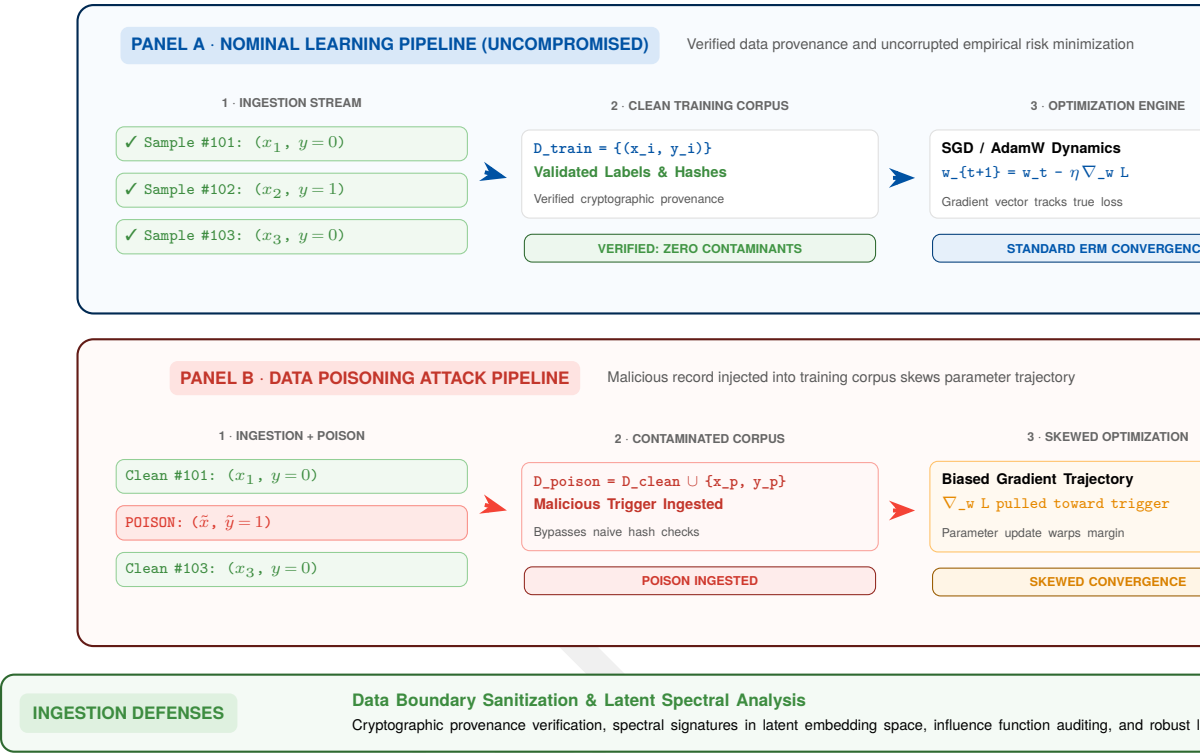
Figure 14.17: Data Poisoning Impact: A single poisoned record injected into the training set corrupts the model the pipeline produces, contrasting a normal learning pipeline (clean data, dataset, learning algorithm, model) against a poisoning attack where one malicious record carries through to the trained model. Even limited adversarial control over training data can disrupt model learning, highlighting the vulnerability of data-driven approaches to malicious manipulation.
