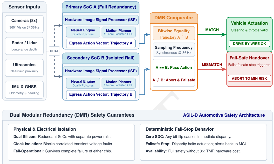
Figure 7.21: Dual modular redundancy (DMR): Tesla’s full self-driving computer employs a DMR architecture, replicating critical computations across two independent system-on-chips (SoCs). A hardware comparator unit validates that both chips produce matching outputs before allowing a control command to reach the vehicle’s actuators, ensuring that a single-chip hardware failure or bit flip cannot trigger dangerous driving behavior.
