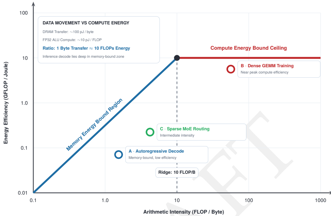
Figure 15.9: Energy Roofline Model: Just as performance rooflines limit FLOP/s based on bandwidth, energy rooflines limit FLOP/J. Workloads with low arithmetic intensity (left) are dominated by memory energy ( E_{\text{move}} ), while compute-heavy workloads (right) are limited by arithmetic energy ( E_{\text{compute}} ). Optimizing the wrong metric yields diminishing returns.
