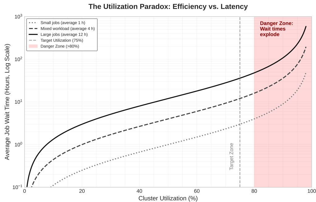
Figure 8.15: The utilization paradox: As cluster utilization approaches saturation (100 percent), job wait times increase hyperbolically and diverge near saturation, not linearly. Operating above 80 percent utilization (the danger zone) causes unpredictable scheduling delays, especially for large jobs, illustrating why 100 percent utilization is an anti-pattern for interactive research clusters. A dashed line shows target utilization at 75 percent.
