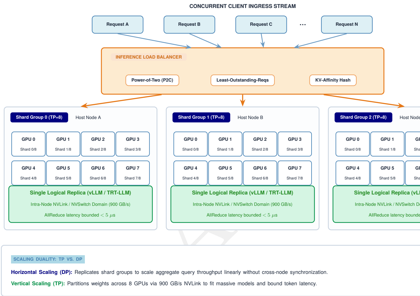
Figure 10.20: Horizontal scaling with shard groups: The load balancer treats each shard group as a single logical inference server. Within each group, 8 GPUs coordinate via tensor parallelism. Adding groups scales throughput linearly; adding GPUs per group reduces per-request latency.
