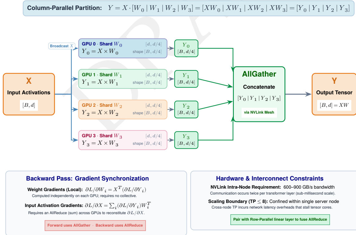
Figure 5.12: Tensor parallelism data flow: Tensor parallelism column-splits a single weight matrix ( W_0 \dots W_3 ) across four GPUs, with each GPU computing a partial output that is recombined through an AllGather. The companion strategy, pipeline parallelism, partitions layers vertically across stages and is shown separately in the layer-block figure. The two strategies are often combined in hybrid 3D parallelism for large models.
