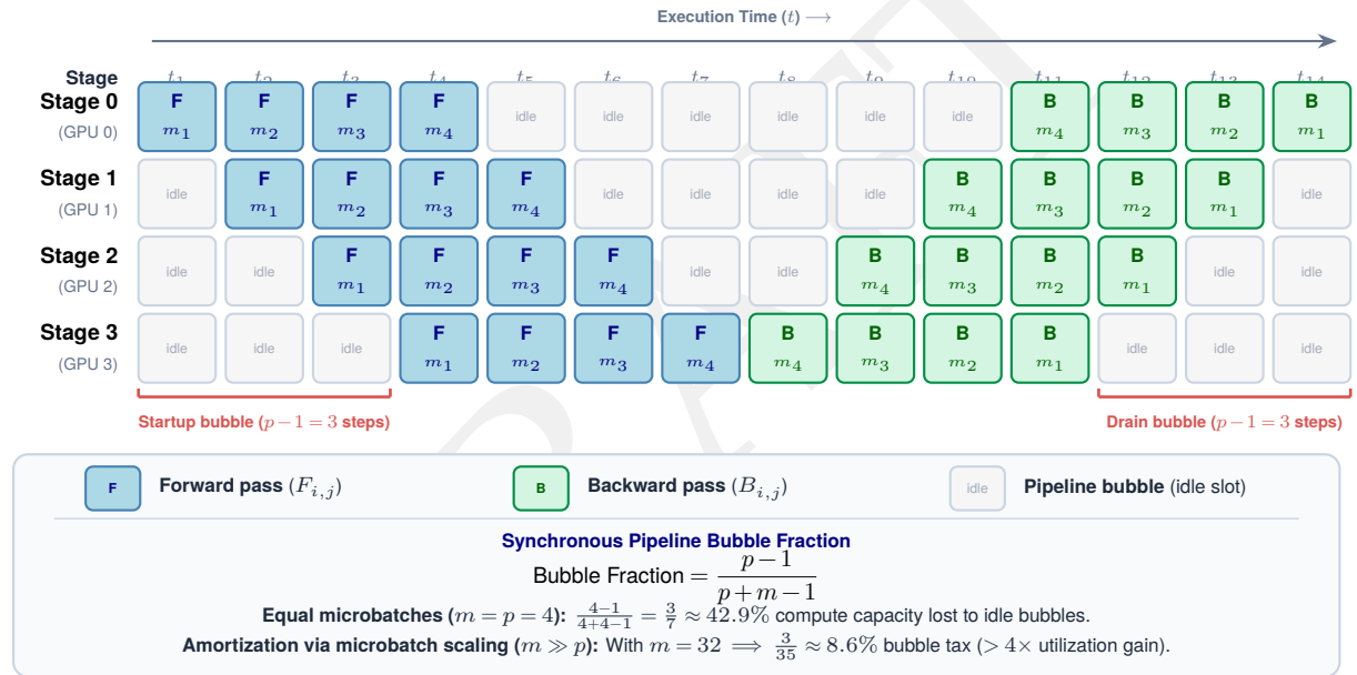
Figure 5.15: Pipeline parallelism schedule: A 4-stage pipeline processes 4 microbatches through forward passes ( F_{i,j} ) and backward passes ( B_{i,j} ) over time. Rows represent pipeline stages, and columns represent time steps. Staggering the work lets one stage process a microbatch while another handles an earlier or later microbatch, reducing idle time without eliminating the fill, drain, and dependency bubbles visible in the schedule.
