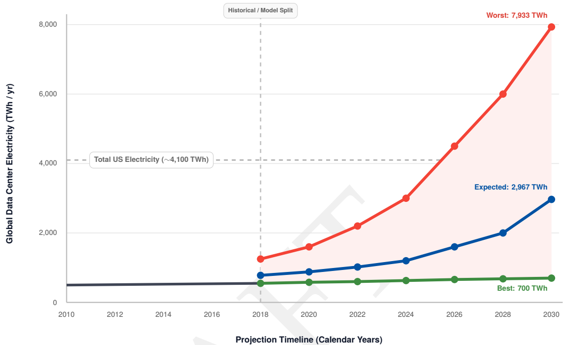
Figure 15.3: High-Growth Data Center Energy Sensitivity Scenarios: Global data center electricity consumption scenarios from 2010 to 2030 under aggressive demand-growth assumptions. The three trajectories—best case, expected, and worst case—diverge sharply after 2018, highlighting the uncertainty and importance of efficiency improvements; they should be read as a sensitivity envelope, not as the IEA baseline projection.
