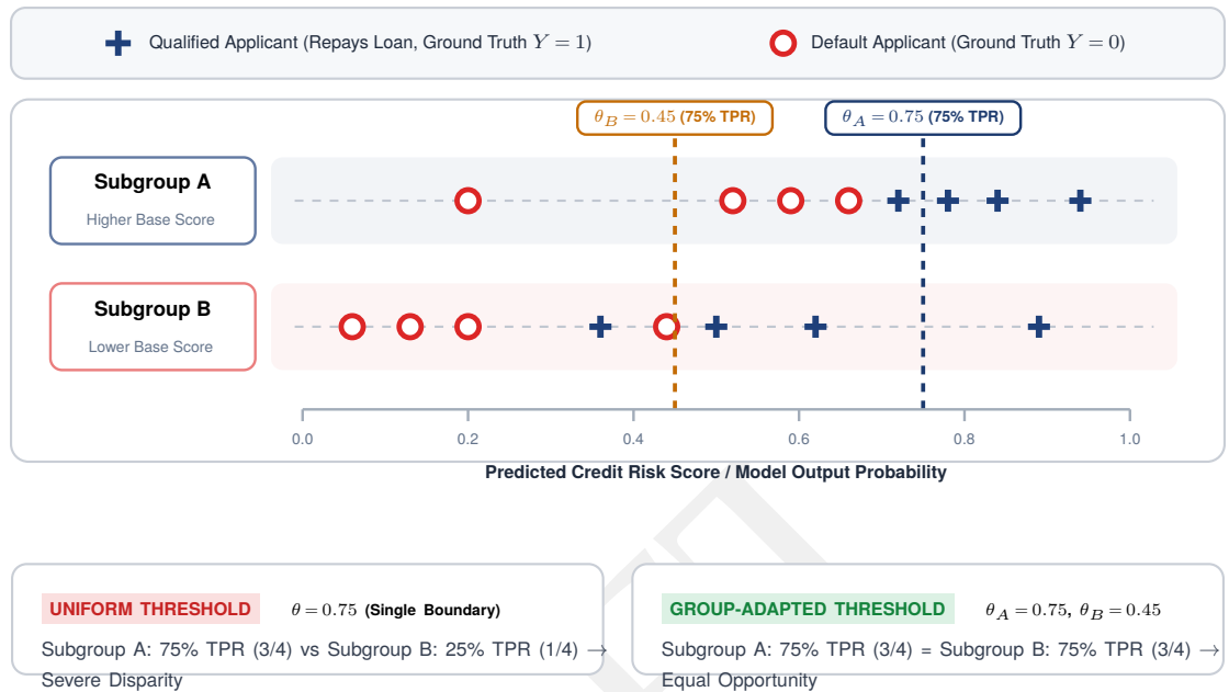
Figure 16.5: Threshold-Dependent Fairness: Varying classification thresholds across subgroups allows equal true positive rates but introduces complexity in model serving and necessitates access to sensitive attributes at inference time. Achieving fairness requires careful consideration of subgroup-specific performance, as a single threshold may disproportionately impact certain groups, highlighting the tension between accuracy and equitable outcomes in machine learning systems.
