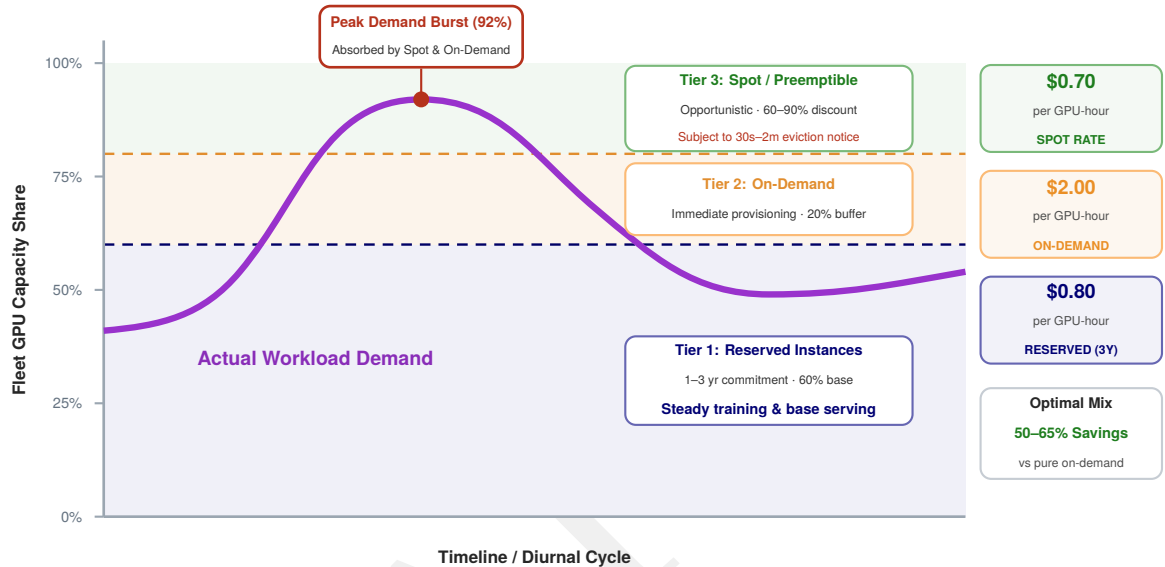
Figure 8.12: Capacity reservation tiers and portfolio optimization: The three cloud capacity tiers (Reserved, On-Demand, and Spot/Preemptible) trade unit cost against commitment and availability guarantees. Schedulers map steady-state baseline demand to reserved capacity, diurnal spikes to on-demand instances, and restart-tolerant training to discounted spot pools.
