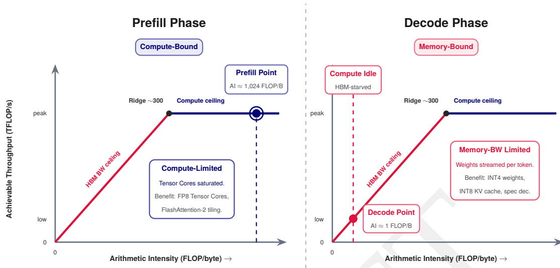
Figure 9.5: Prefill versus decode roofline comparison: Operational regimes of LLM prompt evaluation (prefill) versus autoregressive token generation (decode) plotted on the hardware roofline model. Prefill operates in the compute-bound regime at high arithmetic intensity ( I \gg I_{\text{ridge}} ), whereas decode is bound by HBM memory bandwidth ( I \ll I_{\text{ridge}} ).
