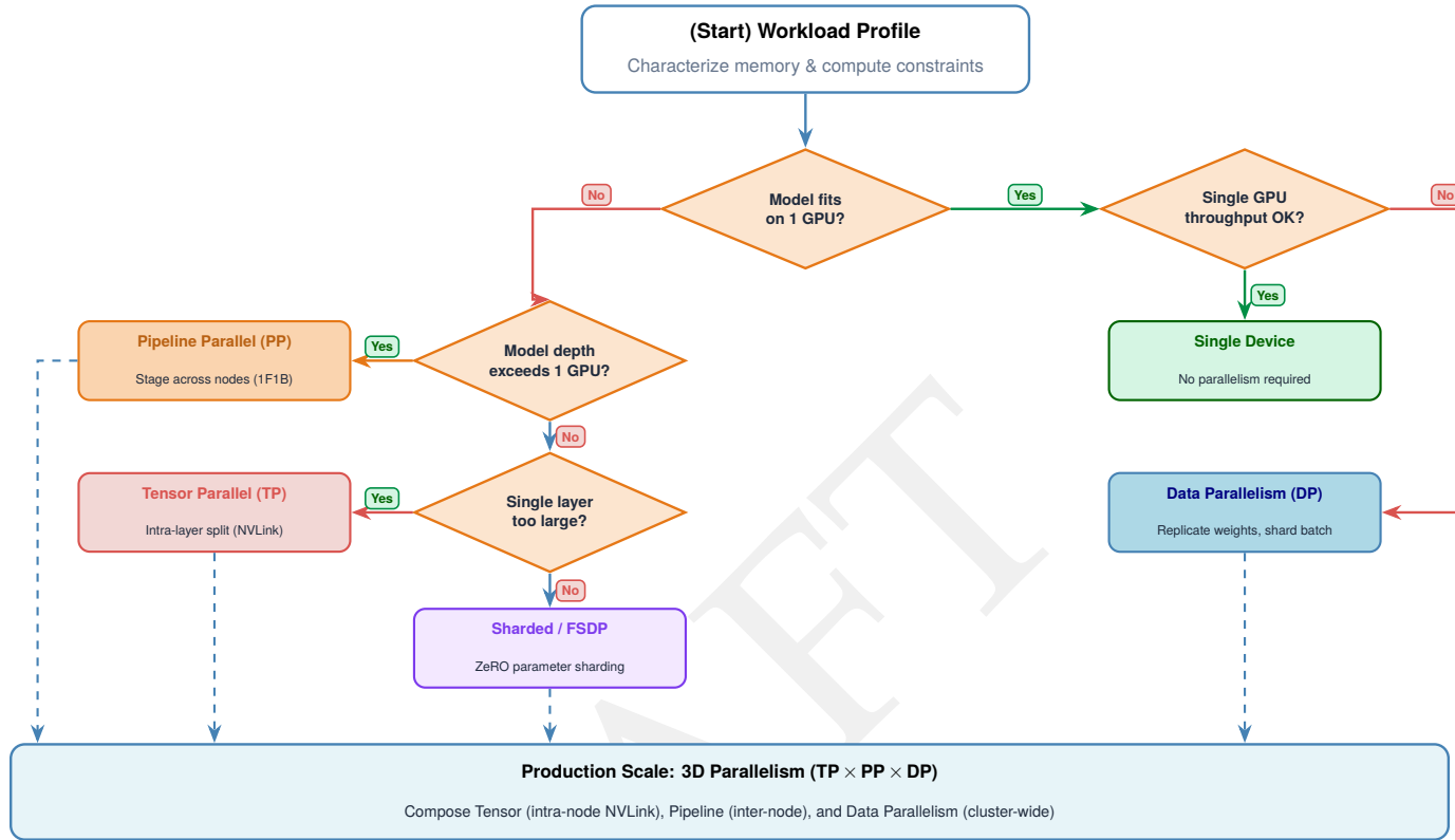
Figure 5.19: Parallelism strategy decision framework: A systematic selection guide based on two key questions: Does the model state fit in single-device memory, and does the required data throughput justify multiple replicas? Models exceeding device memory require model parallelism or sharding; workloads whose model fits but whose throughput target exceeds one device benefit from data parallelism; significant constraints in both dimensions demand hybrid approaches. While simplified, this framework captures the primary decision points before practitioners must consider secondary factors like hardware heterogeneity and workload imbalance.
