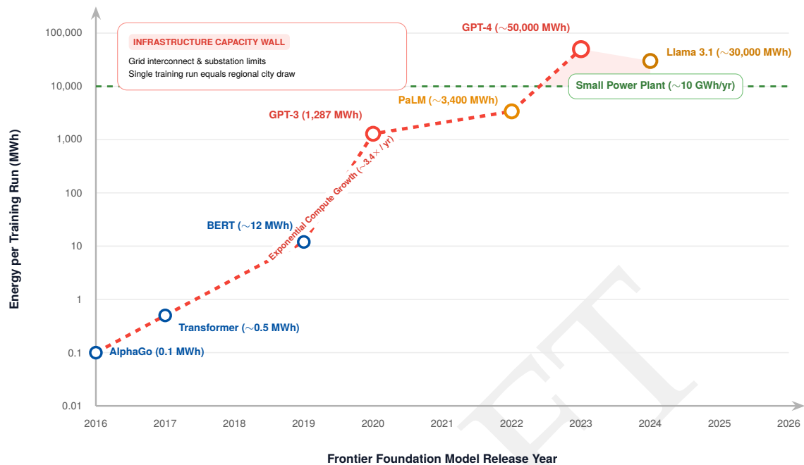
Figure 15.4: The Energy Wall: Training-run energy (MWh) plotted across 2016–2026 against a horizontal power-plant reference line, with milestone models annotated along the trajectory. The curve rises by roughly 350,000× across this window in published estimates while battery density and grid efficiency improve at only 2–5 percent annually, framing the ‘energy wall’ where algorithmic ambition outruns the physical substrate.
