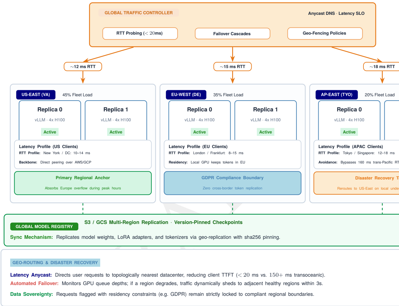
Figure 10.24: Global load balancing across inference regions: A global load balancer routes requests to three independent regional deployments (US-East, EU-West, Asia-Pacific) based on latency. Each region operates independently; a shared model registry synchronizes weights. During regional failure, the LB reroutes to the next nearest healthy region.
