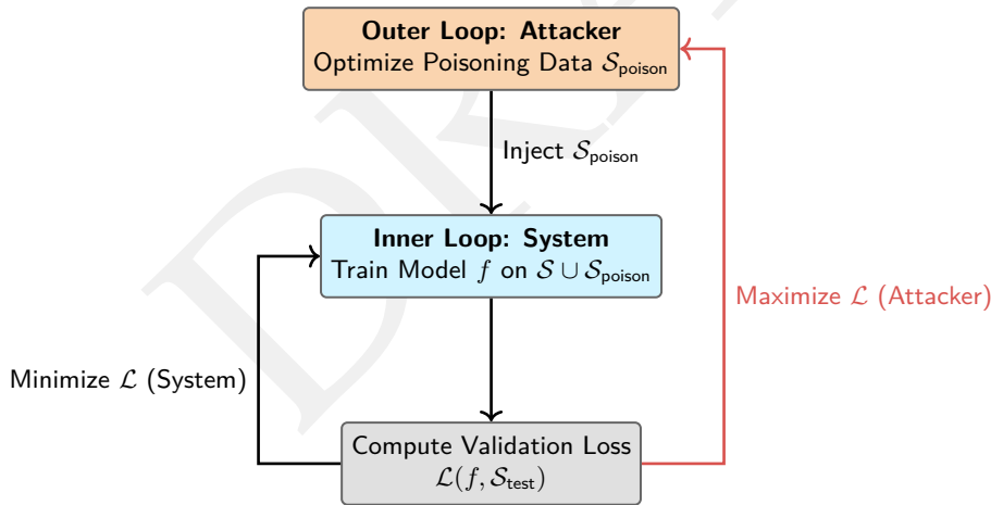
Figure 13.6: Data poisoning as bilevel optimization: The attacker (Outer Loop) seeks to find poisoning data \mathcal{S}_{\text{poison}} that maximizes the model's loss on a target test set. The system (Inner Loop) attempts to minimize its training loss on the combined dataset \mathcal{S} \cup \mathcal{S}_{\text{poison}} . This minimax dynamic makes defending against poisoning computationally difficult, as evaluating a defense requires simulating the full training process.
