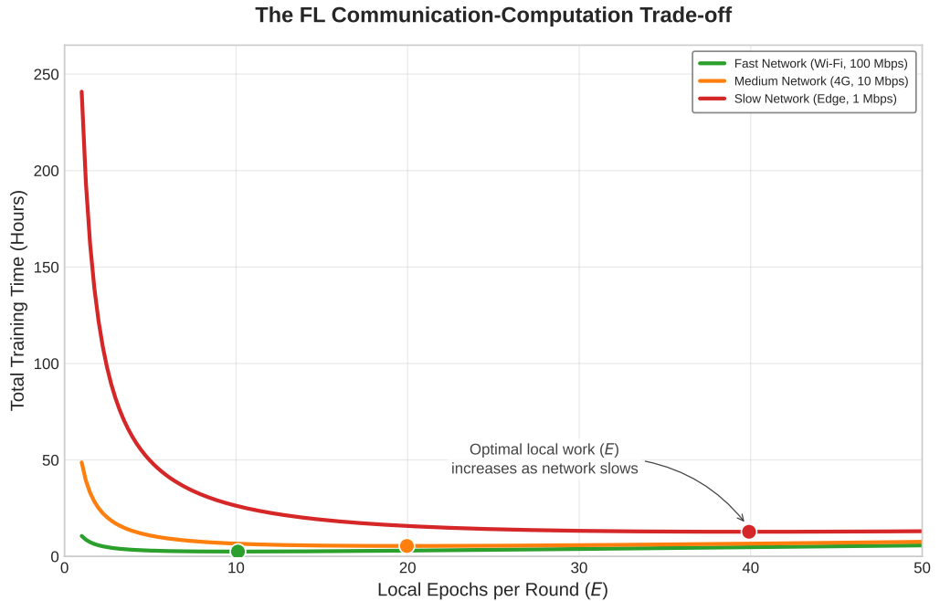
Figure 11.14: Communication-computation trade-off in federated learning: As network bandwidth decreases from fast to slow, the time-minimizing number of local epochs shifts rightward because additional local computation amortizes more communication. Excessive local work eventually increases total time when client drift requires more global rounds to converge.
