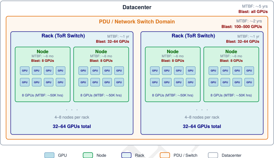
Figure 7.11: Hierarchy of failure domains: Failure domains are often nested or overlapping. A GPU failure affects one device. A node failure affects 8 GPUs. A rack switch failure affects 32-64 GPUs. A power distribution unit (PDU) failure may affect multiple racks. Effective fault tolerance requires placing replicas across independent domains (for example, different racks or rows) to survive correlated failures.
