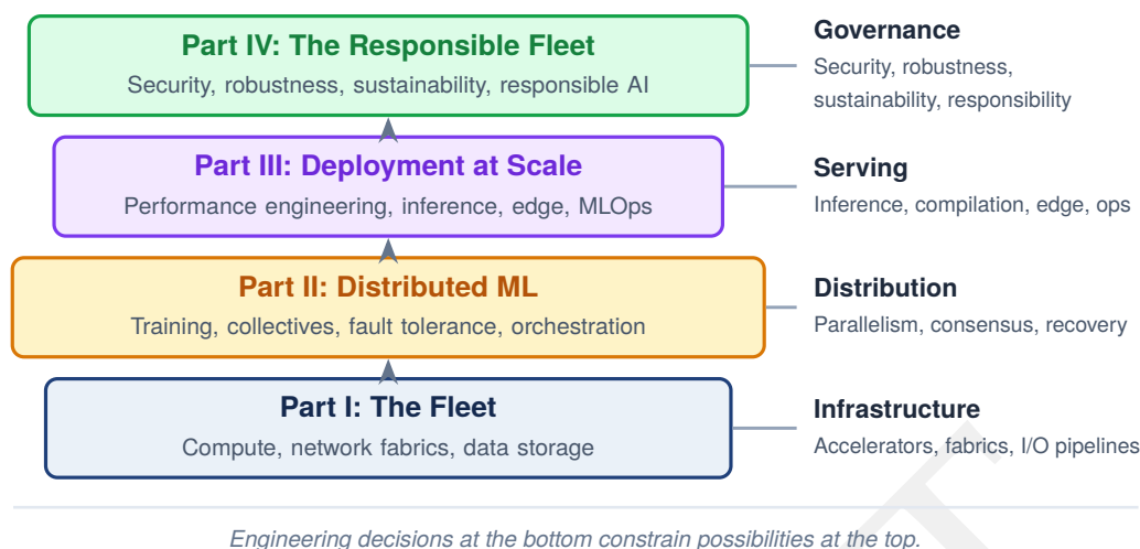
Figure 1.14: The fleet stack: The organizing framework for this book. The architecture builds from the Infrastructure layer (compute, network, data) up through the Distribution layer (parallelism, communication, fault tolerance) and Serving layer (inference, performance, edge, operations) to the Governance layer (security, robustness, sustainability, responsible engineering). Engineering decisions at the bottom constrain possibilities at the top.
