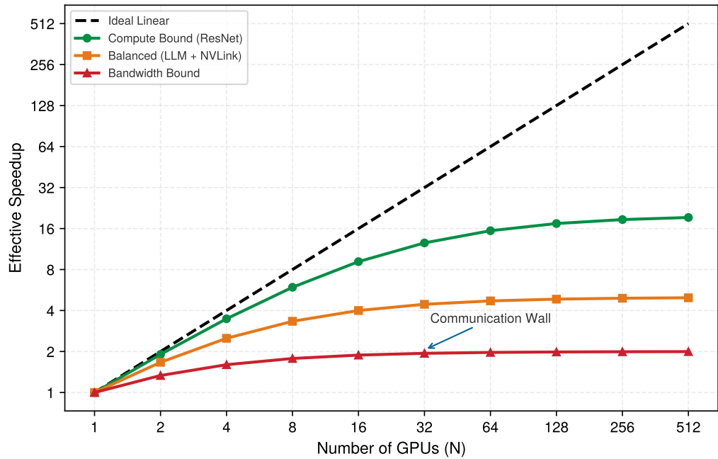
Figure 5.9: The scaling tax: Effective speedup vs. number of GPUs. While ideal scaling (dashed black) is linear, real-world systems pay a ‘tax’ for communication. Compute-bound models like ResNet (green) scale well because they have high arithmetic intensity. Bandwidth-bound models like GPT-3 (red) hit a communication wall where adding more GPUs yields diminishing returns (efficiency < 50 percent).
