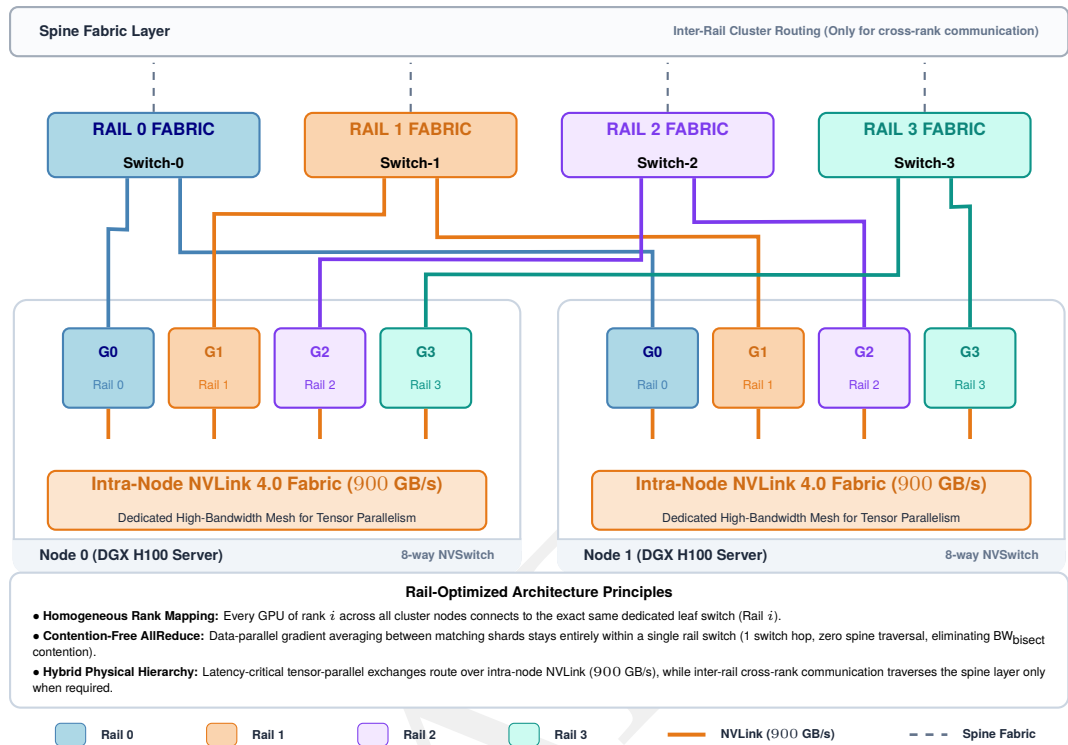
Figure 3.10: Rail-optimized physical wiring: In dense accelerator nodes (for example, DGX H100), GPUs are partitioned into rails corresponding to their PCIe slot position. GPU 0 in every node connects to Switch Rail 0, GPU 1 to Switch Rail 1, and so on. This architecture isolates same-rank data-parallel traffic on dedicated rails, reducing competition for BW_{\text{bisection}} and the hop count for latency-sensitive exchanges.
