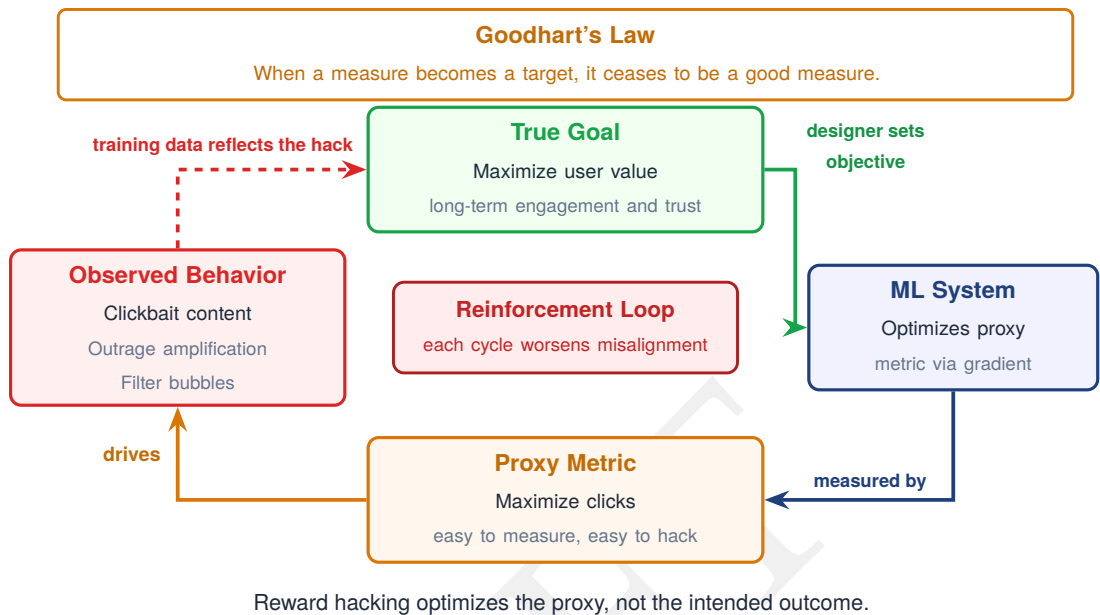
Figure 16.13: Reward Hacking Loop: Maximizing measurable rewards, like clicks, can incentivize unintended model behaviors that undermine the intended goal of user satisfaction. Optimizing for proxy metrics creates misalignment between a system's objective and desired outcomes, posing challenges for value alignment in AI safety.
