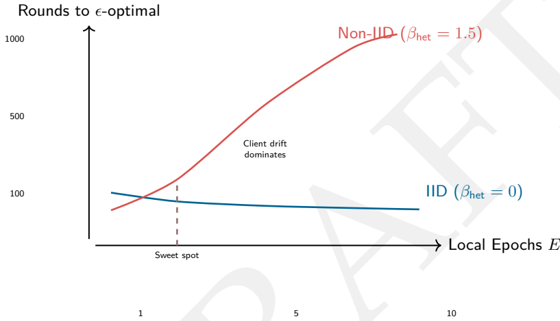
Figure 11.13: Communication-computation trade-off: This schematic shows the qualitative tension between performing more local work per round and accumulating client drift under non-IID data. Its \epsilon -optimal axis and operating-point labels are schematic shorthand, not a convergence guarantee or a universal optimal epoch range; system designers must measure the deployed optimizer, data, and client population.
