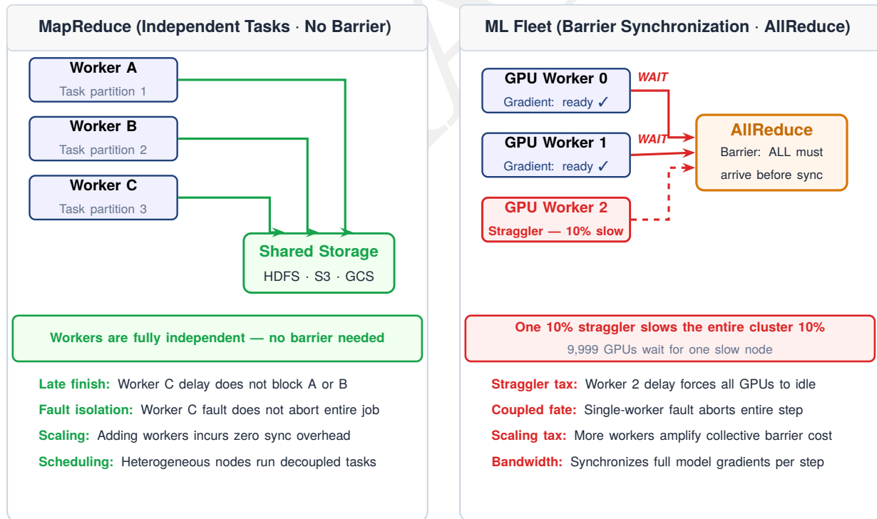
Figure 1.5: Barrier synchronization vs. independent tasks: MapReduce workers (left) operate independently, writing results to shared storage without coordination. A straggler delays only its own output. ML Fleet workers (right) must synchronize gradients at an AllReduce barrier every training step, meaning a single 10% straggler slows the entire cluster by 10%.
