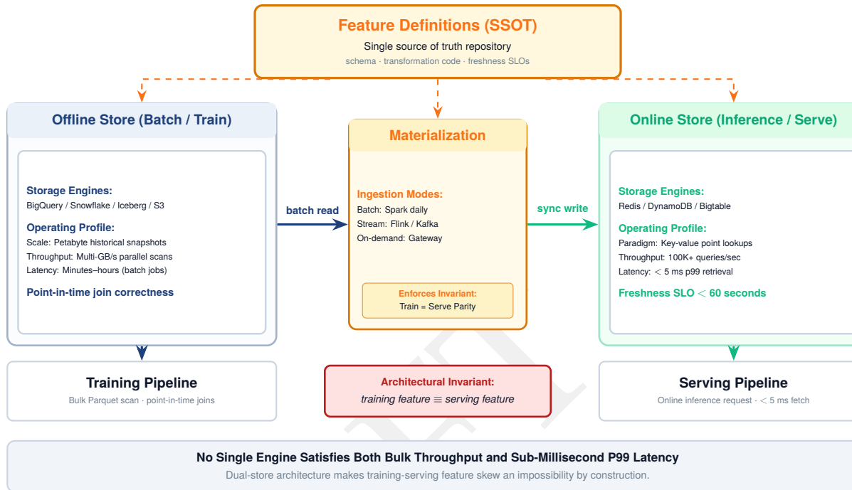
Figure 12.11: Feature store architecture: A dual-store architecture resolves the conflict between training (high-throughput batch scans) and serving (low-latency point lookups). Features are materialized from batch and streaming sources into an offline store (for training) and an online store (for serving), ensuring consistency across the ML lifecycle.
