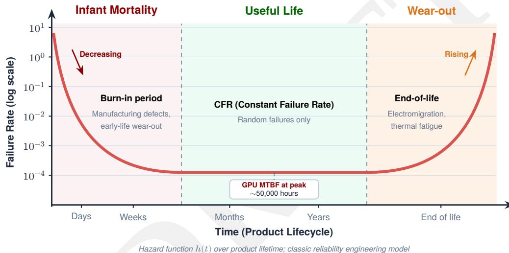
Figure 7.12: The bathtub curve: Hardware failure rates \lambda(t) vary over time. (1) Infant mortality: high failure rate initially due to manufacturing defects. (2) Useful life: constant, low failure rate where random failures dominate. (3) Wear-out: increasing failure rate as components age. Burn-in testing aims to filter out infant mortality failures before deployment.
