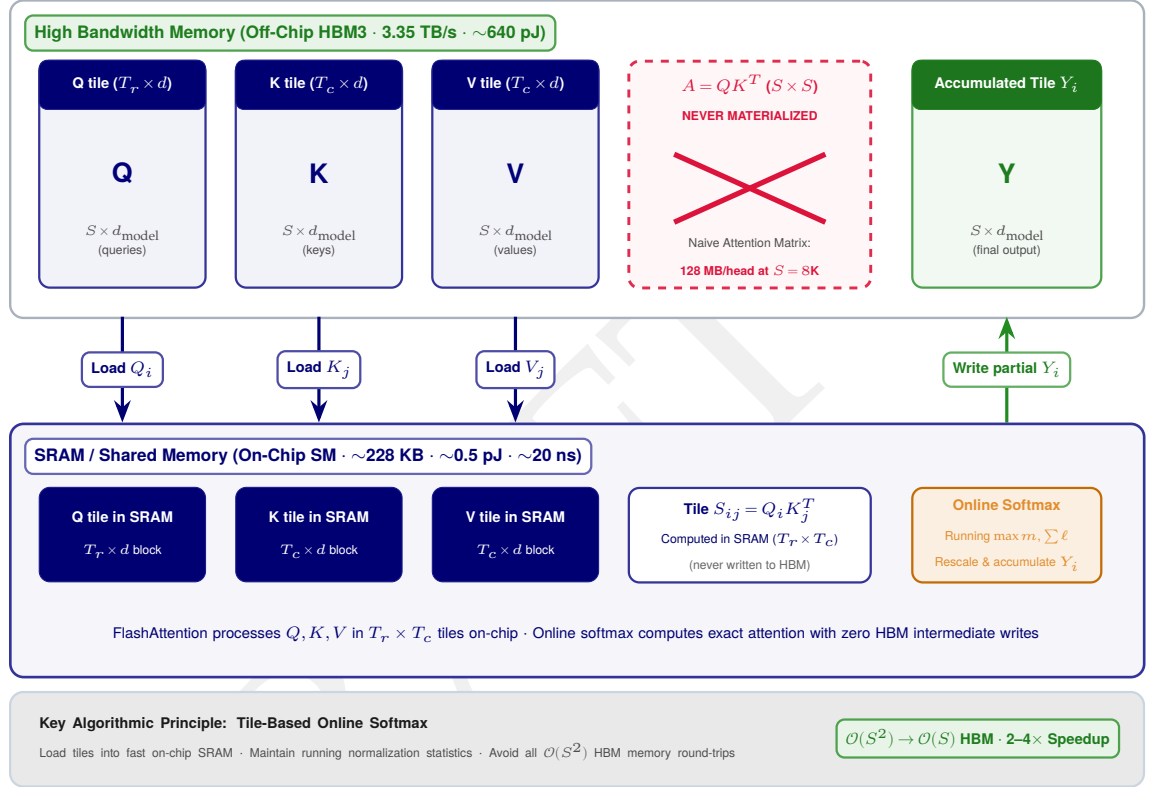
Figure 9.7: FlashAttention memory hierarchy tiling: Block-by-block scheduling of Q , K , and V matrices loaded into on-chip shared memory (SRAM). Attention scores are computed and rescaled online without materializing the quadratic S \times S intermediate matrix in off-chip HBM, reducing memory traffic from \mathcal{O}(S^2) to \mathcal{O}(S) .
