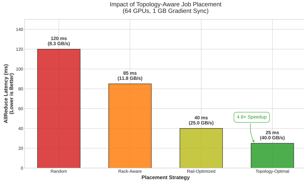
Figure 8.7: Topology placement impact: AllReduce latency across four placement strategies (Random, Rack-Aware, Rail-Optimized, and Topology-Optimal) for a 1 GB gradient sync on 64 GPUs. Topology-aware scheduling reduces sync latency from 120 ms to 25 ms, yielding a 4.8× speedup.
