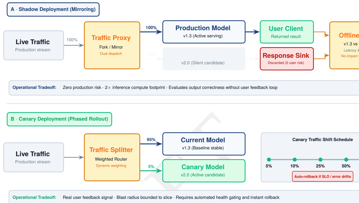
Figure 12.7: Shadow deployment architecture: Production traffic is mirrored to the shadow model asynchronously. The router returns the production response to the user immediately, while both responses are logged for offline quality comparison and operational validation.
