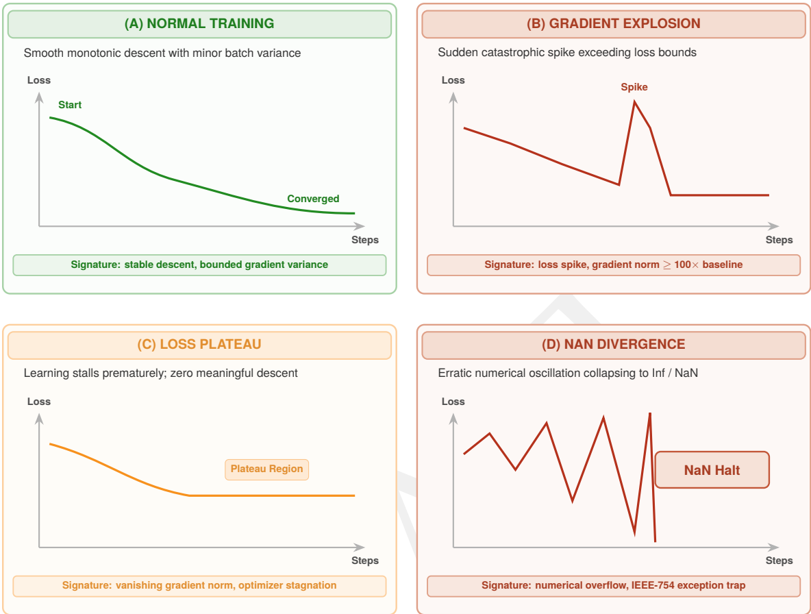
Figure 7.32: Training failure signatures: Common patterns of model loss over time that indicate underlying system or algorithmic failures. (A) Normal training. (B) Gradient explosion. (C) Loss plateau. (D) NaN divergence. Identifying these signatures automatically is essential for rapid recovery in autonomous training pipelines.
