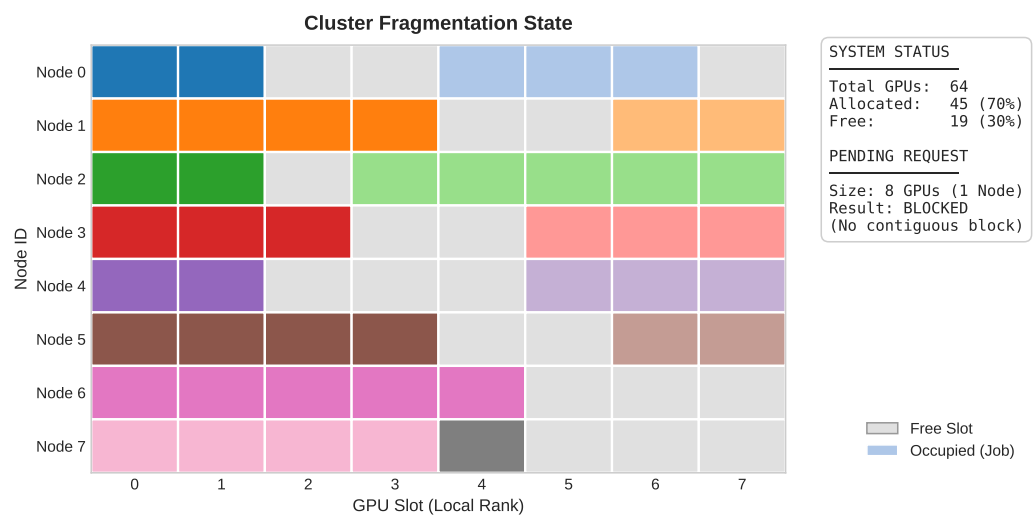
Figure 8.2: The fragmentation problem: The heatmap shows a snapshot of an 8-node cluster (rows) with 8 GPUs each (columns). Different colors represent distinct active jobs, while gray slots represent free GPUs. Although 19 GPUs (roughly 30 percent of capacity) are available globally, they are fragmented across nodes. A new job requiring 8 contiguous GPUs (a full node) cannot be scheduled because no single row is completely empty, illustrating how bin-packing inefficiencies reduce effective cluster capacity.
