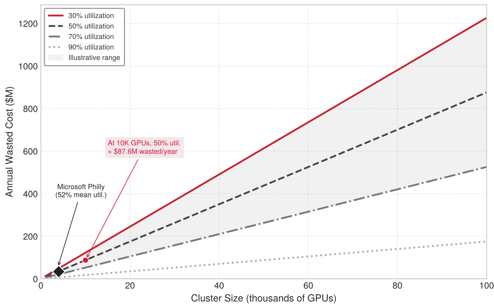
Figure 8.11: The cost of idle GPUs: Annual wasted cost as a function of cluster size for different GPU utilization levels, assuming $2/GPU-hour (cloud equivalent). The shaded region between 30 percent and 70 percent is an illustrative operating range for the scenario analysis. At 10,000 GPUs with 50 percent utilization, the model yields $87.6 million in annual wasted capacity. The Microsoft Philly data point marks the published mean GPU utilization of 52 percent. Data sources: (Jeon et al. 2019; Li et al. 2023).
