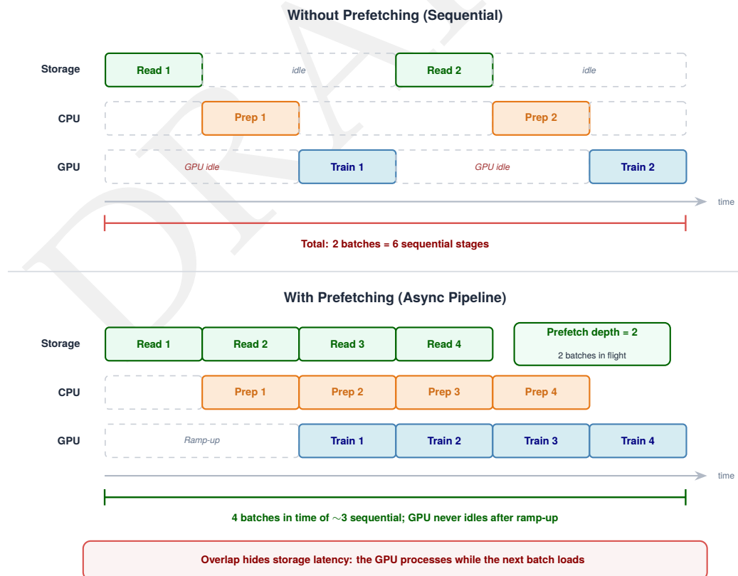
Figure 4.8: Pipelined data loading: The CPU prepares batch i + 1 while the GPU processes batch i . Pipelining hides storage latency, but only if the prefetch buffer is deep enough to absorb variance.
