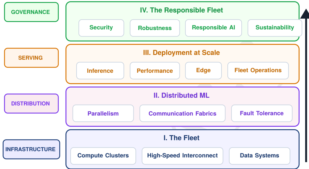
Figure 17.1: The Fleet Stack: The physical foundation (The Fleet) determines capability, while the distribution layer (Distributed ML) and serving layer (Deployment) define the engineering environment. These are constrained by governance requirements (The Responsible Fleet), with the emergent property of Scale creating qualitative changes that unify the discipline.
