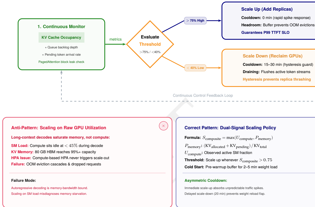
Figure 8.13: Inference autoscaling closed-loop control: A dual-signal control architecture monitors both GPU memory pressure (KV cache occupancy) and compute load (SM utilization, queue depth). Telemetry feeds both a reactive HPA loop and a predictive prewarming controller that provisions replicas ahead of cold-start deadlines.
