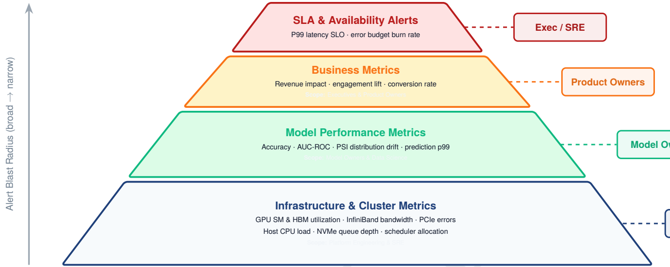
Figure 12.9: Hierarchical monitoring architecture: To prevent alert fatigue, monitoring operates at four abstraction levels. High-level business metrics trigger alarms for broad issues, while lower-level metrics are used primarily for investigation and root cause analysis.
