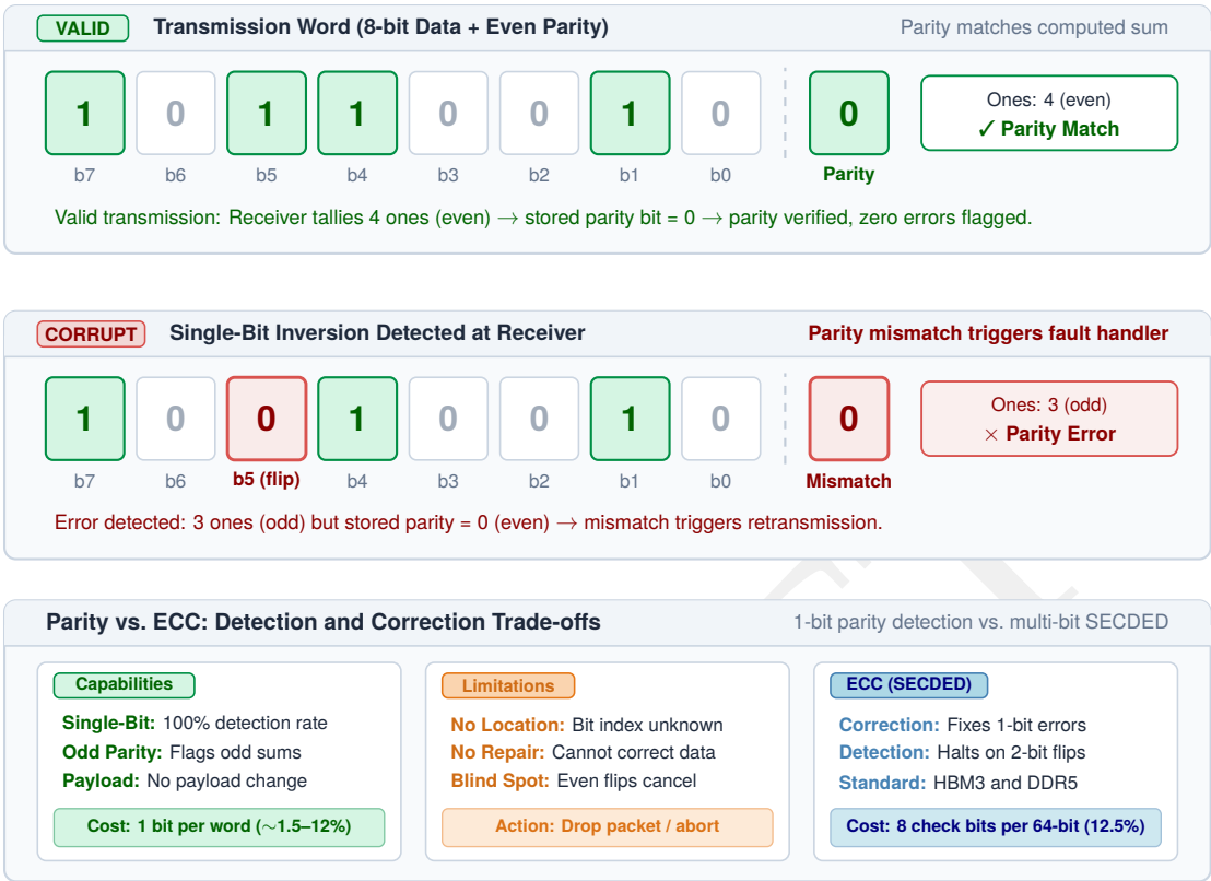
Figure 7.20: Parity-bit error detection and trade-offs: Even-parity bit check scheme where an extra parity bit detects single-bit inversions during data transmission or memory storage. While parity detects single-bit errors with minimal overhead, it cannot locate or correct errors, and double-bit flips cancel out undetected—motivating multi-bit SECDED ECC in high-density accelerator memory.
