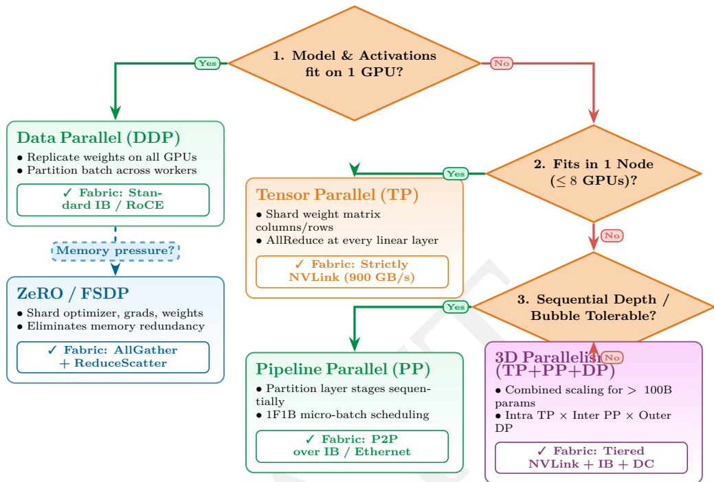
Figure 5.3: Parallelism strategy decision tree: Starting from the model’s memory footprint, the tree evaluates hardware-boundary constraints to identify viable execution strategies. The branches compare parameter and activation capacity against single-device and single-node physical limits, pairing each resulting strategy with its required interconnect tier.
