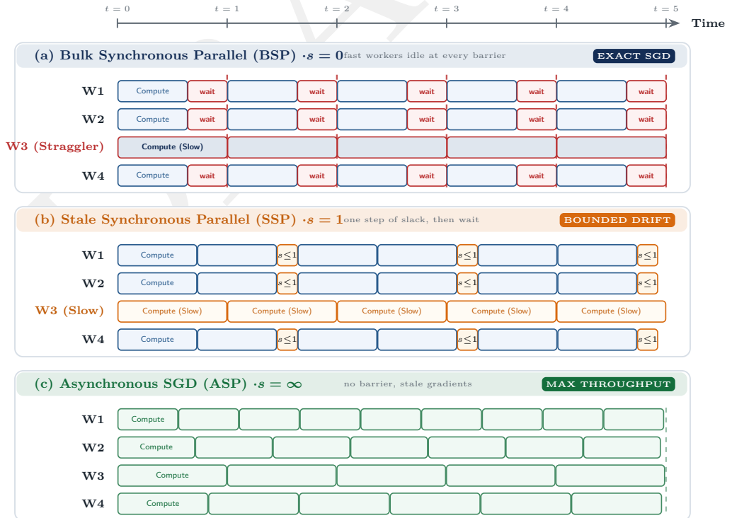
Figure 5.6: Distributed synchronization models: The timelines compare three synchronization strategies. (a) Bulk synchronous parallel (BSP) forces all workers to wait at a global barrier every step. (b) Stale synchronous parallel (SSP) allows workers to proceed up to s steps ahead of the slowest worker. (c) Asynchronous SGD eliminates barriers, increasing throughput at the cost of gradient staleness.
