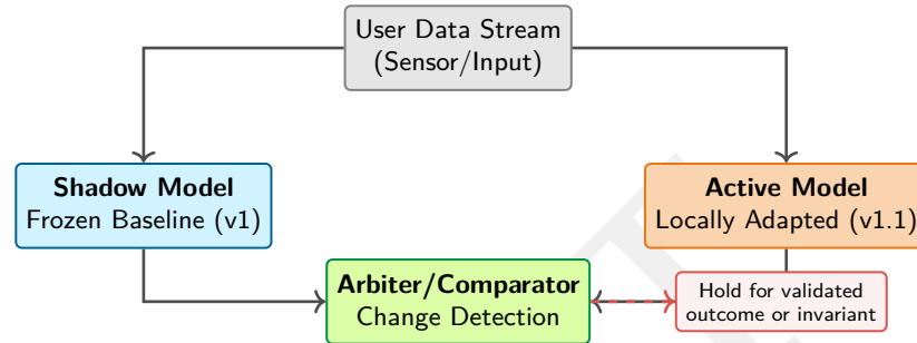
Figure 11.20: On-device shadow validation: A frozen baseline runs beside the active model. Their disagreement, confidence, latency, and resource deltas can flag a change without labels; a rollback decision still requires a validated outcome signal or safety invariant.
