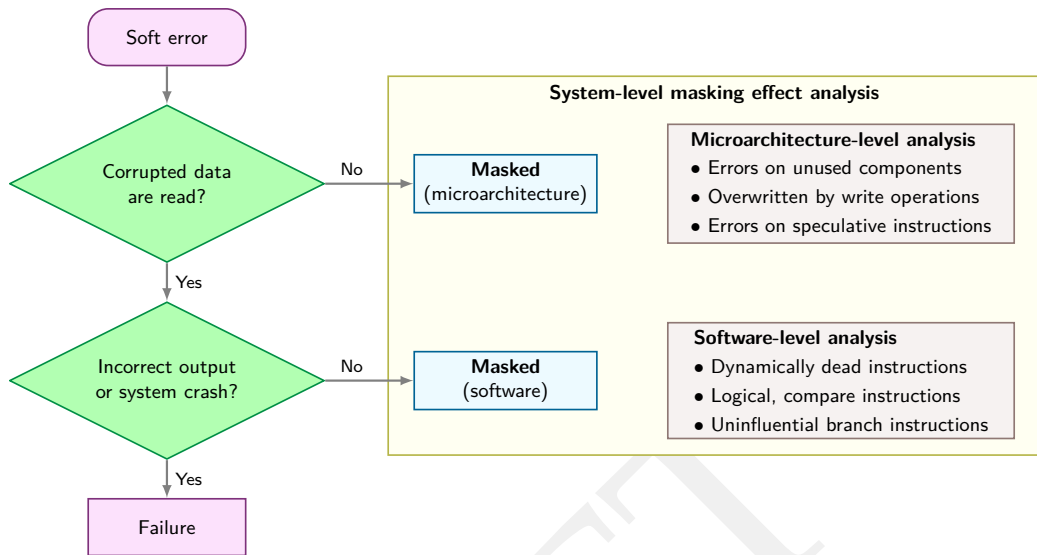
Figure 7.23: Error masking: Microarchitectural redundancy can absorb single-bit faults before they propagate to observable system errors, highlighting a discrepancy between hardware-level and software-level fault models. This figure details how fault masking occurs within microarchitectural components, demonstrating that software-based error detection tools may underestimate the true resilience of a system to transient errors.
