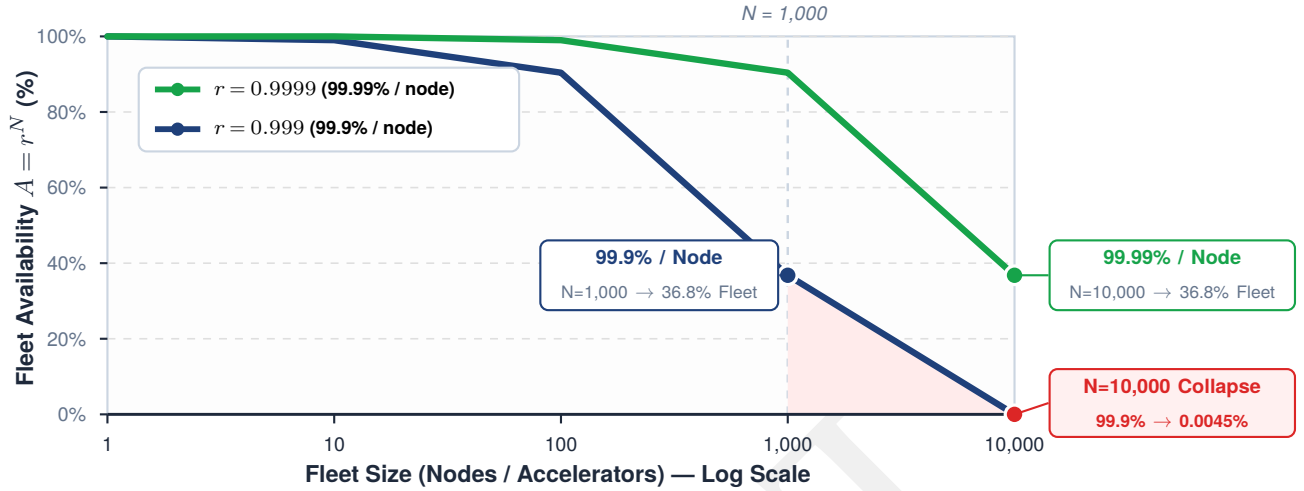
Figure 1.12: The reliability collapse: The simultaneous availability of every node required by an unreplicated job, shown as a function of job size for two per-node availability levels under an independence assumption. At 99.9% per-node availability (blue), all-node availability is only 36.8% for a 1,000-GPU job and approaches zero for a 10,000-GPU job. Even 99.99% per-node availability (green) yields 36.8% at 10,000-GPU scale.
