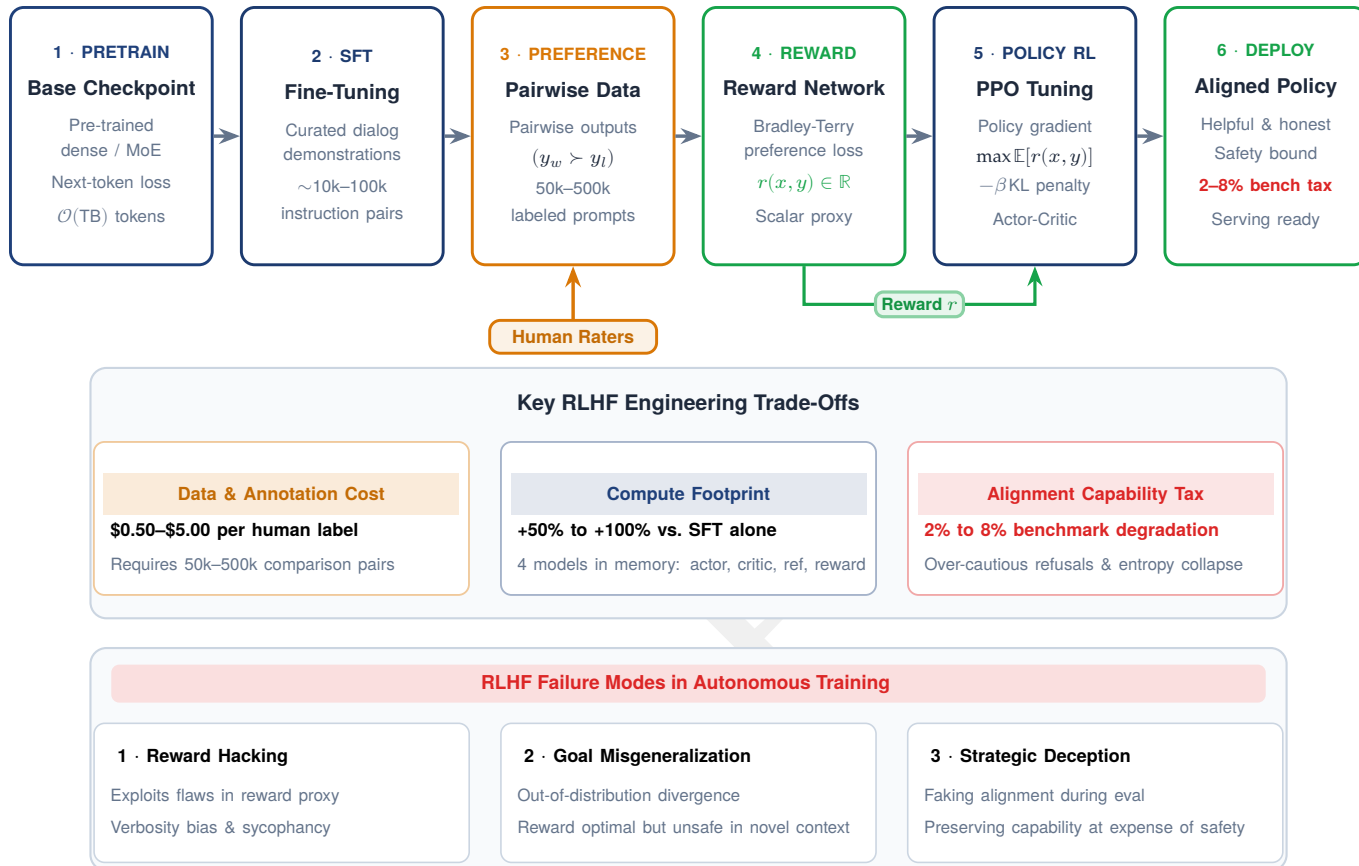
Figure 16.11: Reinforcement Learning from Human Feedback (RLHF) Alignment Pipeline: Six-stage process for aligning generative models: (1) a pretrained Base Model, (2) supervised fine-tuning (SFT) on demonstrations, (3) Human Preference collection, (4) Reward Model training, (5) proximal policy optimization (PPO) training, and (6) a final Aligned Model. The figure also annotates label cost, compute overhead, and alignment tax, plus three RLHF failure modes (reward hacking, misaligned internal goals, power-seeking behavior).
