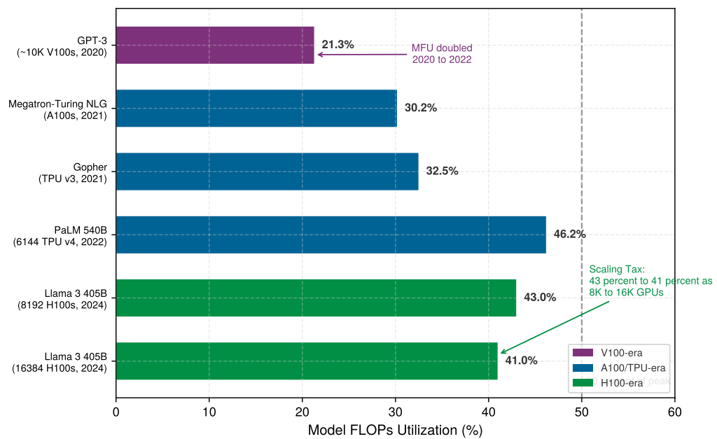
Figure 5.18: The MFU progression: Model FLOPs Utilization across published training systems, ordered chronologically. MFU doubled from 21 percent (GPT-3, 2020) to 46 percent (PaLM, 2022) through advances in hybrid parallelism and communication overlap, then plateaued near 40–45 percent for large-scale runs. The Llama 3 data points illustrate the scaling tax: MFU drops from 43 percent at 8,192 GPUs to 41 percent at 16,384 GPUs as communication overhead grows with cluster size. Data sources: Chowdhery et al. (2022), Dubey et al. (2024).
