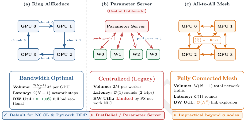
Figure 5.5: Gradient synchronization topologies: The panels compare three communication patterns. (a) Ring AllReduce distributes bandwidth evenly across links but has linear latency scaling. (b) A parameter server centralizes traffic and creates a server bottleneck. (c) An All-to-All mesh completes an exchange in one communication round, but its link count grows quadratically, making the topology impractical beyond small groups.
