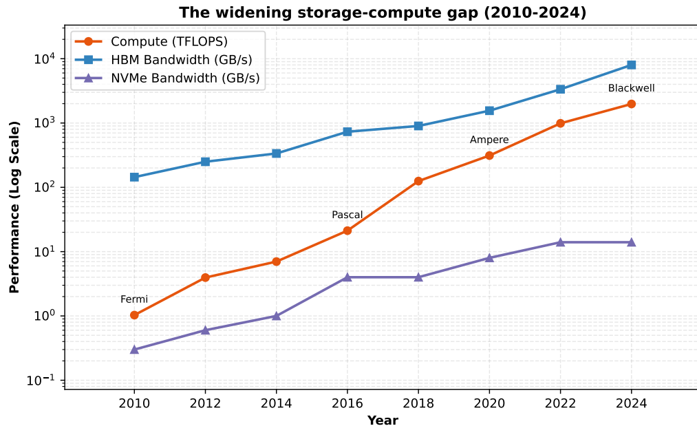
Figure 4.1: The storage-compute gap: Accelerator compute, HBM bandwidth, and NVMe bandwidth from 2010 to 2024 on a common log scale. Compute rises fastest and local storage slowest, so the fuel line into the accelerator becomes the binding constraint long before arithmetic does.
