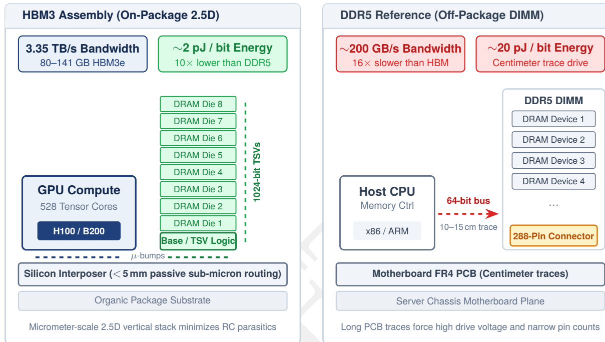
Figure 2.8: HBM 3D-stacked architecture: High-bandwidth memory achieves its performance by vertically stacking DRAM dies and connecting them via through-silicon vias. The entire stack sits on a silicon interposer alongside the GPU die, enabling a 1024-bit-wide bus and reducing signal travel distance from centimeters to micrometers. This physical proximity is the key to breaking the memory wall.
