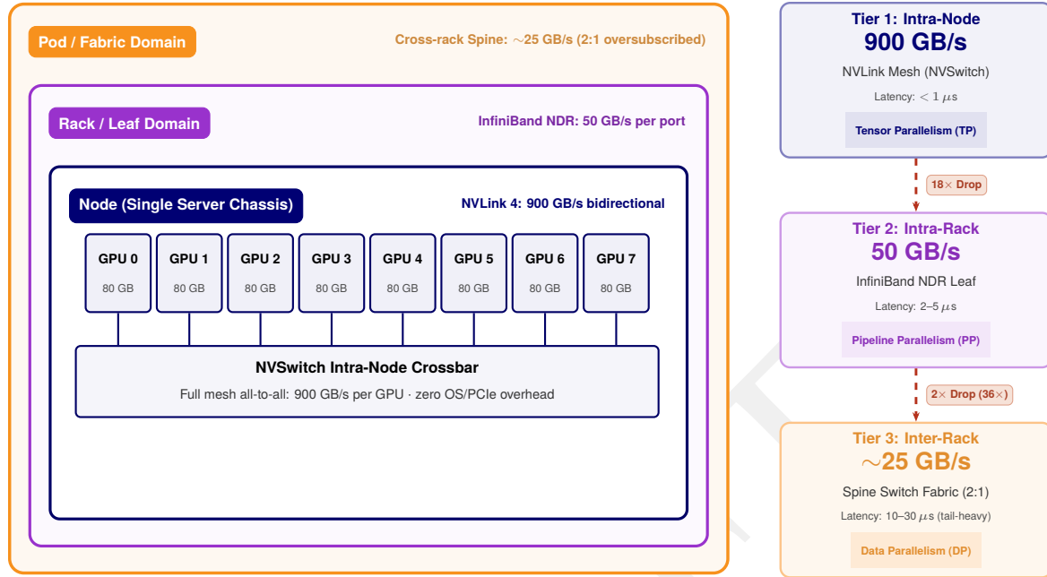
Figure 8.5: Physical topology hierarchy and bandwidth cliffs: Hardware boundaries dictate communication performance across three distinct domains. Within a node, NVLink provides 900 GB/s bidirectional bandwidth for tensor-parallel communication. Within a rack, InfiniBand/RoCE links deliver 50 GB/s for pipeline and data parallelism. Across racks and pods, spine switch fabrics drop effective bandwidth to 12–25 GB/s with 2:1 to 4:1 oversubscription.
