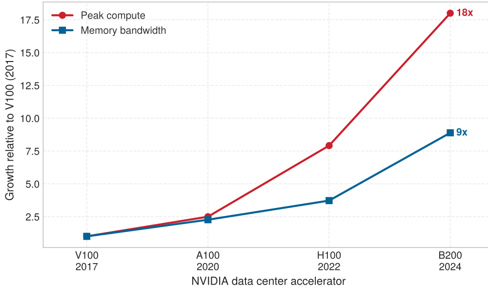
Figure 10.6: Decode inherits the bandwidth deficit: Peak compute and memory bandwidth for four accelerator generations, normalized to the V100. Compute rises 18× against bandwidth’s 8.9×, and because decode reads the full weight set once per token it advances at the lower of the two rates. Specifications come from the MLSysIM hardware registry.
