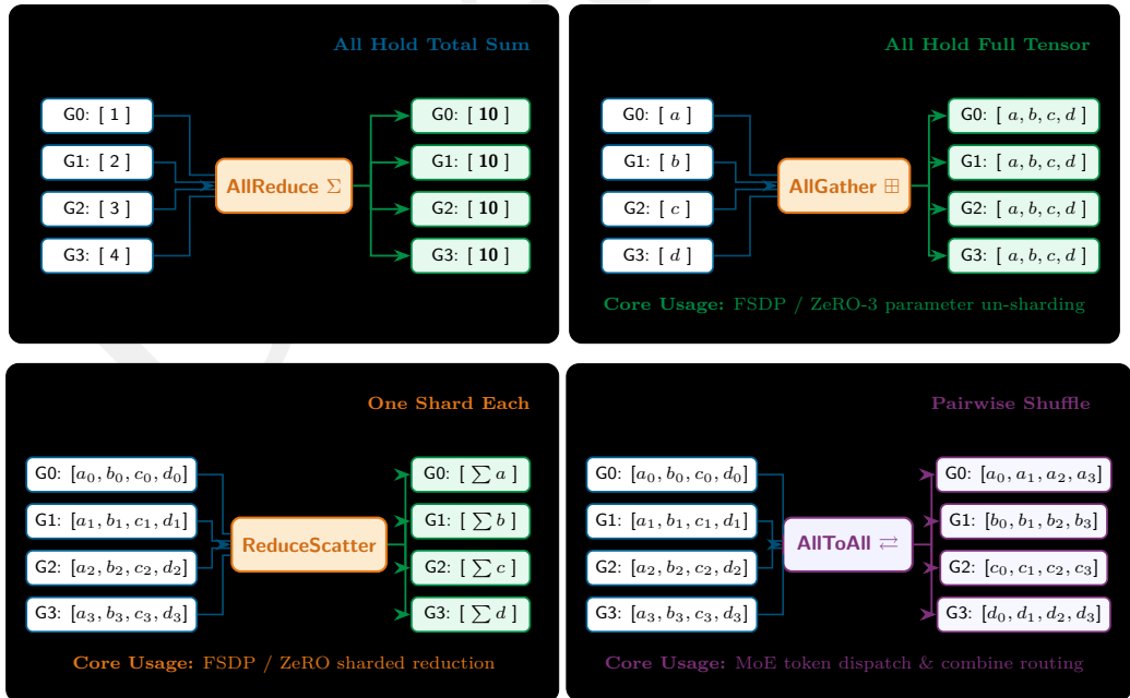
Figure 6.5: Four central collective primitives: Standardized patterns for group communication in distributed systems. (1) AllReduce: all aggregate and all receive the result. (2) AllGather: all send to all and concatenate. (3) ReduceScatter: all aggregate and results are distributed in shards. (4) AllToAll: every process sends unique data to every other process. The two foundational primitives Broadcast (rank 0 sends to all) and Reduce (all aggregate to rank 0) compose the patterns shown here and are defined in the surrounding prose.
