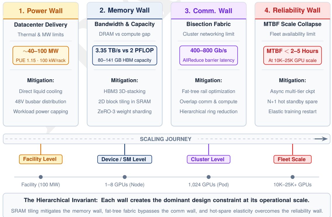
Figure 2.1: The four infrastructure walls: Four dominant constraints arranged across a scaling journey: power wall (data center delivery limits, ~40 MW facility), memory wall (HBM bandwidth gap, 3.35 TB/s HBM3 vs. ~2K TFLOP/s), communication wall (network bisection limit, 400 Gb/s NDR IB per port), and reliability wall (MTBF ~2 hours at 25K GPUs). Each wall becomes the dominant constraint at a different scale, from a single GPU through 8-GPU nodes and 1K-GPU clusters to 25K+ GPU fleets.
