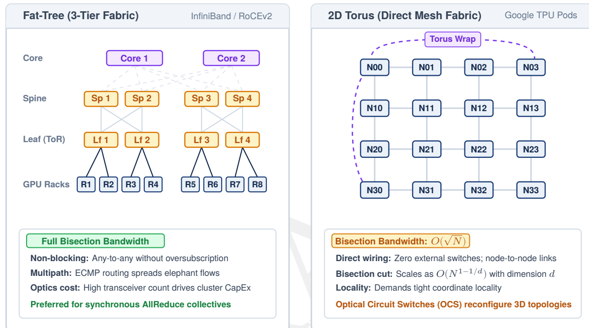
Figure 2.14: Pod-scale network topologies: Two dominant pod topologies compared. (Left) Fat-tree (3-tier) with leaf, spine, and core tiers: full bisection bandwidth, used by InfiniBand clusters such as DGX SuperPOD. (Right) 2D torus with wrap-around links: bisection bandwidth scales as O(\sqrt{N}) , cheaper at scale but rewards workloads with strong locality; used by Google TPU pods. The choice shapes which parallelism strategies run efficiently.
