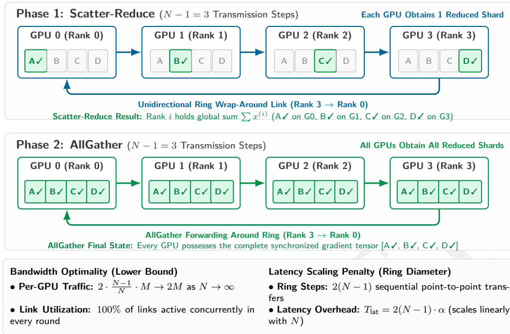
Figure 6.6: Ring AllReduce data flow: Nodes arranged in a logical ring exchange chunks in two phases: a Scatter-Reduce phase (each node accumulates one chunk's partial sum) followed by an AllGather phase (complete sums circulate to all nodes). The figure shows the ring laid out horizontally with a wrap-around bus closing the loop; every link is used simultaneously, achieving bandwidth optimality.
