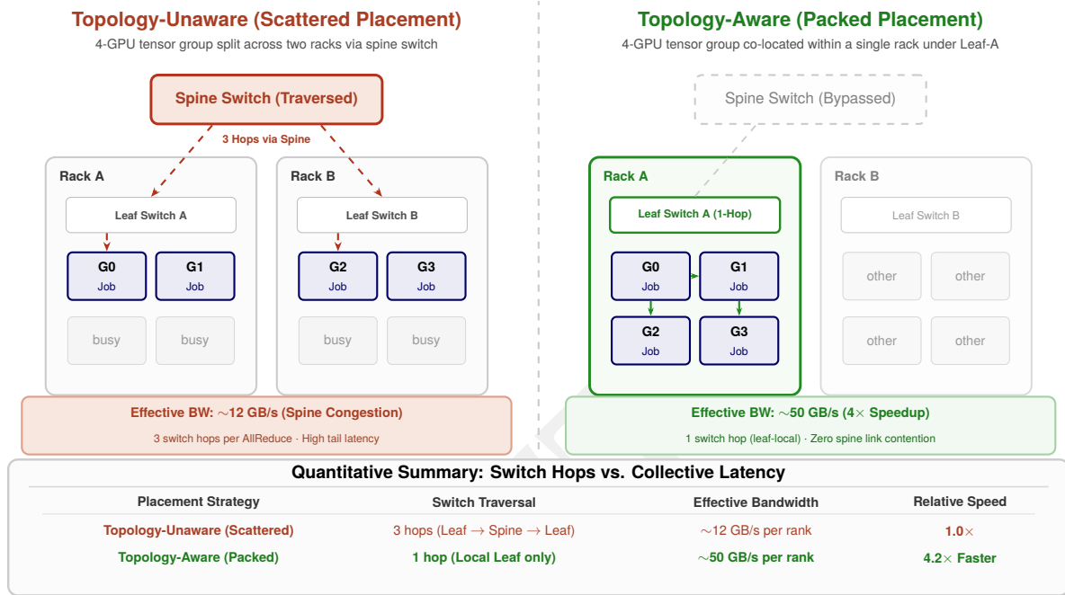
Figure 8.6: Topology-unaware vs. topology-aware placement: A 4-GPU job placed across two racks (left, topology-unaware) must traverse leaf-spine-leaf hops: 3 switch hops per AllReduce message at about 12 GB/s effective bandwidth. The same 4-GPU job packed within one rack (right, topology-aware) uses a single leaf switch: 1 hop at about 50 GB/s, roughly 4× faster. A quantitative summary beneath the figure reports switch-hop counts and effective bandwidth.
