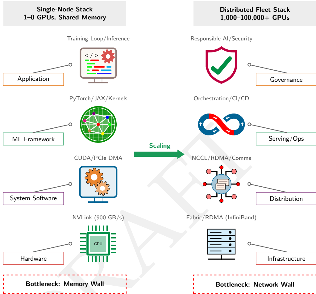
Figure 1.4: The scaling regimes of ML systems: Scaling extends a single-node stack into a distributed fleet stack. Local memory bandwidth often limits single-node workloads; bisection bandwidth can limit communication-intensive distributed workloads. Mastery of intra-node data movement remains a prerequisite for distributed scaling.
