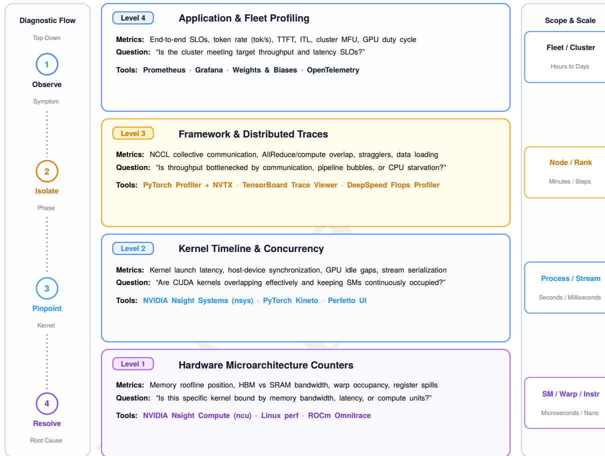
Figure 9.13: The profiling hierarchy: Diagnosis begins with application-level symptoms, then narrows through framework and kernel evidence to hardware counters. Each lower level trades breadth for the detail needed to isolate a root cause.
