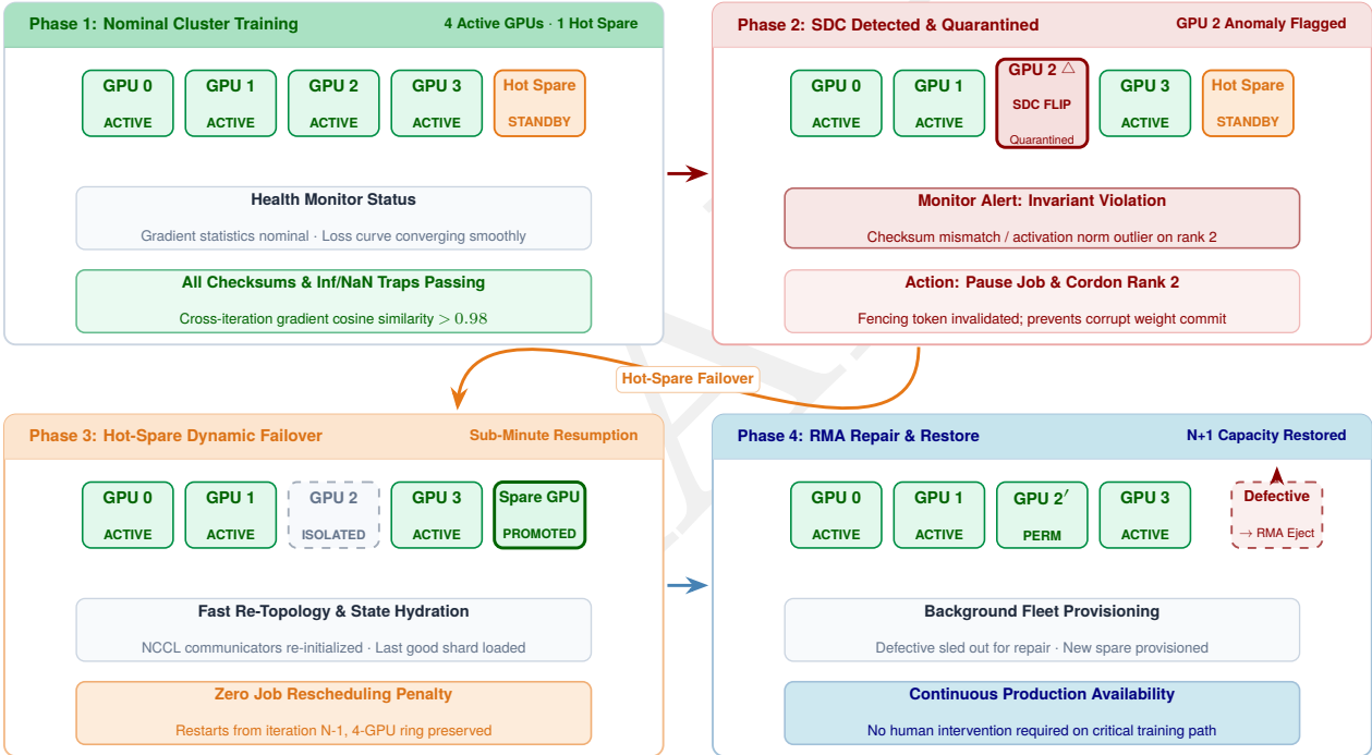
Figure 7.9: Hot-spare redundancy: Google’s data-center examples use spare capacity and sanity checking to keep ML training moving despite hardware faults, transitioning work away from suspect resources when monitors flag anomalies. This approach contrasts with parallel redundancy techniques such as dual modular redundancy and triple modular redundancy by providing a reactive fault-tolerance mechanism. Source: (Dean 2024).
