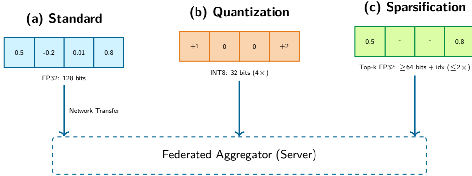
Figure 11.15: Gradient compression techniques: Standard updates transmit full-precision values; quantization maps values to lower-precision buckets, such as FP32 to INT8; and sparsification transmits only the most significant top- k gradients. The latter two mechanisms reduce bytes transferred but introduce representation error or residual state that the training algorithm must manage.
