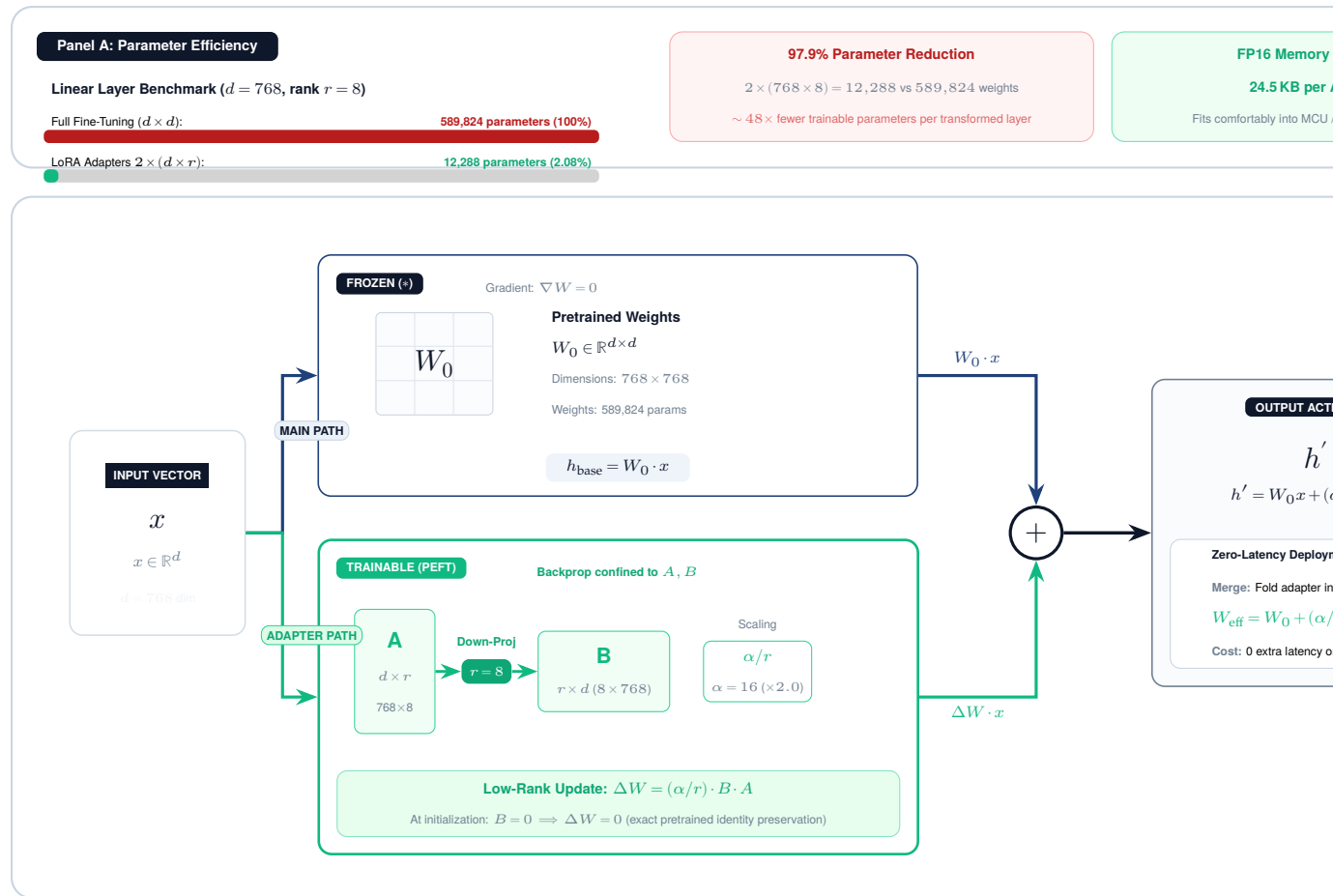
Figure 11.10: LoRA architecture and parameter efficiency: The input x passes through both the frozen base weight matrix W_0 and the low-rank trainable adapter path consisting of down-projection A and up-projection B . At inference, the adapter weights can be folded directly into the base weights with zero additional latency.
