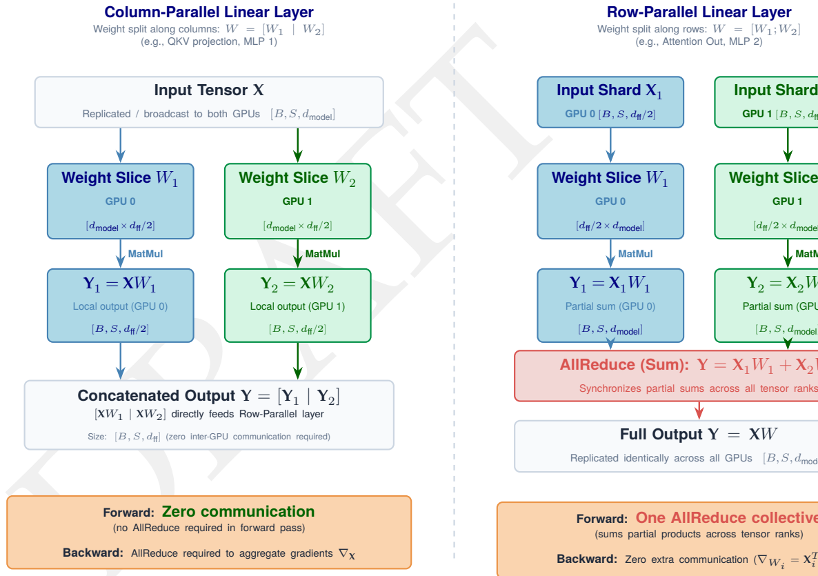
Figure 5.16: Matrix partitioning under tensor parallelism: The first linear layer (for example, QKV) is split column-wise as [W_1 \mid W_2] , and the second (for example, the output projection) is split row-wise as [W_1; W_2] . This Megatron-LM arrangement passes the intermediate result directly between the two splits and requires one AllReduce after the second layer to sum partial outputs.
