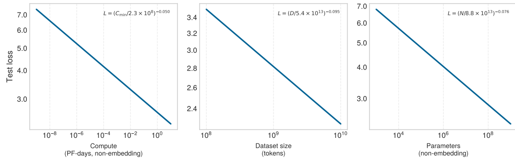
Figure 15.5: Model Scaling Laws: In the ranges studied by Kaplan et al. (2020), increasing model size, dataset size, and compute consistently reduced test loss. The figure reproduces source-paper notation, where N denotes parameter count and C_{\min} denotes compute; elsewhere this book uses P for parameter count and O for operation count. These scaling laws explain why larger models, more data, and increased compute became attractive design choices within that regime.
