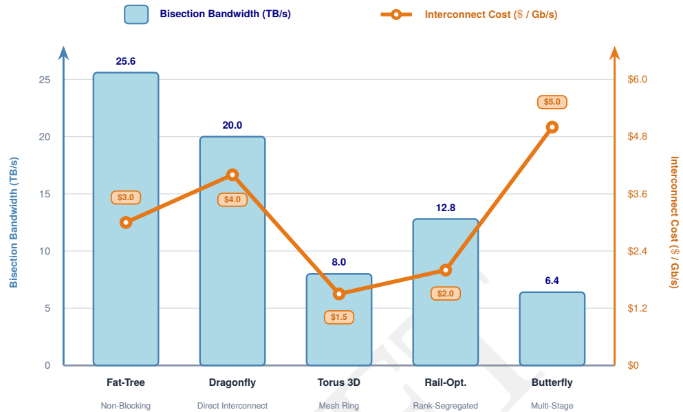
Topology Trade-Offs (1,024-GPU Training Cluster)
