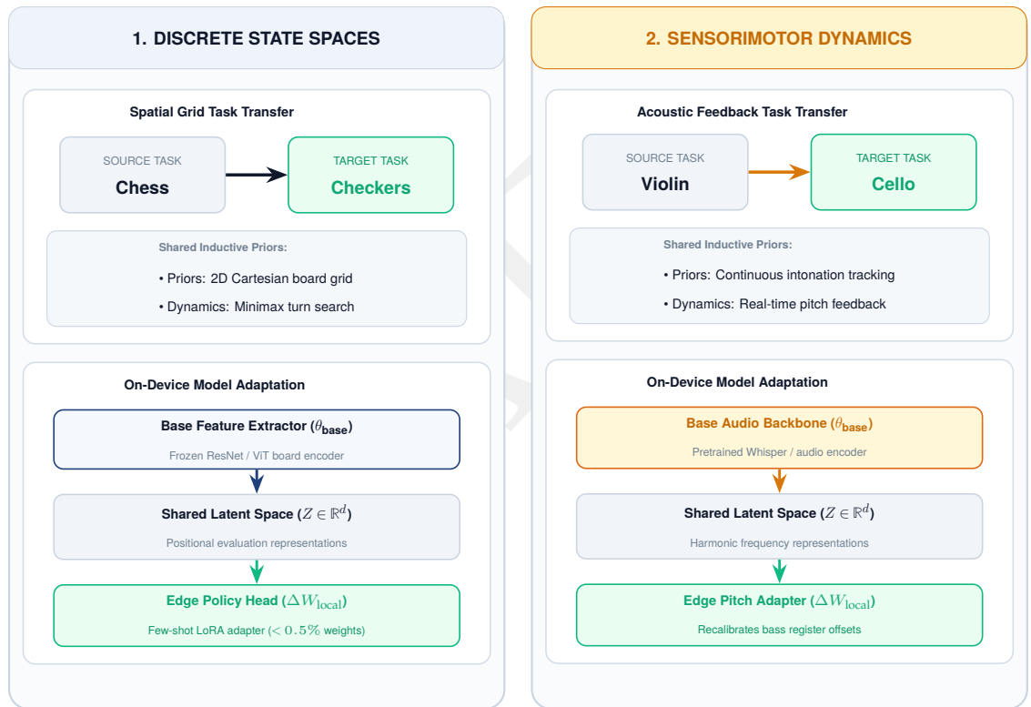
Figure 11.2: Knowledge transfer: Pretrained models accelerate learning on new tasks by using existing representations, as seen by adapting skills between related board games or musical instruments. This transfer extends across domains like bicycle riding and scooter operation, where shared underlying structures allow efficient adaptation with limited new data.
