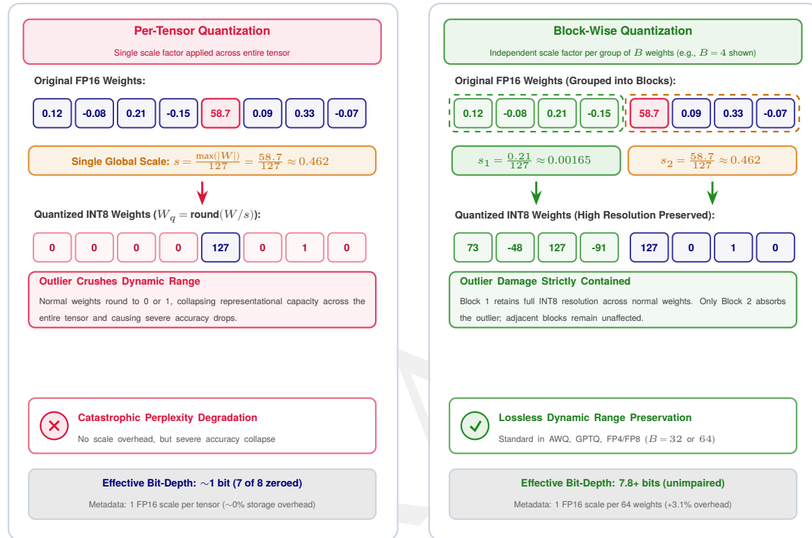
Figure 9.9: Block-wise versus per-tensor quantization: Under per-tensor scaling (left), an extreme outlier weight forces a wide scale factor that crushes normal weights to zero and destroys precision. Under block-wise quantization (right), weights are partitioned into independent groups, strictly isolating outlier damage to a single block and preserving full INT8 dynamic range across remaining parameters.
