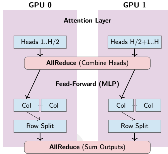
Figure 10.13: Tensor parallelism for inference: Computation is distributed across devices by splitting tensor operations. Attention heads are partitioned across GPUs, requiring an AllReduce operation to synchronize results. Feed-forward networks use a column-row splitting strategy that requires only one AllReduce synchronization per block. This approach reduces latency for large models but introduces communication overhead that demands high-bandwidth interconnects like NVLink.
