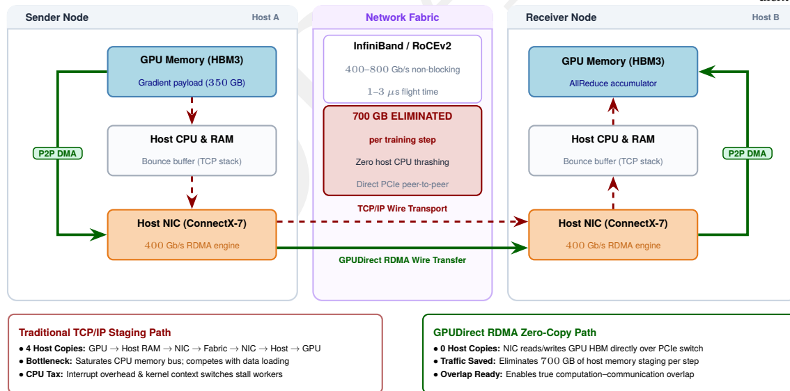
Figure 3.6: GPUDirect RDMA data path: The red traditional path stages an accelerator payload in registered host memory before the NIC reads it. The green GPUDirect path lets the NIC access GPU memory over PCIe, eliminating the host-memory bounce.
