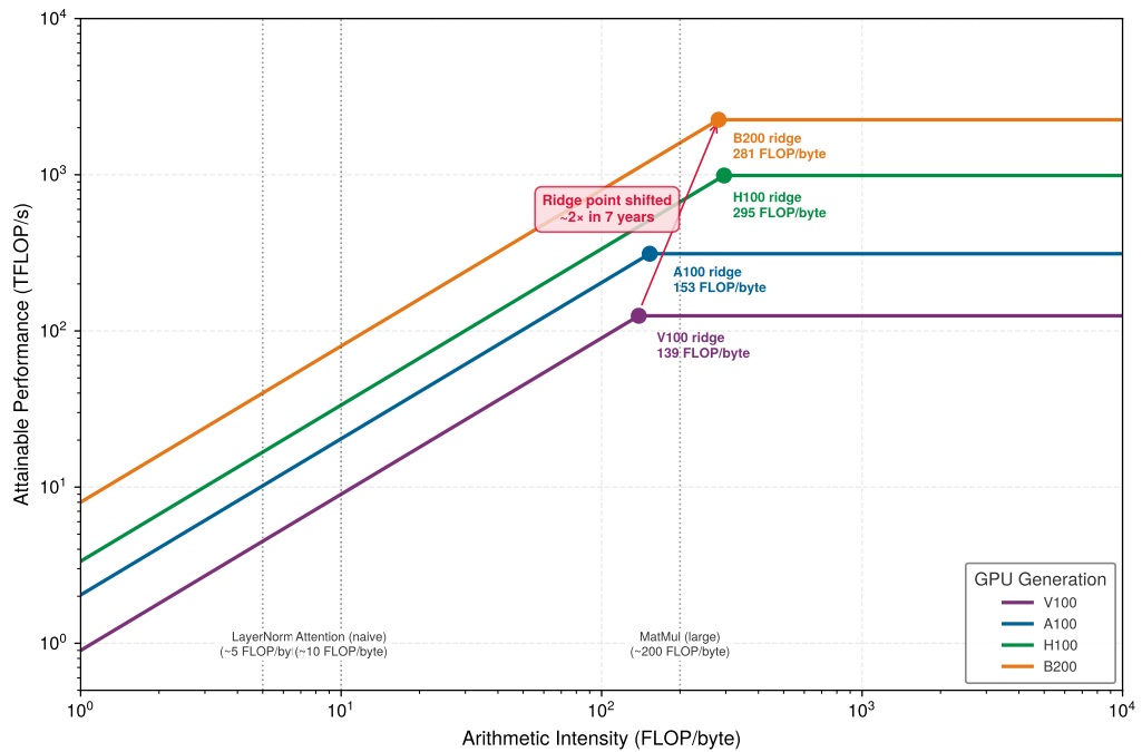
Figure 9.4: The shifting roofline across GPU generations: Overlaid FP16/BF16 roofline models for V100 through B200 show the ridge point growing from 139 to 281 FLOP/byte. Operations near 200 FLOP/byte can change regime as the roofline shifts. The same kernel can change performance regime across hardware generations.
