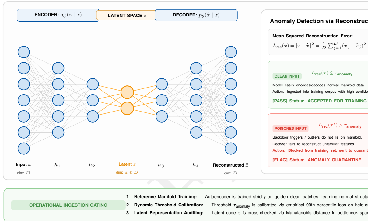
Figure 14.21: Autoencoder Architecture: Autoencoders learn compressed data representations by minimizing reconstruction error, enabling anomaly detection by identifying inputs with high reconstruction loss. During training on normal data, the network learns efficient encoding and decoding, making it sensitive to deviations indicative of potential poisoning attacks. Source: adapted from a Towards Data Science autoencoder tutorial.
