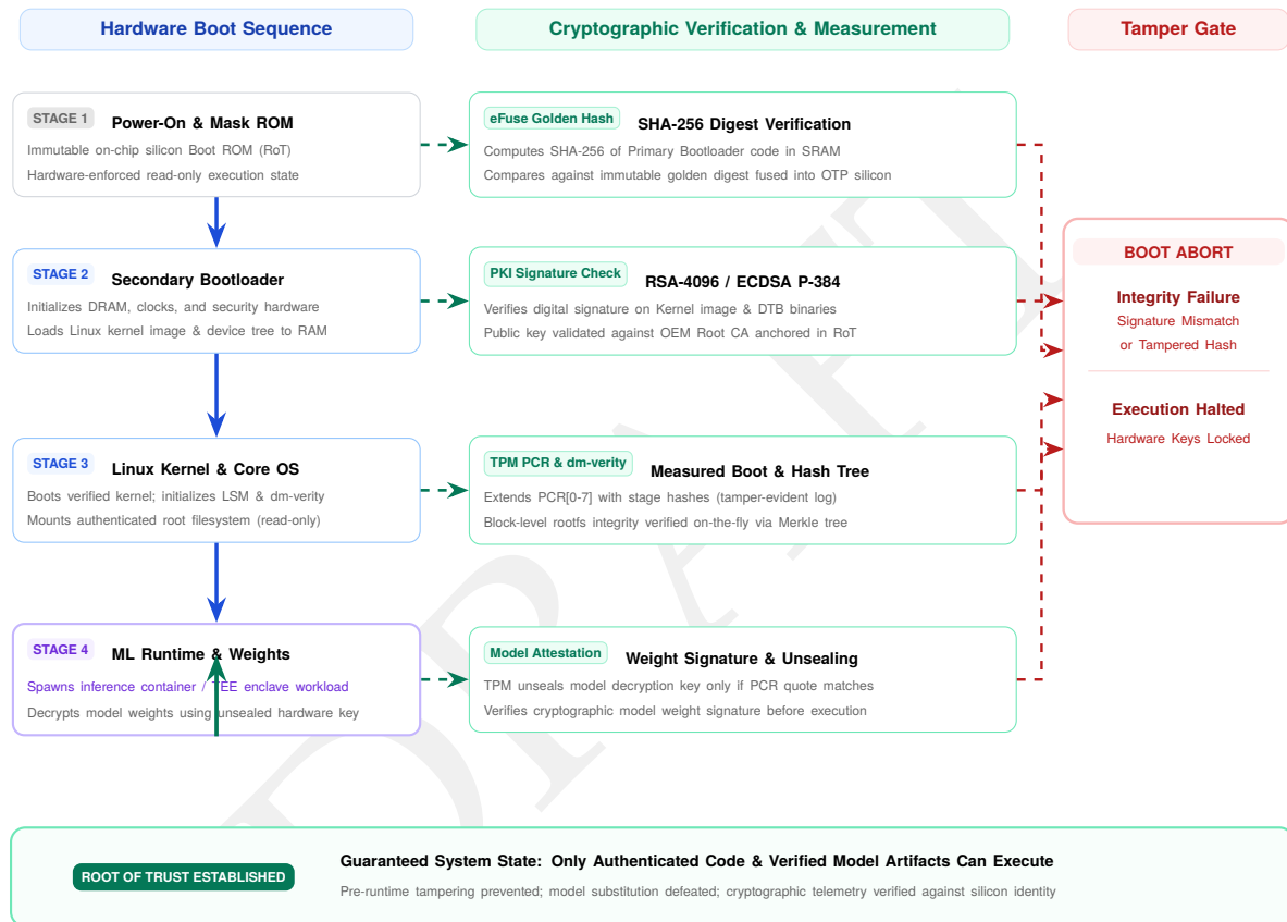
Figure 13.23: Secure boot sequence: Embedded systems employ a layered boot process to verify firmware and software integrity, establishing a root of trust before executing machine learning workloads and protecting against preruntime attacks. This architecture ensures only authenticated code runs, safeguarding model data and preventing unauthorized model substitution or modification during deployment.
