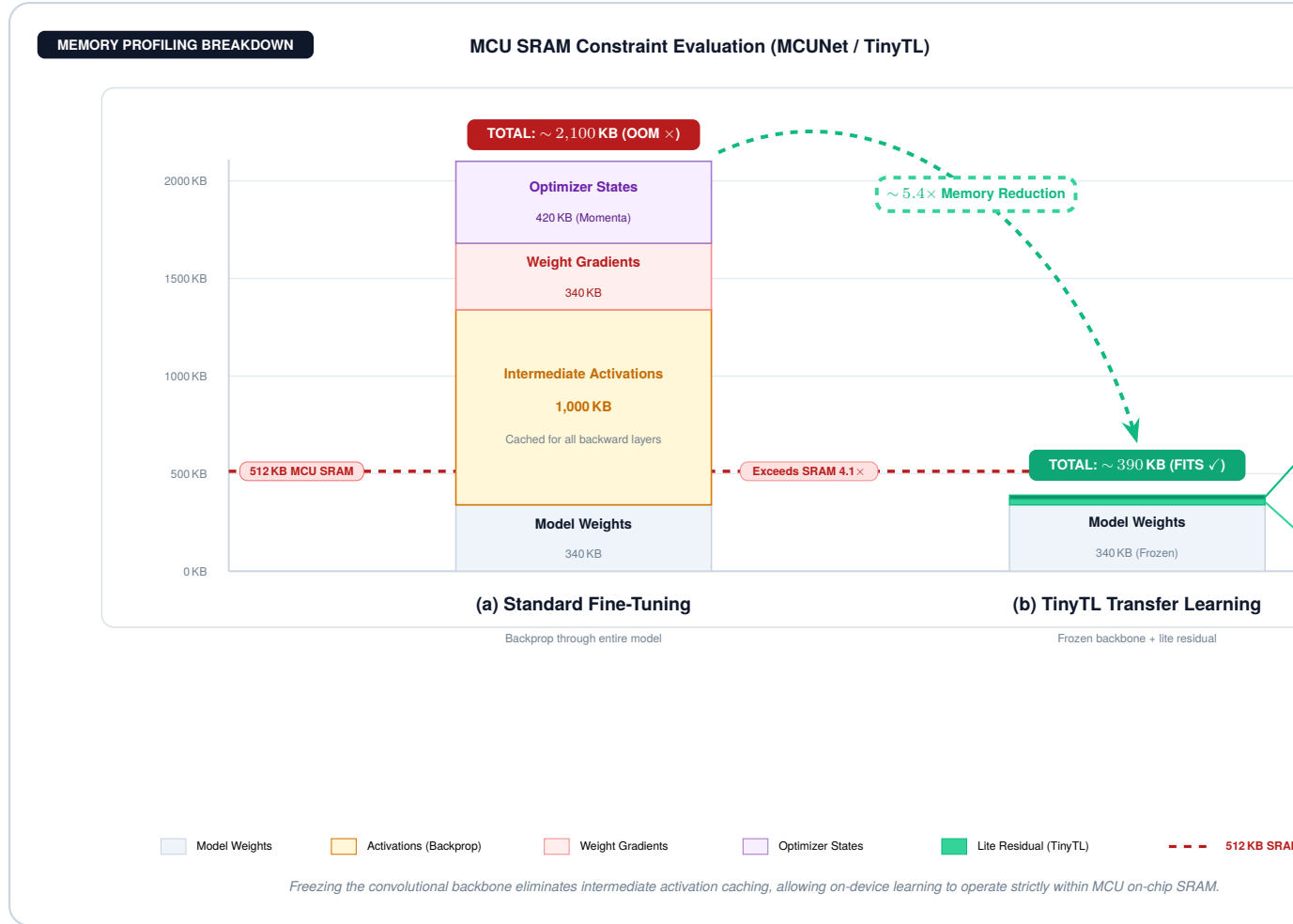
Figure 11.9: TinyTL memory breakdown: Comparison of training memory breakdown between standard fine-tuning and TinyTL on microcontroller hardware. Standard backpropagation requires storing intermediate activations that exceed the 512 KB SRAM ceiling, whereas TinyTL operates comfortably within SRAM by eliminating backbone activation caching.
