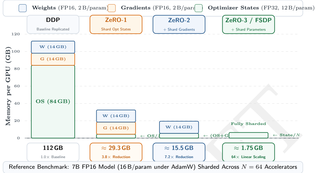
Figure 5.7: ZeRO memory reduction: Standard data parallelism (DDP) replicates all model states across every GPU. ZeRO progressively partitions these states: ZeRO-1 shards optimizer states, ZeRO-2 adds gradient sharding, and ZeRO-3 shards the parameters themselves. ZeRO-3 achieves linear memory scaling, enabling models with 100B+ parameters to fit on accelerators that could not hold the replicated state.
