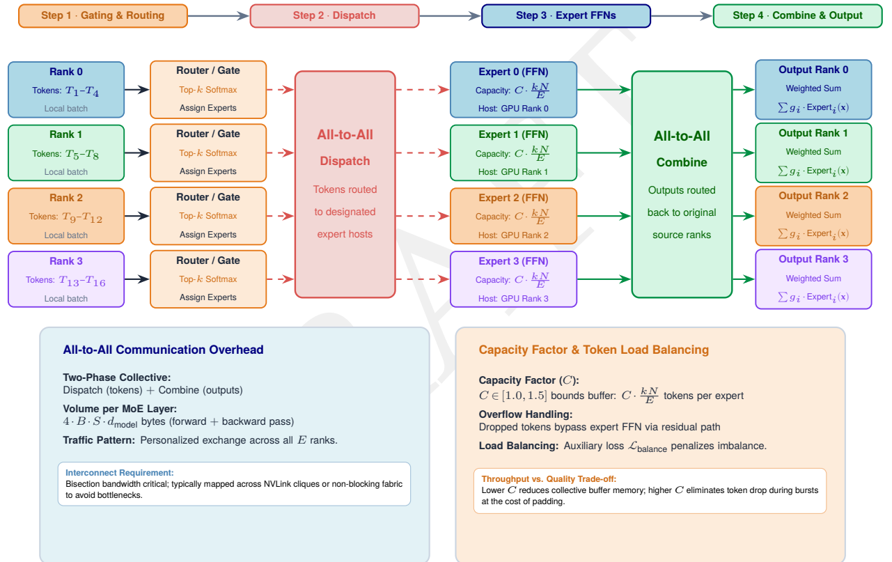
Figure 5.17: Mixture-of-experts (MoE) AllToAll routing: Expert parallelism requires a unique “All-to-All” communication pattern. Tokens from a local batch are routed by a gating network to experts sharded across the cluster. This involves a global shuffle where every GPU sends tokens to and receives tokens from potentially every other GPU, stressing the cluster’s bisection bandwidth.
