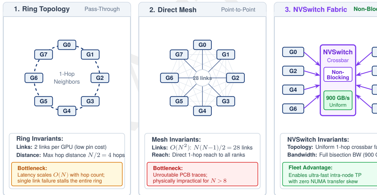
Figure 2.12: Intra-node GPU topology comparison: Three approaches to wiring GPUs inside a node. (Left) Ring: sequential pass-through, ~50 GB/s per link, latency scales with distance. (Center) Full mesh: all-to-all direct links, N-1 links per GPU, impractical beyond ~8 GPUs. (Right) NVSwitch crossbar: non-blocking fabric with 112 GB/s per NVLink and 900 GB/s aggregate, any-GPU-to-any-GPU in one hop, enabling tensor-parallel AllReduce within a node.
