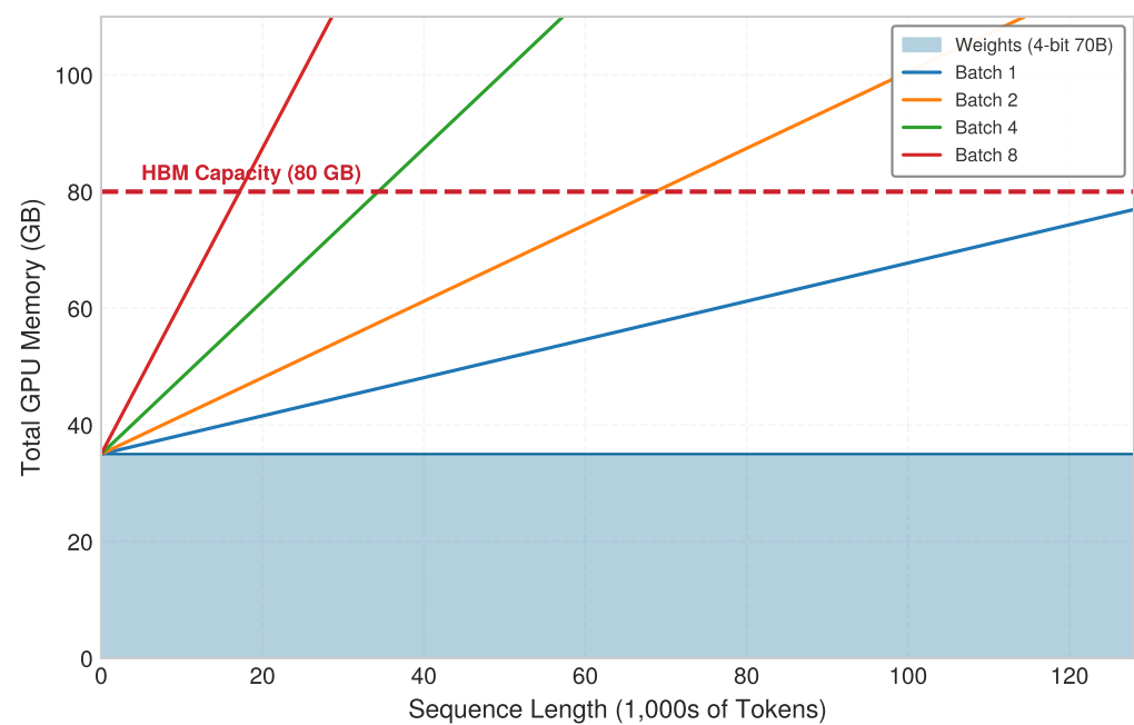
Figure 10.10: The KV cache wall: Total GPU memory usage for a 4-bit quantized 70B model (35 GB weights) on an 80 GB H100. While the model fits easily at small context lengths, the KV cache (sloped lines) eventually consumes all remaining HBM. At 128K context, a batch size of 2 is physically impossible on a single GPU (35 GB + 84 GB > 80 GB), forcing the system to either reduce batch size (killing throughput) or shard the model.
