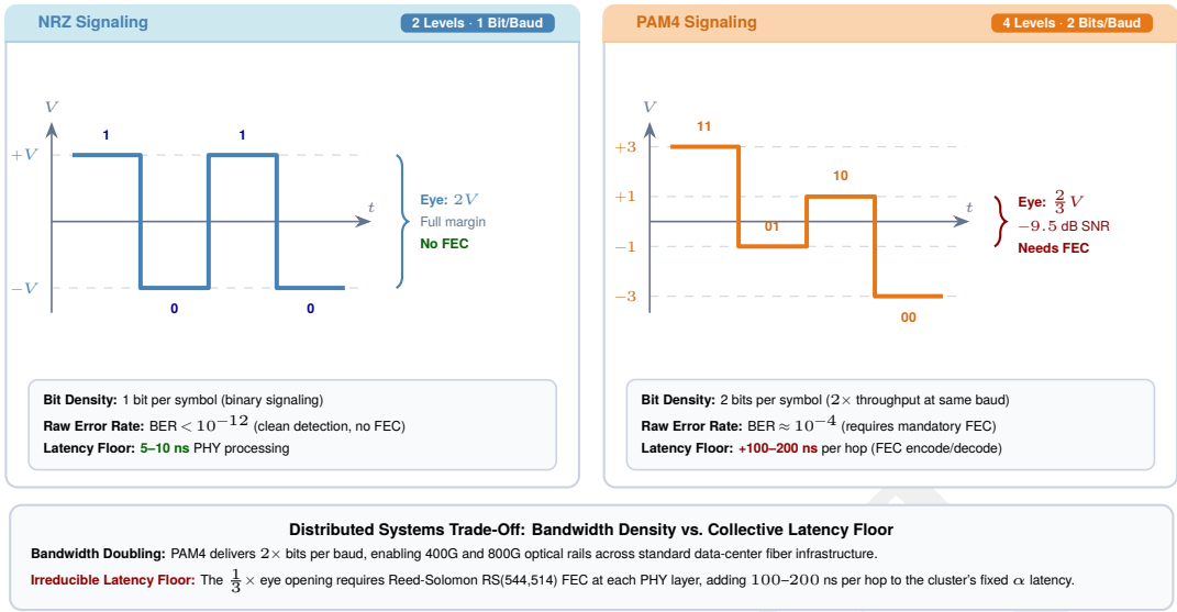
Figure 3.5: From NRZ to PAM4 signaling: To increase bandwidth without doubling clock frequency, high-speed interconnects moved from NRZ (2 voltage levels, 1 bit per symbol) to PAM4 (4 voltage levels, 2 bits per symbol). The trade-off is reduced noise margin: the ‘eye’ of the signal is smaller, necessitating forward error correction (FEC) and increasing the irreducible \alpha latency of the fabric.
