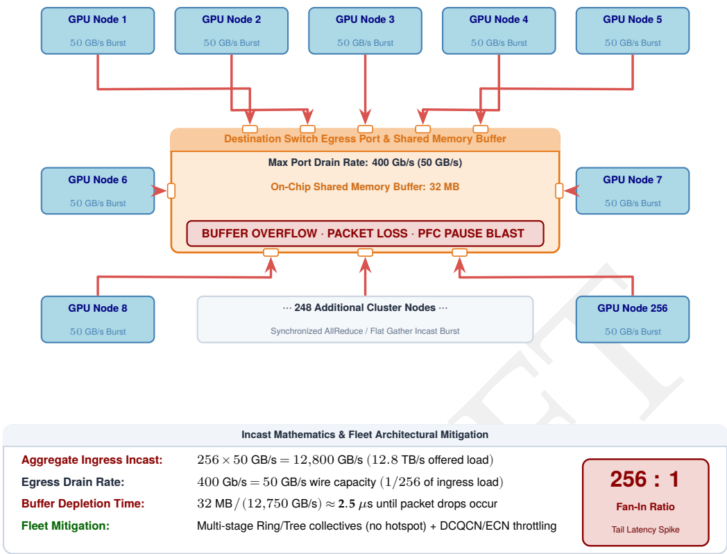
Figure 3.12: A true incast burst: This deliberately worst-case fan-in scenario sends 256 sources at 50 GB/s toward one 400 Gb/s (50 GB/s) egress with a 32 MB buffer. The 12.8 TB/s offered load oversubscribes the destination egress by 256×. Flat aggregation or synchronized reads can create this pattern; bandwidth-optimal ring AllReduce does not, because each rank exchanges point-to-point chunks.
