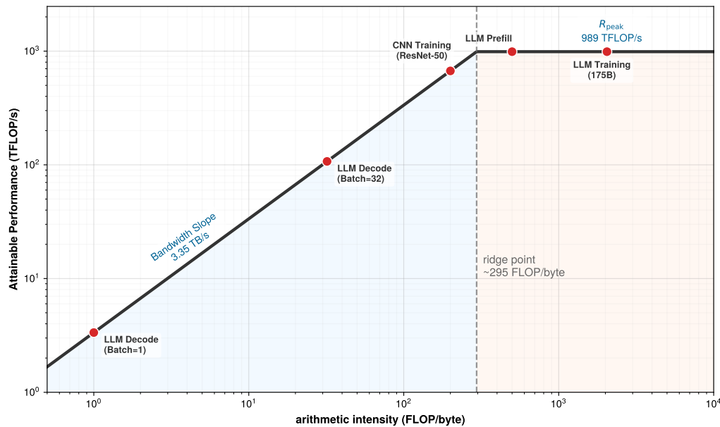
Figure 2.10: The H100 roofline landscape: The FP16 roofline for an NVIDIA H100 marks the memory-bandwidth and peak-compute ceilings, with representative ML workloads spanning memory-bound and compute-bound regions.
