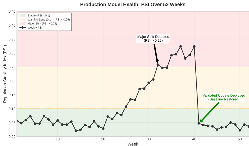
Figure 14.11: A Calibrated Distribution-Shift Workflow: In this synthetic service, PSI enters the warning zone as user behavior shifts and crosses the service’s escalation threshold at week 32. Root-cause analysis, offline validation, and a model release precede the restored baseline at week 41.
