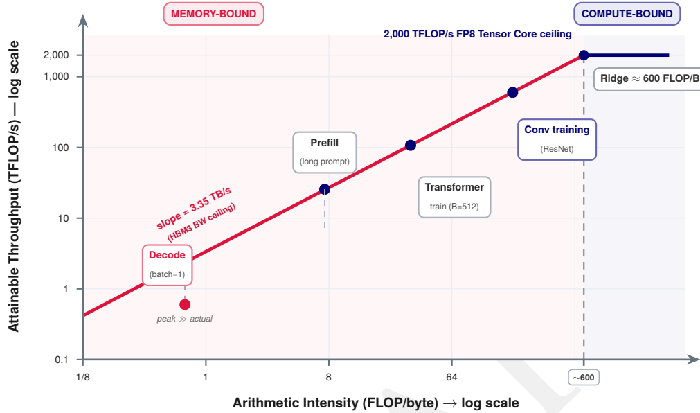
Figure 9.3: The roofline model: Achievable performance (y-axis) as a function of arithmetic intensity (x-axis) on a log-log plot. The sloped line represents the memory bandwidth ceiling; the flat line represents the compute ceiling at the labeled precision (FP8 tensor-core throughput on H100, approximately 1979 TFLOP/s); their intersection is the ridge point at roughly 590.7 FLOP/byte for FP8. Most transformer inference operations fall in the memory-bound region (left of the ridge point), while large batched GEMMs fall in the compute-bound region (right). The corresponding FP16 ridge point is roughly 295 FLOP/byte (989 TFLOP/s divided by 3.35 TB/s).
