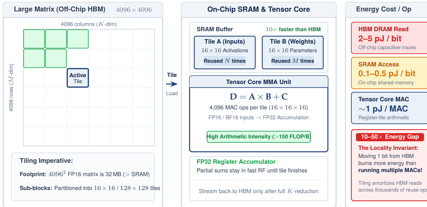
Figure 2.7: Tensor Core tiling strategy: To overcome the HBM bandwidth bottleneck, GPUs decompose large matrix operations into small tiles that fit within the streaming multiprocessor’s (SM) fast SRAM. Data is loaded once into SRAM and reused across multiple Tensor Core operations, effectively multiplying the arithmetic value of every byte fetched from HBM.
