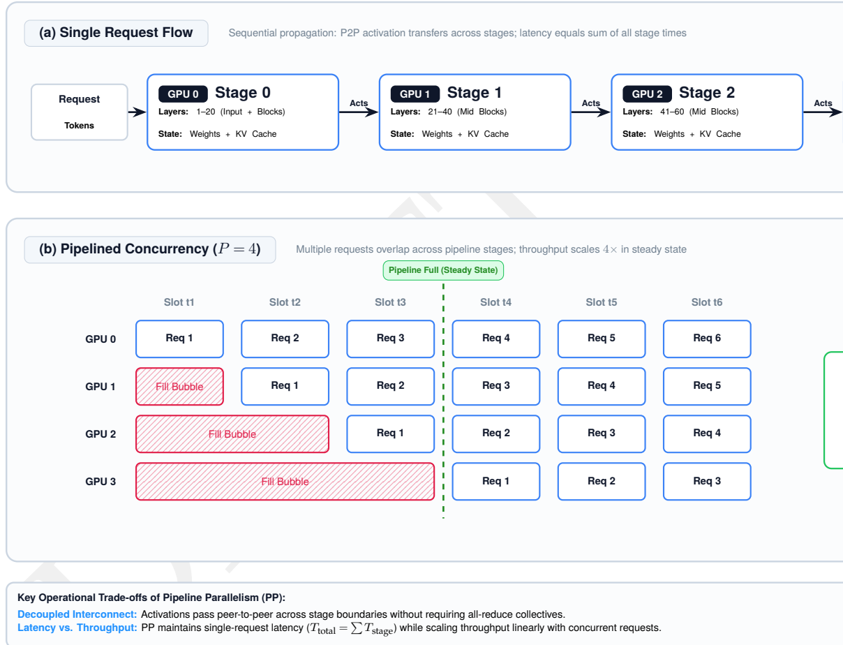
Figure 10.14: Pipeline parallelism bubbles: For a single inference request (top), pipeline parallelism offers no latency benefit as the request must traverse all four stages sequentially. When processing multiple concurrent requests (bottom), the pipeline fills and throughput scales with the number of stages. This makes pipeline parallelism ideal for high-throughput batch processing but less suitable for latency-critical interactive serving.
