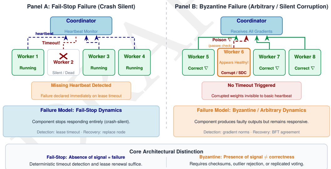
Figure 7.10: Fail-stop vs. Byzantine failures: In the fail-stop model (left), a failed worker simply ceases to send messages, which is easily detected by timeouts. In the Byzantine model (right), a failed worker continues to participate but sends incorrect data (for example, corrupted gradients reported as valid), which can poison the global model state if not detected by redundant validation.
