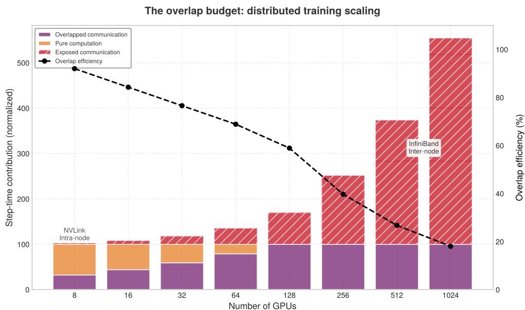
Figure 9.12: The overlap budget: This illustrative normalized scenario holds the computation budget at 100 units as GPU count increases from 8 to 1,024. Communication overhead grows with scale, leaving more communication exposed above the fixed compute budget. The black line reports the fraction of communication hidden behind computation, which falls from roughly 90 percent to roughly 18 percent.
