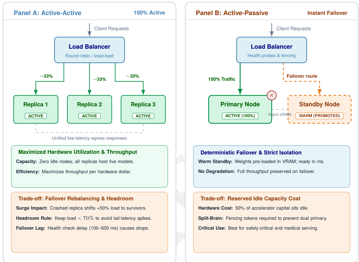
Figure 7.29: Serving redundancy strategies: Comparison of active-active vs. active-passive replication. Active-active (left) distributes load across three active replicas, each receiving roughly one-third of traffic, maximizing utilization but requiring capacity headroom to absorb failures. Active-passive (right) keeps standby replicas idle and synchronized via heartbeat, simplifying failover logic at the cost of idle resource utilization.
