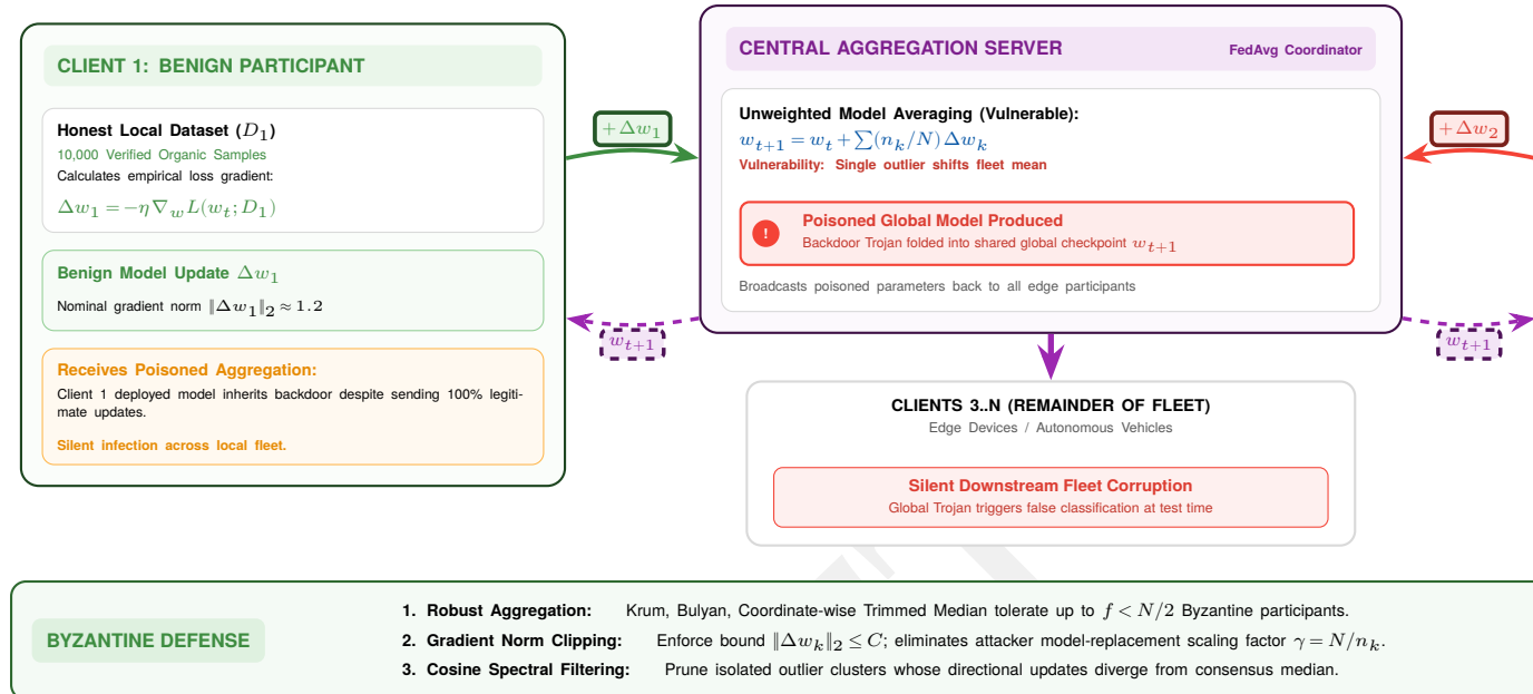
Figure 14.18: Collaborative Poisoning via Aggregation: In a collaborative learning setting, multiple clients each train on local data and contribute model updates to a central server that aggregates them into a shared global model. A single malicious participant can inject poisoned updates that the server folds into the aggregated model, so the corruption spreads to every client without any one obvious anomaly. This attack surface differs from adversarial examples because it targets the model during training rather than at inference .
