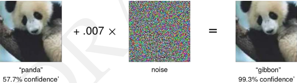
Figure 14.14: GoogLeNet Imperceptible Misclassification: Subtle, intentionally crafted noise added to an image causes a trained deep neural network (GoogLeNet) to misclassify a panda as a gibbon, despite the perturbed image remaining visually indistinguishable to humans. This classic demonstration underscores neural network fragility and motivates adversarial training. Source: (Goodfellow et al. 2015).
