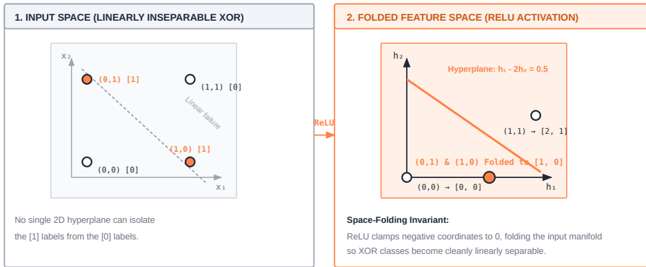
Figure 2.2: Space folding with ReLU: Linear layers in sequence collapse into a single affine transformation unable to partition linearly inseparable patterns such as XOR. An intervening elementwise \text{ReLU}(z) = \max(0, z) folds the negative quadrant onto the coordinate axes, bending the representation space so a downstream hyperplane can separate classes.
