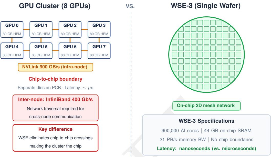
Figure 2.2: Wafer-scale engine (WSE) architecture: Unlike a cluster assembled from discrete packages and boards, a WSE uses most of a 300 mm wafer as one routed compute fabric. Defect-aware software routes around unusable regions, while the on-wafer mesh and distributed SRAM replace off-package transfers for mapped operations.
