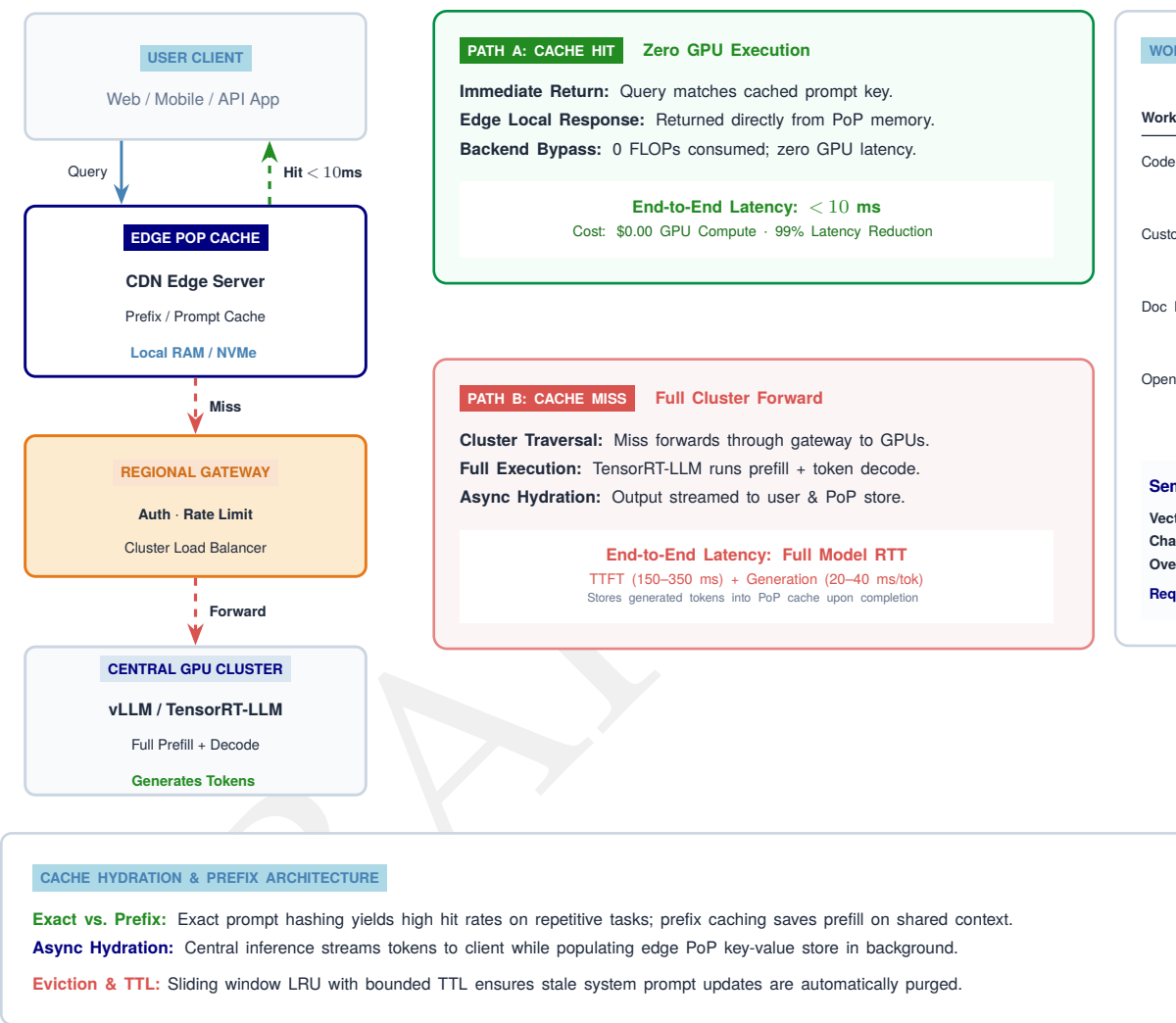
Figure 10.25: Cache hit and cache miss paths at the edge: A cache hit returns immediately from the CDN edge node ( <10\text{ ms} ). A cache miss flows through to central inference and populates the cache on return. Hit rate determines the effective cost saving; open-ended generative workloads have low repeatability and benefit little from this pattern.
