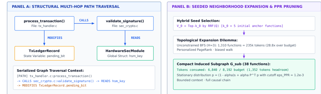
Figure 6.8: Code Property Graph Multi-Hop Traversal: Structural call-path traversal versus isolated text chunk retrieval. Panel A traces deterministic multi-hop edges across files (CALLS, READS, MODIFIES). Panel B demonstrates seeded neighborhood expansion with Personalized PageRank (PPR) pruning, preventing exponential context overflow while retaining intact causal dependency chains.
