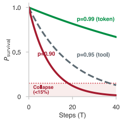
In unverified execution, compounding errors drive trajectory survival below 15 percent after 40 steps.
