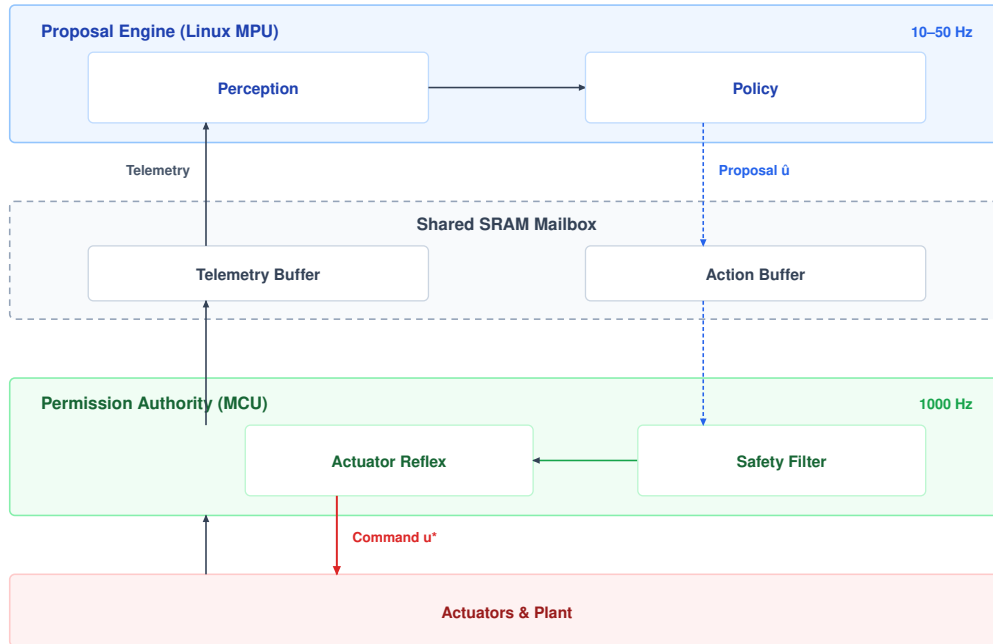
Figure 1.11: One dual-brain implementation: An application processor publishes learned proposals to a shared mailbox. An independently scheduled microcontroller checks freshness and physical limits before commanding motor current, and executes a defined fallback on stale or unsafe proposals. The indicated rates and mailbox are design examples whose suitability depends on the plant’s measured response budget.
