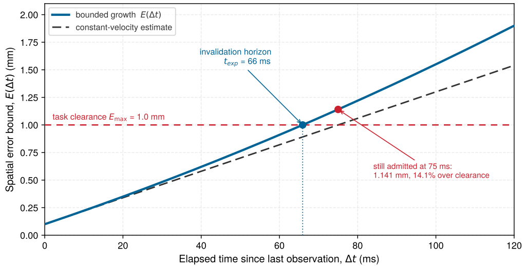
Figure 9.8: Belief uncertainty and invalidation horizon: Spatial error bound E(\Delta t) expanding quadratically under unobserved forward propagation until intersecting task clearance E_{\max} = 1.0 mm at invalidation horizon t_{\text{exp}} = 66 ms. A lower lifecycle timeline marks transitions from valid through degraded to expired operational regimes. Belief has a shelf life governed by physical disturbance dynamics; sensor re-acquisition resets the evidence clock, whereas republishing cached matrices conceals physical drift.
