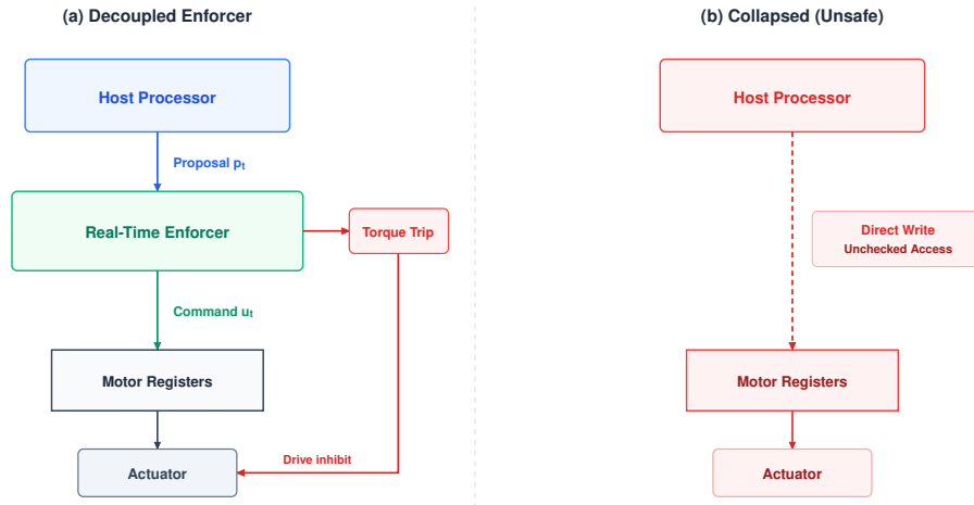
Figure 4.6: Hardware privilege boundary: (a) Decoupled safety enforcer isolating the real-time microcontroller with exclusive write privilege over motor drive registers while the host processor proposes trajectories across a shared-memory link. (b) Collapsed unsafe architecture where unverified host software writes actuator registers directly, creating a single failure domain.
