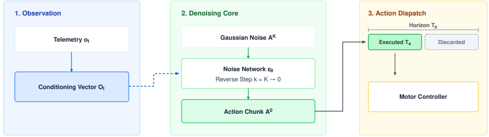
Figure 6.3: Diffusion policy architecture: A continuous trajectory diffusion policy for visuomotor control, denoising a candidate action chunk from Gaussian noise across K iterations and dispatching only a prefix of it before re-planning. Asynchronous buffering and an independent high-rate permission path can separate slower chunk generation from actuation. Conditional denoising can represent alternative demonstrated paths without taking their direct-regression mean. (Adapted from Chi et al. (Chi et al. 2024)).
