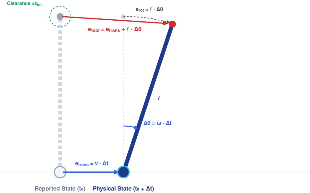
Figure 9.3: Transform staleness and lever-arm error propagation: Geometric error propagation under uncompensated transform latency \Delta t . Base translation shifts the origin by e_{\text{trans}} = v \Delta t , while joint rotation across link length \ell swings the tool tip by e_{\text{rot}} \approx \ell \omega \Delta t , accumulating into total tool displacement e_{\text{tool}} \approx e_{\text{trans}} + \ell \Delta \theta that breaches clearance tolerance \pm \epsilon_{\text{tol}} .
