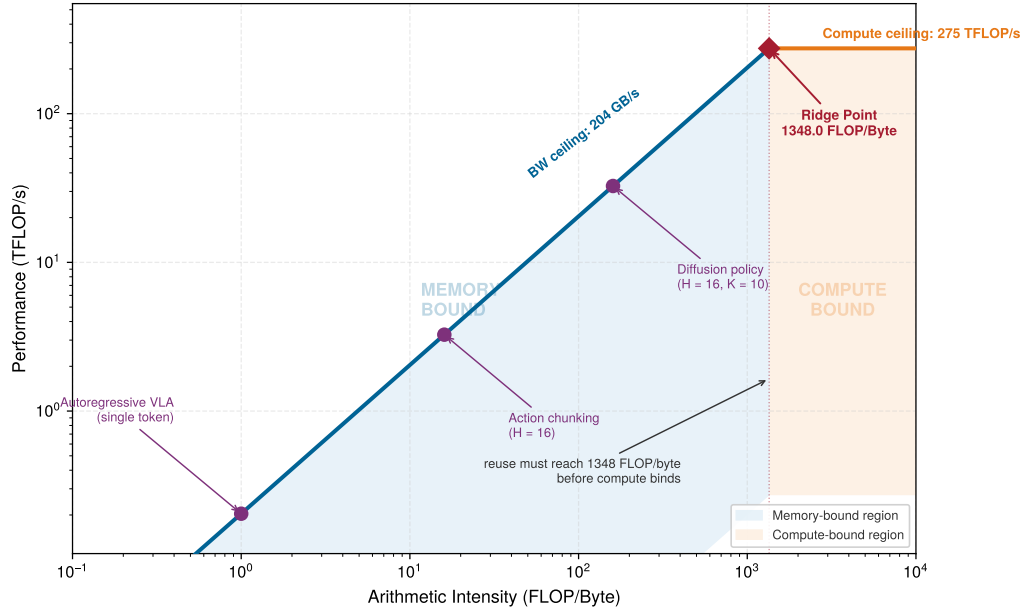
Figure 3.10: Illustrative embodied roofline: Arithmetic intensity against attainable throughput for an example edge accelerator. Single-token weight streaming can be memory-bound; reuse across a chunk may increase work per byte. The plotted positions illustrate possible workloads, not measured policy cadence. A separate real-time loop executes accepted waypoints between fresh model updates.
