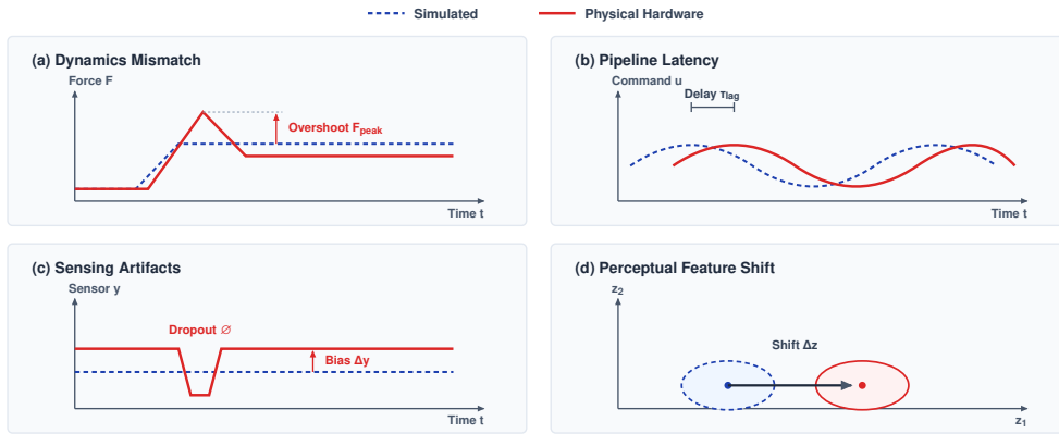
Figure 6.8: Sim-to-real reality gap vector: The sim-to-real gap decomposed across four physical channels, dynamics, latency, sensing, and perceptual feature shift, each measured from paired traces rather than from an aggregate loss. The decomposition is the point, because the four channels fail differently and a scalar loss averages them into a number that names none of them. A 5.5 percent pixel discrepancy that looks trivial masks a 6.0 mm spatial shift that exceeds the assembly tolerance.
