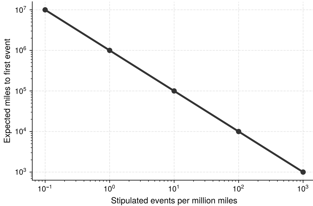
Figure 15.2: Illustrative rare-event exposure: For independent miles with a stipulated constant event rate r per million miles, expected distance to the first event is 10^6/r miles. The constructed points show why passive observation becomes costly as the target event becomes rarer; they are not measured fleet disengagement or crash data.
