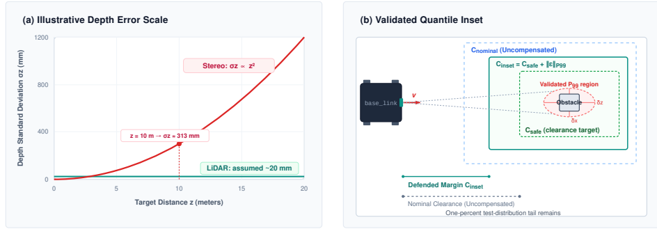
Figure 8.8: Depth error scale and clearance insets: (A) An illustrative stereo one-standard-deviation depth scale grows with squared range for fixed disparity spread; a qualified time-of-flight sensor can be flatter. (B) A validated 99th-percentile norm-error quantile can enlarge the nominal clearance inset, leaving residual tail and bias risk. A hard clearance guarantee requires a justified deterministic error bound and feasible stopping response. Attribution: Book geometric error analysis, CC BY 4.0.
