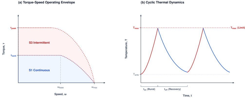
Figure 2.7: Motor torque-speed operating envelope: The permanent magnet synchronous motor torque-speed plane, separating continuous S_1 thermal equilibrium from intermittent S_3 peak acceleration, alongside the exponential thermal accumulation trajectory during peak bursts and conductive cooling during recovery. Winding thermal limits constrain sustainable duty cycle rather than peak inverter current.
