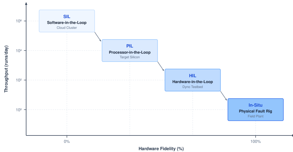
Figure 15.4: Four-stage qualification ladder: Four rungs trading throughput for fidelity, from roughly 10^6 software-only runs a day at zero hardware realism down to a handful of in-situ physical fault injections at full realism. The ladder is not a progression toward accuracy but a sequence of different blind spots, because each stage establishes evidence only within its own causal loop and stays blind to every mechanism outside it.
