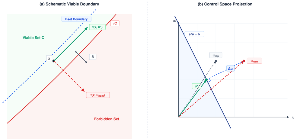
Figure 12.4: Kinetic barrier and torque projection: Panel (a) schematically shows a velocity-dependent viable boundary inset from geometric clearance; the raw distance alone has relative degree two for torque. Panel (b) illustrates Euclidean projection onto a supplied torque half-space. The [2, 1] normal and 5 \text{ N} \cdot \text{m} threshold are abstract arithmetic inputs, not coefficients derived from the arm example. Projection changes torque direction and does not alone certify the Cartesian path.
