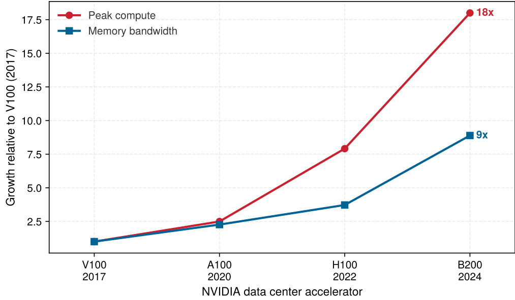
Figure 13.2: Memory bandwidth deficit: Peak compute and memory bandwidth for data center accelerators, normalized to the V100. Compute rises 18× against bandwidth’s 8.9×, and a placement decision works against that ratio because an on-robot budget cannot buy its way past a bandwidth limit. Selected vendor peak or up-to specifications are recorded with source links in the local gpu_memory_wall.csv (B200 dense FP16/BF16 and HBM bandwidth); the plotted ratios do not measure sustained or on-robot latency.
