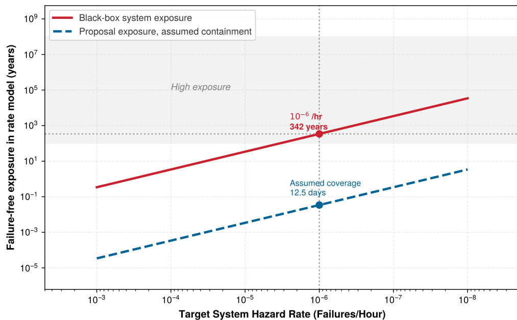
Figure 16.3: Constructed exposure comparison: Red is one-sided 95 percent zero-event exposure for an assumed constant system hazard rate. Blue is exposure to bound the policy's hazardous-proposal rate if independent, representative evidence establishes 99.99 percent containment of those proposals. Hardware failures, ODD gaps, and common-cause faults are additional terms; the blue curve is not an observed release result.
