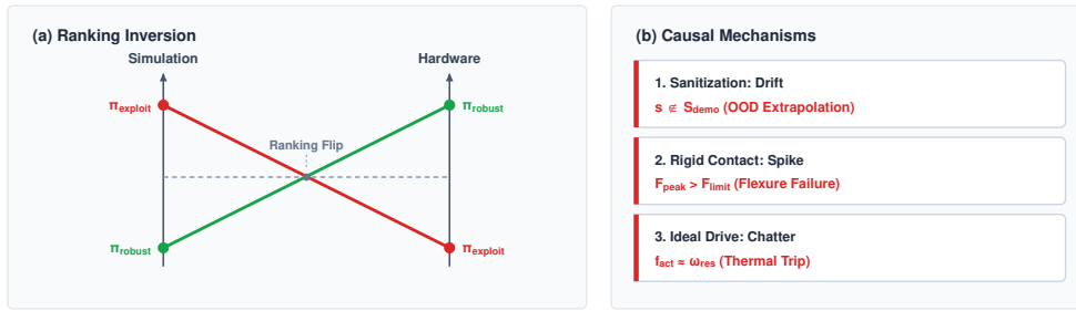
Figure 6.9: Policy ranking inversion on hardware: (a) A parallel-coordinate slope graph illustrating ranking inversion between simulated benchmark score and physical hardware yield: an exploitative policy \pi_{\text{exploit}} scores highest in simulation by gaming unmodeled phenomena but collapses on hardware, while a robust policy \pi_{\text{robust}} preserves physical yield. (b) Causal failure mechanisms that drive ranking flips: out-of-distribution drift from data sanitization ( s \notin \mathcal{S}_{\text{demo}} ), impact force spikes from rigid contact solvers ( F_{\text{peak}} > F_{\text{limit}} ), and actuator resonant torque chatter ( f_{\text{act}} \approx \omega_{\text{res}} ).
