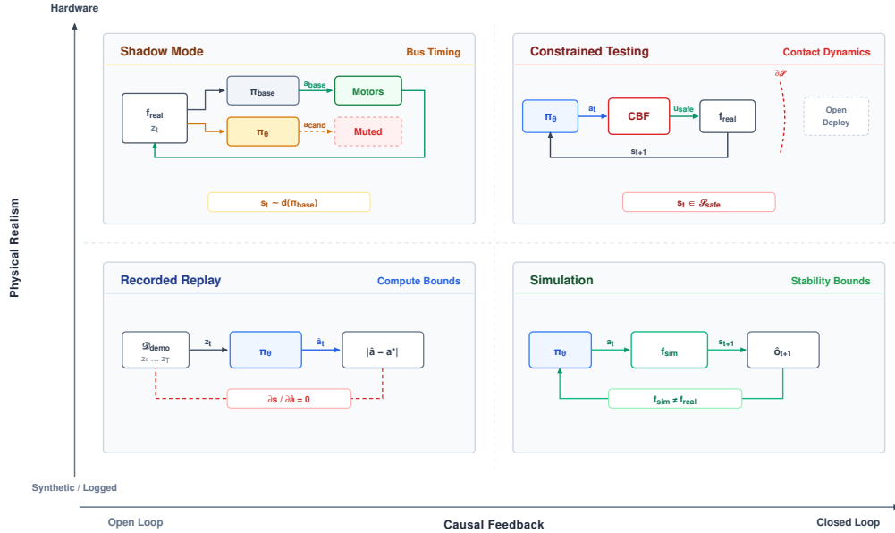
Figure 7.3: Evaluation evidence regimes across the causal-physical manifold: Testing environments span a two-dimensional trade-off space parameterized by causal feedback (open-loop versus closed-loop) and physical realism (synthetic/logged versus live hardware). Recorded replay (bottom left) evaluates computational throughput on static demonstration buffers \mathcal{D}_{demo} , but cannot observe compounding drift ( \partial s_{t+1} / \partial \hat{a}_t = 0 ). Closed-loop simulation (bottom right) restores dynamic state transitions via synthetic physics f_{sim} , testing behavior under modeled dynamics while leaving the unmodeled reality gap unresolved. Shadow operation (top left) subjects candidate inference to real sensor jitter and bus timing, but locks the physical trajectory to the active baseline controller ( s_t \sim d^{\pi_{base}} ). Constrained physical testing (top right) closes the embodied control loop on real hardware f_{real} , but truncates tail failure dynamics at the safety supervisor boundary ( \partial \mathcal{S} ). Open-world deployment beyond the safety boundary remains untestable in any single isolated regime.
