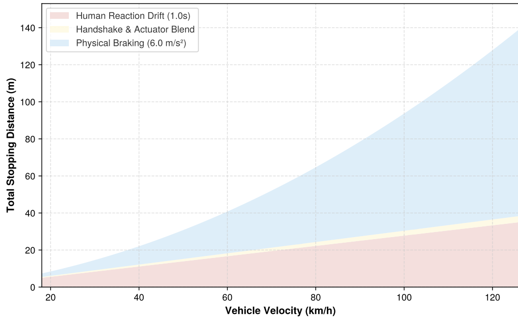
Figure 14.2: Spatial takeover budget: Constructed stopping distance against vehicle velocity, decomposed into human reaction drift, protocol handshake and actuator blend, and physical braking. The reaction and handshake terms grow linearly with speed while braking grows quadratically under the stated constant-deceleration model.
