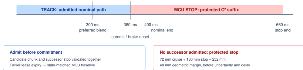
Figure 11.5: Nominal tracking and MCU-owned stop: The worked arm permits a checked replacement before the 360 ms physical stop onset. Nominal references would end at 400 ms, while the separately authorized, C^2 stop reaches rest at 660 ms. The suffix is matched to the commitment state; earlier invalidation needs a state-matched MCU baseline. All deadlines use the MCU monotonic clock, and physical clearance includes the full response and stop.
