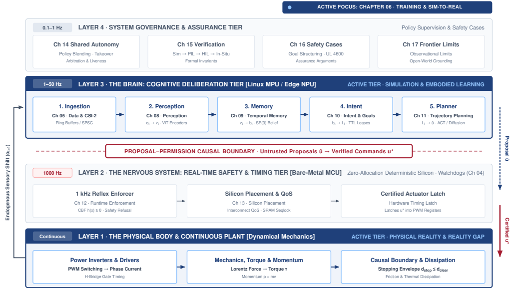
Figure 6.1: Reality gap in stack: The four-tier physical AI systems architecture (Brooks 1986b) highlights the cognitive deliberation tier together with the physical body beneath it, with the reality gap between them as this chapter’s active focus. Read the highlighted pair as the two ends of every sim-to-real transfer, because a policy synthesized against simulated dynamics acquires authority only over the real plant.
