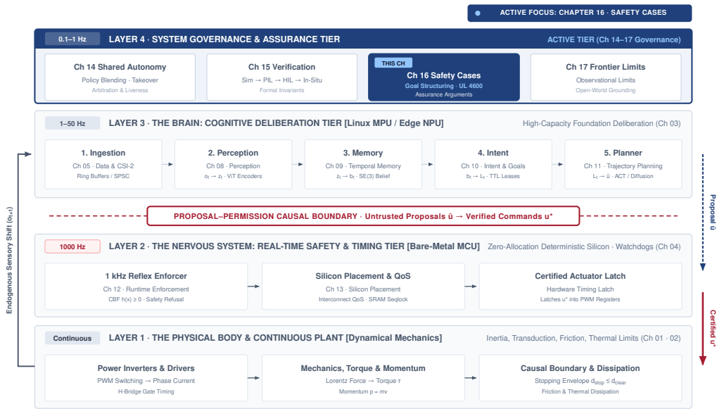
Figure 16.1: Safety cases architecture focus: The four-tier physical AI systems architecture highlights the system governance and assurance tier, with safety cases as this chapter’s active focus. Read the highlighted box as the point where measurements and runtime enforcers from every lower tier are assembled into an auditable argument, because deciding that a machine may operate requires proof rather than statistical optimism.
