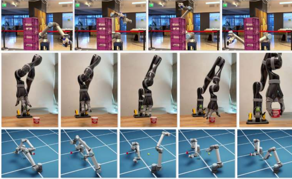
Figure 11.3: Real-time trajectory optimization: GPU-accelerated motion generation executing minimum-jerk splines on hardware, avoiding a dynamic obstacle against a signed distance field, executing a constrained pick-and-lift, and coordinating two arms in a shared workspace. Collision distance is evaluated in continuous time rather than at waypoints, which is what allows the trajectory to be re-optimized while it is being executed. Adapted from (Sundaralingam et al. 2023).
