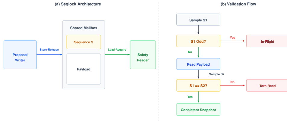
Figure 13.4: Lock-free boundary contract: (a) Inter-core lock-free state exchange architecture where an untrusted proposal writer and a real-time safety reader coordinate through a shared mailbox using atomic memory barriers and a monotonic sequence counter S . (b) Non-blocking validation decision flow where sampling sequence snapshots ( S_1, S_2 ) rejects in-flight updates on one bounded attempt ( S_1 odd) or torn reads ( S_1 \neq S_2 ) without acquiring locks or waiting on the writer.
