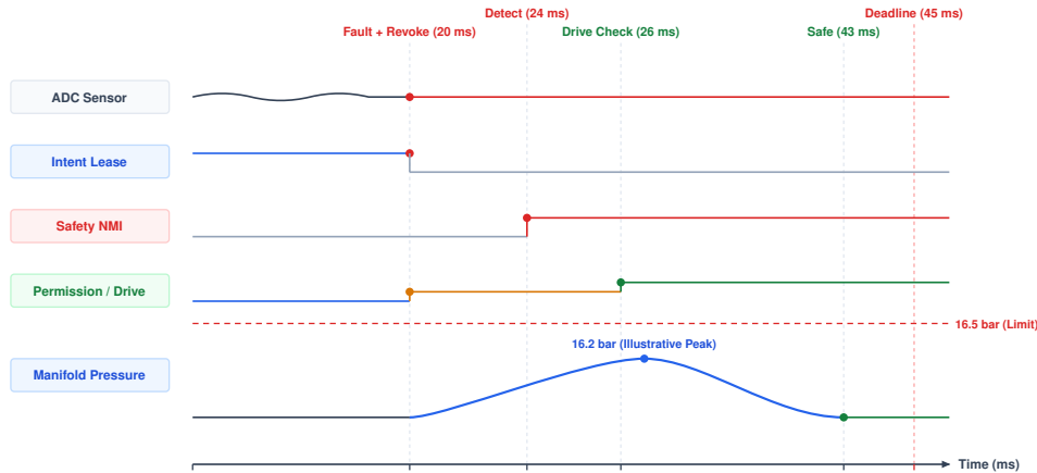
Figure 15.6: Illustrative fault-injection timeline: At 20 ms, lease expiry revokes policy proposal permission and the MCU enters its resident fallback. A separate state-sensor fault asserts a diagnostic NMI at 24 ms; the drive override is confirmed at 26 ms, two milliseconds later. Thus fault-to-detection is 4 ms, NMI-to-drive confirmation is 2 ms, and fault-to-bounded state is 23 ms at 43 ms. The 16.2-bar pressure peak under a 16.5-bar scenario limit is a constructed acceptance trace pending plant and sensor validation.
