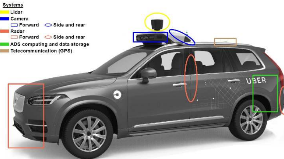
Figure 1.10: Tempe test vehicle sensor locations: The NTSB diagram identifies the developmental ADS vehicle's lidar, camera, radar, computing, and telecommunications locations. Uber ATG disabled the factory forward collision warning and automatic emergency braking during ADS operation, removing a redundancy layer (National Transportation Safety Board 2019). (Source: NTSB, public domain).
