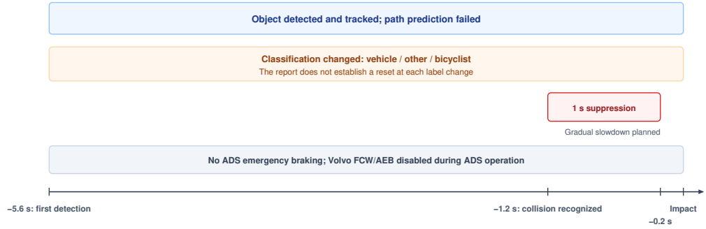
Figure 12.7: Tempe detection and braking timeline: The NTSB reports first detection 5.6 s before impact and recognition of imminent collision 1.2 s before impact. The ADS suppressed its motion plan for one second and then planned gradual slowing; it did not perform emergency braking. Classification and path prediction failed. The Volvo forward-collision warning and automated emergency braking functions were disabled while the developmental ADS operated. The report does not establish a Kalman-filter reset at each label change. (Adapted from NTSB/HAR-19/03 (National Transportation Safety Board 2019).)
