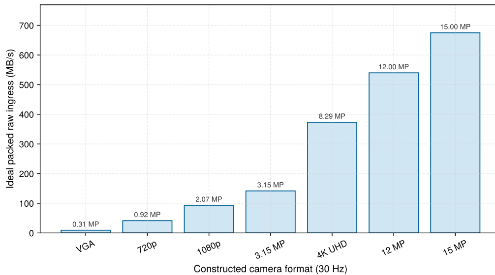
Figure 8.5: Illustrative camera format ingress: Packed raw bytes per second for selected constructed formats, all at 30 Hz. The rates exclude interface overhead, copies, ISP traffic, and arbitration; they are not historical fleet measurements or safety-read delay.
