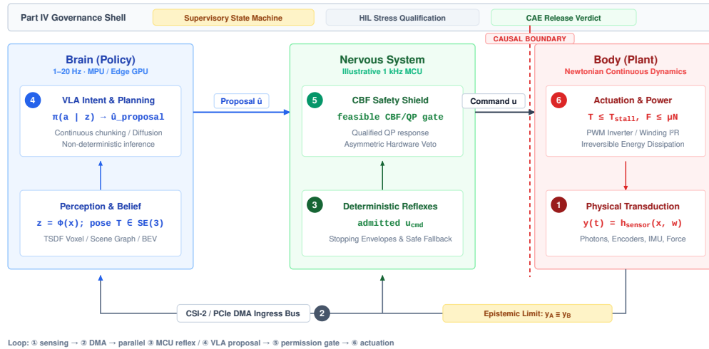
Figure 17.6: Closed causal loop: Learned planning submits proposals; an illustrative 1 kHz MCU checks a feasible permission constraint under its state, plant, actuator, and deadline assumptions. Governance records the tests and release conditions. The drawing is an architecture, not an ASIL certification or a universal controller rate.
