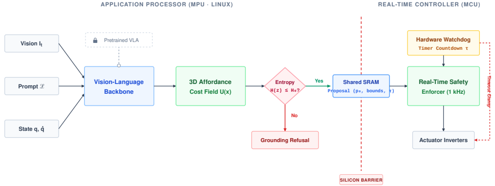
Figure 10.5: Grounded intent pipeline architecture: This proposed implementation turns multimodal inputs into a candidate spatial field, applies an ambiguity filter, and passes a bounded proposal across an MPU-to-MCU permission boundary. The MCU validates evidence age, configured limits, and feasible fallback before admitting a local countdown. Cross-attention and prompting supply proposals, not certified physical constraints (synthesized from Huang et al. (2023), Ahn et al. (2023), and Gray (1989)).
