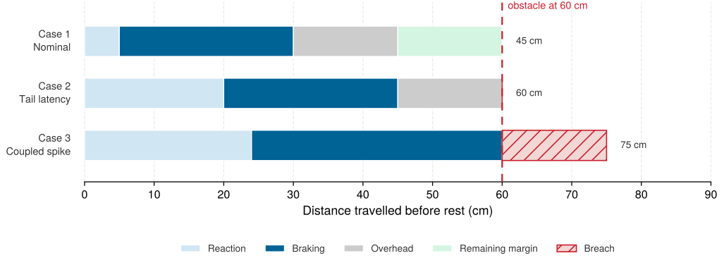
Figure 2.3: Dynamic stopping distance envelope: Total stopping distance decomposed into linear reaction lag, quadratic kinetic braking travel, and spatial overhead. Of the speed- and delay-dependent terms, doubling latency expands the pair by 17 percent, whereas doubling velocity quadruples braking travel for a 267 percent expansion; the spatial overhead is fixed. Case 1 operates with safe clearance; Case 2 compresses margin under tail latency; and Case 3 breaches the obstacle envelope when speed and compute delay couple.
