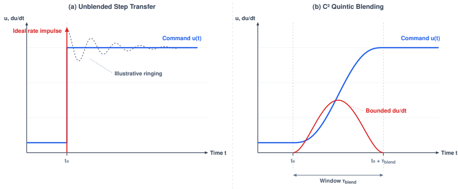
Figure 14.5: Illustrative command transfer: A step and fixed-endpoint quintic blend are compared. Blue is the command; red is its ideal derivative, and gray ringing is schematic. The profile bounds the commanded rate for the assumed endpoints; plant response needs measurement.
