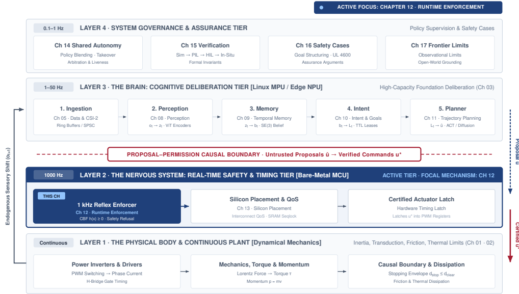
Figure 12.1: Reflex enforcer architecture focus: In the physical AI systems architecture, the deterministic nervous system sits between the unverified deliberative brain and the dynamical body, serving as the sole authority permitted to translate advisory commands into physical force or refuse them outright. Operating on a bounded millisecond control period, the enforcer projects candidate actions onto forward-invariant safe sets and manages a multi-tier fallback hierarchy to retain a conditional, tested fallback path.
