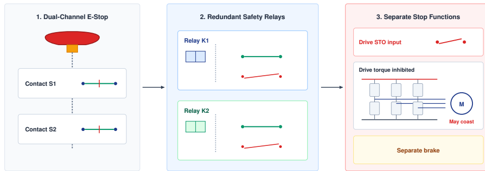
Figure 12.5: Illustrative emergency-stop circuit: Two emergency-stop contacts feed safety relays and drive STO inputs. A spring-applied brake is shown as a separate optional path; an external supply contactor, if fitted, is another independent function. The diagram specifies no response time, performance level, or stopping distance. A moving motor can coast after STO, so the physical stop must be validated for the load and state.
