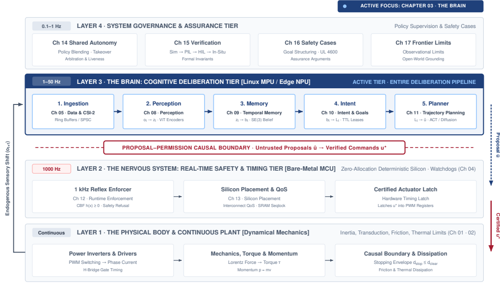
Figure 3.1: The brain in the Physical AI stack: The four-tier physical AI systems architecture highlights the cognitive deliberative layer. Operating above the real-time nervous system and physical body, the learned brain processes high-dimensional multimodal streams to generate candidate proposals, with execution authority reserved for downstream deterministic safety governors.
