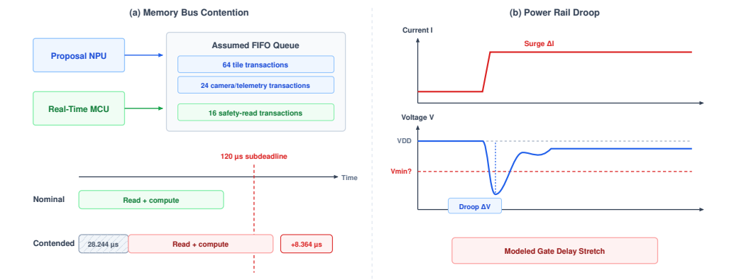
Figure 13.3: Heterogeneous SoC interference: (a) In the constructed FIFO example, 88 queued 4,096-byte transactions delay a 65,536-byte safety read and push read plus compute to 128.364, \mu\text{s} against a 120, \mu\text{s} subdeadline; priority bypass would change the result. (b) A separate assumed 6 A in 2 ns current step gives 138 mV PDN droop. The drawn V_{\min} crossing is a conditional hazard, not established by that droop calculation.
