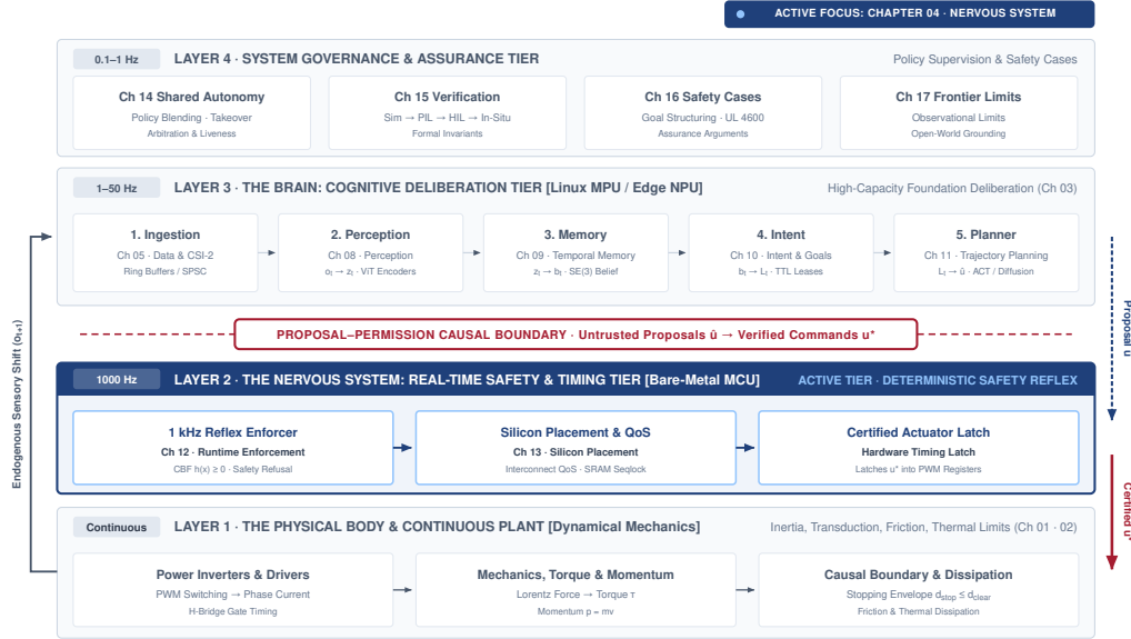
Figure 4.1: The real-time nervous system: The four-tier physical AI systems architecture highlights the real-time nervous system (Layer 2). Operating between the deliberative brain (Layer 3) and dynamical body (Layer 1), the deterministic nervous system enforces multi-rate synchronization, transports sensorimotor signals under hard real-time deadlines, and maintains exclusive execution authority over actuator power.
