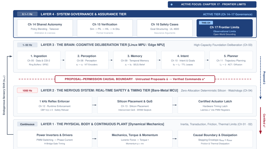
Figure 17.1: Frontier limits architecture focus: The four-tier physical AI systems architecture highlights the system governance and assurance tier, with frontier limits as this chapter’s active focus. Read the highlighted box as the edge of the assurance argument, where cataloged failure modes outrun the runtime detectors built to catch them and architectural containment has to carry whatever risk remains.
