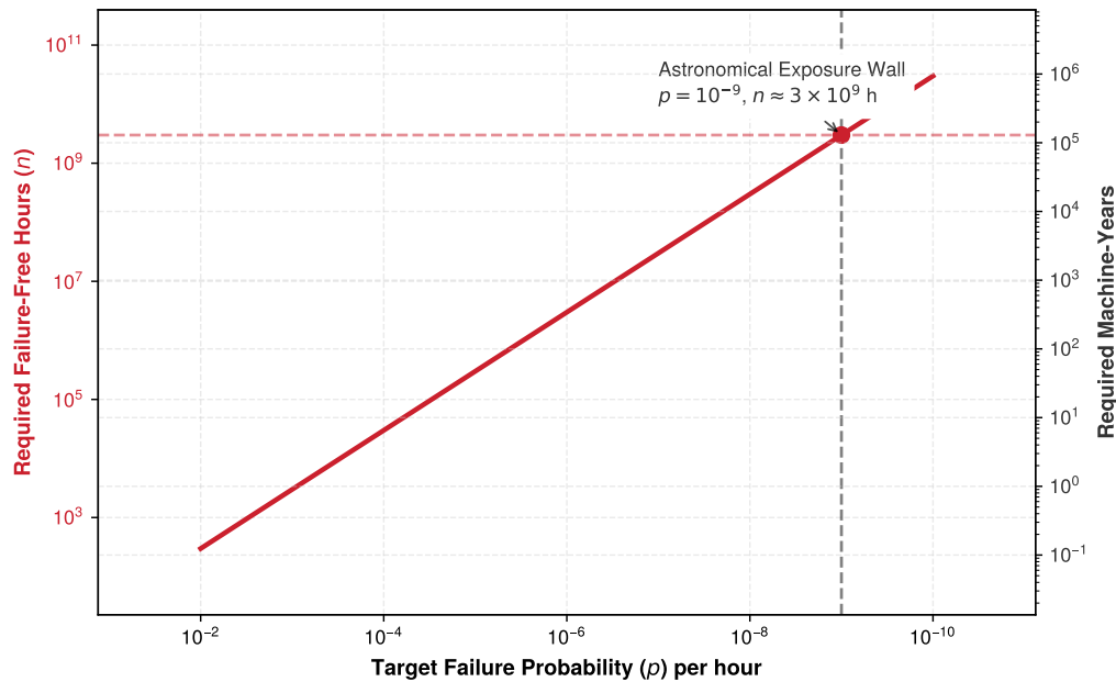
Figure 17.2: Astronomical exposure wall: Required failure-free exposure hours against target failure probability per hour, under a Poisson zero-event model at 95 percent confidence, with the equivalent machine-years on the opposing axis. Certifying 10^{-9} per hour demands roughly three billion failure-free hours, which this fleet cannot accumulate within its 90-day update interval.
