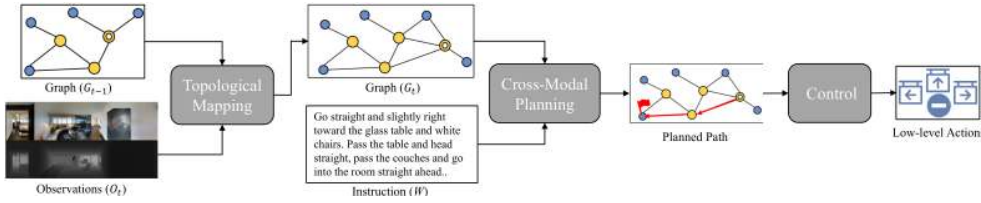
Figure 3.8: Topological vision-language navigation: Embodied navigation architecture executing natural-language spatial instructions. Panoramic visual observations are encoded into perceptual tokens, matched against prompt embeddings, and cross-referenced with a dynamically updated topological navigation graph. The action decoder prunes unreachable nodes and emits metric waypoint offsets ( \Delta x, \Delta y ) and heading setpoints to guide the chassis along traversable semantic frontiers without requiring an exact geometric prior map. (Adapted from An et al. (An et al. 2023)).
