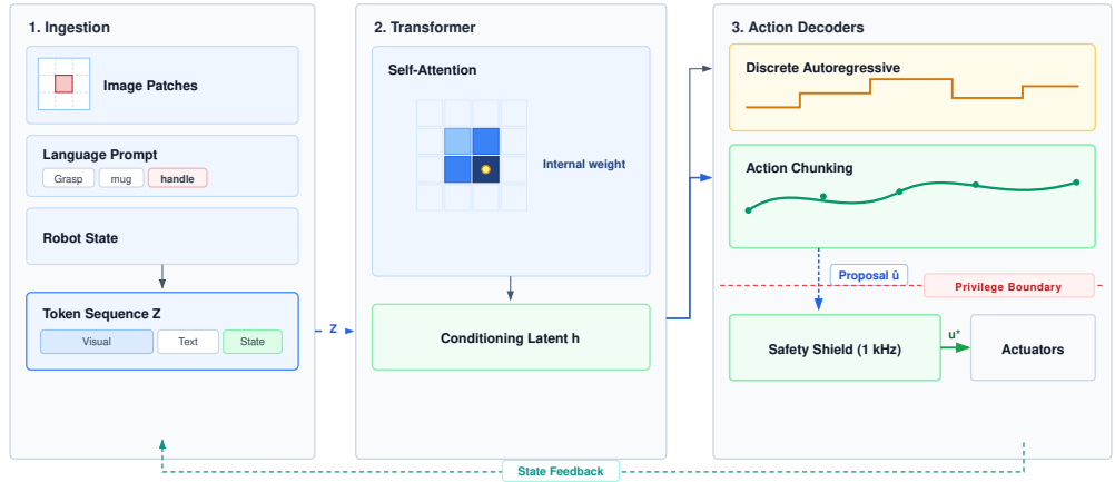
Figure 3.7: Embodied Vision-Language-Action (VLA) architecture: A representative dataflow. (1) Camera patches receive 2D image-position and camera identifiers alongside language and robot-state tokens; metric depth still requires calibrated evidence. (2) Self-attention mixes the combined token sequence; the colored grid illustrates internal attention weights, not a verified affordance or grasp pose. (3) Discrete autoregressive decoders emit tokens sequentially, whereas continuous decoders generate candidate multi-step chunks ( \mathbf{A}_{t:t+H-1} ) through one pass or iterative denoising. (4) An independent permission path checks candidate motion against sensed state and modeled limits before actuation. (Synthesized from Brohan et al. (Brohan, Brown, Carbajal, Chebotar, Dabis, et al. 2023; Brohan, Brown, Carbajal, Chebotar, Chen, et al. 2023), Kim et al. (Kim et al. 2024), and Octo Model Team (Octo Model Team et al. 2024)).
