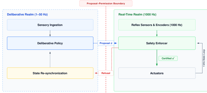
Figure 3.12: Two-speed brain architecture: An untrusted deliberative realm running at 1–50 Hz and a trusted real-time realm running at 1000 Hz, separated by the proposal-permission privilege boundary. The independent safety supervisor checks sensed state and modeled limits on each control cycle before granting execution permission; protection depends on valid sensing and feasible fallback.
