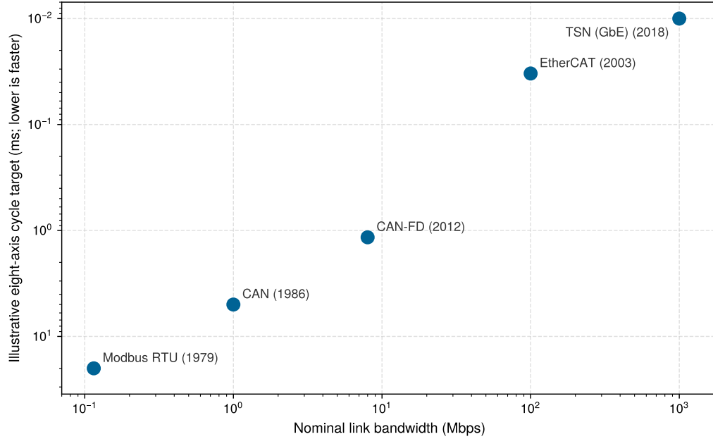
Figure 4.5: Illustrative fieldbus design space: Nominal link bandwidth and selected eight-axis cycle targets for five protocol scenarios. The cycle values are teaching assumptions, not measured device results or a protocol-level guarantee; workload, implementation, faults, and full response-time analysis determine feasible cycles.
