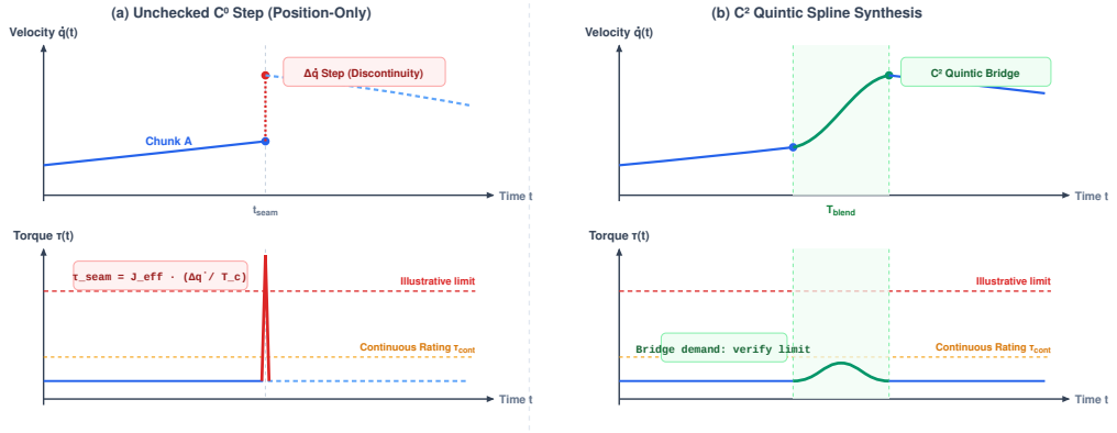
Figure 11.4: Seam demand and checked bridge: A position-matched velocity step creates a large one-tick inertial torque request. A finite C^2 bridge removes the reference velocity step, but its interior jerk, torque, and joint response still require validation.
