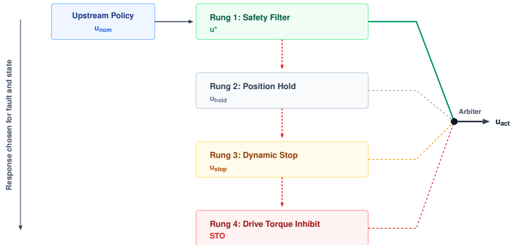
Figure 12.6: Available enforcement responses: A deterministic arbiter can select feasible torque projection, controlled hold, controlled stop, or drive torque inhibit according to the current fault and measured plant state. The responses are alternatives with different prerequisites; descending the diagram does not imply increasing physical safety or faster arrest.
