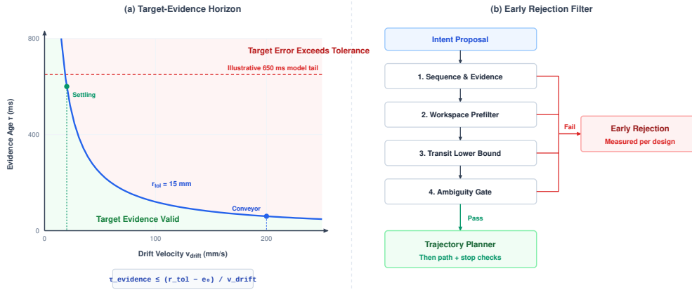
Figure 10.7: Target-evidence horizon and early filters: Panel (a) plots the illustrative bound \tau_{\text{evidence}} \leq (r_{\text{tol}} - e_0) / v_{\text{drift}} ; its green region means only that the target remains within the stipulated error tolerance. A 650 ms model cadence cannot renew the 60 ms conveyor case. Panel (b) shows conceptual early rejection stages before full path and stopping checks; no universal runtime is claimed.
