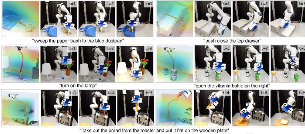
Figure 10.3: Manipulator 3D affordance grounding: VoxPoser composes language-guided 3D value maps for manipulation tasks (Huang et al. 2023). The illustrated research system proposes spatial objectives; an independent permission and stopping wrapper would require separate design and validation. (Source: Huang et al., 2023 (Huang et al. 2023), CC BY 4.0).
