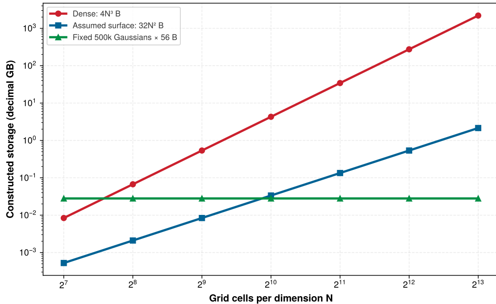
Figure 9.6: Constructed spatial-memory storage scenarios: A dense cube uses four bytes per voxel, the illustrative octree allocates one 32-byte surface cell per squared grid dimension, and the Gaussian scene holds a fixed count and packing while grid resolution varies. These are storage models, not equal-fidelity or measured runtime benchmarks; Gaussian count must rise if a stricter geometry target requires it.
