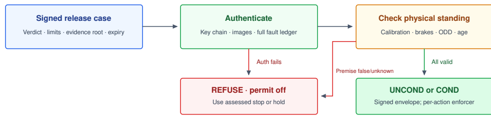
Figure 16.6: Fail-closed release pipeline: The signed verdict and evidence root pass key, image, and complete fault-ledger authentication, then current calibration, brake, and ODD checks. Either check can refuse permission. Only a valid signed full or separately signed restricted case reaches per-action enforcement. Attribution: Textbook production team (CC BY-NC-ND 4.0).
