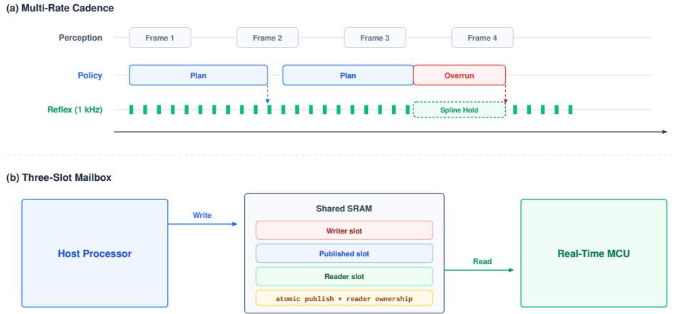
Figure 4.3: Multi-rate cadence and buffer exchange: (a) Representative perception, policy, and reflex rates; the reflex loop retains the last valid spline during a policy overrun only until its freshness limit. (b) A conceptual three-slot mailbox; the following algorithm specifies a simpler single-slot seqlock baseline. A production three-slot variant additionally needs atomic publication and reader-slot ownership (synthesized from Slotine & Li (1991) and ARM Architecture Reference Manual).
