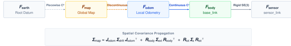
Figure 8.2: Coordinate frame tree and uncertainty: The spatial coordinate frame hierarchy formalizes the separation between continuous local dead reckoning ( \mathcal{F}_{odom} \rightarrow \mathcal{F}_{body} ) consumed by high-frequency tracking loops and discontinuous global map corrections ( \mathcal{F}_{map} \rightarrow \mathcal{F}_{odom} ) consumed by global planners. Spatial covariance compounds across the kinematic chain ( \Sigma_{map} \approx J_{odom} \Sigma_{drift} J_{odom}^T + R_{body} \Sigma_{ext} R_{body}^T + R_{tot} \Sigma_z R_{tot}^T ), requiring downstream consumers to reject observations that lack an explicit coordinate key \mathcal{F}_{sensor} , acquisition epoch t_0 , and covariance envelope \Sigma_z . Attribution: Book kinematic systems diagram, CC BY 4.0.
