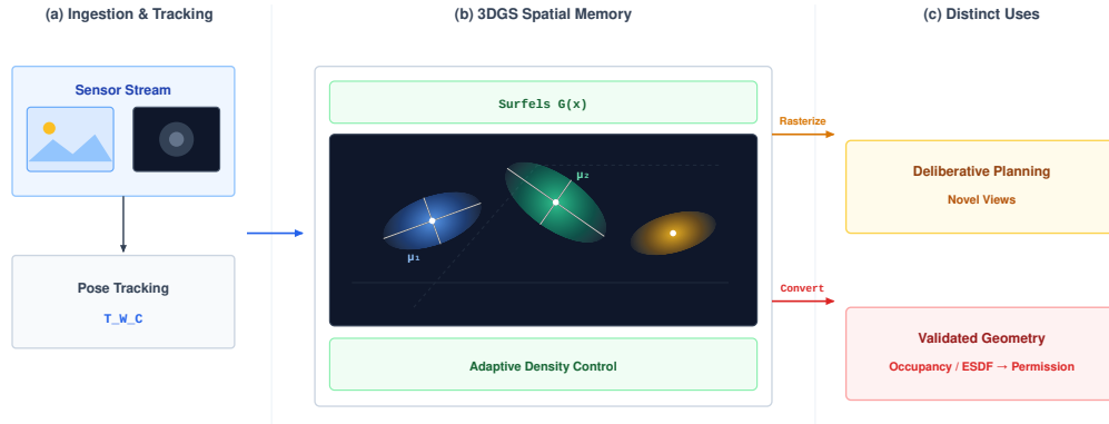
Figure 9.5: Gaussian memory and clearance handoff: Camera observations update a Gaussian scene for novel-view rendering. Its visual output does not directly supply conservative collision distance; a separately validated geometry or occupancy conversion and permission check are required (Kerbl et al. 2023; Matsuki et al. 2024).
