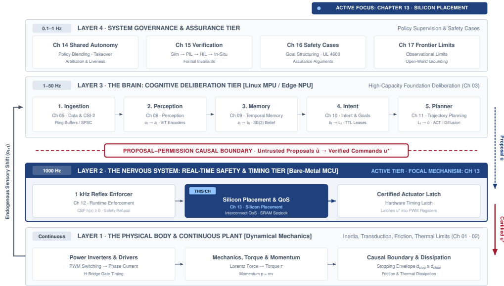
Figure 13.1: Silicon placement architecture focus: The four-tier physical AI systems architecture highlights the real-time safety tier, with silicon placement as this chapter’s active focus. Read the highlighted box as the physical co-location boundary where cognitive bursts and hard real-time reflex loops land on one system-on-chip and then compete for memory controllers, interconnect crossbars, power rails, and thermal mass.
