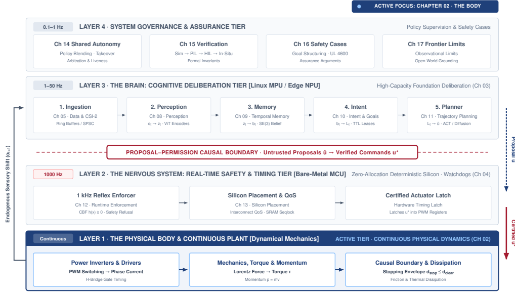
Figure 2.1: The body in the Physical AI stack: The four-tier physical AI systems architecture highlights the physical world at its foundation, bounded by mechanics, thermodynamics, and electromagnetism. Above the causal boundary, the nervous system and learned brain must budget all sensing latency, stopping distances, and actuation requests against these non-negotiable physical constraints.
