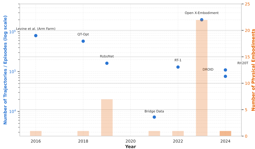
Figure 5.6: Robot learning dataset snapshots: Unconnected blue markers show episode counts for selected datasets (logarithmic left axis), not a cumulative time series. Orange bars show embodiment counts (right axis), including the pooled Open X-Embodiment jump in 2023. Dataset metadata: Open X-Embodiment Collaboration et al. (2024) and the chapter CSV.
