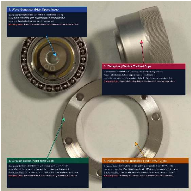
Figure 2.4: Strain wave gear assembly: Robotic strain wave transmission component set: (1) elliptical wave generator with flexible ball bearings, (2) flexible cup flexspline with external teeth, (3) rigid circular spline with internal teeth, and (4) transmission systems invariant governing reflected rotor inertia ( J_{ref} = N^2 J_m ). Elastic deformation enables zero initial backlash at high reduction ratios (50 : 1 to 160 : 1), but introduces torsional compliance, hysteresis, and tooth fatigue vulnerability under sudden shock loads.
