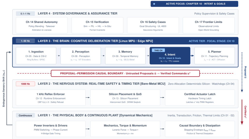
Figure 10.1: Intent stage architecture focus: The four-tier physical AI systems architecture highlights the cognitive deliberation tier, with intent as the fourth brain stage and this chapter's active focus. The stage turns belief b_t into a goal \ell_t , projecting semantic objectives across the privilege boundary as time-bounded geometric leases that expire on their own unless the nervous system receives a refresh.
