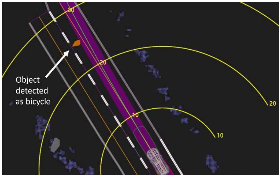
Figure 14.6: Tempe preliminary playback still: One overhead NTSB playback frame about 1.3 seconds before impact, not a classification or braking telemetry trace. The NTSB final report separately records first detection at 5.6 seconds, emergency recognition at 1.2 seconds, and a one-second ADS emergency-brake suppression through about 0.2 seconds before impact. Image: NTSB preliminary Figure 2, via Wikimedia Commons, U.S. public domain.
