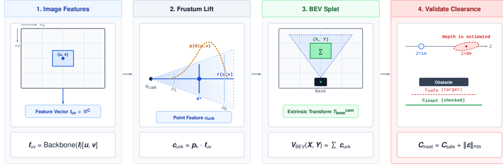
Figure 8.7: Camera ray frustum lifting and BEV splatting: LSS (Philion and Fidler 2020) places learned depth hypotheses from each camera in a shared metric BEV frame; that coordinate transform does not resolve monocular depth ambiguity. The final clearance inset requires separately validated metric residuals, bias, and a chosen tail quantile or deterministic error bound before permission. (Architecture adapted from Philion and Fidler (2020).)
