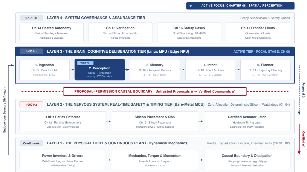
Figure 8.1: Perception stage architecture focus: The four-tier physical AI systems architecture highlights the cognitive deliberation tier, with perception as the second brain stage and this chapter’s active focus. The stage converts raw observations o_t into latent state z_t , bounded upstream by sensor transduction it cannot improve and downstream by the memory that must store whatever it infers.
