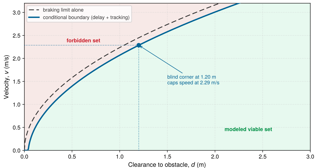
Figure 12.3: Conditional stopping envelope: A parabolic boundary separates states with modeled braking clearance from states that have already exhausted it. The inset includes bounded response delay, transient tracking error, and any nonzero position-estimate bound. The curves are valid only for the stated lower bound on braking deceleration and operating envelope.
