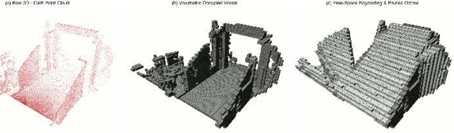
Figure 9.4: Probabilistic octree volumetric mapping: A corridor traversal reconstructed from raw point cloud into a probabilistic octree and then into explicit free, occupied, and unknown space (Hornung et al. 2013). The third panel is what distinguishes spatial memory from an accumulated point cloud, because raycasting records evidence of emptiness along sightlines, letting the map actively retire a phantom obstacle track instead of waiting for a timeout to expire it. (Credit: Hornung et al. / Autonomous Intelligent Systems Lab, University of Freiburg, CC BY 3.0).
