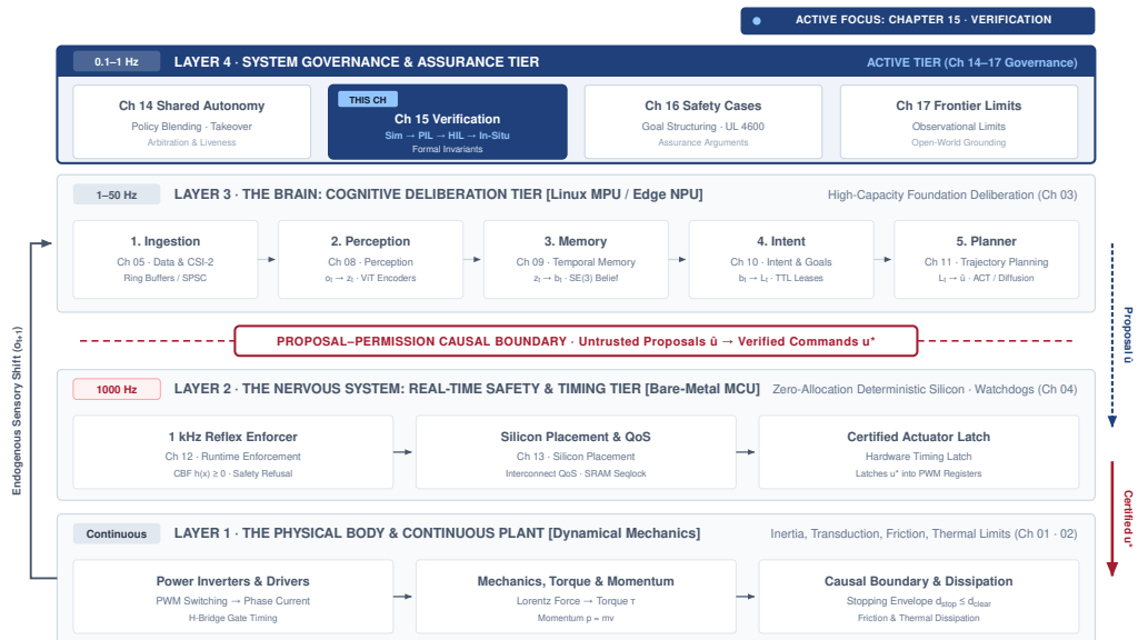
Figure 15.1: Verification architecture focus: The four-tier physical AI systems architecture highlights the system governance and assurance tier, with verification as this chapter's active focus. Read the highlighted box as the qualification ladder that walks a safety claim from simulation through processor-in-the-loop and hardware-in-the-loop stages to in-situ trials, attacking one cyber-physical boundary at each rung.
