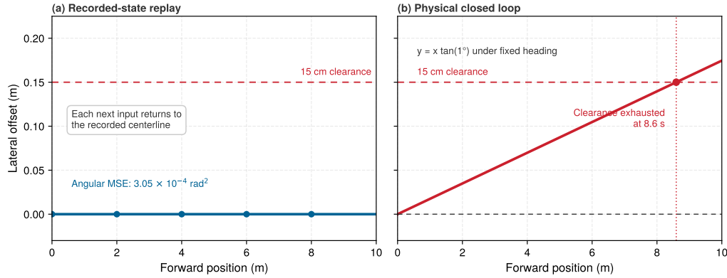
Figure 7.2: Open versus closed loop divergence: A stipulated persistent 1.0^\circ heading offset gives 3.05 \times 10^{-4} \text{ rad}^2 angular mean squared error on recorded centerline states. In the physical corridor example, admitted motion with that fixed heading drifts linearly and reaches the 15 cm side clearance at 8.6 s. The example makes no claim about recovery by a different controller.
