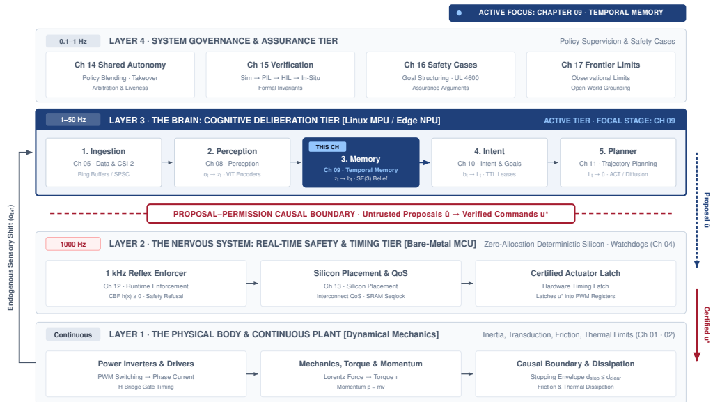
Figure 9.1: Memory stage architecture focus: The four-tier physical AI systems architecture highlights the cognitive deliberation tier, with memory as the third brain stage and this chapter's active focus. The stage carries latent state z_t into a persistent spatial belief b_t , making it the only place the system holds what its sensors can no longer see.
