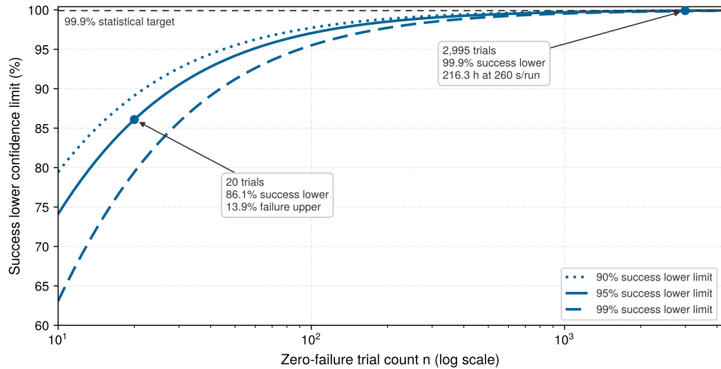
Figure 7.6: Confidence bounds and testing budgets: One-sided Clopper-Pearson success lower limits after zero failures at 90, 95, and 99 percent confidence. At 95 percent confidence, 20 iid runs give an 86.1 percent success lower limit and a 13.9 percent failure upper limit under the tested distribution. Reaching a 99.9 percent success lower limit requires 2,995 zero-failure draws under the same assumptions, or 216.3 hours at the illustrative 260-second cycle. Neither threshold grants deployment permission or proves component wear life.
