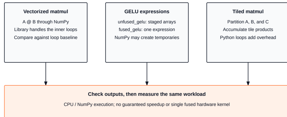
Figure 19.1: Three NumPy execution paths: Vectorized multiplication delegates to a library, the GELU helps retain different intermediate arrays, and tiled multiplication explicitly accumulates block products. Every comparison checks values before measuring time.
