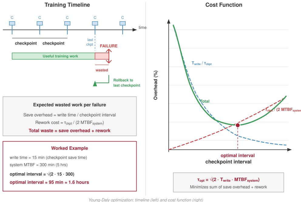
Young-Daly optimization: timeline (left) and cost function (right)
