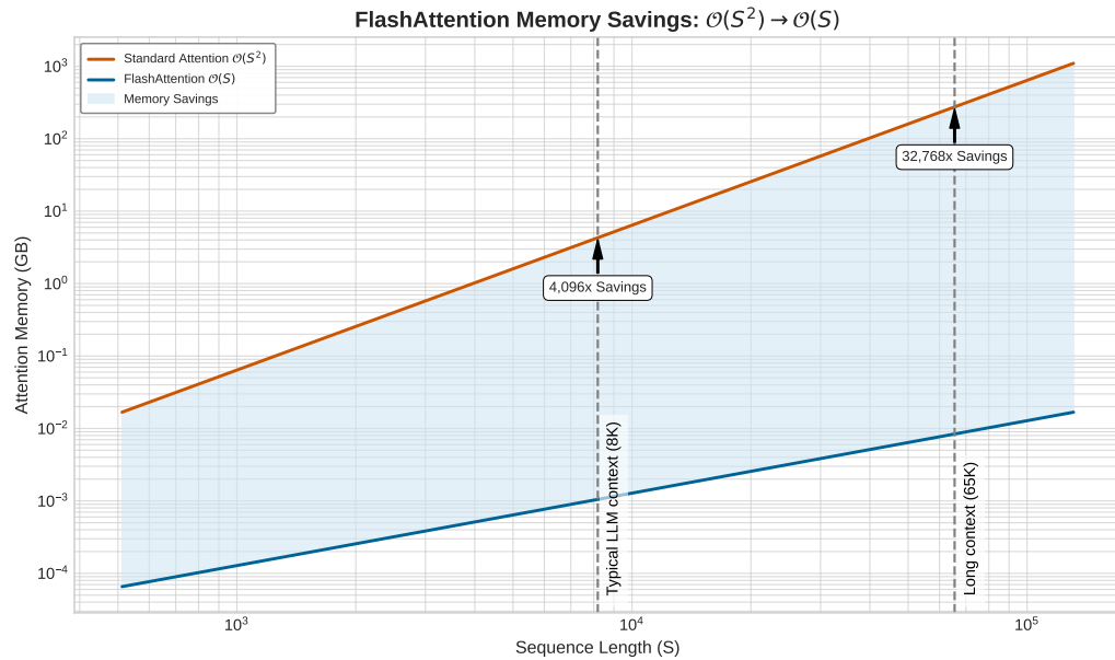
Figure 9.5: FlashAttention Memory Savings: O(S^2) \rightarrow O(S) . Standard attention allocates the full S \times S score matrix in HBM, while FlashAttention maintains only O(S) running statistics. The shaded region represents memory freed for KV cache, activations, or larger batch sizes. This workspace-only comparison uses a narrower boundary than the traffic scenario in the text; its point is the widening shape of the gap as context grows, not a headline ratio.
