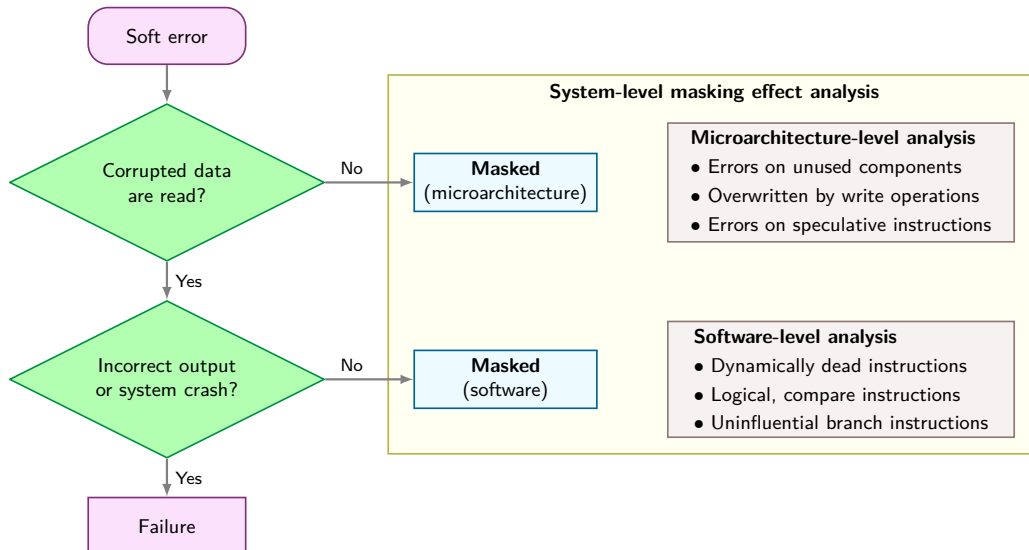
Figure 7.24: Error Masking: Microarchitectural redundancy can absorb single-bit faults before they propagate to observable system errors, highlighting a discrepancy between hardware-level and software-level fault models. This figure details how fault masking occurs within microarchitectural components, demonstrating that software-based error detection tools may underestimate the true resilience of a system to transient errors.
