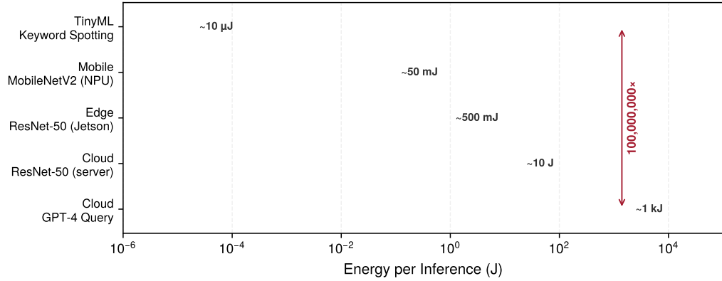
Figure 2.6: Illustrative Energy per Inference Anchors: Order-of-magnitude scenario anchors span eight orders of magnitude, from ~10 \mu J for TinyML keyword spotting to ~1 kJ for a cloud LLM query. These are pedagogical deployment anchors rather than measurements produced by the analytical node model used later in table 2.12.
