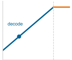
Decode sits memory-bound, left of the roofline ridge.
