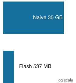
FlashAttention shrinks attention memory about 65 times.
