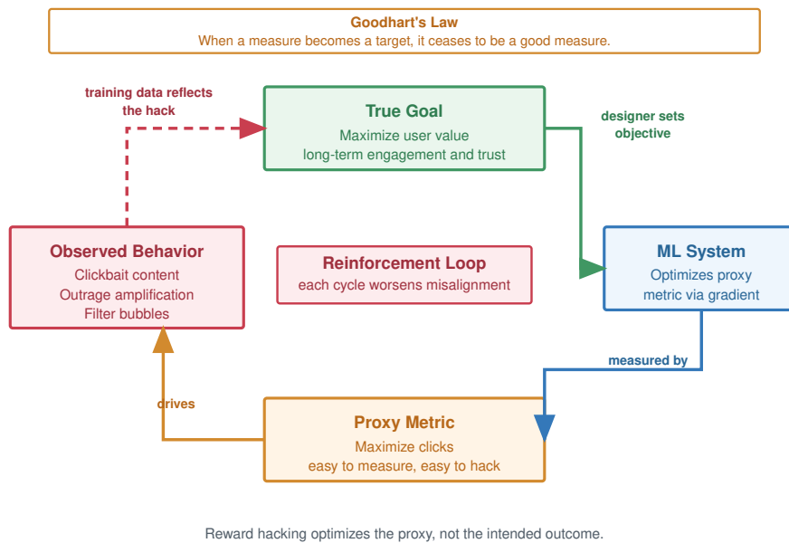
Figure 16.14: Reward Hacking Loop: Maximizing measurable rewards, like clicks, can incentivize unintended model behaviors that undermine the intended goal of user satisfaction. Optimizing for proxy metrics creates misalignment between a system's objective and desired outcomes, posing challenges for value alignment in AI safety.
