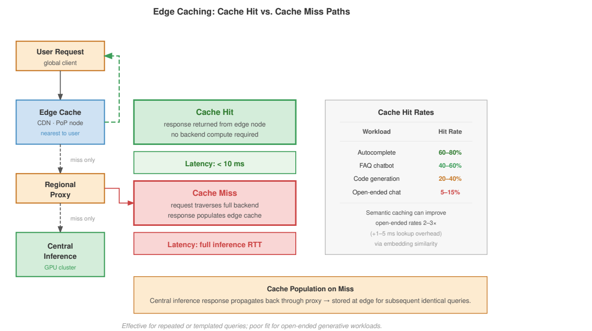
Figure 10.25: Edge Caching: Cache Hit vs. Cache Miss Paths: A cache hit returns immediately from the CDN edge node (<10 ms). A cache miss flows through to central inference and populates the cache on return. Hit rate determines the effective cost saving; open-ended generative workloads have low repeatability and benefit little from this pattern.
