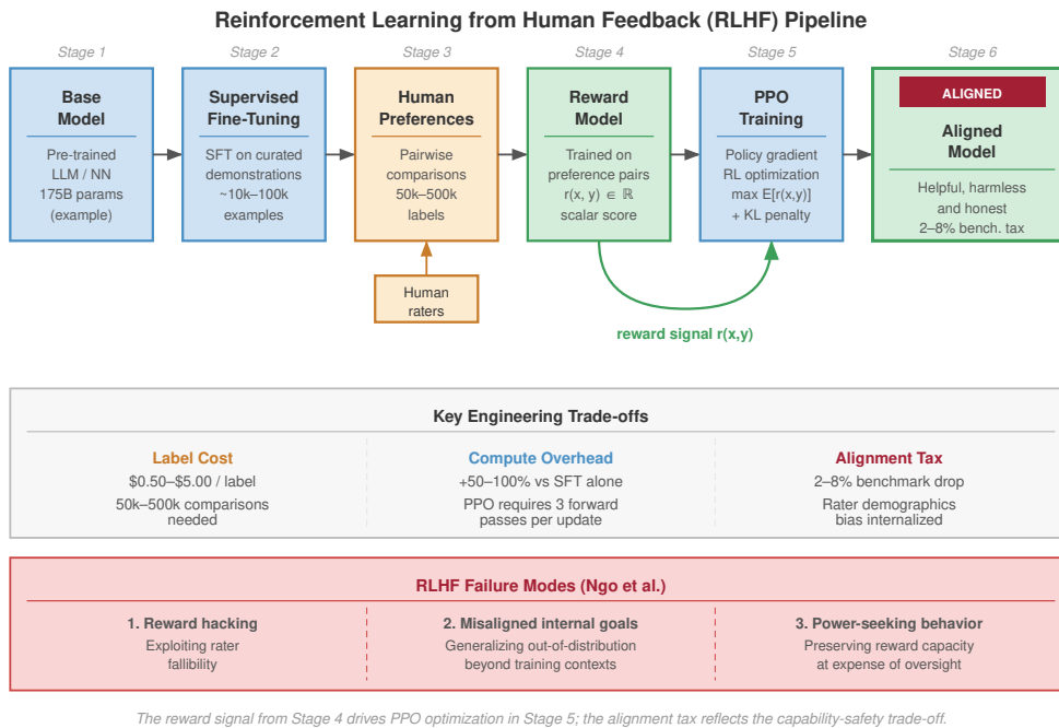
Figure 16.12: Reinforcement Learning from Human Feedback (RLHF) Alignment Pipeline: Six-stage process for aligning generative models: (1) a pretrained Base Model, (2) Supervised Fine-Tuning (SFT) on demonstrations, (3) Human Preference collection, (4) Reward Model training, (5) Proximal Policy Optimization (PPO) Training, and (6) a final Aligned Model. The figure also annotates label cost, compute overhead, and alignment tax, plus three RLHF failure modes (reward hacking, misaligned internal goals, power-seeking behavior).
