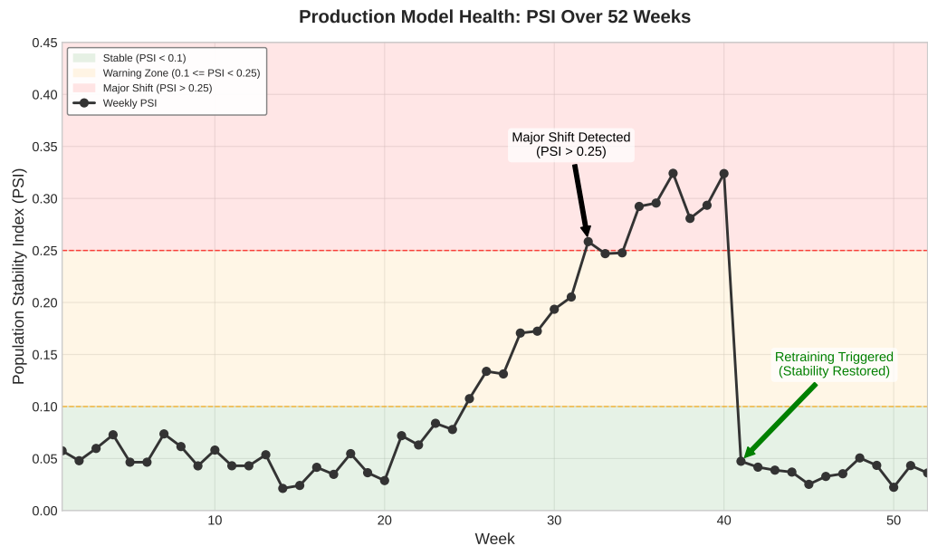
Figure 14.10: The Distribution Shift Detector: Monitoring Population Stability Index (PSI) over a year. The model remains stable through week 24, enters the orange warning zone at week 25 as user behavior shifts, and breaches the red critical threshold at week 32. Automated retraining restores model stability at week 41.
