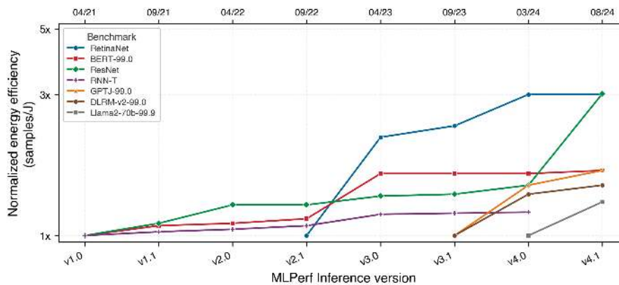
Figure 12.8: Data-Center Energy Efficiency Gains: Each series is normalized to its own first plotted version, so compare improvement within a workload rather than absolute efficiency across workloads. Source: (Tschand et al. 2024).
