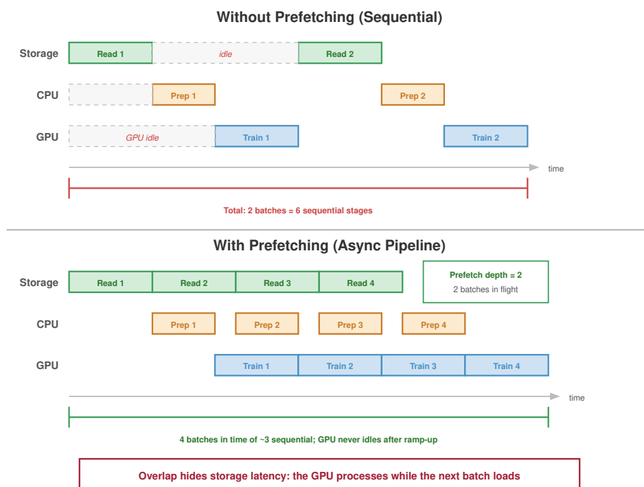
Figure 4.5: Pipelined Data Loading: The CPU prepares Batch i + 1 while the GPU processes Batch i . Pipelining hides storage latency, but only if the prefetch buffer is deep enough to absorb variance.
