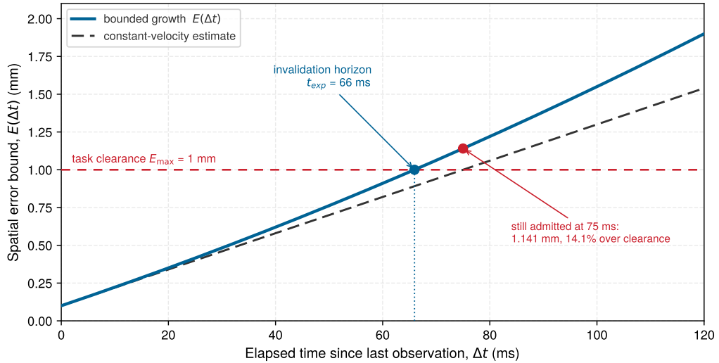
Figure 9.5: Belief uncertainty and invalidation horizon: Spatial error bound E(\Delta t) of a gripper finger entering the cage door's latch-release slot, expanding quadratically under unobserved forward propagation until intersecting the slot clearance E_{\max} = 1 mm at invalidation horizon t_{\exp} = 66 ms. A dashed constant-velocity estimate grows more slowly, and the red marker shows that estimate still admitting the belief after the bounded error has passed the clearance. Belief has a shelf life governed by physical disturbance dynamics, and only sensor re-acquisition resets the evidence clock.
