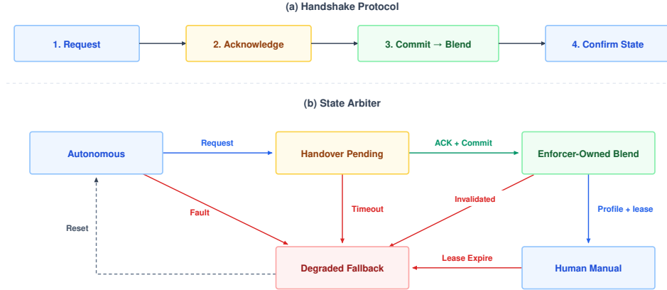
Figure 14.3: Authority handshake and owner states: Request and acknowledgment precede atomic commit. At commit the policy token is revoked and the enforcer owns the blend between checked, latched endpoints; manual proposals begin only after profile completion with a live lease. Timeout invokes a separately validated fallback.
