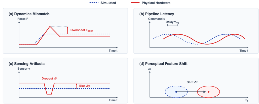
Figure 6.5: Sim-to-real reality gap vector: The sim-to-real gap decomposed across four physical channels, dynamics (a), sensing (c), appearance as perceptual feature shift (d), and timing (b), each measured from paired traces rather than from an aggregate loss. The decomposition is the point, because the four channels fail differently and a scalar loss averages them into a number that names none of them. A 5.5 percent pixel discrepancy that looks trivial masks a 6.0 mm spatial shift that exceeds the assembly tolerance.
