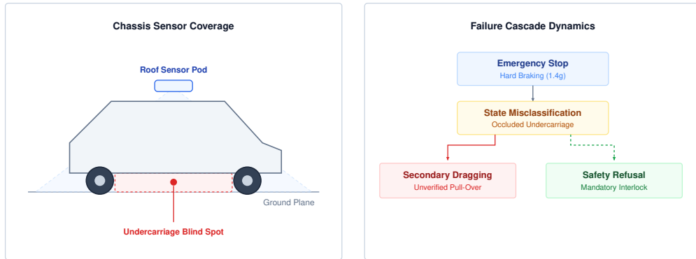
Figure 5.8: Cruise undercarriage blind spot failure: The test vehicle’s roof-mounted sensors survey the perimeter at and above bumper level, leaving a blind spot beneath the floorpan, and the failure cascade that followed. The first stop worked, halting in 0.46 s at 1.4g. What turned a collision into a dragging was the recovery: the state was misclassified as a side-swipe, the nominal pull-over primitive engaged, and drive torque was reapplied without any positive check for undercarriage clearance.
