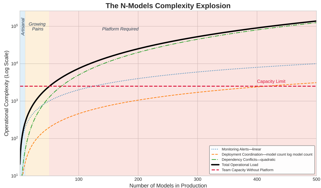
Figure 12.1: The N-Models Complexity Explosion: Monitoring alerts grow linearly with model count, deployment coordination grows as O(N_{\text{models}} \log N_{\text{models}}) , and dependency conflicts grow quadratically as models share features and data sources. The total operational load crosses team capacity around 50 models, marking the transition from artisanal model management to platform-required operations.
