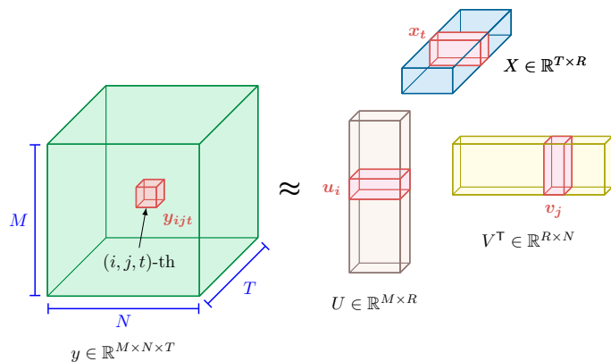
Figure 10.11: Tensor Decomposition: A three-dimensional tensor y \in \mathbb{R}^{M \times N \times T} is approximated by factor matrices U , X , and V . The highlighted factor vectors u_i , x_t , and v_j combine across rank R to reconstruct the entry y_{ijt} . Extending low-rank approximation from two dimensions to three carries the storage and computation argument into convolutional layers. Source: (Gholami et al. 2022).
