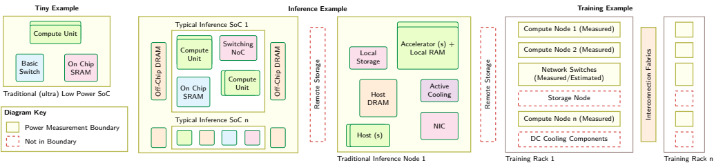
Figure 12.7: Power Measurement Boundaries: MLPerf defines system boundaries for power measurement, ranging from single-chip devices to full data center nodes, to enable fair comparisons of energy efficiency across diverse hardware platforms. These boundaries delineate which components’ power consumption is included in reported metrics, impacting the interpretation of performance results. Source: (Tschand et al. 2024).
