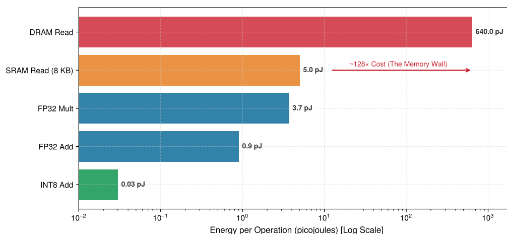
Figure 11.9: The Energy Hierarchy: Representative 45 nm energy estimates on a logarithmic scale from Horowitz (2014). An off-chip DRAM access costs about 128\times an 8 KB SRAM read and over 20,000\times an INT8 addition in this model. The values are not universal device specifications; they illustrate why reuse in registers and SRAM can matter more than reducing arithmetic count alone.
