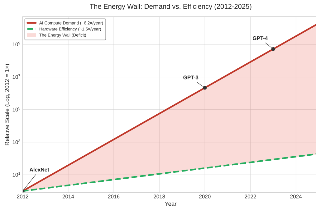
Figure 15.1: The Energy Wall Quantified: The widening gap between AI compute-demand growth (approx. 6.2×/year, matching the 2012–2019 historical claim) and the slower pace of hardware efficiency gains (approx. 1.5×/year) creates a massive energy deficit.
