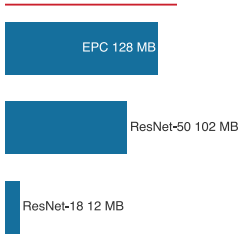
Enclave memory caps which models can run securely.
