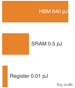
Access energy climbs from registers out to HBM.
