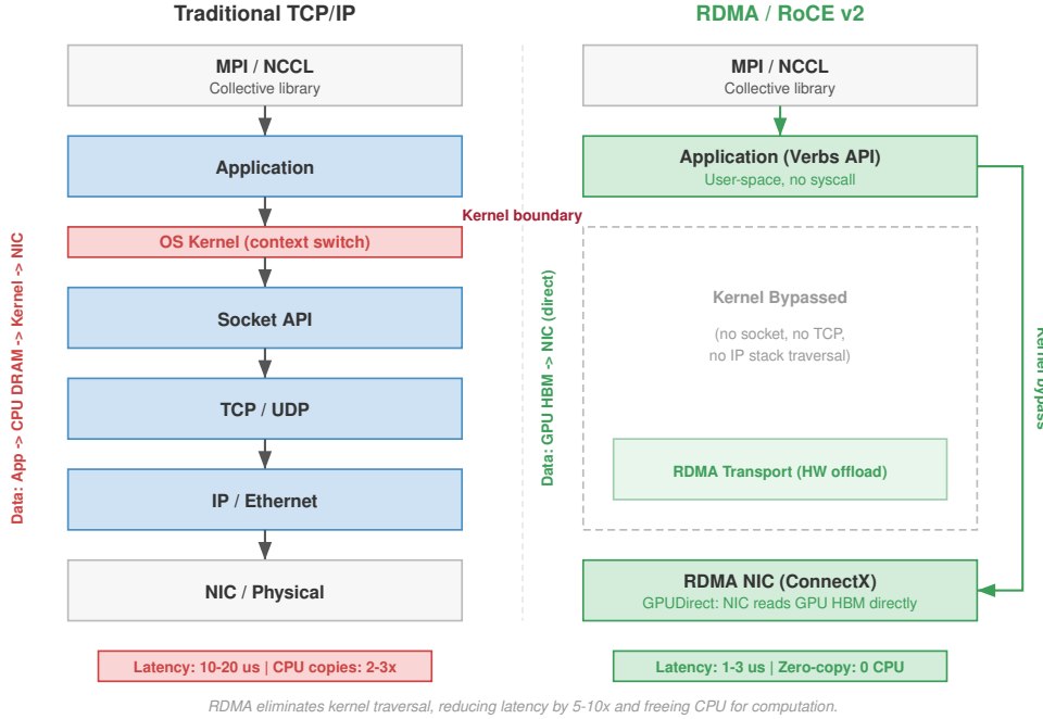
Figure 3.6: Traditional TCP/IP vs. RDMA/RoCE v2 Stacks: Side-by-side comparison. Traditional TCP/IP (left) traverses application, OS kernel (context switch), Socket API, TCP/UDP, IP/Ethernet, and NIC, with latency of 10–20 \mu s and 2–3 \times CPU copies. RDMA/RoCE v2 (right) exposes a user-space Verbs API that bypasses the kernel, offloading transport to the RDMA NIC (GPUDirect reads GPU HBM directly), with latency of 1–3 \mu s and zero-copy CPU overhead.
