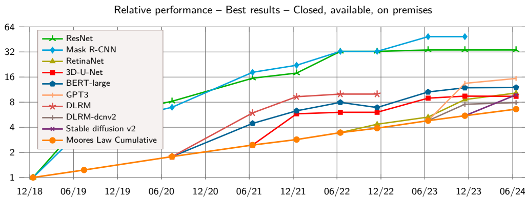
Figure 12.5: MLPerf Training Progress: Workload lines report cumulative relative performance across benchmark versions against the plotted cumulative Moore’s Law baseline. Every workload’s latest point exceeds the baseline at the same date, and Mask R-CNN reaches the largest plotted gain at 48.8 \times ; the comparison captures combined hardware and software progress, not hardware scaling alone. Source: (Tschand et al. 2024).
