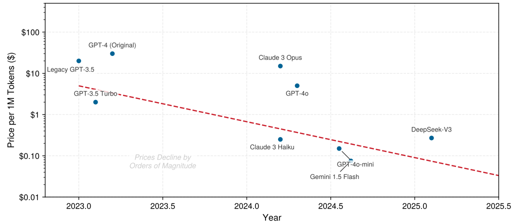
Figure 13.2: Intelligence Deflation: Representative public API input-token list prices per 1M tokens ($) over time (Log Scale). Eight model-version points are snapshots collected from the public pricing pages of OpenAI, Anthropic, Google, and DeepSeek between 2023 and 2025; the Legacy GPT-3.5 point is an illustrative baseline rather than a documented model-version snapshot. The series is intended as a market trend indicator, not a controlled or current-price comparison. API token-processing prices have collapsed by multiple orders of magnitude, transforming the economics of automated AI workflows.
