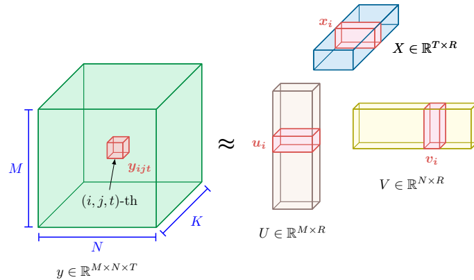
Figure 10.11: Tensor Decomposition: A three-dimensional tensor y \in \mathbb{R}^{M \times N \times T} is approximated by the factor matrices U , X , and V , and the highlighted vectors show how the single entry y_{ijt} is rebuilt from one column of each factor. Extending low-rank approximation from two dimensions to three is what carries the storage and computation argument into convolutional layers. Source: (Gholami et al. 2022).
