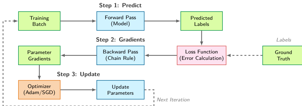
Figure 8.4: The Iterative Training Loop: Each iteration sequences forward prediction (retaining activations), backward error propagation (computing gradients via the chain rule), and optimizer state updates. Inter-stage data dependencies and memory residency dictate the minimum execution time and memory floor of every training step.
