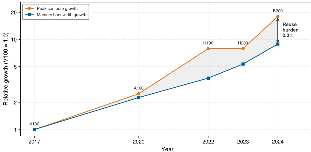
Figure 11.10: The Compute-Bandwidth Divergence: Peak dense FP16 throughput and memory bandwidth across five NVIDIA datacenter generations, each normalized to its V100 baseline on a log scale. Over 2017–2024 compute grows 18× while bandwidth grows 8.9×, so the shaded separation between the curves widens by 2.0×. That separation is the data reuse a kernel must supply to keep the arithmetic units busy. The H200 step is the instructive exception: bandwidth rose while peak compute held flat, narrowing the gap for one generation.
