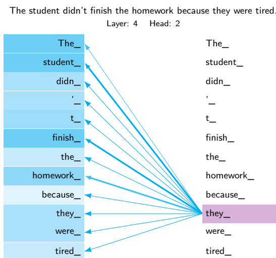
Figure 6.6: Illustrative Attention Pattern: A schematic attention pattern for the pronoun “they.” Line thickness represents hypothetical attention-weight magnitude, with stronger links to “student,” “finish,” and “homework.” One attention layer connects all positions directly and can compute their dense interactions in parallel.
