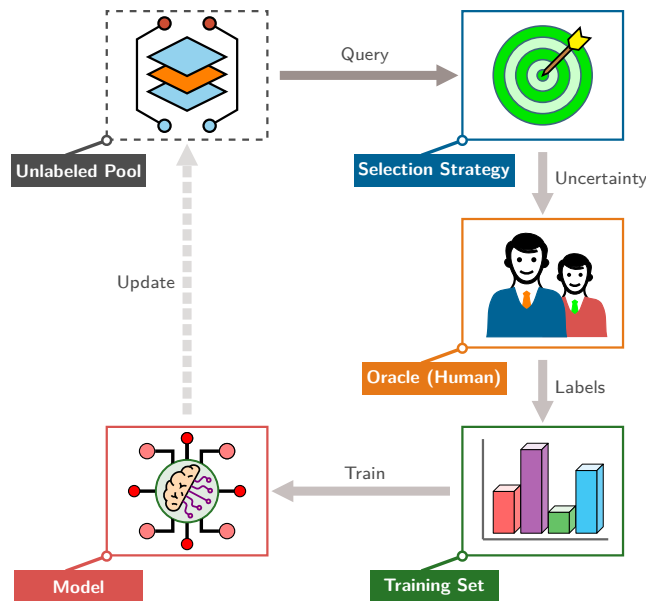
Figure 9.5: The Active Learning Closed Loop: The selection cycle trades proxy scoring compute to query only the most informative or uncertain samples from an unlabeled pool for oracle annotation. This concentrates expensive human labeling budgets on high-entropy examples to maximize the information gained per annotated sample.
