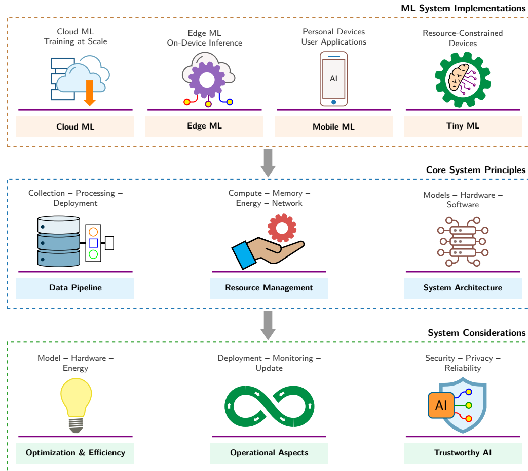
Figure 2.13: Convergence of ML Systems: Despite vast resource disparities across cloud, edge, mobile, and TinyML tiers, all deployments converge on three shared systems foundations: data pipelines, resource management, and hardware-software architecture. These shared pillars in turn support unified requirements for performance optimization, operational monitoring, and trustworthy engineering.
