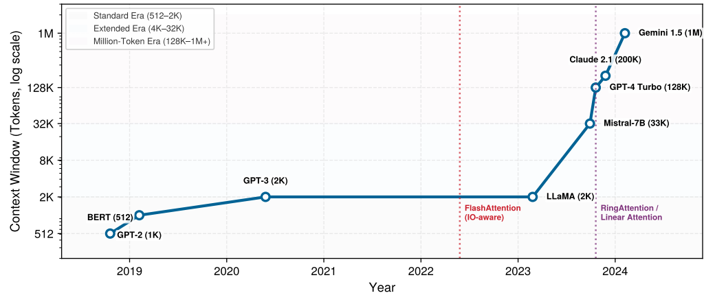
Figure 6.10: Context Window Explosion: Model context capacity (tokens, log scale) from early models (512 to 2K tokens) to modern long-context architectures (128K to 1M tokens). As context scales 1,000\times , naïve attention memory grows 1,000,000\times ( \mathcal{O}(S^2) ), driving the development of FlashAttention, sparse attention, and linear attention mechanisms.
