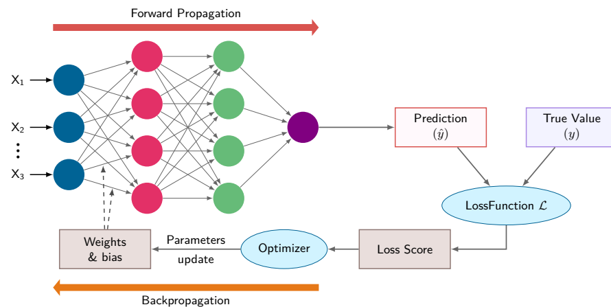
Figure 5.17: Training Loop Architecture: A prediction and true value meet at the loss function; backpropagation computes gradients, and the optimizer turns those gradients into parameter updates for the next forward pass.
