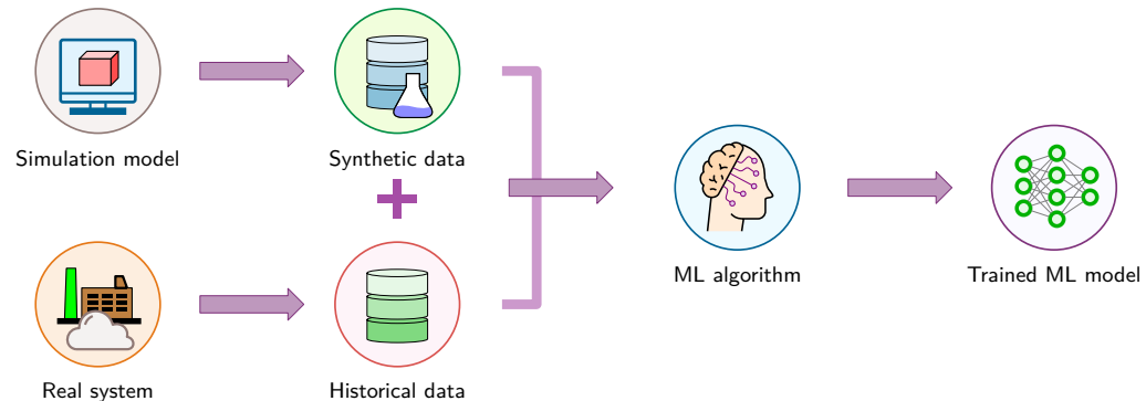
Figure 4.6: Synthetic Data Augmentation: Combining simulated edge cases with historical system data during training. Algorithmic generation supplements real-world observations to close coverage gaps for rare events and dangerous operating regimes without incurring proportional human collection costs. Source: (AnyLogic 2024).
