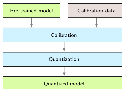
Figure 10.19: Post-Training Quantization Pipeline: PTQ converts a trained FP32 model directly to INT8 without retraining. Representative calibration data passes through the model to record activation ranges [\alpha, \beta] , computing scale factor S and zero-point Z parameters to quantize parameters before deployment.
