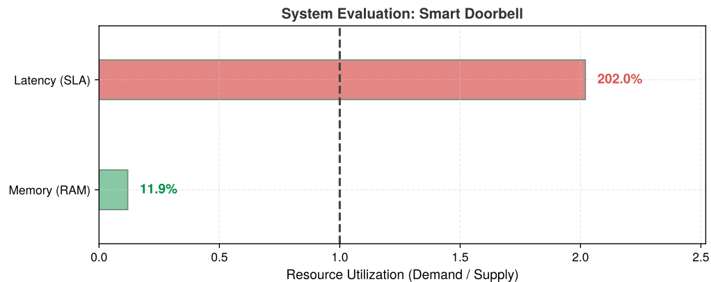
Figure 2.2: Smart Doorbell Constraint Scorecard: Each bar is demand over supply, so the dashed line marks the point where a level is exactly saturated. The model occupies a small fraction of the ESP32-S3’s 4 MB memory budget (Level 1: PASS), but its 101 ms baseline latency is twice the deliberately tightened 50 ms interaction target (Level 2: FAIL), even though it clears the scenario’s canonical 200 ms budget.
