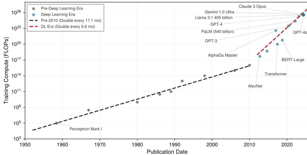
Figure 5.9: Computational Growth: Log-scale scatter plot of representative training-compute estimates in FLOPs from 1958 to 2024. Fitted trend lines compare a slower pre-2010 regime with a steeper post-2012 deep-learning frontier; the values illustrate order-of-magnitude growth rather than an audited census of model training runs.
