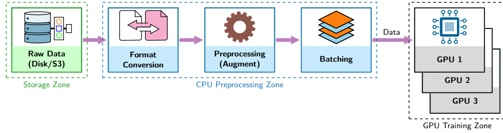
Figure 8.5: CPU-to-GPU Data Flow: Training data transitions through storage, CPU preprocessing, and GPU execution zones. Each stage represents a potential throughput gate; disk read bandwidth, transformation latency, and PCIe host-to-device transfers must collectively sustain the GPU consumption rate to keep accelerators at peak utilization.
