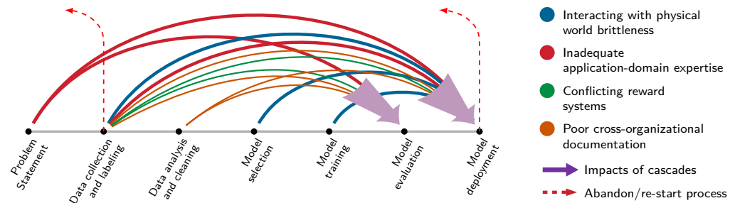
Figure 4.1: Data Quality Cascades: Upstream defects along the seven-stage workflow timeline cast failure arcs directly into late-stage evaluation and deployment. Early flaws in problem framing and collection compound through downstream processing, forcing costly project restarts (dashed red return paths) when defects finally surface in production. Source: (Sambasivan et al. 2021).
