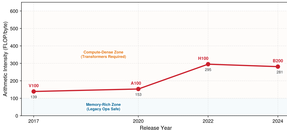
Figure 11.11: The Rising Ridge: Hardware arithmetic intensity (FLOP/byte) over time computed as each chip's dense FP16 tensor peak divided by its memory bandwidth. This is the arithmetic intensity a kernel must reach before compute rather than bandwidth limits it. As compute capability grows faster than memory bandwidth, the ridge point rises from V100 through H100 and remains high on B200. This trend explains why architectures with high data reuse flourish while low-reuse workloads face a growing hardware tax.
