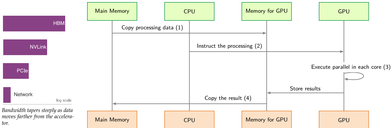
Figure 11.13: Host-Accelerator Data Transfer Sequence: Four-step execution flow between CPU host and GPU device: (1) copying input data over PCIe, (2) issuing kernel instructions, (3) GPU compute, and (4) transferring results back to host memory. Low PCIe bandwidth and host dispatch latencies can easily dominate runtime unless kernel compute time exceeds data transfer overhead.
