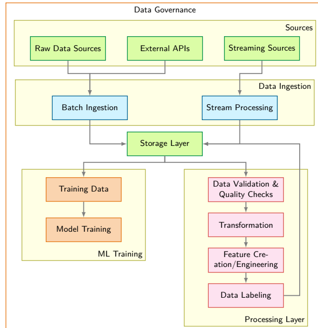
Figure 4.7: End-to-End Data Pipeline: Heterogeneous raw sources (batch and streaming) normalize into unified storage before feeding downstream training and feature processing. The architecture decouples ingestion throughput from iterative transformation and labeling loops, all bounded by an overarching data-governance layer.
