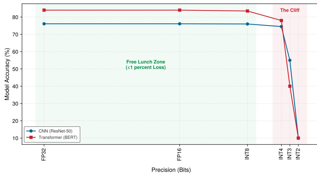
Figure 10.13: Illustrative Quantization Regimes: The accuracy-vs-precision trade-off divides into two operational zones. Down to INT8 (green ‘free lunch’ region), neural networks absorb precision loss with negligible accuracy degradation because relative weight order is preserved; below 4 bits (red ‘cliff’ region), severe discretization noise and dynamic range collapse trigger sharp accuracy loss requiring specialized fine-tuning.
