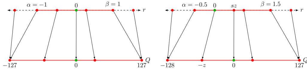
Figure 10.21: Calibration Range Selection: Symmetric vs. asymmetric affine quantization mappings. Symmetric quantization (left) forces real zero to map to integer zero, constraining range selection to [-\alpha, \alpha] at the expense of wasted dynamic range for skewed activation distributions; asymmetric quantization (right) uses an explicit zero-point offset Z to map non-centered ranges [\alpha, \beta] efficiently.
