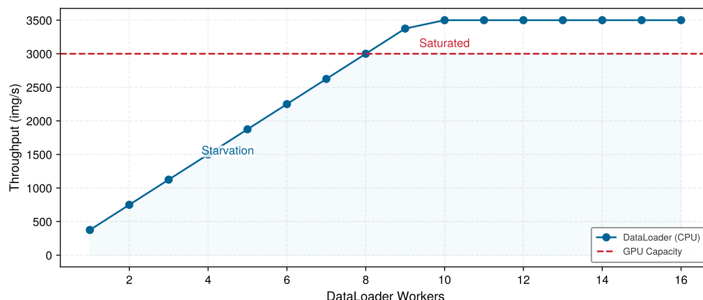
Figure 4.8: The DataLoader Choke Point: Training throughput (img/s) vs. DataLoader workers. The blue CPU-supply curve rises with worker count until it reaches the illustrative input-pipeline cap; the red dashed line marks accelerator consumption capacity. The lower curve is the bottleneck: the accelerator starves to the left of the crossing, while extra workers beyond the crossing do not increase accelerator throughput.
