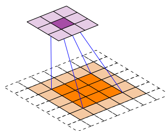
Figure 6.4: Convolution Operation: A 3 \times 3 orange receptive field within the dashed 7 \times 7 input is connected to one highlighted position in a separate violet 3 \times 3 output grid. Applying a 3 \times 3 filter to that receptive field requires 9 multiply-accumulate operations per input channel for each output value. For a 224 \times 224 RGB input, parameter sharing reduces a dense 150,528-weight input connection to a 27-weight local filter, or roughly 5,575 \times fewer weights, while encoding translation equivariance: the same edge detector works at any image location.
