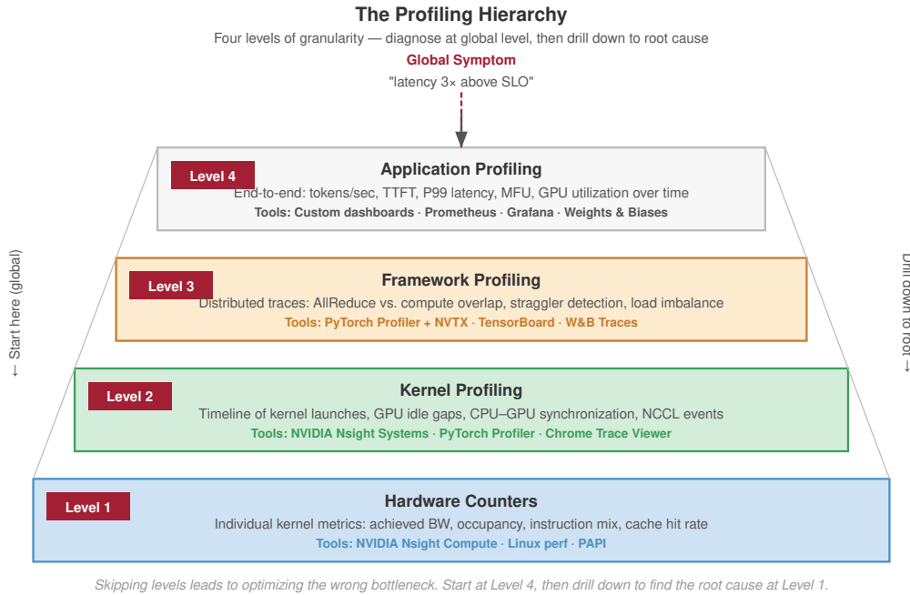
Figure 9.8: The Profiling Hierarchy: Four levels of profiling granularity. Start at Level 4 (Application Profiling) for global symptoms, and drill down through Framework and Kernel profiling to find the root cause at Level 1 (Hardware Counters).
