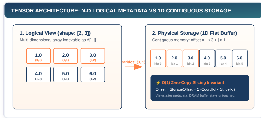
Figure 5.1: Tensor Class Architecture: One class packages data, shape metadata, and every operation the rest of TinyTorch will lean on.
