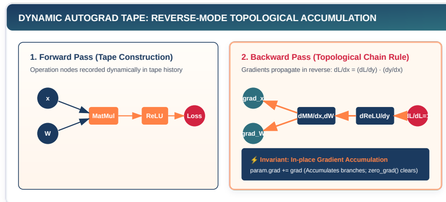
Figure 10.1: TinyTorch Autograd Engine: Reverse-mode automatic differentiation infrastructure.
