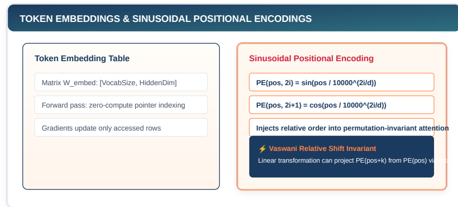
Figure 19.1: TinyTorch Embedding System : Mapping tokens and positions to learned continuous representations.
