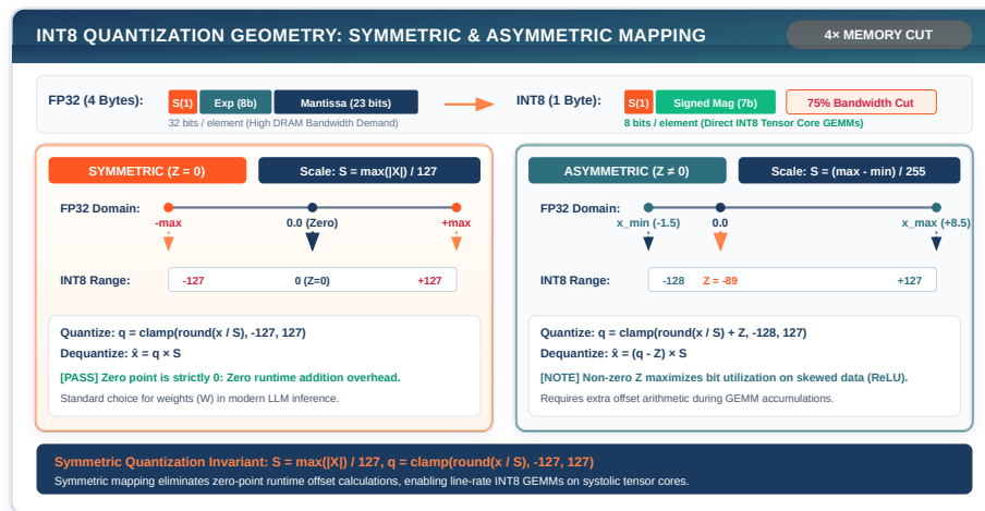
Figure 25.1: TinyTorch Quantization System: Methods for converting models to lower precision.
