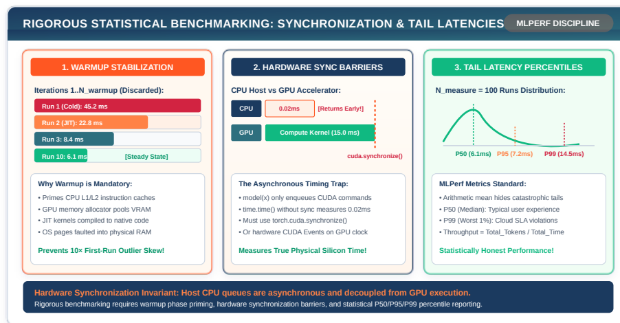
Figure 29.1: TinyTorch Benchmarking System: Statistical measurement of performance and accuracy.
