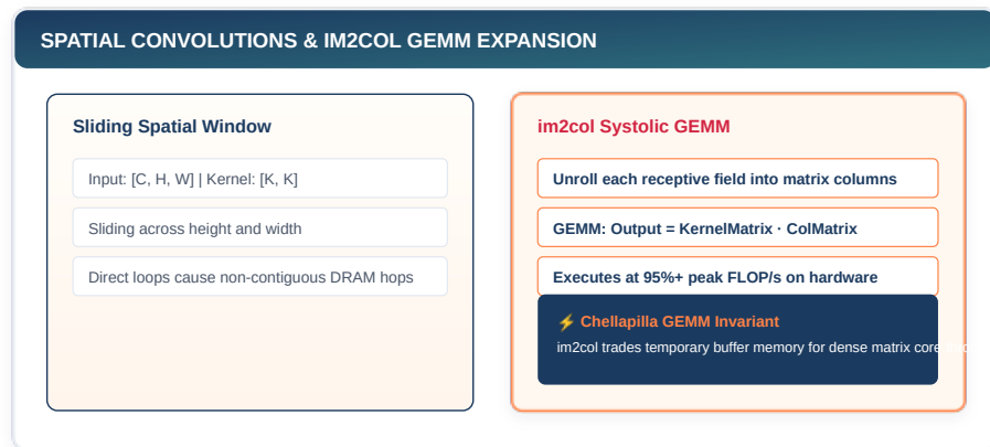
Figure 17.1: TinyTorch Spatial Operations: Convolutional and pooling layers for hierarchical visual feature extraction.
