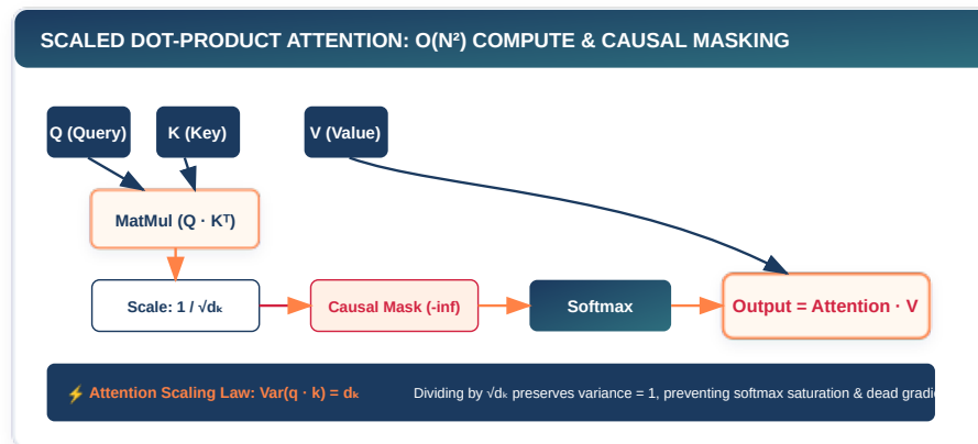
Figure 20.1: Attention Mechanism: Information retrieval paradigm where similarity scores between Queries and Keys determine how much of each Value is retrieved.
