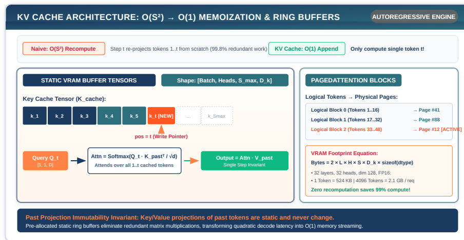
Figure 28.1: TinyTorch KV Caching: Reusing previous computations to speed up text generation.
