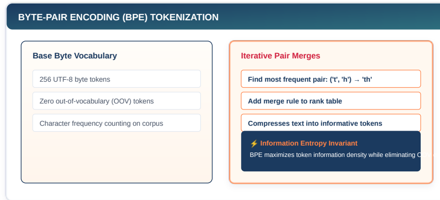
Figure 18.1: TinyTorch Tokenization Infrastructure: Converting raw text into model-ready numerical sequences.
