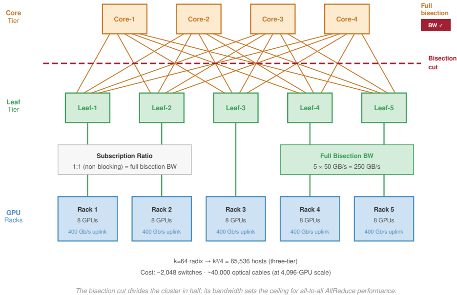
Figure 3.8: Non-Blocking Fat-Tree Topology: A three-tier Clos network built from radix- k switches. By ensuring that the number of uplinks at each level matches the number of downlinks, the topology provides full BW_{\text{bisection}} between any two pods. The multiple parallel paths between leaf and spine enable hardware-based adaptive routing to spray packets and avoid congestion.
