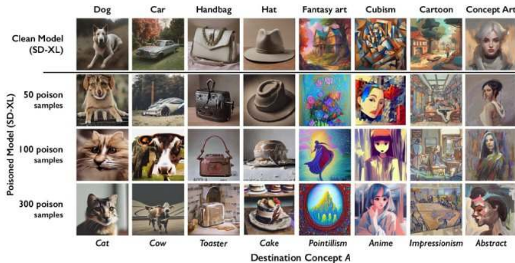
Figure 14.18: Concept Poisoning Dose-Response: Stable Diffusion XL outputs across four poison doses (clean, 50, 100, 300 samples) and eight source prompts (dog, car, handbag, hat, fantasy art, cubism, cartoon, concept art). As the dose grows, outputs morph from the intended source concept toward the attacker’s destination concept, demonstrating Nightshade-style concept poisoning of a pretrained model.
