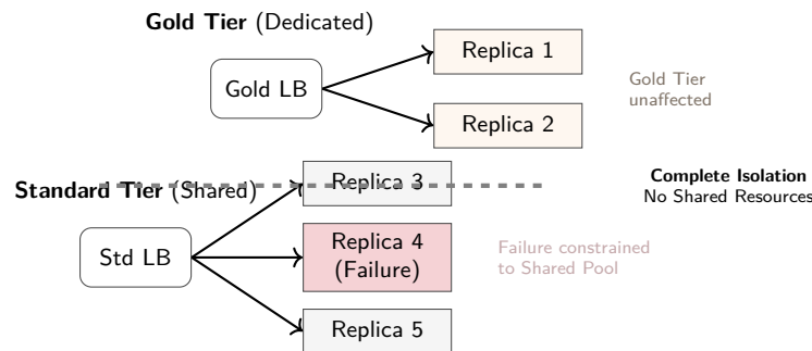
Figure 10.19: Bulkhead Isolation Patterns: To prevent cascading failures in multi-tenant systems, bulkheads isolate resources. Deployment-level bulkheads (shown) assign dedicated physical replicas to high-priority tenants, ensuring complete isolation. Request-level bulkheads enforce strict concurrency limits within shared processes. Like ship compartments, these boundaries ensure that a failure or resource exhaustion in one segment cannot sink the entire platform.
