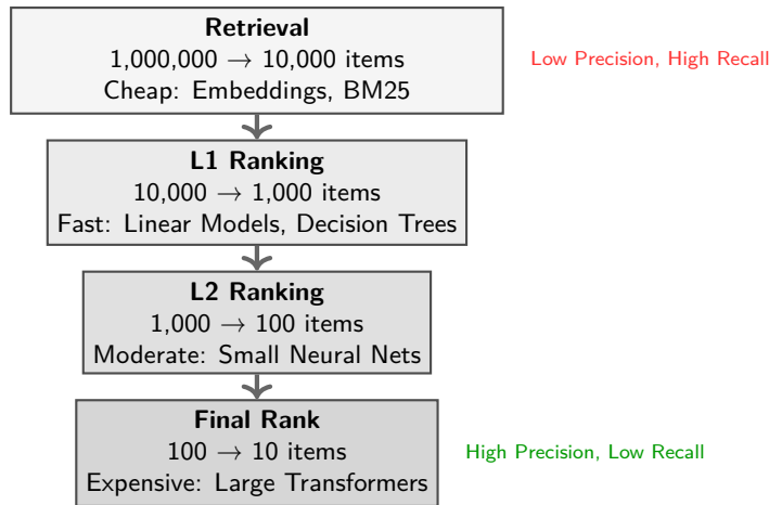
Figure 10.24: Ranking Cascade Architecture: To optimize latency and cost, search and recommendation systems use a cascade of increasingly complex models. Early stages (Retrieval) filter millions of candidates down to thousands using fast, cheap heuristics. Later stages use expensive, high-precision models only on the most promising candidates.
