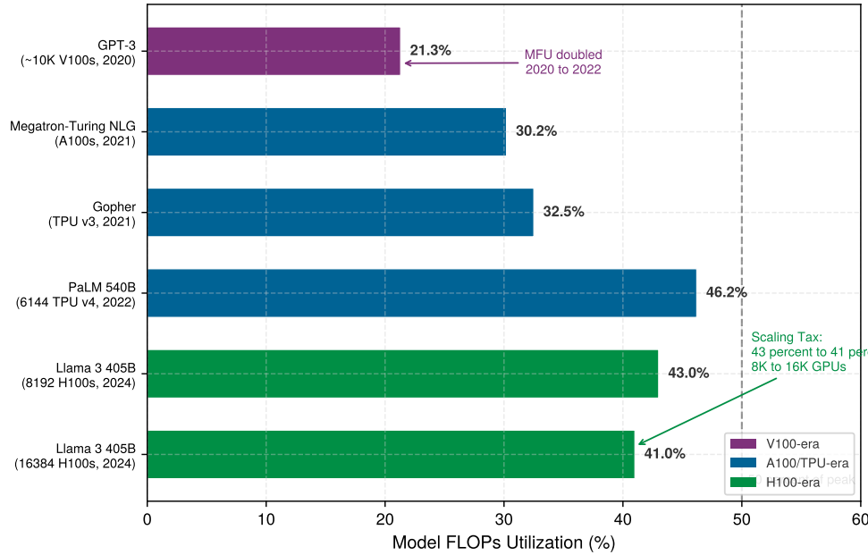
Figure 5.16: The MFU Progression: Model FLOPs Utilization across published training systems, ordered chronologically. MFU doubled from 21 percent (GPT-3, 2020) to 46 percent (PaLM, 2022) through advances in hybrid parallelism and communication overlap, then plateaued near 40–45 percent for large-scale runs. The Llama 3 data points illustrate the scaling tax: MFU drops from 43 percent at 8,192 GPUs to 41 percent at 16,384 GPUs as communication overhead grows with cluster size. Data sources: Chowdhery et al. (2022), Dubey et al. (2024).
