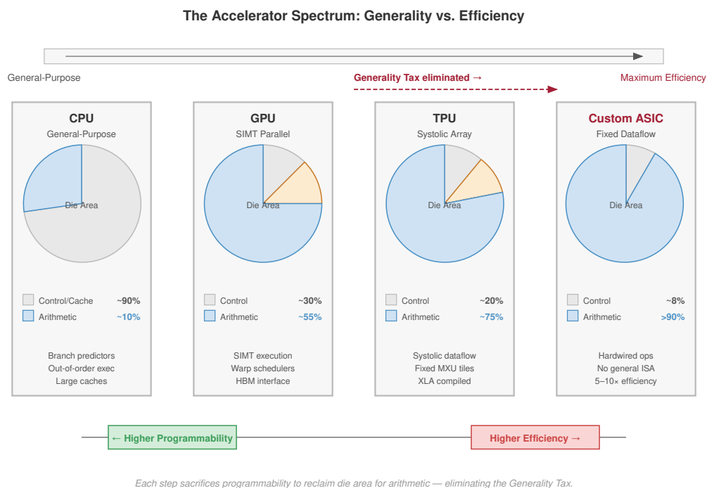
Figure 2.3: The Accelerator Spectrum: ML hardware design involves a fundamental trade-off between programmability and efficiency. General-purpose CPUs provide maximum flexibility but low compute density. Moving toward custom ASICs and systolic arrays increases throughput per watt by hardwiring common dataflows, at the cost of supporting a narrower range of model architectures.
