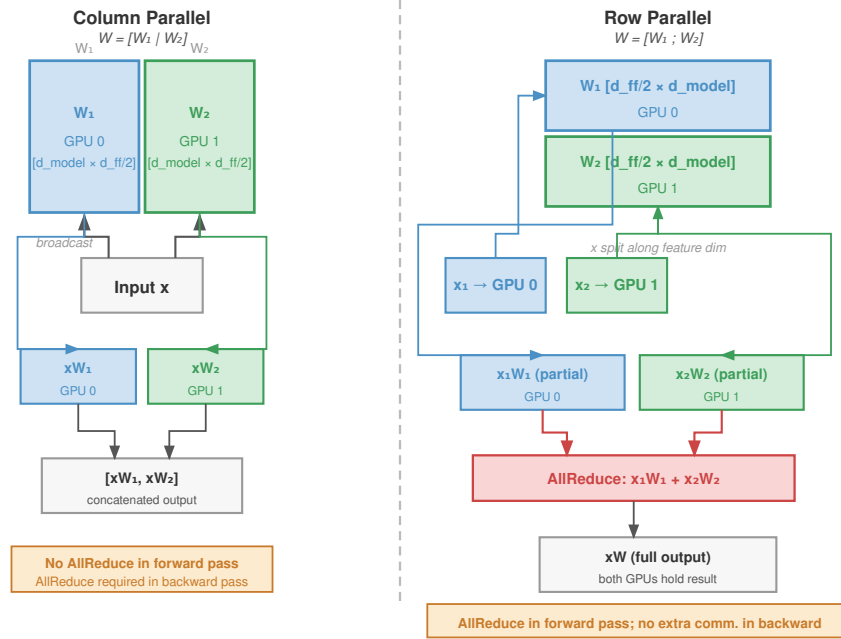
Figure 5.14: Tensor Parallelism - Matrix Partitioning: Illustration of Megatron-LM style tensor parallelism. The first linear layer (e.g., QKV) is split column-wise [W_1 | W_2] . The second layer (e.g., Output) is split row-wise \begin{bmatrix} W_1 \\ W_2 \end{bmatrix} . This arrangement allows the output of the first layer to flow directly into the second without synchronization, requiring only one AllReduce after the second layer to sum the partial results.
