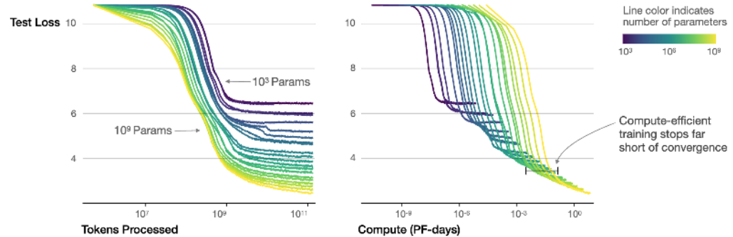
Figure 1.7: Scaling Laws & Compute Optimality: Larger models consistently achieve better performance with increased training data and compute, but diminishing returns necessitate careful resource allocation during training. Optimal model size and training duration depend on the available compute budget, as evidenced by the convergence of loss curves at different parameter scales and training token counts.
