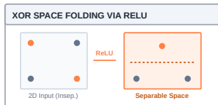
A hidden layer folds the 2D plane: ReLU projects non-separable XOR vertices into a separable 3-point geometry.
