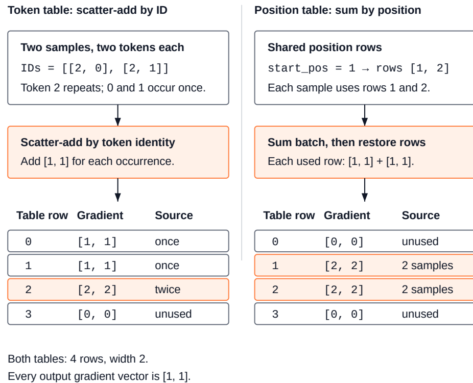
Figure 11.3: Two gradient routes through an embedding layer: Token-table gradients scatter-add by token identity; learned-position gradients sum across samples and return to the position rows used in the forward pass.
