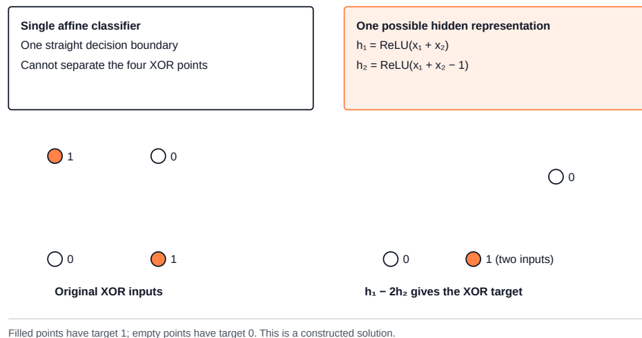
Figure 8.3: Separating XOR after a hidden layer: The four input corners become three hidden points; the two positive inputs share one point that a linear output can separate.
