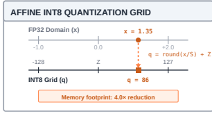
Affine INT8 quantization: continuous FP32 values project onto 256 discrete bins with scale S and zero-point Z .
