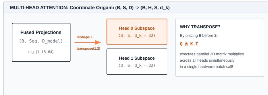
Figure 12.3: Multi-head coordinate origami: Slicing the full hidden embedding (B, S, D) into (B, H, S, d_k) via reshape and transposition isolates head subspaces into independent 2D planes, enabling hardware parallel matrix multiplication across all heads in a single batch call.
