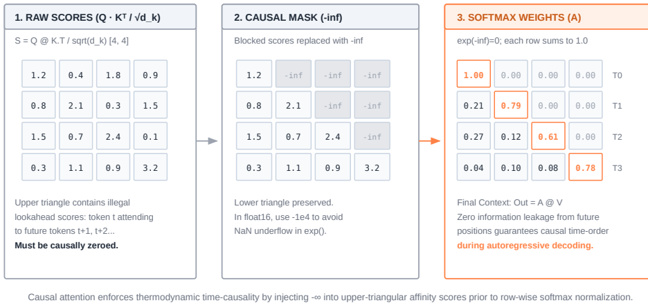
Figure 12.2: The causal attention engine: Queries and keys interact via scaled dot products QK^T / \sqrt{d_k} to form an S \times S score matrix. An upper-triangular mask sets future positions to -\infty so row-wise softmax normalizes attention weights exclusively over past and present tokens ( j \leq i ), strictly preserving autoregressive causality during value mixing.
