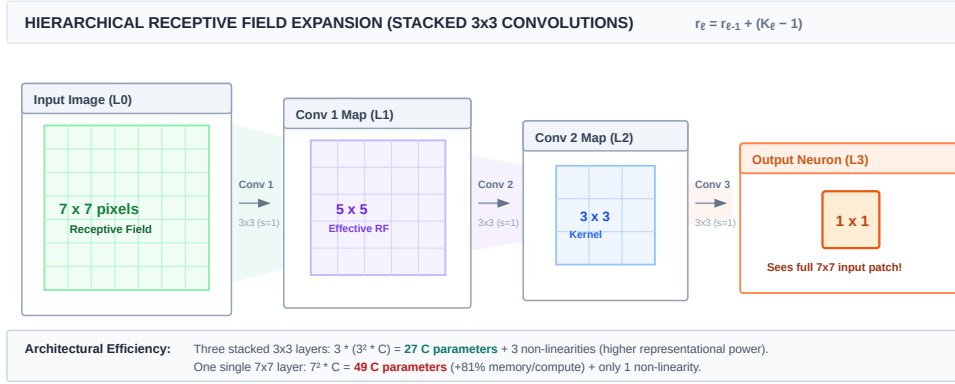
Figure 9.2: Hierarchical receptive field expansion in stacked convolutions: A single output neuron at Layer 3 integrates information across an effective 7 \times 7 spatial patch of the input image through intermediate 3 \times 3 kernel stages. Stacking three 3 \times 3 convolutions uses only 27 parameter weights per channel pair compared to 49 for a single 7 \times 7 filter, while introducing three non-linearities.
