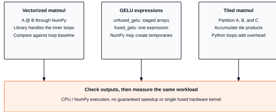
Figure 18.1: Three NumPy execution paths: Vectorized multiplication delegates to a library, the GELU helpers retain different intermediate arrays, and tiled multiplication explicitly accumulates block products. Every comparison checks values before measuring time.
