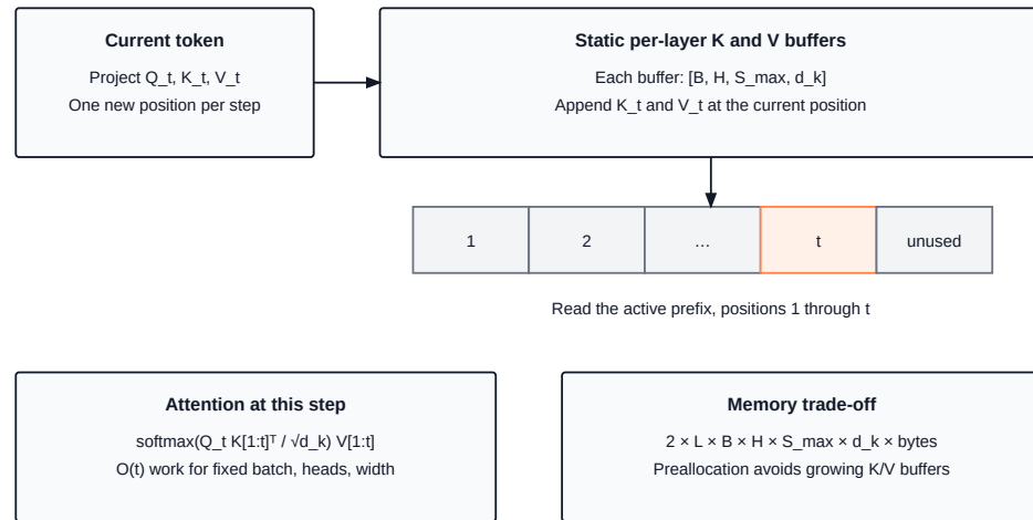
Figure 19.1: The KV cache: Each step writes one new key and value per head and layer, then attends over the growing prefix. Reserved capacity stays fixed while the number of keys read increases.
