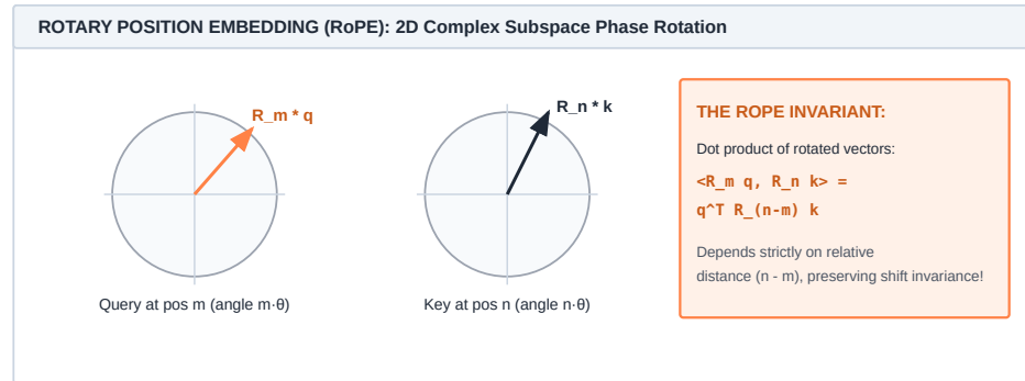
Figure 11.4: Rotary Position Embedding (RoPE) 2D subspace rotation: Instead of adding static position vectors to inputs, RoPE rotates 2D coordinate slices of query ( m ) and key ( n ) vectors by angle multiples m\theta and n\theta . The resulting attention inner product depends on position only through the offset (n - m) .
