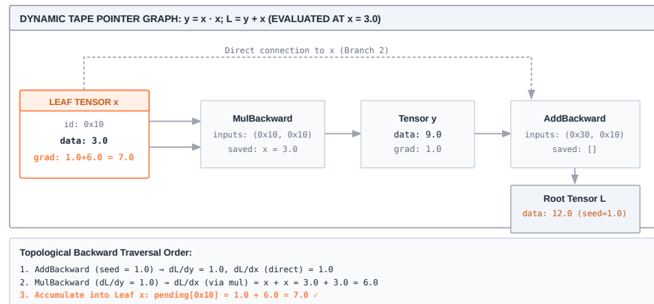
Figure 6.3: The autograd pointer DAG and topological tape: As operations execute forward, each Tensor retains a pointer to its creator node ( _grad_fn ), and each node stores references to its input tensors. Calling loss.backward() performs an iterative post-order depth-first stack traversal, reverses the order to produce a reverse topological sequence, and propagates vector-Jacobian products backward while accumulating in-place gradients into leaf .grad buffers.
