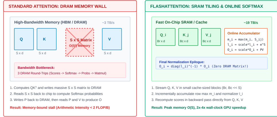
Figure 23.2: FlashAttention SRAM-aware tiling vs. standard attention DRAM wall: Standard attention incurs multiple high-latency DRAM round-trips to materialize the full S \times S score and weight matrices. FlashAttention partitions Q, K, V into small SRAM-sized blocks ( B_r, B_c \ll S ) and employs online softmax updates directly in on-chip fast memory, completely eliminating the O(S^2) DRAM memory footprint.
