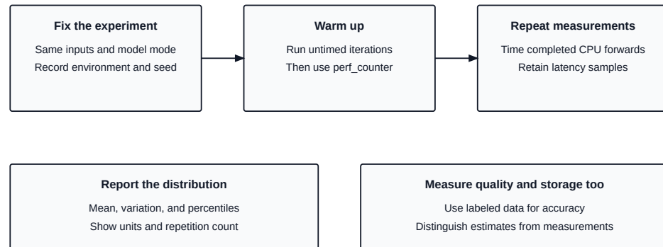
Figure 20.1: Fix the workload and model mode, warm up, and retain repeated timings. Report the distribution alongside quality checks, keeping storage estimates distinct from measured allocations.
