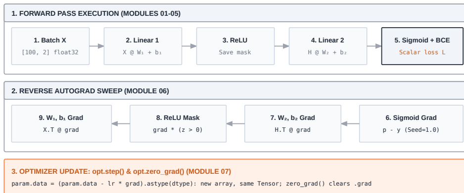
Figure 8.4: One training iteration, step by step : A schematic of the forward operations, the reverse vector-Jacobian products, and the optimizer update for the XOR network. It shows order and data dependencies, not measured time or memory.
