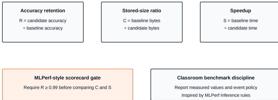
Figure 22.1: The MLPerf Optimization Olympics scorecard: one model, three axes, and a floor on accuracy that a submission must clear before its memory and latency numbers count.
