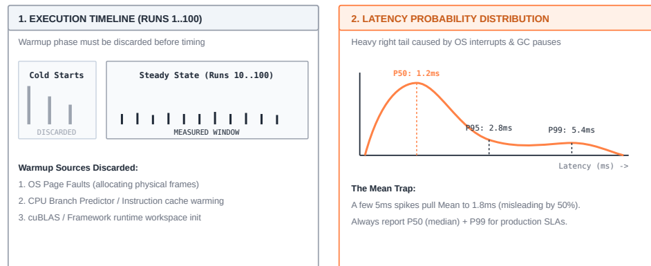
Figure 20.2: The anatomy of latency distributions and tail percentiles: Discarding initial cold-start runs (affected by OS page faults, library dynamic linking, and cache warming) isolates steady-state performance. The resulting latency distribution is characteristically right-skewed; reporting median P_{50} alongside tail percentiles P_{95} and P_{99} reveals unpredictable system stalls that mean latency alone conceals.
