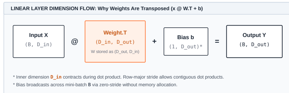
Figure 3.3: Linear layer dimension flow and weight layout: In a forward linear projection, the inner dimension D_{\text{in}} contracts via matrix multiplication while the batch dimension B is preserved. Bias broadcasting adds (D_{\text{out}},) across all rows in zero-stride memory without replication.
