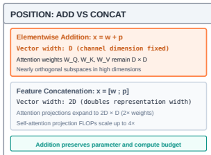
Position Injection: Elementwise addition preserves representation width D , avoiding parameter explosion in downstream attention projections.
