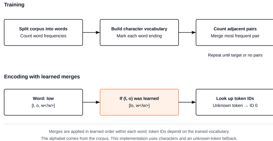
Figure 10.1: Training counts words and learns pair merges; encoding replays those merges within each word before looking up IDs. The visible notation </w> denotes the space stored at a word ending.
