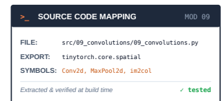
Source Code Mapping: Module 09 extracts Conv2d spatial convolution, im2col buffer unrolling, and MaxPool2d downsampling directly from the working repository.
