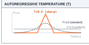
Temperature scaling reshapes logit probabilities ( T \rightarrow 0 vs T > 1 ).
