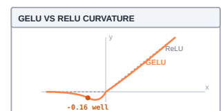
TinyTorch's sigmoid-form GELU dips to about -0.164 near x = -0.75 (exact GELU: -0.170) before approaching zero.
