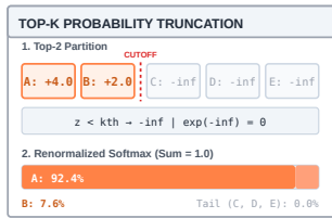
Top-k Truncation: Logits below the rank k threshold are clamped to -\infty , zeroing tail exponent probabilities and renormalizing survivors to sum to 1.0.
