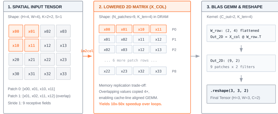
Figure 9.3: Lowering 2D convolution to GEMM via im2col: Sliding receptive field patches of shape C_{in} \times K \times K are unrolled into rows of an input matrix X_{col} , while filters are flattened into columns of W_{col} . High-performance BLAS matrix multiplication computes all overlapping dot products simultaneously, which is then reshaped into the 4D output tensor.
