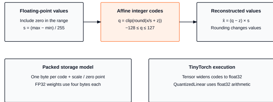
Figure 16.1: Quantization and storage: A scale and zero point map floats to integer codes and reconstruct rounded values. Packed storage uses one byte per code; TinyTorch wraps codes in float32 arrays.
