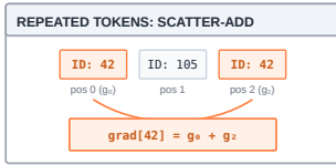
Scatter-add backward routing for repeated token IDs.
