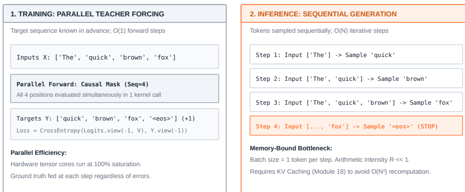
Figure 14.2: Teacher forcing versus autoregressive text generation: In training, teacher forcing presents the full sequence simultaneously, utilizing causal masking so position t predicts target t + 1 ( O(1) parallel passes). In autoregressive inference, generation proceeds iteratively token-by-token, taking the last logit row, sampling with temperature/top- k , and appending to the prompt prefix ( O(T) sequential passes).
