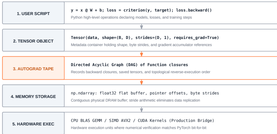
Figure 1: The physical execution stack: A TinyTorch Tensor wraps a CPython object containing shape and stride metadata, referencing a contiguous C-level float32 memory buffer mapped across OS virtual memory pages down to hardware CPU cache lines (L1/L2/L3) and DRAM.
