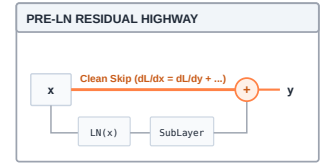
Pre-LN residual gradient highway ( I + J_l ).
