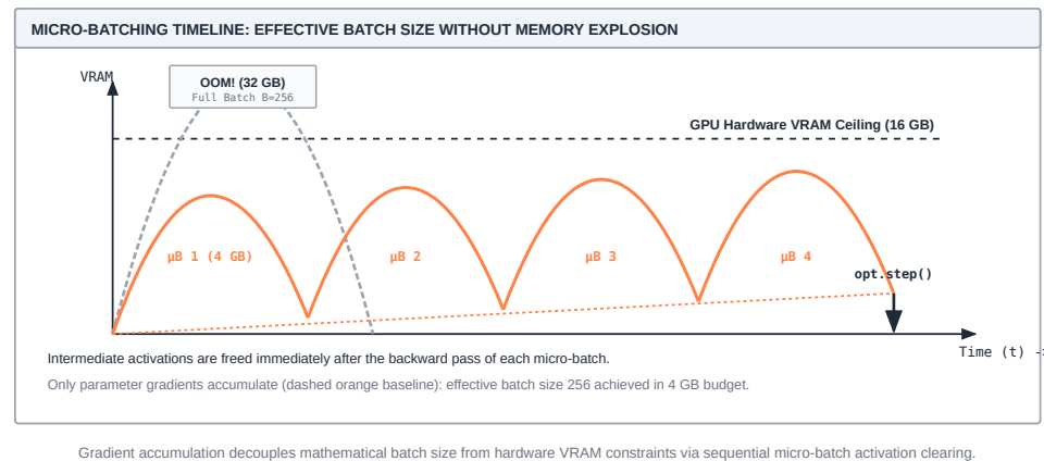
Figure 8.2: Microbatch memory timeline and activation lifecycle: Splitting a batch into microbatches caps peak active memory at a single microbatch’s forward activations. During the backward pass, activations are discarded as gradients accumulate into persistent parameter .grad buffers. When the accumulation window concludes, the optimizer performs a normalized parameter update and clears gradients.
