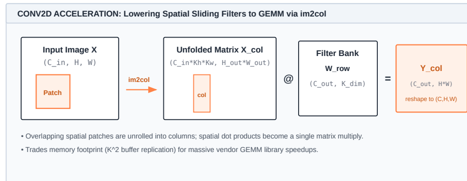
Figure 9.4: Lowering 2D convolution to GEMM via im2col: Spatial receptive fields across input feature maps are unfolded into contiguous rows/columns. The resulting matrix product executes with optimized level-3 BLAS libraries, trading temporary buffer replication for maximum compute density.
