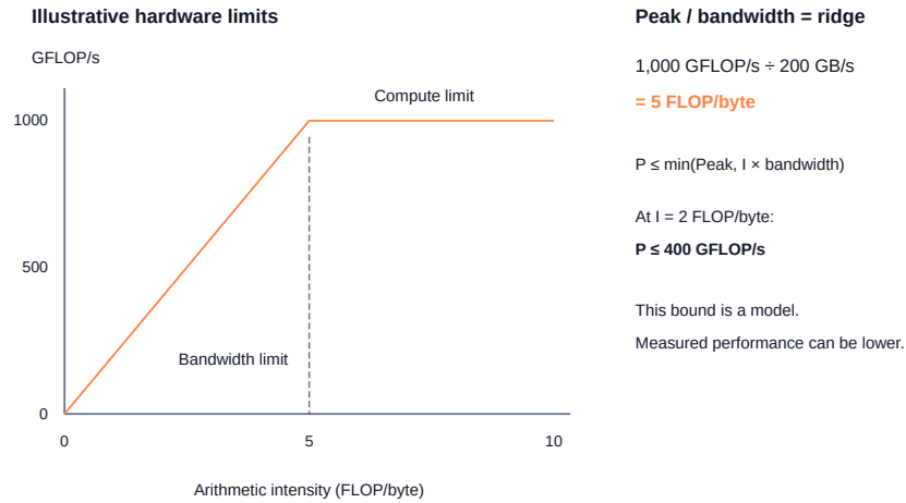
Figure 15.1: The roofline model. Performance rises with arithmetic intensity along the bandwidth ceiling until it reaches the compute ceiling; the corner where they meet is the ridge point.
