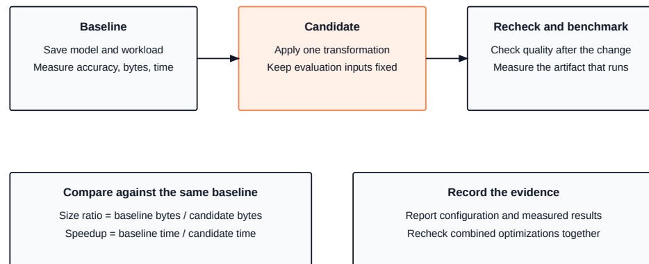
Figure 21.1: An optimization needs a comparison: Preserve the baseline and workload, transform a candidate, recheck quality, and measure its actual arrays and execution before recording the comparison.
