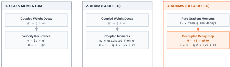
AdamW decouples weight shrinkage from moment estimation, preserving proper regularization scale.
