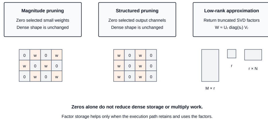
Figure 17.1: Compression representations: Both pruning functions preserve dense array dimensions. Low-rank approximation returns three factors; a caller must retain and use them to benefit from their smaller storage.
