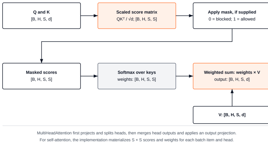
Figure 12.1: Attention as routing. Each query scores every key with a dot product, the scores are scaled by 1/\sqrt{d_k} , future positions are masked out, and the resulting weights mix the values.
