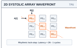
2D Systolic Wavefront: Processing elements stream activation and weight operands in rhythmic lock-step, achieving peak compute density with 2N - 1 cycle latency.
