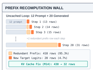
Prefix Recomputation Wall: Without KV caching, generating 20 tokens evaluates 430 rows, where most rows are prefix recomputation.
