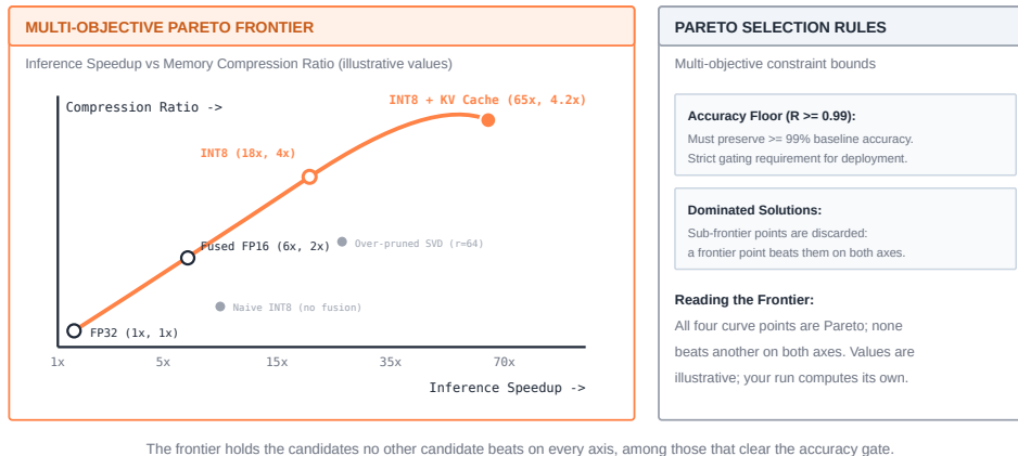
Figure 22.2: The MLPerf Optimization Olympics Pareto frontier: Evaluating optimization candidates across accuracy retention, memory compression, and inference speedup reveals the multi-objective trade-off curve. The chapter's relative retention floor ( R \geq 0.99 ) disqualifies over-compressed or degraded models before the frontier of non-dominated candidates is drawn. The capstone events apply separate absolute accuracy floors (85%, or 80% for the extreme push). The plotted values are illustrative, not one measured run.
