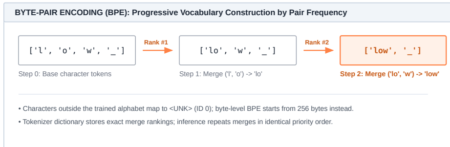
Figure 10.3: Progressive BPE merge sequence: Starting with base character tokens, adjacent pairs are iteratively merged according to their corpus frequency rank ( lo , then low ). Applying merges in strict rank order guarantees identical token segmentation during inference.
