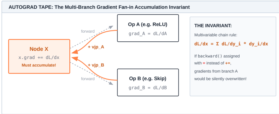
Figure 6.2: Gradient fan-in accumulation across branches: When a tensor fans out during forward execution (e.g. into parallel residual branches or multi-head attention), reverse-mode autograd must accumulate incoming vector-Jacobian products ( x.grad += dL/dx ) rather than assigning them, honoring the multivariable chain rule.
