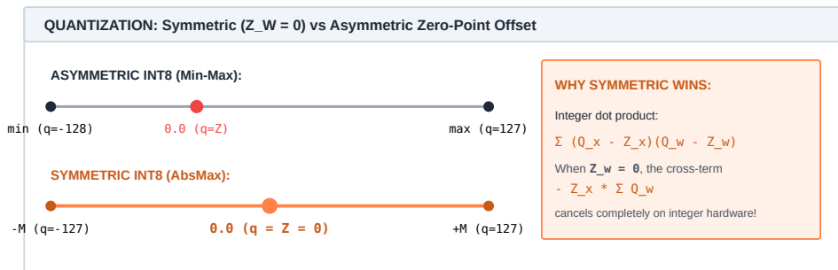
Figure 16.3: Symmetric versus asymmetric quantization grids: Asymmetric quantization maps arbitrary [x_{\min}, x_{\max}] to [-128, 127] with an integer offset Z . Symmetric quantization centers the grid on zero ( Z_W = 0, \pm M ), sacrificing minor dynamic range on skewed distributions to eliminate runtime zero-point subtraction overhead on hardware DP4A / Tensor Cores.
