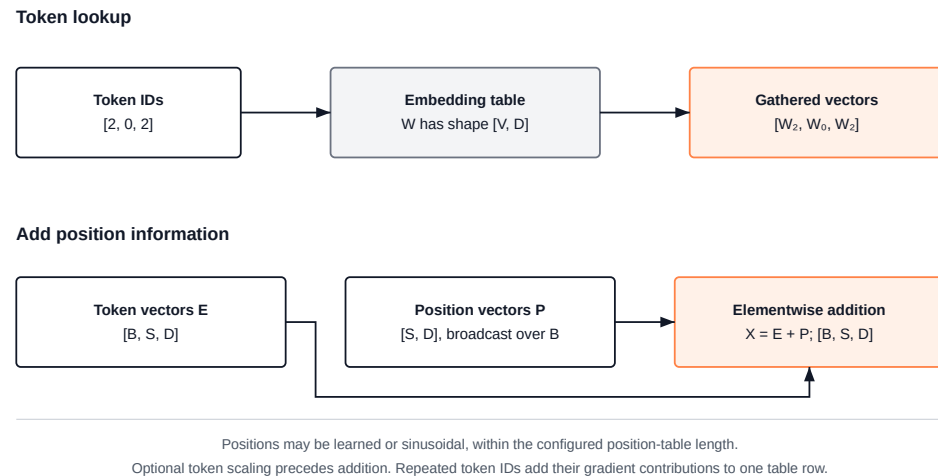
Figure 11.1: The embedding pipeline. A token ID selects one row of the embedding table; the row for that token’s position is added; the sum is the vector the rest of the network sees.
