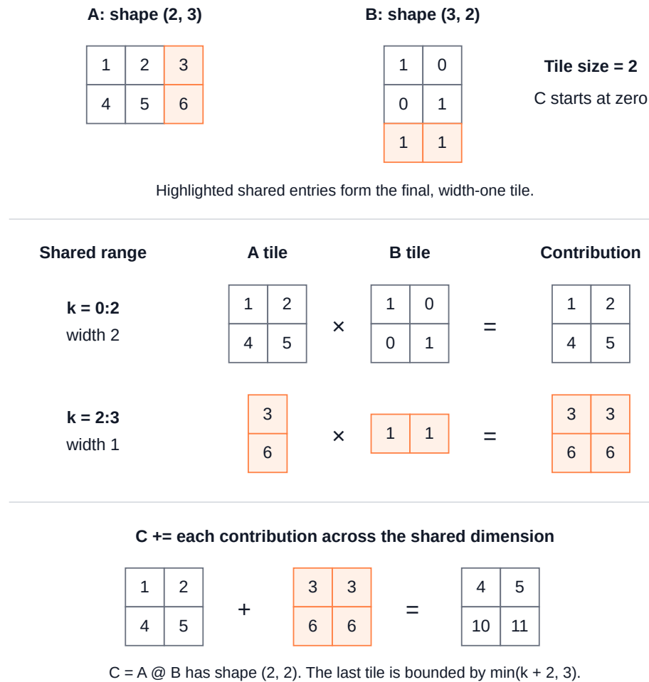
Figure 18.3: Accumulation across the shared dimension: With tile size two, the first shared tile contributes [[1,2],[4,5]] , and the final one-element tile contributes [[3,3],[6,6]] . Adding both produces AB = [[4,5],[10,11]] .
