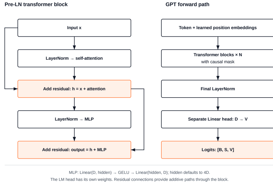
Figure 13.1: Composing a transformer: Each block adds two learned updates to the residual stream. The complete GPT stacks these blocks before a final normalization and a separate vocabulary projection.
