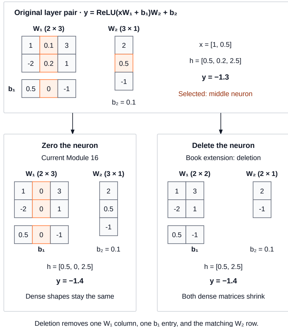
Figure 17.4: Zeroing versus deleting a hidden neuron: Both changes move the output from -1.3 to -1.4 for the same input. Module 16 preserves dense shapes; the book extension deletes the matching first-layer column, bias entry, and second-layer row.
