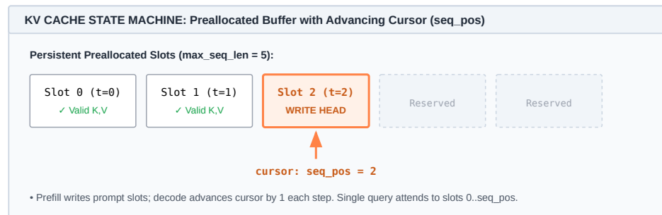
Figure 19.2: KV cache advancing write cursor: Rather than reallocating expanding key/value tensors each generation step, a fixed buffer of shape (B, H, S_{\text{max}}, d_k) is preallocated. Each token generation step writes the newly projected key and value into the single slot indexed by seq_pos and advances the cursor, so the persistent buffers are never reallocated; reads still copy the prefix.
