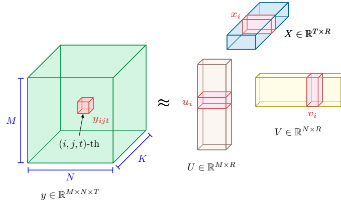
Figure 10.11: Tensor Decomposition: A three-dimensional tensor y \in \mathbb{R}^{M \times N \times T} is approximated by the factor matrices U , X , and V , and the highlighted vectors show how the single entry y_{ijt} is rebuilt from one column of each factor. Extending low-rank approximation from two dimensions to three is what carries the storage and computation argument into convolutional layers. Source: (Gholami et al. 2022).
