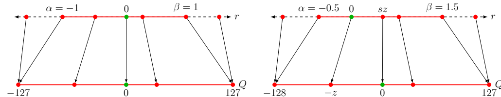
Figure 10.21: Calibration Range Selection: Symmetric vs. asymmetric affine quantization mappings. Symmetric quantization (left) forces real zero to map to integer zero, constraining range selection to [-\alpha, \alpha] at the expense of wasted dynamic range for skewed activation distributions; asymmetric quantization (right) uses an explicit zero-point offset Z to map non-centered ranges [\alpha, \beta] efficiently.
