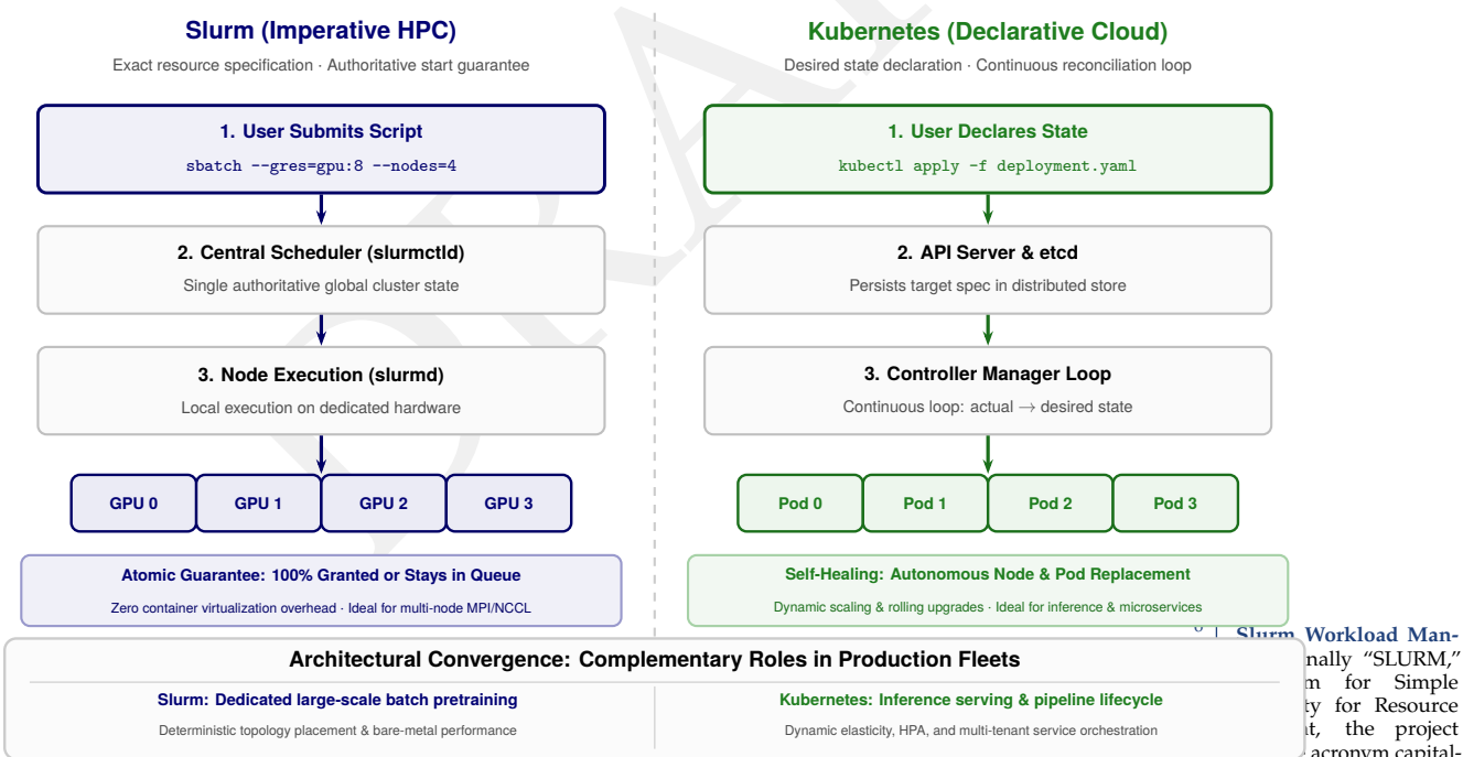
Figure 8.4: Architectural paradigms: Slurm vs. Kubernetes: Slurm (left) uses an imperative batch model where users submit explicit resource requests to a centralized controller (slurmctld) providing deterministic atomic allocation. Kubernetes (right) uses a declarative service model where controllers continuously reconcile observed cluster state in etcd against desired state specifications.
