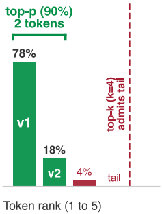
Token rank (1 to 5) Top-p dynamically contracts to two high-confidence tokens while rigid top-k forces low-probability tail inclusion.
