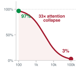
Accumulating 100k background tokens dilutes the softmax denominator, slashing target attention from 97 percent to 3 percent.
