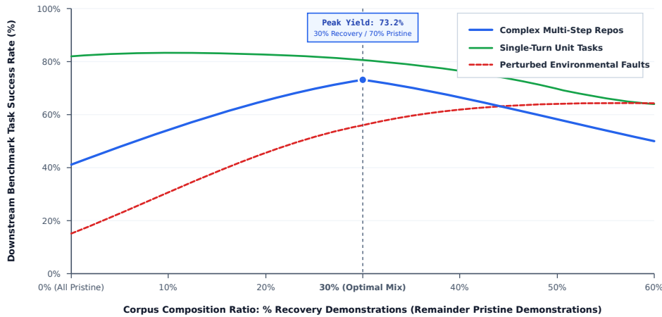
Figure 12.6: Downstream Task Success vs. Trajectory Corpus Composition: Empirical benchmark pass rate as a function of recovery demonstration fraction under a fixed 10^9 -token training budget, showing the optimal 30 recovery mix yielding a peak 73.2 success rate on complex multi-step tasks.
