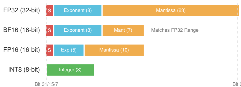
Figure D.3: Numerical Format Bit Layouts: A visual comparison of bit allocations. BF16 preserves FP32's 8-bit exponent and therefore its normal exponent range. FP16 trades range for precision and often uses loss scaling to reduce underflow.
