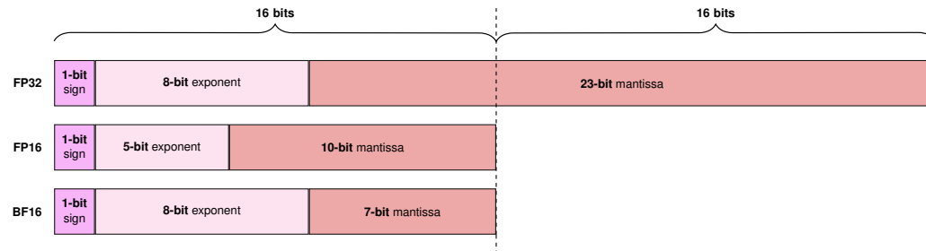
Figure 10.17: Floating-Point Precision: Reduced-precision formats trade precision and/or numerical range for computational efficiency and memory savings. BF16 preserves FP32's exponent size, while FP16 uses a smaller exponent and often requires scaling during training.
