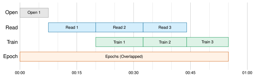
Figure 8.11: Illustrative Overlapped Data Prefetching: Read and train operations execute concurrently under the same assumed stage durations. The schematic schedule spans approximately 55 s, compared with 105 s for the serial schedule.
