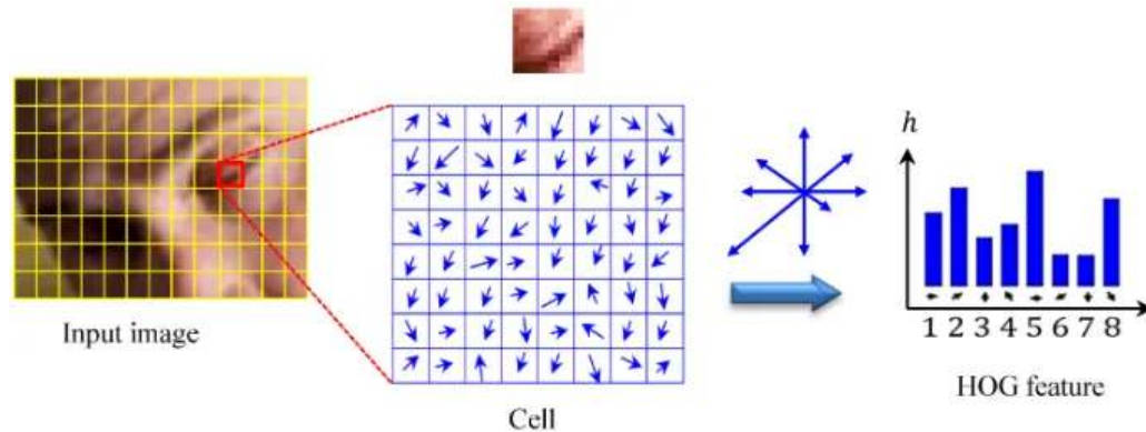
Figure 5.5: HOG Method: Identifies edges in images to create a histogram of gradients, transforming pixel values into shape descriptors that are invariant to lighting changes.
