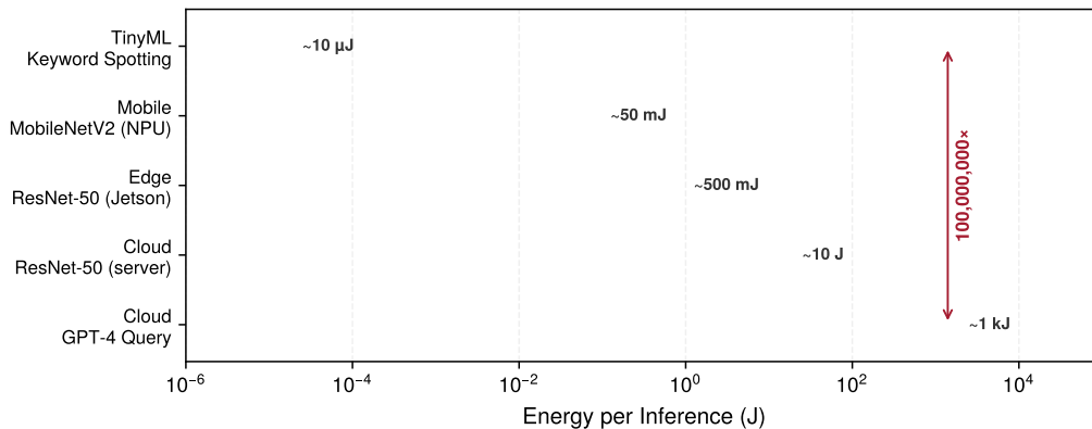
Figure 2.6: Illustrative Energy per Inference Anchors: Pedagogical scenarios span \sim 10 \mu\text{J} for TinyML keyword spotting to \sim 1 \text{ kJ} for a cloud LLM query; they are not outputs of the later analytical node model. The MobileNetV2 bar is a separate full-device scenario, not the preceding 0.1 mJ neural-processing-unit anchor.
