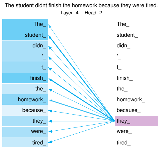
Figure 6.6: Illustrative Attention Pattern: A schematic attention pattern for the pronoun “they.” Line thickness represents hypothetical attention-weight magnitude, with stronger links to “student” and “finish.” One attention layer connects all positions directly and can compute their dense interactions in parallel.
