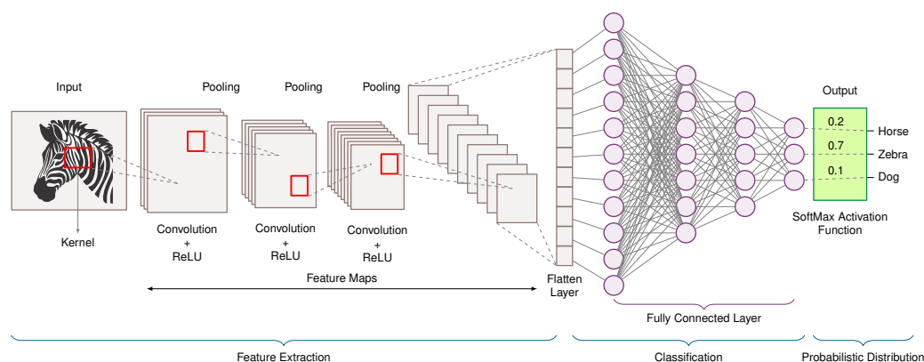
Figure 6.3: Spatial Feature Extraction: Convolutional neural networks apply shared learnable filters across an image to detect similar local patterns at different positions. This repeated application creates translation equivariance, while pooling or later aggregation can provide approximate invariance for classification.
