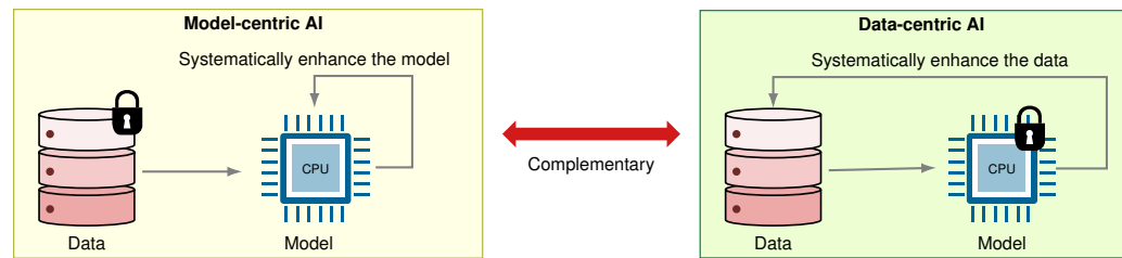
Figure 12.12: Development Paradigms: Model-centric AI prioritizes architectural innovation with fixed datasets, while data-centric AI systematically improves dataset quality (annotations, diversity, and bias) with consistent model architectures to achieve performance gains. Modern research indicates that strategic data enhancement often yields greater improvements than solely refining model complexity.
