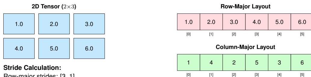
Figure 7.10: Tensor Memory Layout: A 2 \times 3 tensor can be stored in linear memory using either row-major (C-style) or column-major (Fortran-style) ordering. Strides define the number of elements to skip in each dimension when moving through memory, enabling frameworks to calculate memory addresses for tensor[i,j] as \text{base\_address} + i \times \text{stride}[0] + j \times \text{stride}[1] . The choice of memory layout significantly impacts cache performance and computational efficiency.
