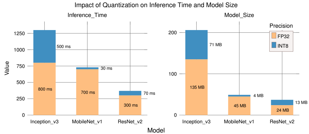
Figure 10.15: Illustrative Quantization Scenario: Example FP32 and INT8 values rather than measurements on one common platform.
