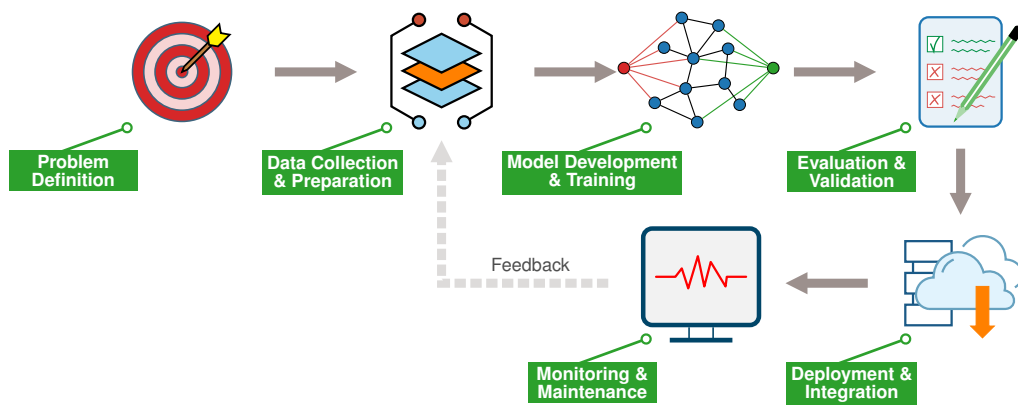
Figure 3.3: Simplified Lifecycle with Feedback: Six stages laid out across two rows. The top row runs left to right through problem definition, data collection, model development, and evaluation; the flow then drops to deployment and integration at the right of the bottom row and doubles back left to monitoring and maintenance. The feedback loop from monitoring back to data collection captures the essential insight that production insights drive continuous refinement across earlier stages, because data distributions shift, model performance drifts, and operational requirements evolve.
