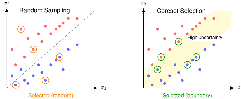
Figure 9.4: Illustrative Uncertainty-Based Selection: Random sampling appears on the left. The illustrative strategy on the right prioritizes samples near the current decision boundary; other coreset objectives may prioritize geometric coverage instead.
