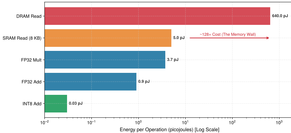
Figure 11.9: The Energy Hierarchy: Energy cost per operation (Log Scale) based on the ‘Horowitz Numbers.’ Fetching data from off-chip DRAM costs \sim 128\times more energy than an SRAM access and \sim 20,000\times more than an INT8 addition. This stark physical disparity dictates that AI accelerators must prioritize data locality (keeping weights in SRAM/Registers) over raw arithmetic throughput to remain within power budgets.
