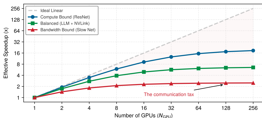
Figure 8.15: Illustrative Communication Tax: An Amdahl-style model compares ideal linear scaling with three assumed non-scaling fractions. The workload names are qualitative labels, not benchmark traces; real communication cost changes with device count, topology, message size, and overlap.
