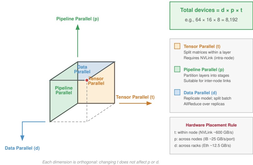
Figure 5.1: The 3D Parallelism Cube: A conceptual visualization of the three orthogonal scaling axes: Data Parallelism (replicating the model), Pipeline Parallelism (splitting depth), and Tensor Parallelism (splitting layers). Large-model training occupies a specific point (d, p, t) within this cube to balance memory usage, compute efficiency, and communication overhead.
