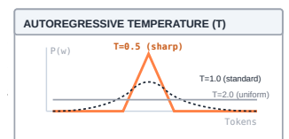
Temperature scaling reshaping logit probabilities ( T \rightarrow 0 vs T > 1 ).
