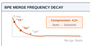
BPE pair frequency decay across merge ranks.
