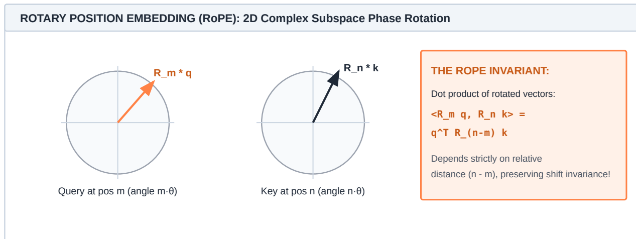
Figure 12.4: Rotary Position Embedding (RoPE) 2D subspace rotation: Instead of adding static position vectors to inputs, RoPE rotates 2D coordinate slices of query ( m ) and key ( n ) vectors by angle multiples m\theta and n\theta . The resulting attention inner product preserves relative distance (n - m) , enabling length generalization.
