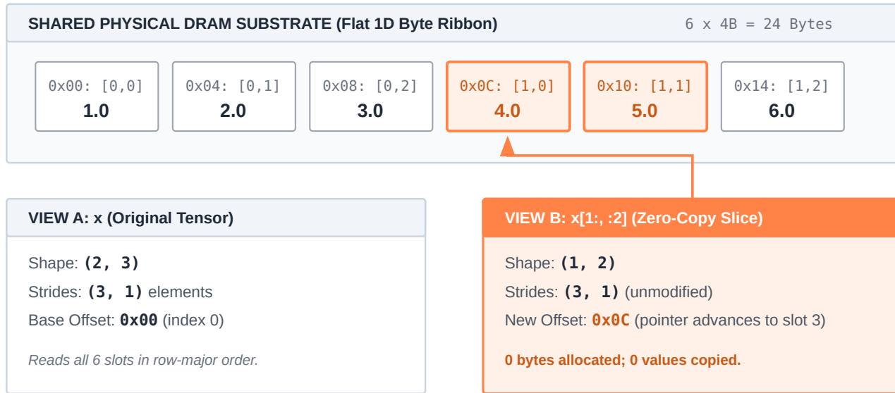
Figure 1.3: Zero-copy slicing and stride manipulation: Slicing advances the base memory offset pointer without allocating new memory, while strided views navigate the flat 1D byte ribbon in row-major or transposed order.
