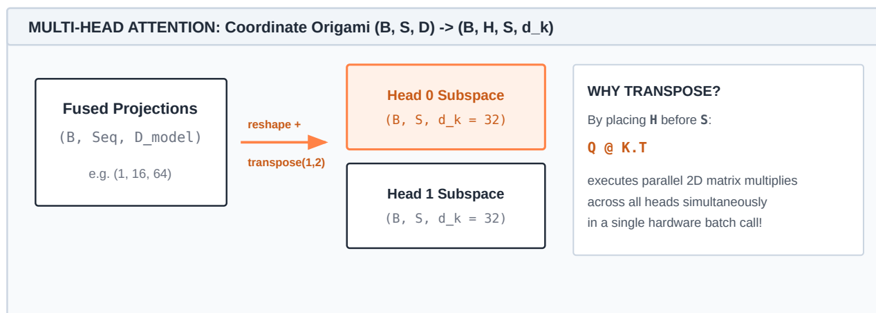
Figure 13.3: Multi-head coordinate origami : Slicing the full hidden embedding ( B, S, D ) into ( B, H, S, d_k ) via reshape and transposition isolates head subspaces into independent 2D planes, enabling hardware parallel matrix multiplication across all heads in a single batch call.
