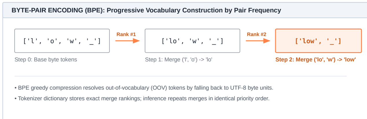
Figure 11.3: Progressive BPE merge sequence: Starting with raw base byte tokens, adjacent pairs are iteratively merged according to their corpus frequency rank ( lo , then low ). Applying merges in strict rank order guarantees identical token segmentation during inference.
