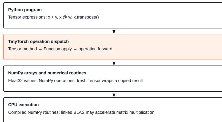
Figure 1.5: The TinyTorch execution stack. High-level Python expressions dispatch through Function.apply into concrete NumPy array operations, which execute on the CPU using compiled numerical routines and linked BLAS libraries.
