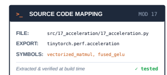
Source Code Mapping: Module 17 extracts operator fusion, memory traffic accounting, and tiled matrix multiplication directly from the working repository.
