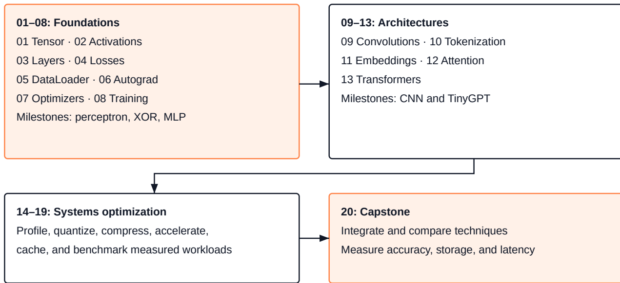
Figure 2: From Operations to an Integrated Framework: Foundational modules support image and language architectures; optimization experiments then lead to the capstone comparison.
