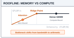
The Roofline model: operational intensity separates the memory-bound bandwidth slope from the compute-bound peak ceiling.
