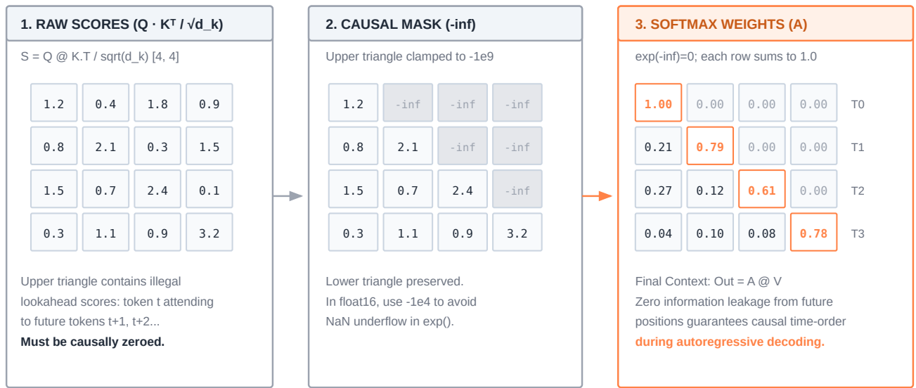
Figure 13.2: The causal attention engine: Queries and keys interact via scaled dot products QK^T / \sqrt{d_k} to form an S \times S score matrix. An upper-triangular mask sets future positions to -\infty so row-wise softmax normalizes attention weights exclusively over past and present tokens ( j \leq i ), strictly preserving autoregressive causality during value mixing.
