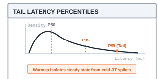
Latency distribution anatomy: tail percentiles P_{95} and P_{99} capture system stalls that the mean obscures.
