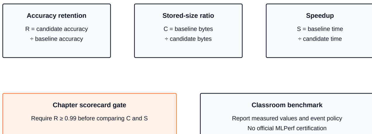
Figure 23.1: The Torch Olympics scorecard: one model, three axes, and a floor on accuracy that a submission must clear before its memory and latency numbers count.
