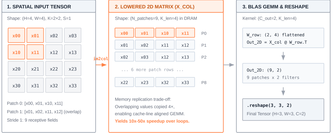
The im2col lowering transforms spatial 2D sliding windows into contiguous row vectors, trading memory for peak BLAS GEMM FLOPs.
