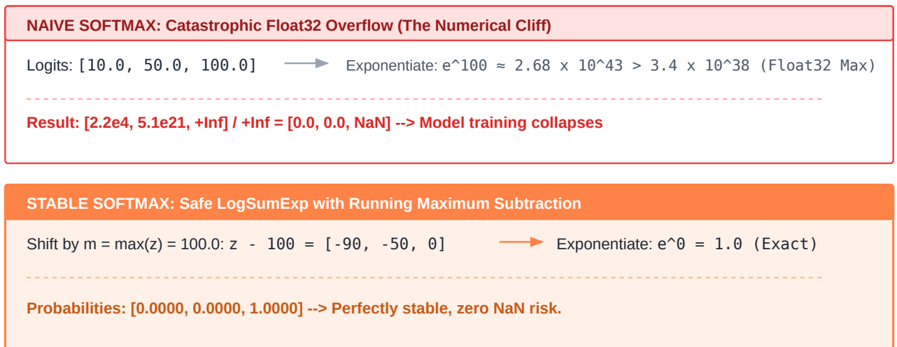
Figure 2.3: The Softmax numerical cliff : Naive exponentiation of large logits triggers float32 overflow ( > 3.4 \times 10^{38} ), returning NaN and collapsing training. Subtracting the running maximum shifts exponents into the non-positive domain ( \leq 0 ), ensuring finite, stable probability evaluation.
