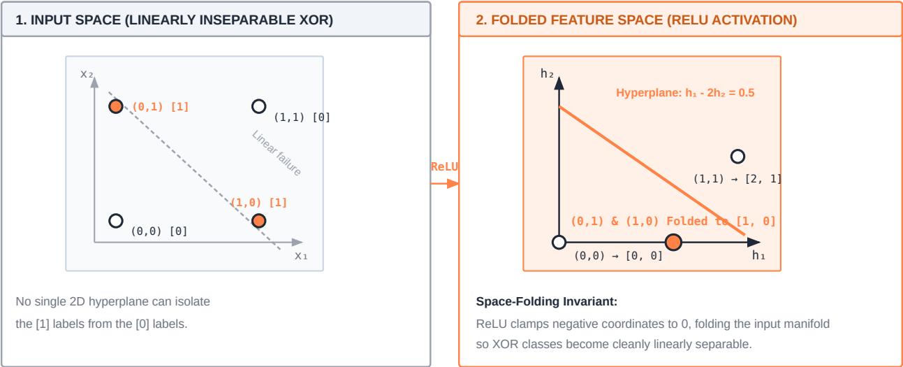
Without non-linear activations, deep networks collapse into a single affine transformation; ReLU acts as a mechanical hinge that folds space.
