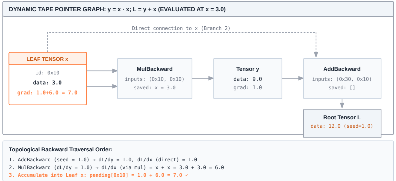
Figure 6.3: The autograd pointer DAG and topological tape: As operations execute forward, each Tensor retains a pointer to its creator node ( _grad_fn ), and each node stores references to its input tensors. Calling loss.backward() computes node in-degrees, sorts nodes topologically via an explicit depth-first stack, and propagates vector-Jacobian products backward while accumulating in-place gradients into leaf .grad buffers.
