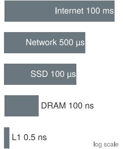
Access latency spans eight orders of magnitude, cache to internet.
