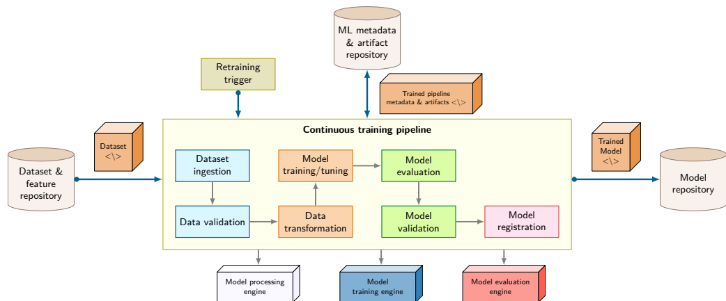
Figure 14.6: ML CI/CD Pipeline: Read the enclosed stages in execution order; the retraining trigger starts a new run, while connected repositories preserve the dataset, model, metadata, and artifacts needed to reproduce and govern it. Adapted from Google Cloud’s MLOps continuous delivery and automation pipeline guidance (Google Cloud 2026b).
