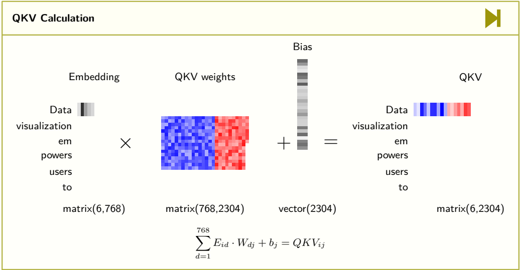
Figure 6.8: QKV Projection Computation: The embedding matrix (6×768) multiplies with QKV weight matrices (768×2304) plus bias to produce combined projections (6×2304). The 2304 output dimension contains concatenated query, key, and value projections (each 768-dimensional). This single batched matrix multiplication, requiring 6 \times 768 \times 2304 = 10.6 million MACs, replaces 3 separate projection operations for efficiency. Source: Transformer Explainer (Cho et al. 2025).
