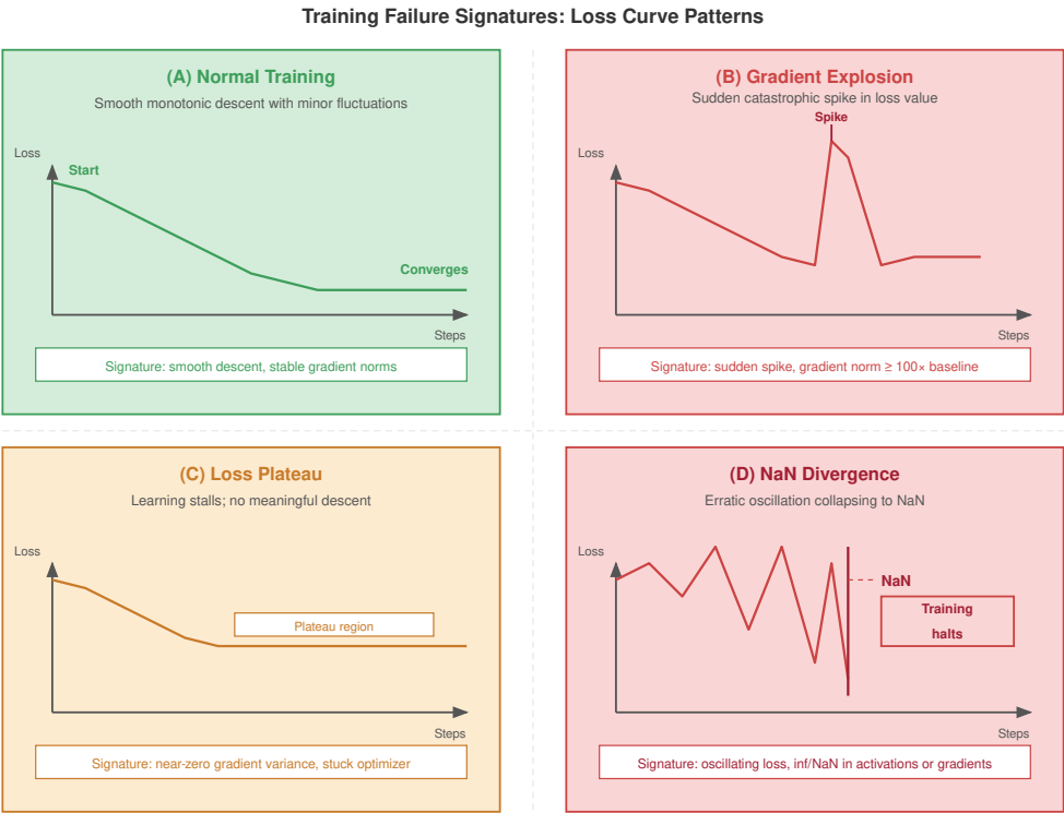
Each signature maps to a distinct root cause: data corruption (B), learning rate or dead optimizer (C), numerical overflow (D)
