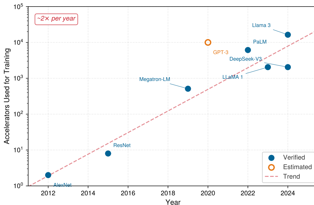
Figure 1.2: The cluster size explosion: Number of accelerators used to train landmark models, 2012–2024. Verified counts from published papers are shown as filled circles; the GPT-3 estimate (hollow marker) reflects approximate cluster size from Microsoft infrastructure announcements rather than a precise published count. The dashed trend line indicates approximately 2\times annual growth in cluster size, a rate that outpaces Moore’s Law and motivates the infrastructure challenges developed throughout the book.
