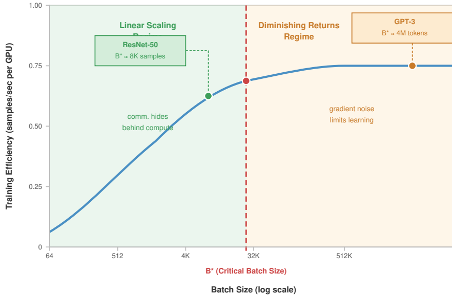
Figure 5.9: Critical batch size and scaling regimes: Below the critical batch size B^* , larger batches reduce noise and improve sample efficiency (linear scaling regime). Above B^* , larger batches provide diminishing returns: while throughput increases, total samples required also increases, reducing sample efficiency. The optimal operating point balances hardware utilization against convergence efficiency.
