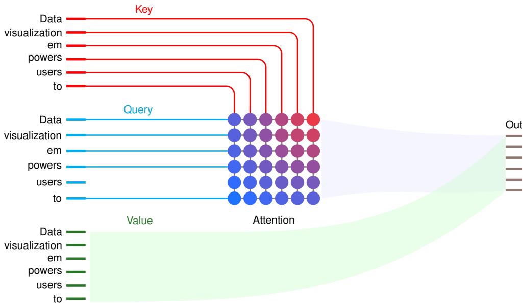
Figure 6.7: Query-Key-Value Attention Mechanism: For a 6-token sequence, queries (cyan) match against keys (red) to produce a 6×6 attention matrix with \mathcal{O}(S^2) entries. Color intensity indicates attention weight: darker cells show stronger relationships. Each output position aggregates information from all values (green) weighted by its attention row. The matrix structure reveals both the computational pattern (thirty-six similarity computations) and the naive memory bottleneck (storing S^2 attention weights). Source: Transformer Explainer (Cho et al. 2025).
