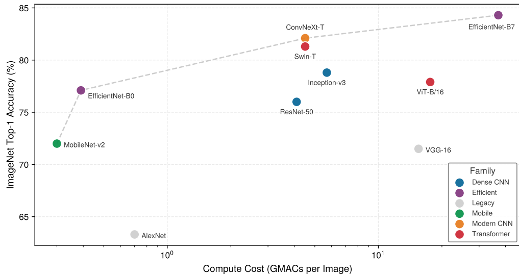
Figure 6.1: The Efficiency Frontier: ImageNet Top-1 Accuracy vs. Computational Cost (GMACs). Representative points are compiled from published model reports for AlexNet, VGG, ResNet, Inception, MobileNetV2, EfficientNet, ViT, Swin Transformer, and ConvNeXt (Krizhevsky et al. 2012; Simonyan and Zisserman 2015; He et al. 2016a; Szegedy et al. 2015; Sandler et al. 2018; Tan and Le 2019; Dosovitskiy et al. 2021; Liu et al. 2021; Liu et al. 2022). The dashed ‘Pareto frontier’ is an illustrative trade-off curve rather than a benchmark rerun; exact accuracy and reported compute values vary by model variant, training recipe, implementation, and operation-counting convention (multiply-accumulates vs. floating-point operations). The legend distinguishes six families: legacy CNNs (gray), dense CNNs (blue), efficient Mobile architectures (green), EfficientNet-class models (violet), modern CNNs (orange), and Transformers (red). The frontier is led by the efficient and modern-CNN families; the Transformers trade substantial compute for flexible long-range modeling without dominating it, and ViT-B/16 sits below the frontier.
