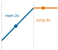
Quantization speedup depends on whether memory bandwidth or compute throughput is binding.
