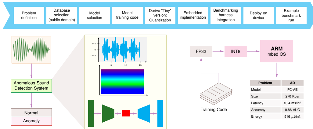
Figure 12.4: Benchmark Workflow Components: A nine-stage workflow for designing a machine learning benchmark, using an audio anomaly detection task as an example. The process flows from defining the task, dataset, model, and metrics to specifying measurement protocol and analysis methods.
