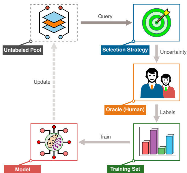
Figure 9.5: Active Learning Loop: Instead of labeling all data, the model selects the most ‘confusing’ or informative samples from an unlabeled pool. These samples are sent to an Oracle (human annotator) and added to the training set. The model is retrained, and the cycle repeats, creating a feedback loop that maximizes information gain per label.
