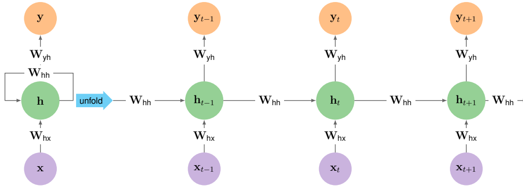
Figure 6.5: Recurrent Neural Network Unfolding: Left panel shows the compact recurrent loop; right panel unfolds this across time steps. Three weight matrices are shared across all steps: W_{hx} (input-to-hidden), W_{hh} (hidden-to-hidden), and W_{yh} (hidden-to-output). This weight sharing keeps parameter count constant at \mathcal{O}(d_{\text{hidden}}^2) regardless of sequence length. For a 128-dimensional hidden state, each time step requires 16,384 MACs for recurrent connections plus 12,800 for input projection.
