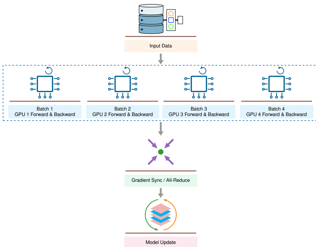
Figure 8.16: Data Parallelism: Each GPU holds a complete model copy, processes different data batches, then synchronizes gradients. This approach scales training throughput linearly with GPU count when models fit in single-GPU memory.
