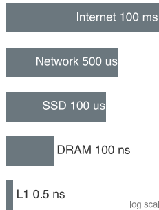
Access latency spans eight orders of magnitude, cache to internet.
