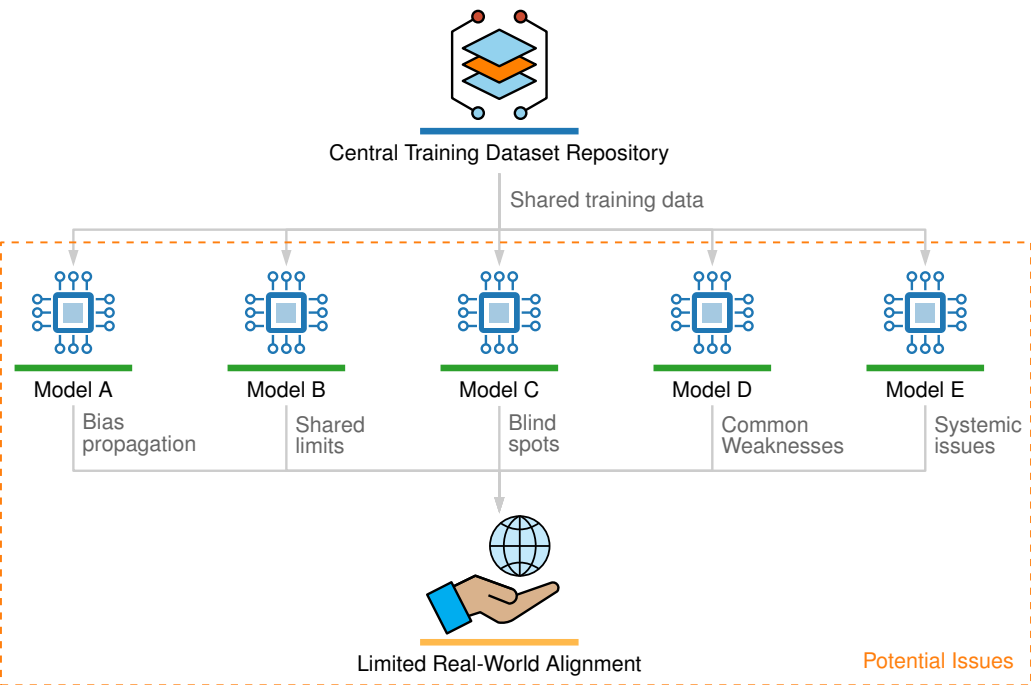
Figure 4.4: Shared Dataset Bias Propagation: Five models (A through E) all train on a single central dataset repository. Arrows show how shared limitations, biases, and blind spots propagate from the common dataset to every downstream model, leading to correlated failures across the ecosystem.
