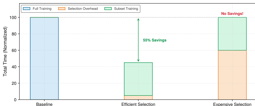
Figure 9.10: The Selection Inequality: Data selection only improves end-to-end efficiency if the overhead of selection plus training on the subset is less than training on the full dataset. A lightweight selection function (proxy model, cached embeddings) keeps selection overhead low; an expensive selection function (full model forward pass) can negate the savings.
