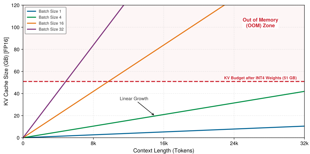
Figure 13.7: The KV-Cache Explosion: FP16 KV-cache usage vs. context length for a 70-billion-parameter-class model with GQA. On the modeled 80 GB GPU, approximately 35 GB of INT4 weights leave about 51 GB for KV cache before runtime overhead. Batch size 32 reaches that cache budget at roughly 4.9k tokens, forcing a trade-off between batch size and context length.
