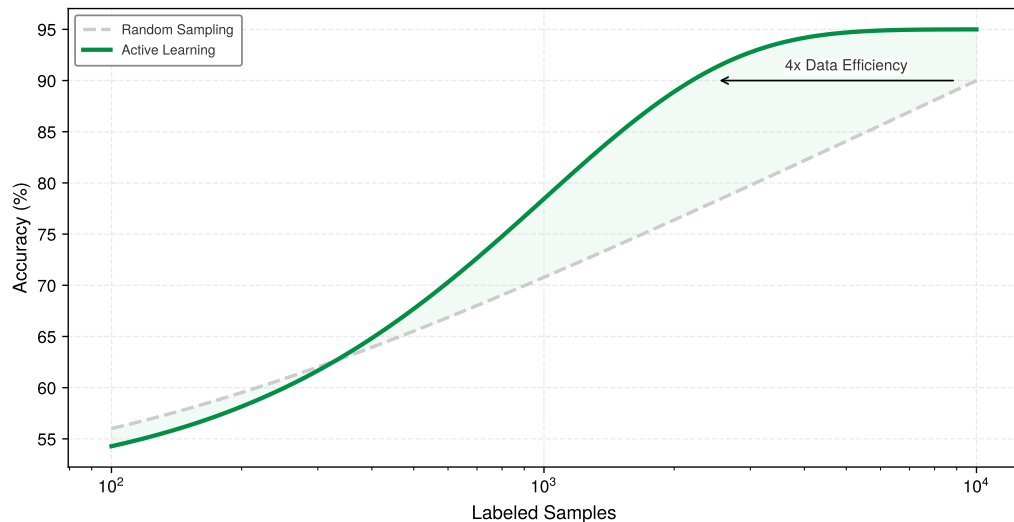
Figure 9.6: The Active Learning Multiplier: Model accuracy vs. number of labeled samples (log scale). Random sampling (gray dashed) yields linear improvements, often requiring massive datasets to capture rare edge cases. Active learning (green solid) targets informative samples, reaching the same accuracy with fewer labels. Curves are illustrative to show the qualitative advantage.
