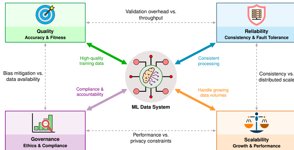
Figure 4.2: The Four Pillars of Data Engineering: Quality, Reliability, Scalability, and Governance form the foundational framework for ML data systems. Each pillar contributes essential capabilities (solid arrows), while trade-offs between pillars (dashed lines) require careful balancing: validation overhead affects throughput, consistency constraints limit distributed scale, privacy requirements impact performance, and bias mitigation may reduce available training data.
