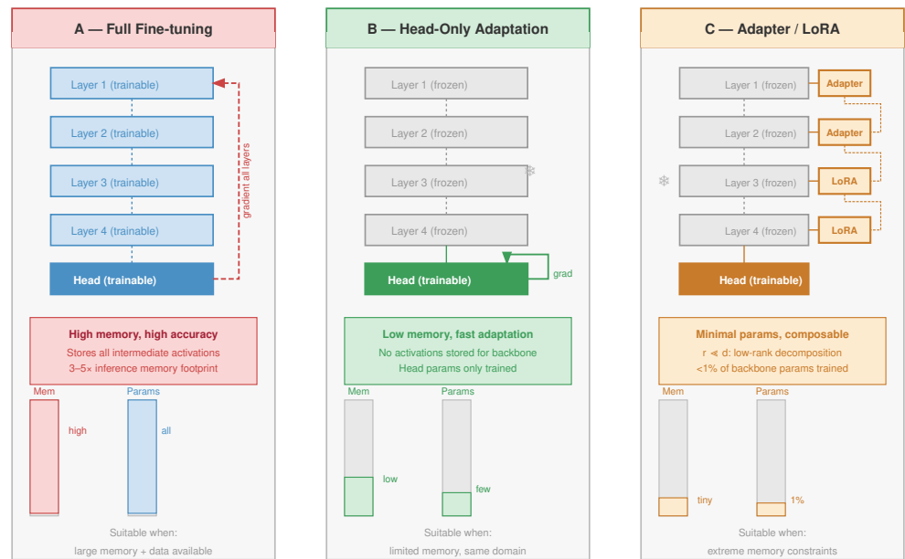
Personalization strategies trade expressivity for memory efficiency; adapters approach near-full accuracy at 1% parameter cost.
