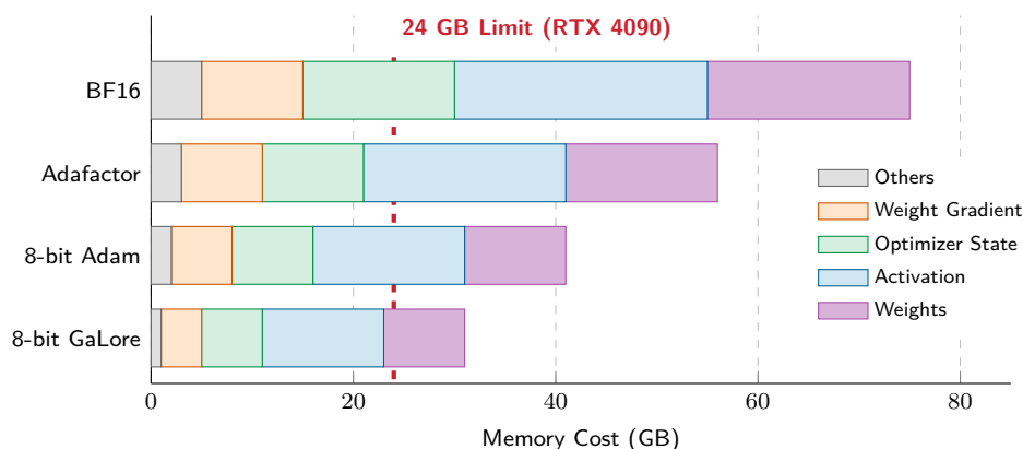
Figure 8.6: Illustrative Memory Footprint Breakdown: Memory usage of a 7-billion-parameter LLaMA model across four memory-efficient optimizer configurations (BF16 Adam, Adafactor, 8-bit Adam, and 8-bit GaLore), decomposed into weights, activations, optimizer state, weight gradients, and other components. The dashed red line marks the RTX 4090 24 GB memory limit. Standard FP32 Adam (omitted from the bars; it requires well above 70 GB for this model) does not fit on a single 24 GB GPU; the bars compare relative memory reductions, but even the smallest illustrated total remains above the 24 GB line, with 8-bit GaLore shrinking optimizer state most aggressively.
