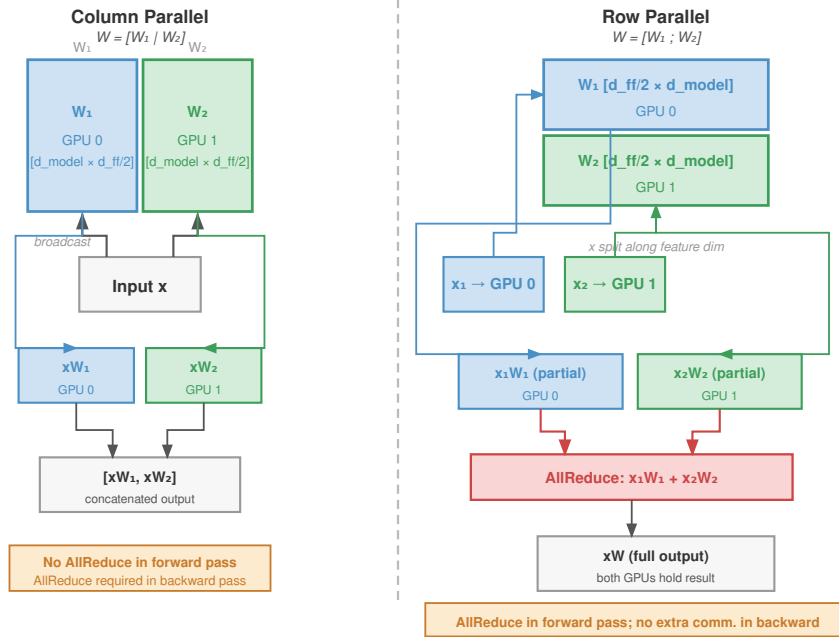
Figure 5.15: Matrix partitioning under tensor parallelism: The first linear layer (for example, QKV) is split column-wise as [W_1|W_2] , and the second (for example, the output projection) is split row-wise as [W_1; W_2] . This Megatron-LM arrangement passes the intermediate result directly between the two splits and requires one AllReduce after the second layer to sum partial outputs.
