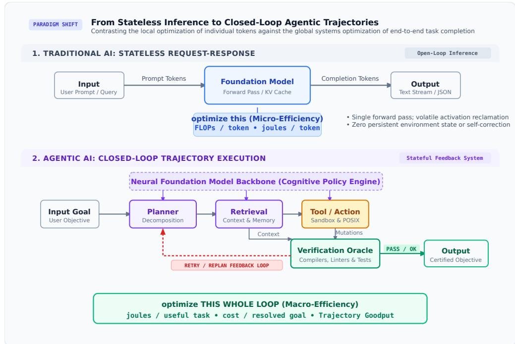
Figure 17.2: From Model Serving to Closed-Loop Agentic Fleets: Traditional ML fleet infrastructure optimizes the micro-efficiency of the open-loop forward pass (FLOPs per token, Joules per token). Emerging agentic workloads shift the unit of optimization to the macro-efficiency of the complete closed loop: coordinating planning, retrieval, tool execution, and deterministic verification to maximize Joules per useful task completed.
