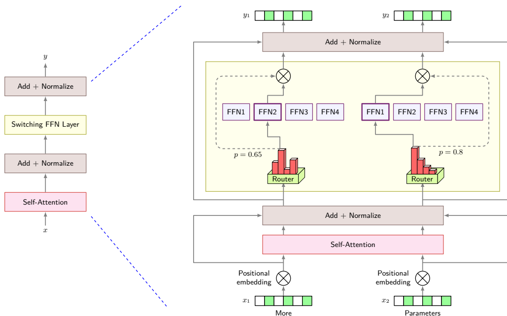
Figure 10.27: Switch Transformer Architecture: Replacing dense feedforward layers with a Switching FFN layer (left) enables sparse conditional routing. A gating network routes each token to a single expert (right) out of a large pool, decoupling total model capacity (parameters) from per-token compute cost (FLOPs). Source: (Fedus et al. 2022).
