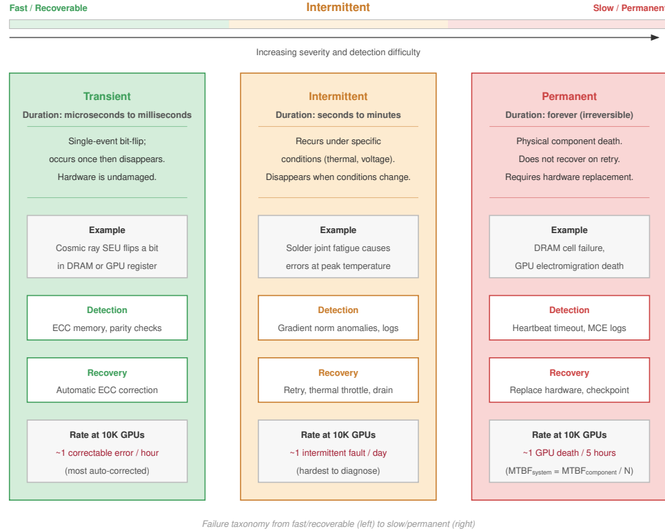
Figure 7.1: The ML Failure Spectrum: Reliability challenges at scale span a temporal taxonomy from transient errors (bit flips, single-event upsets) through intermittent errors (aging, marginal components) to permanent errors (stuck-at faults, dead components). Each category demands different detection latency and recovery strategy, and fault tolerance engineering must address all three to maintain fleet-scale throughput.
