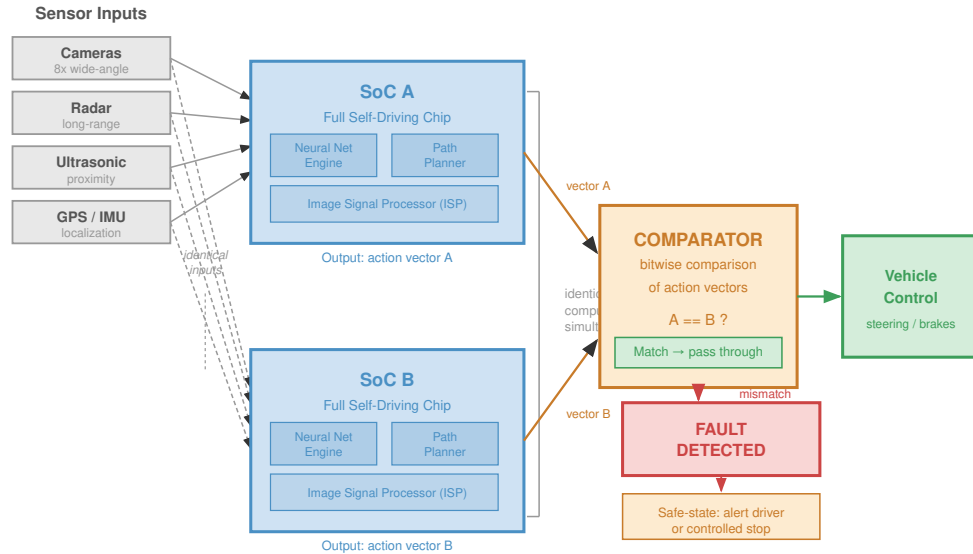
DMR (Dual Modular Redundancy): two independent computation paths; comparator detects any output divergence Tesla FSD chip: two independent SoCs on one package, continuous real-time cross-checking at inference frequency Each SoC contains: 12-core CPU + Neural Processing Unit + ISP + safety MCU
