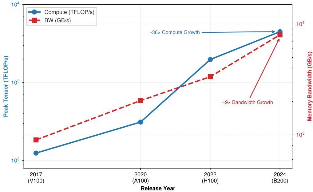
Figure 2.8: The Compute-Memory Divergence: GPU peak Tensor throughput has grown approximately 36× from V100 to B200 when following each generation’s advertised low-precision Tensor Core mode, while HBM bandwidth has grown only 9× over the same period. The widening gap between these curves is the memory wall: each generation of accelerator becomes proportionally more starved for data.
