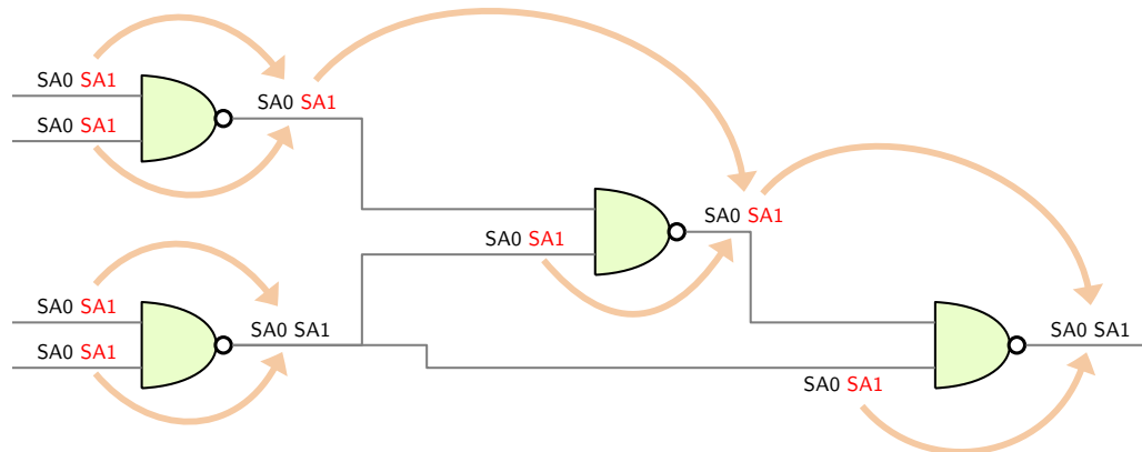
Figure 7.16: Stuck-at Fault Model: Digital logic circuit exhibiting a stuck-at-0 fault, where a signal line remains fixed at a logical 0 regardless of input. Source: accendo reliability.
