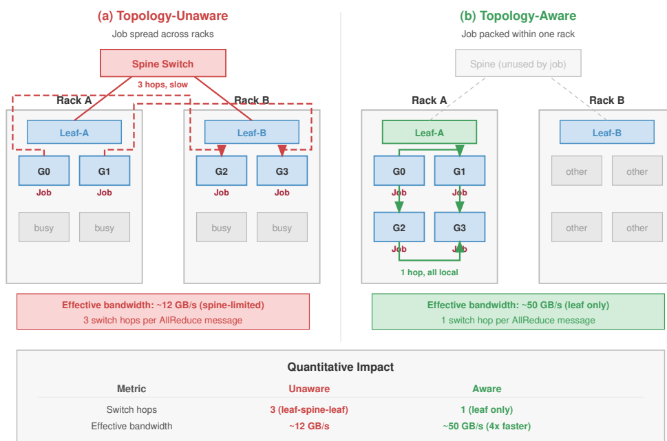
Figure 8.3: Topology-Unaware vs. Topology-Aware Placement: A 4-GPU job placed across two racks (left, topology-unaware) must traverse leaf-spine-leaf hops: 3 switch hops per AllReduce message at about 12 GB/s effective bandwidth. The same 4-GPU job packed within one rack (right, topology-aware) uses a single leaf switch: 1 hop at about 50 GB/s, roughly 4× faster. A quantitative summary beneath the figure reports switch-hop counts and effective bandwidth.
