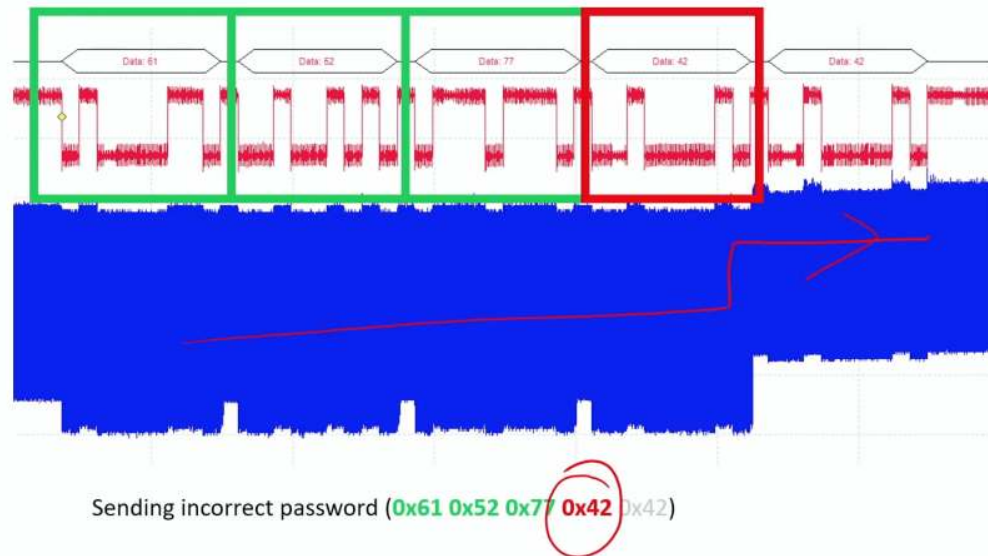
Figure 13.13: Side-Channel Attack Vulnerability: Power consumption patterns reveal cryptographic key information during authentication; consistent power usage indicates correct password bytes, while abrupt changes signal incorrect input and halted processing. Even without knowing the password, an attacker can infer it by analyzing the device's power usage during authentication attempts. Source: Colin O'Flynn.
