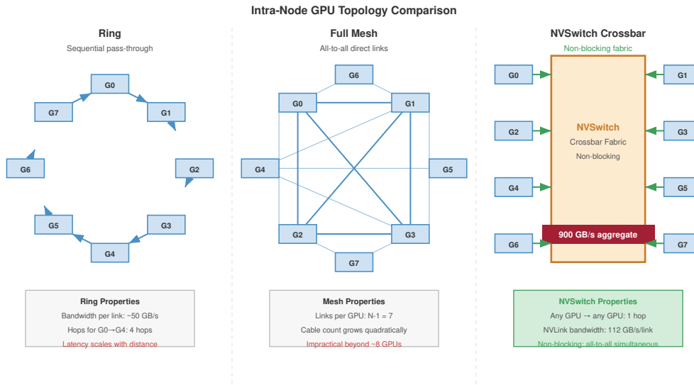
Figure 2.11: Intra-Node GPU Topology Comparison: Three approaches to wiring GPUs inside a node. (Left) Ring: sequential pass-through, ~50 GB/s per link, latency scales with distance. (Center) Full Mesh: all-to-all direct links, N - 1 links per GPU, impractical beyond ~8 GPUs. (Right) NVSwitch Crossbar: non-blocking fabric with 112 GB/s per NVLink and 900 GB/s aggregate, any-GPU-to-any-GPU in one hop, enabling tensor-parallel AllReduce within a node.
