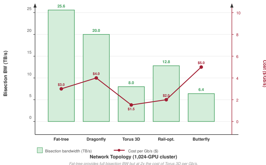
Figure 3.10: Network Topologies for ML: An Illustrative Bandwidth-Cost Scenario: Assumed BW_{\text{bisection}} (TB/s, left axis) and cost per Gb/s (right axis) for five topology configurations on a 1,024-GPU cluster: Fat-tree (25.6 TB/s, $3.0/Gb/s), Dragonfly (20.0, $4.0), Torus 3D (8.0, $1.5), Rail-opt (12.8, $2.0), and Butterfly (6.4, $5.0). These scenario values illustrate the comparison method rather than universal properties of each topology family.
