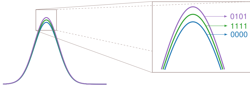
Figure 13.16: Power Traces: Cryptographic computations reveal subtle, data-dependent variations in power consumption that reflect internal states during specific operations.
