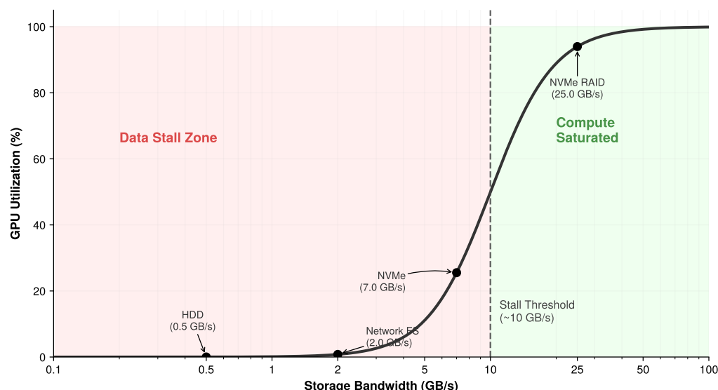
Figure 4.4: The Data Stall Frontier: GPU utilization follows a steep S-curve as a function of storage bandwidth. Around the stall threshold (~10 GB/s for a typical 8-GPU node), utilization crosses from waiting-dominated to compute-dominated. The position of common storage technologies on this curve explains why tiered architectures are essential.
