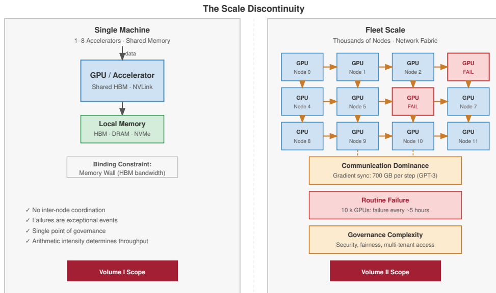
Figure 1.2: The Scale Discontinuity: Single-machine systems (left) are governed by local memory bandwidth and operate with no inter-node coordination, exceptional failures, and a single point of governance. Fleet-scale systems (right) introduce communication dominance, routine hardware failure, and governance complexity as first-order engineering constraints.
