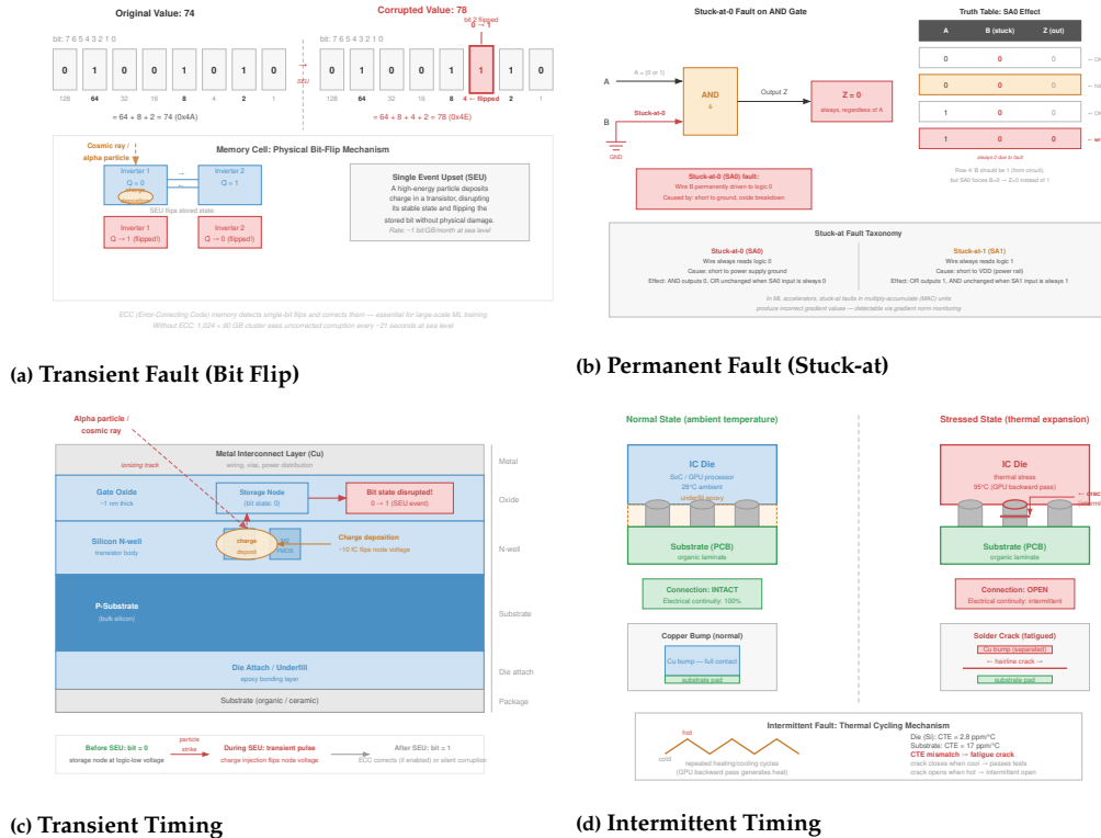
Figure 7.12: Temporal Taxonomy of Hardware Faults: Four panels show how the three temporal categories manifest in practice. Transient panels (bit flip and timing glitch) show temporary disruptions that do not cause permanent damage. The Intermittent panel shows sporadic errors driven by unstable conditions or aging. The Permanent panel (stuck-at-0/1) shows irreversible physical damage that requires replacement.
