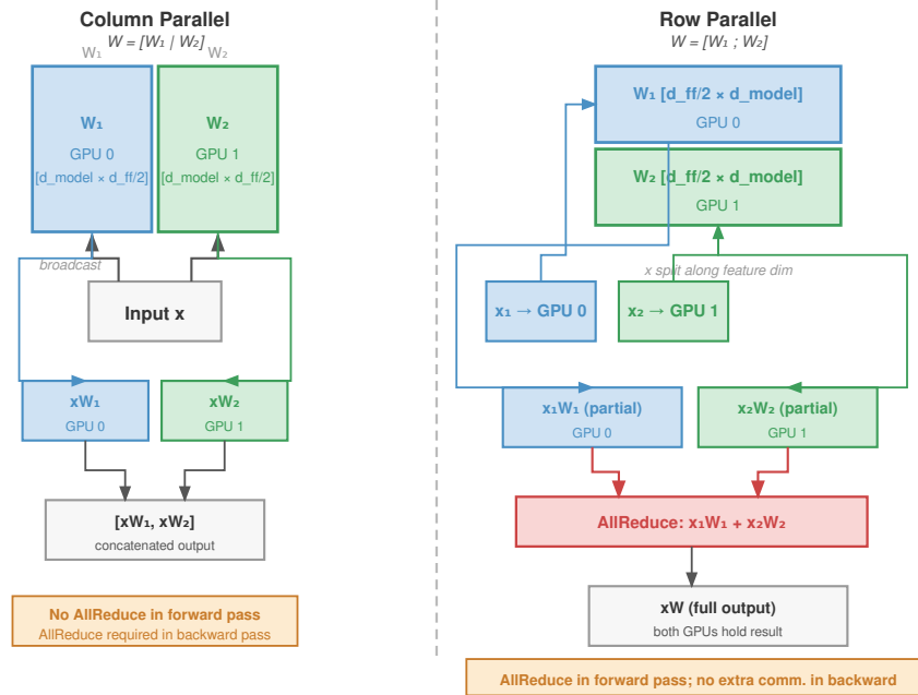
Figure 5.14: Tensor Parallelism - Matrix Partitioning: Illustration of Megatron-LM style tensor parallelism. The first linear layer (e.g., QKV) is split column-wise [W_1 | W_2] . The second layer (e.g., Output) is split row-wise \begin{bmatrix} W_1 \\ W_2 \end{bmatrix} . This arrangement allows the output of the first layer to flow directly into the second without synchronization, requiring only one AllReduce after the second layer to sum the partial results.
