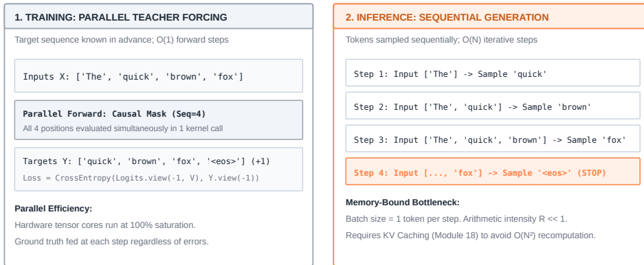
Figure 15.2: Teacher forcing versus autoregressive text generation: In training, teacher forcing presents the full sequence simultaneously, utilizing causal masking so position t predicts target t + 1 ( O(1) parallel passes). In autoregressive inference, generation proceeds iteratively token-by-token, taking the last logit row, sampling with temperature/top- k , and appending to the prompt prefix ( O(T) sequential passes).
