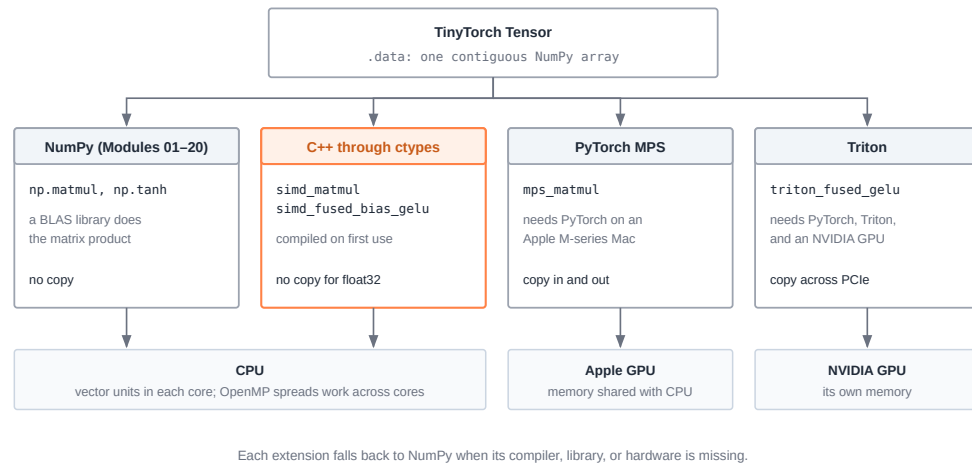
Figure 24.1: Four ways to run an operation on a TinyTorch Tensor. The modules use NumPy. The extensions reach the CPU’s vector units directly through compiled C++, or move the data to a GPU and back.
