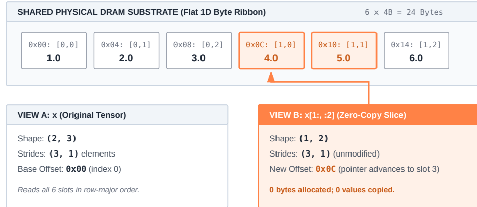
Figure 1.3: Zero-copy slicing and stride manipulation: Slicing advances the base memory offset pointer without allocating new memory, while strided views navigate the flat 1D ribbon in row-major or transposed order.
