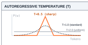
Temperature scaling reshaping logit probabilities ( T \rightarrow 0 vs T > 1 ).
