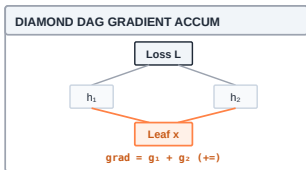
Diamond DAGs require gradient accumulation:
