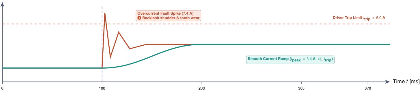
⚡ (c) Actuator Phase Current i(t) [A] & Gearbox Backlash Stress
