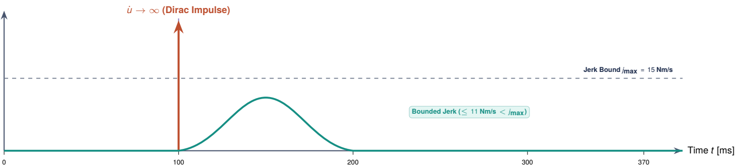
(b) Torque Rate of Change \dot{u}(t) \propto \ddot{q}(t) (Actuator Jerk) [Nm/s]
