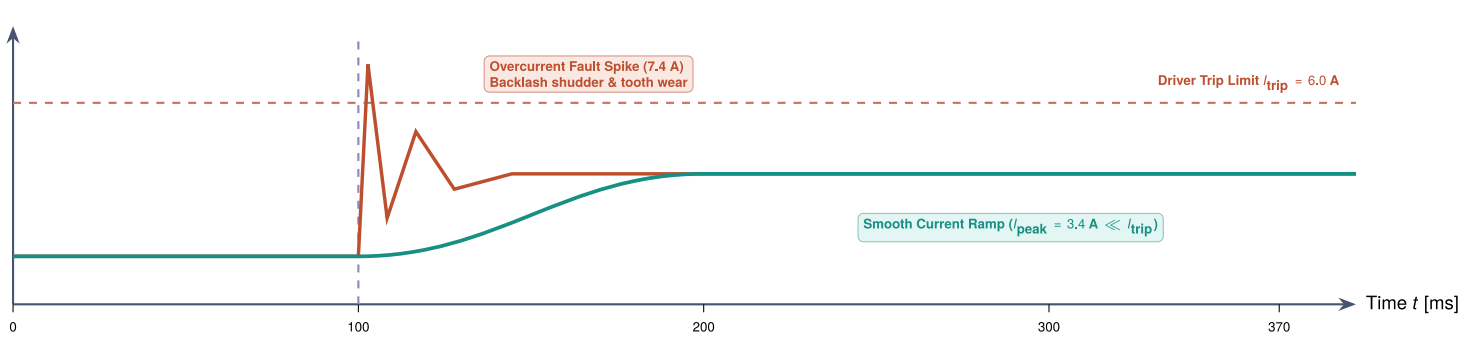
(c) Actuator Phase Current i(t) [A] & Gearbox Backlash Stress
