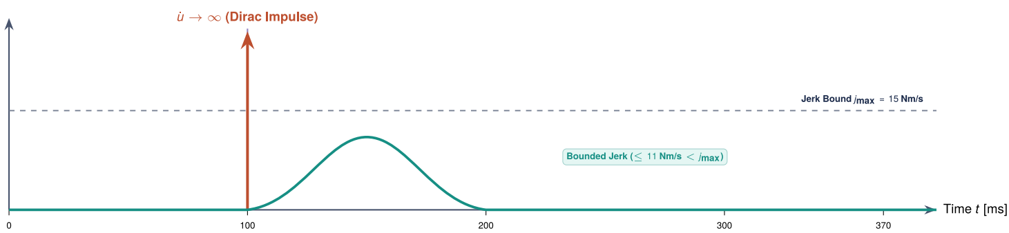
(b) Torque Rate of Change \dot{u}(t) \propto \ddot{q}(t) (Actuator Jerk) [Nm/s]
