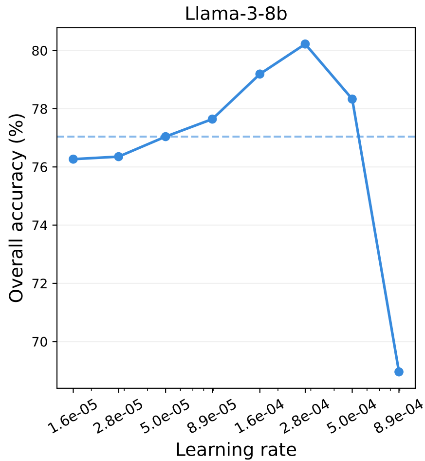
\mathcal{D}_{\text{train}} fine-tuning by model: overall accuracy vs learning rate
