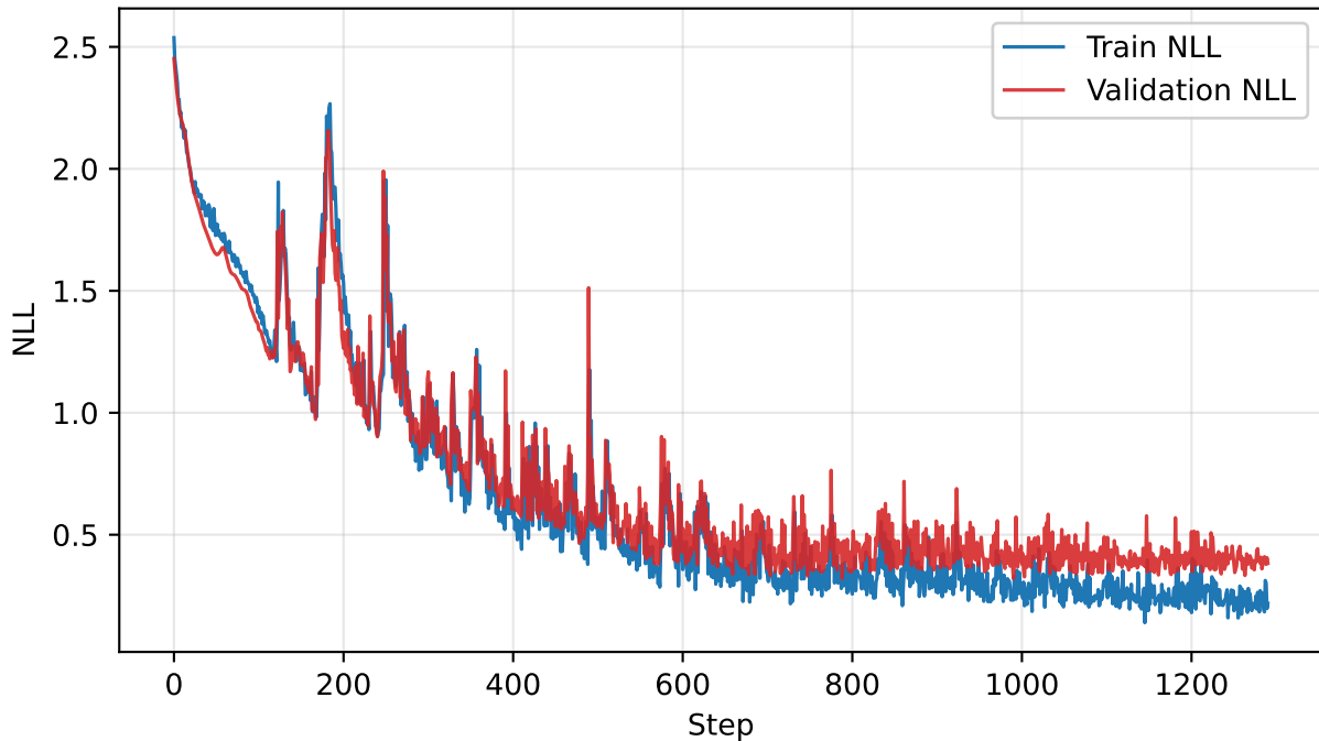
Final model: train vs validation NLL
