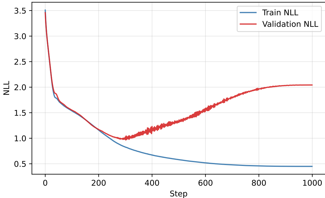
Tiny subset (128 points): train vs validation NLL
