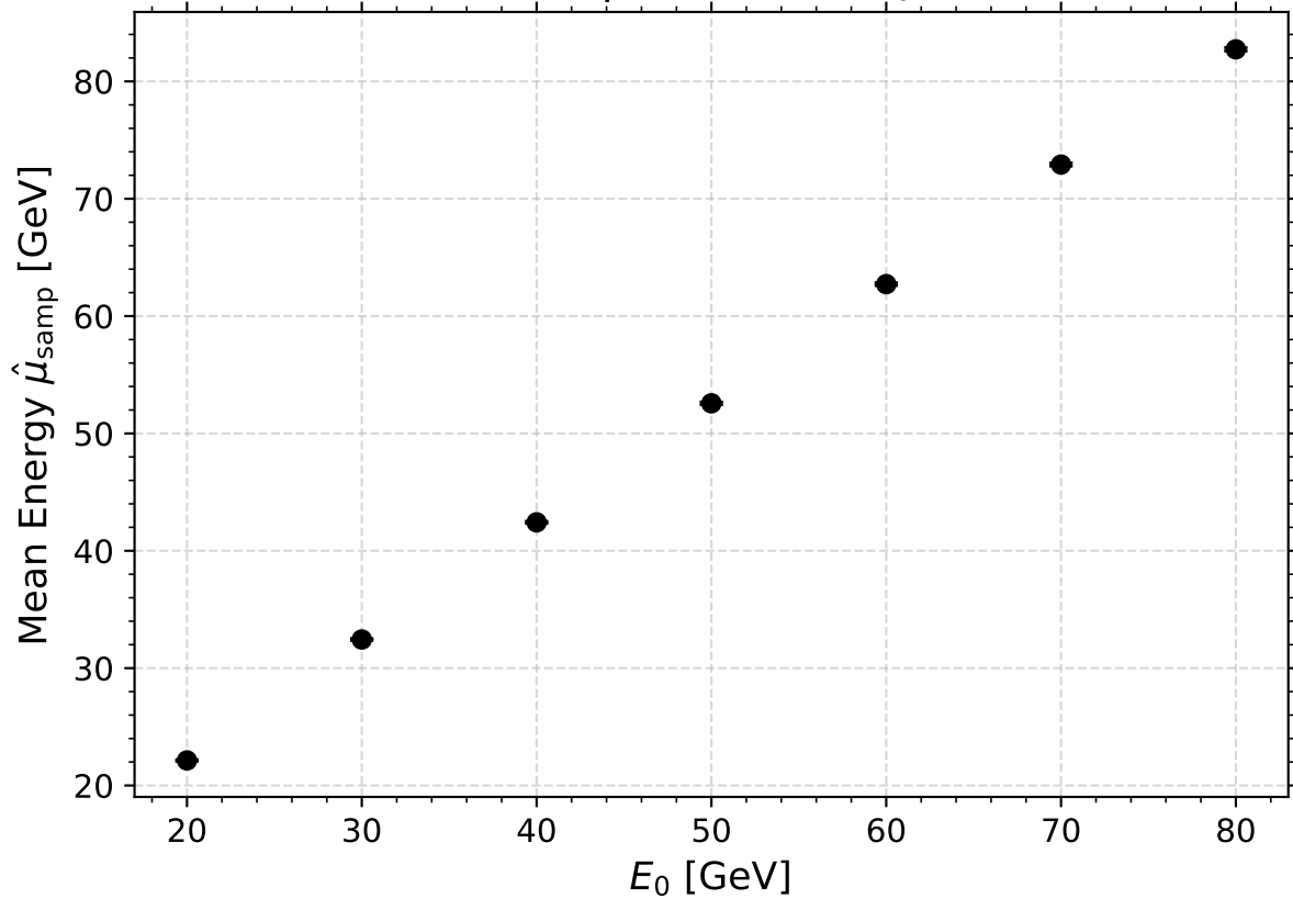
Sample Mean vs E_0
