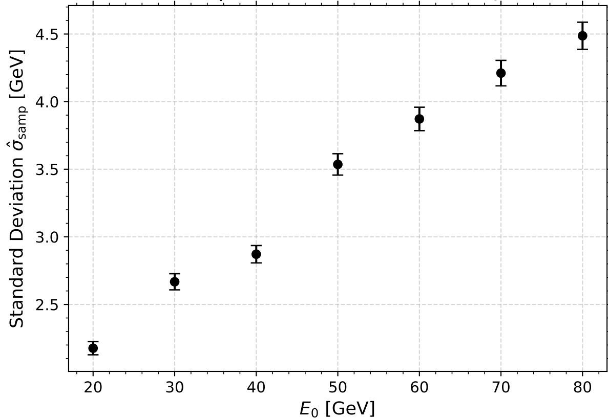
Sample Standard Deviation vs E_0
