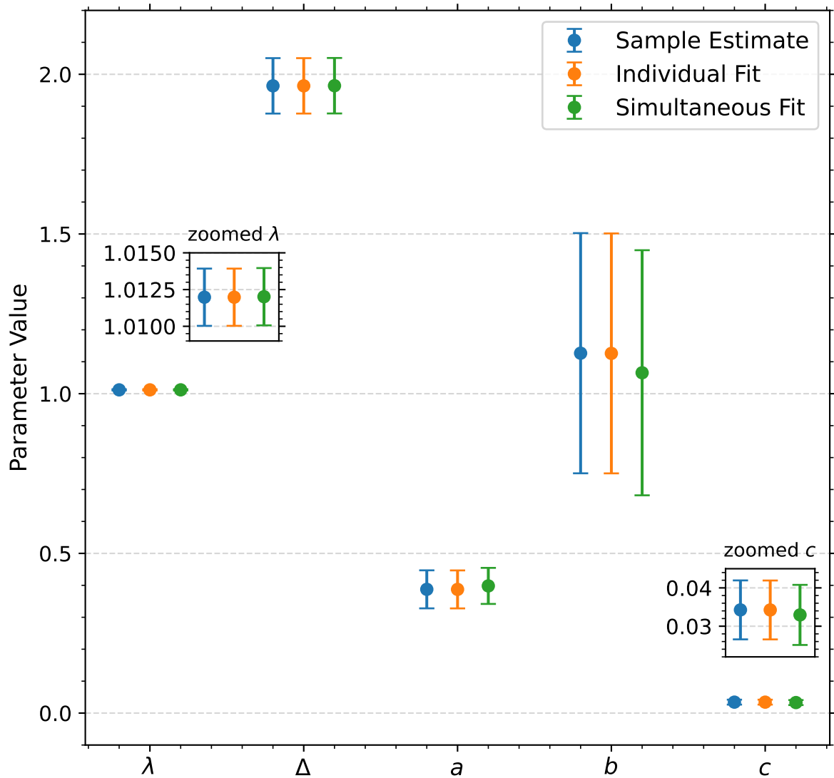
Figure 3.2: Parameter Values by Method
