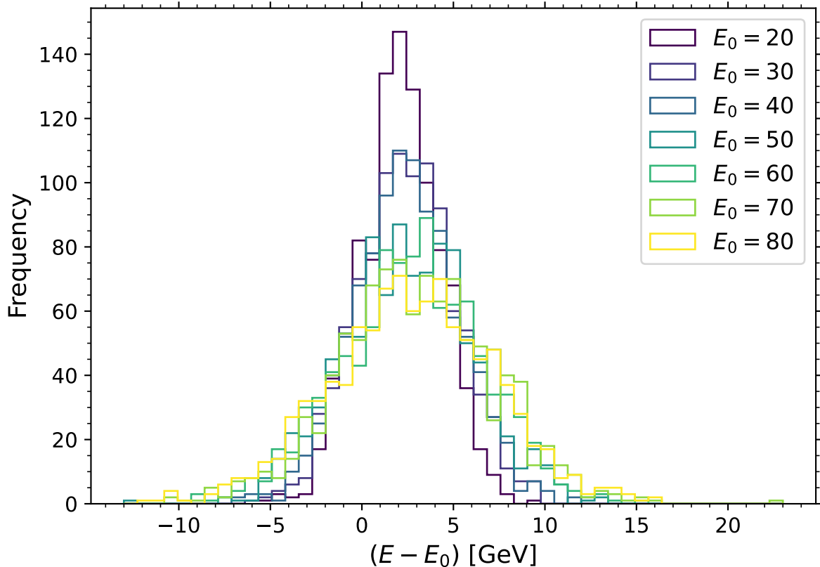
Figure 1.2: Overlaid Residual Distributions
