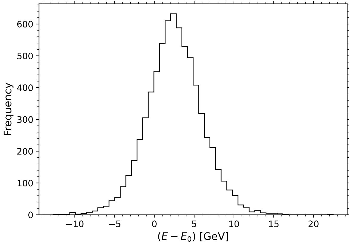
Figure 1.1: Distribution of Residuals
